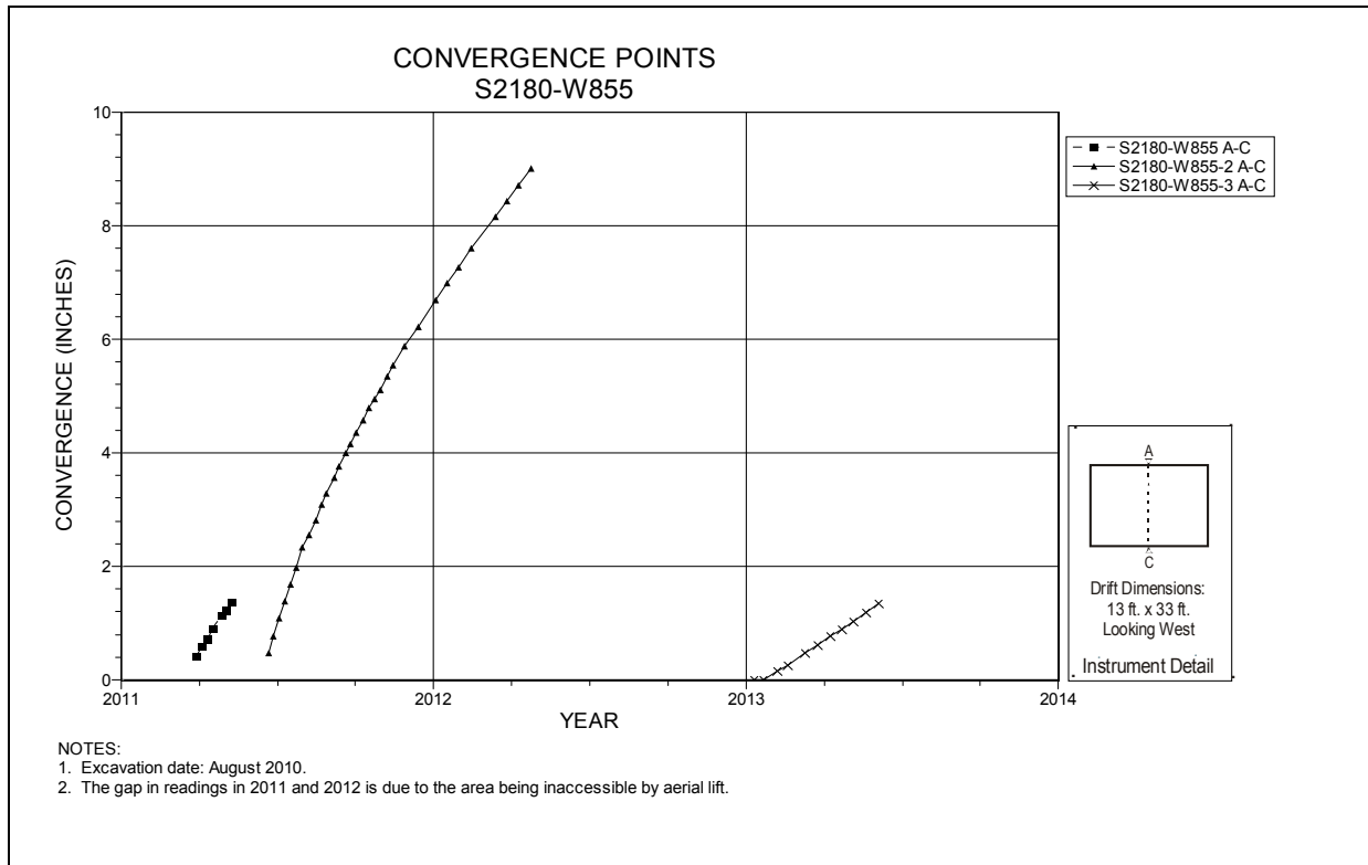
Figure 5-82 Convergence Point Array S2180 W855 – Roof to Floor
