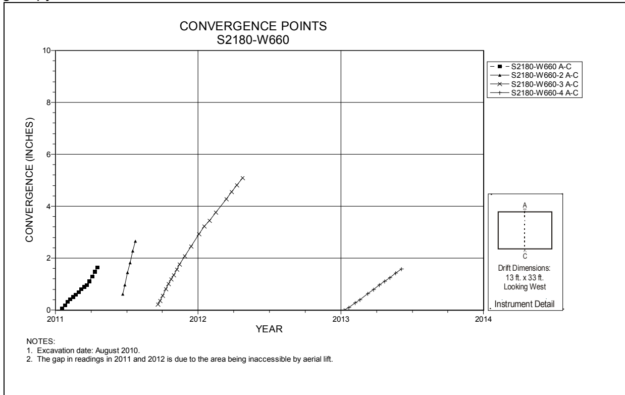
Figure 5-79 Convergence Point Array S2180 W660 Intersection (Room 3 Panel 7) – Roof to Floor
