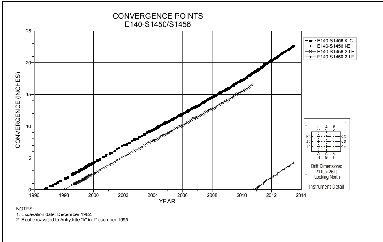
Figure 4-87 Convergence Point Array E140 S1450/S1456 – Rib to Rib Quarter Points
