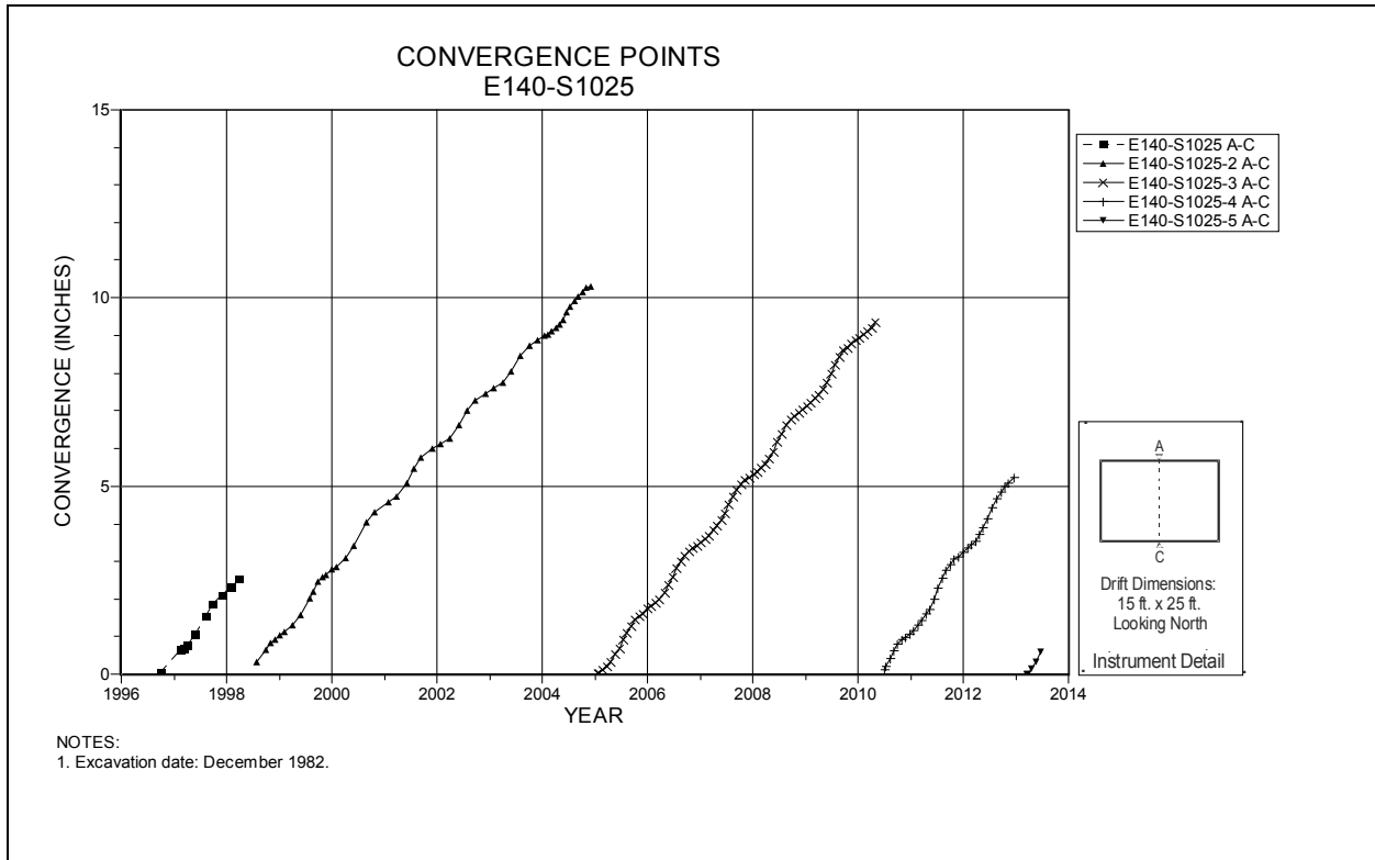
Figure 4-71 Convergence Point Array E140 S1025 – Roof to Floor
