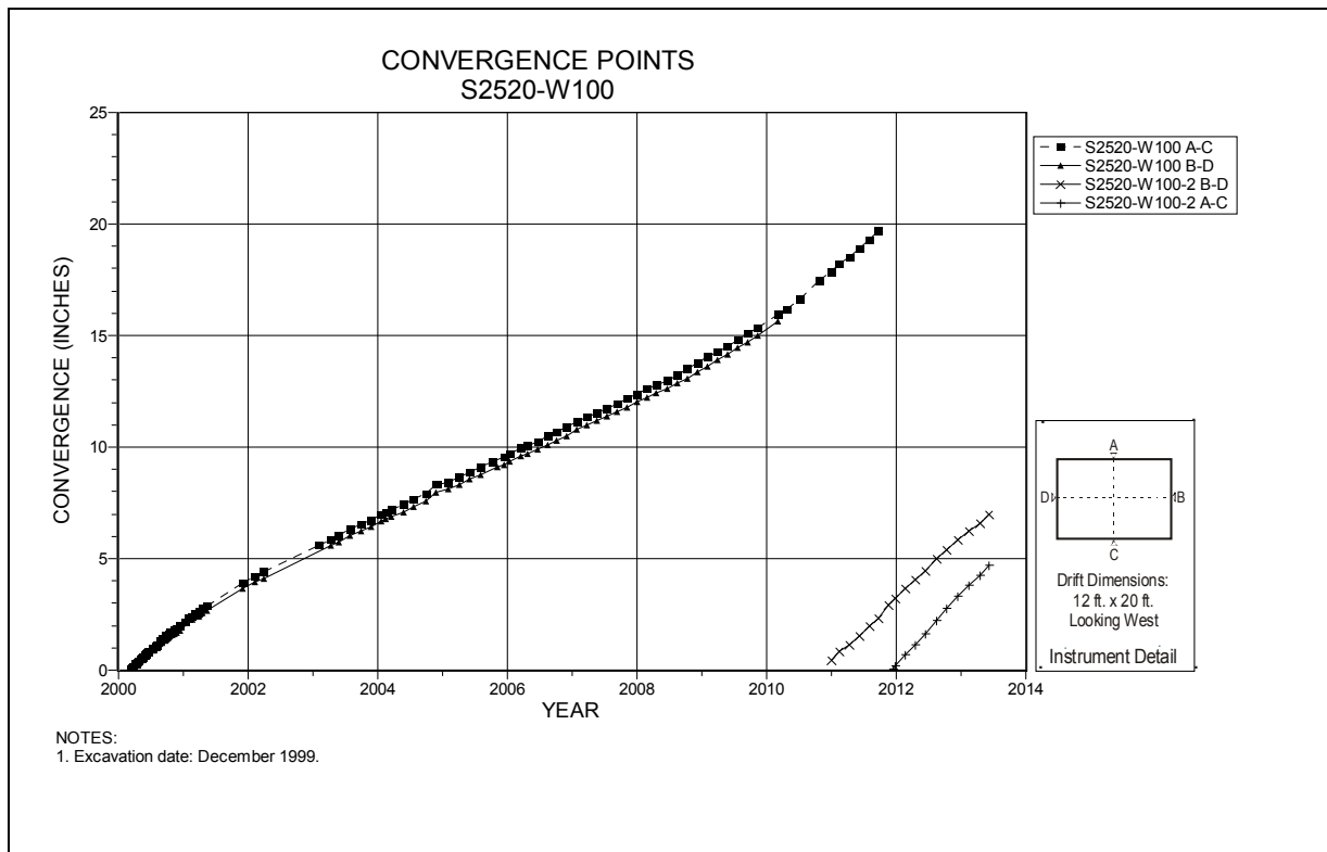
Figure 4-186 Convergence Point Array S2520 W100 – All Chords
