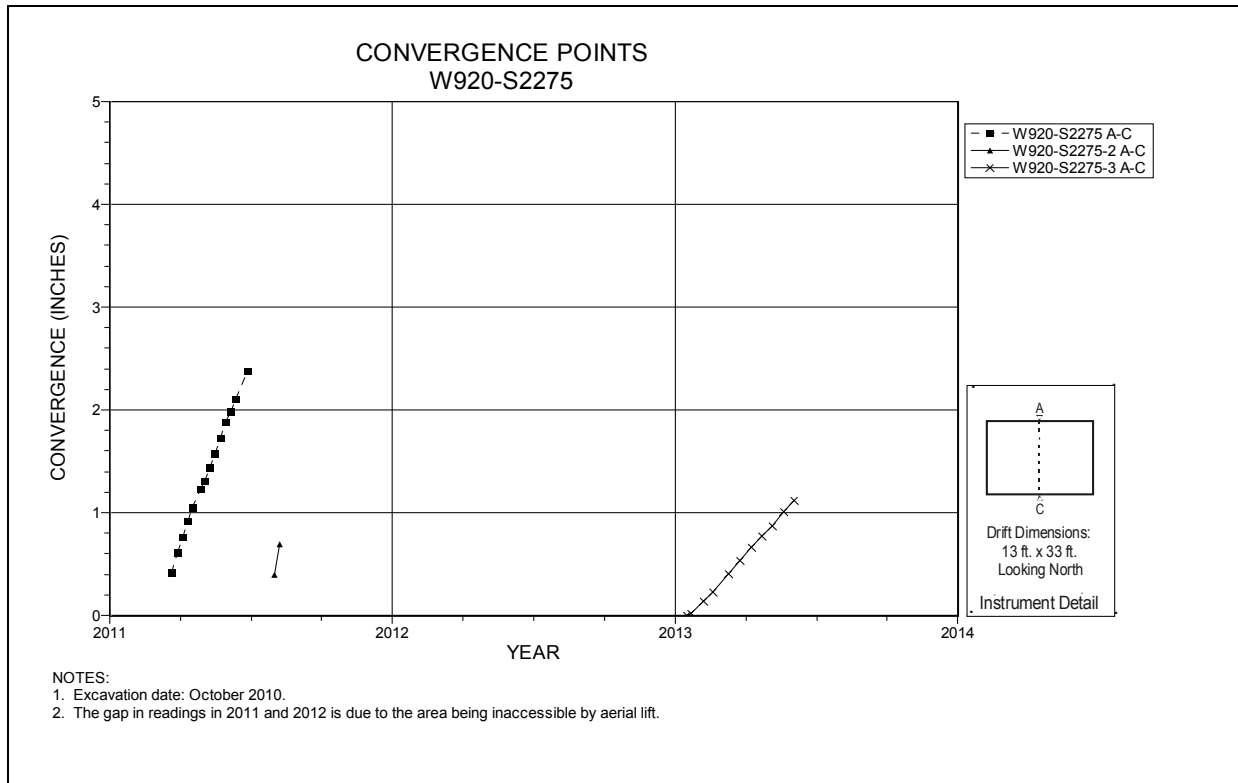
Figure 5-100 Convergence Point Array Room 5, Panel 7 at W920 S2275 – Roof to Floor
