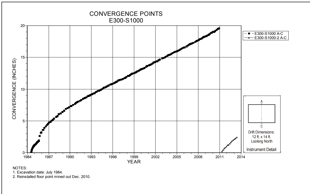
Figure 4-132 Convergence Point Array E300 S1000 – Roof to Floor
