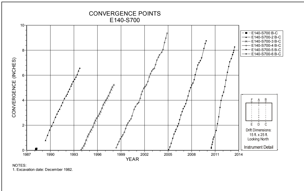
Figure 4-66 Convergence Point Array E140 S700 – Roof to Floor – East Quarter Point
