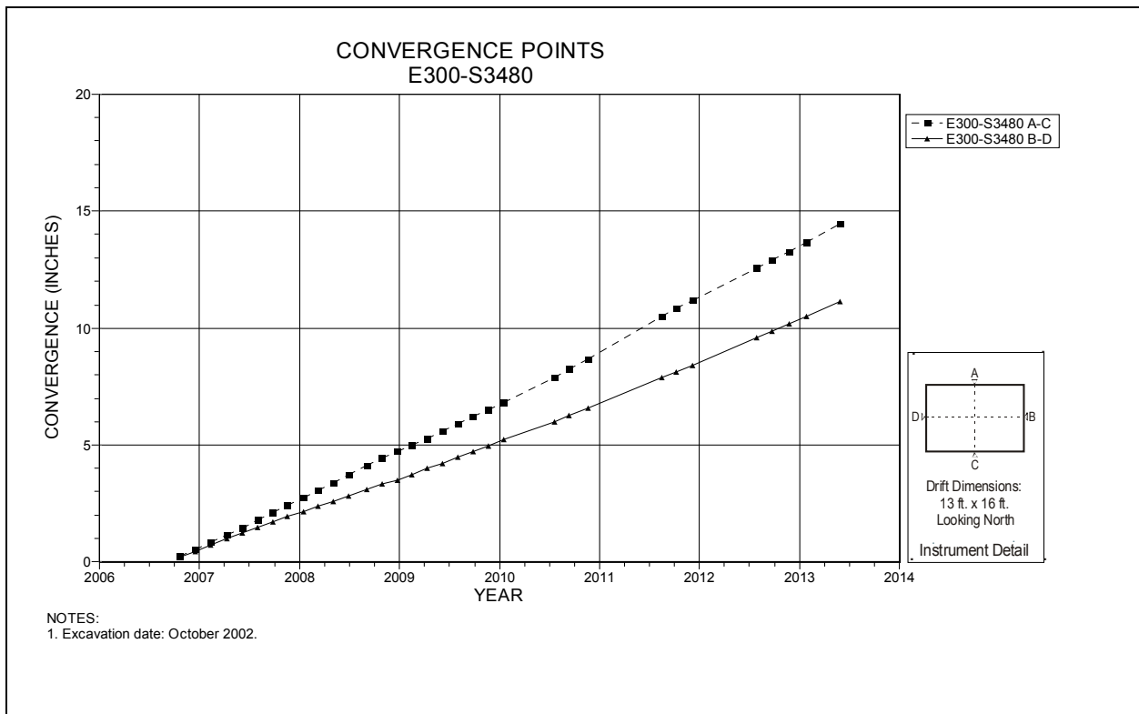
Figure 4-150 Convergence Point Array E300 S3480 – All Chords
