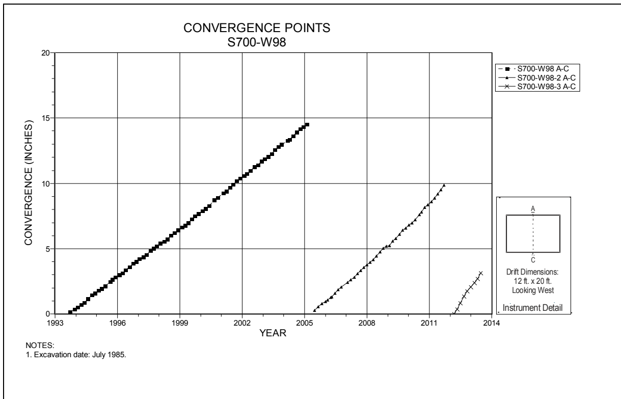
Figure 4-168 Convergence Point Array S700 W98 – Roof to Floor
