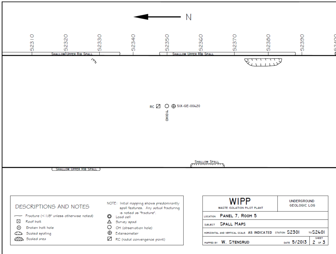
Figure 7-21 Panel 7 Room 5, S2301-S2401 Roof Fractures
