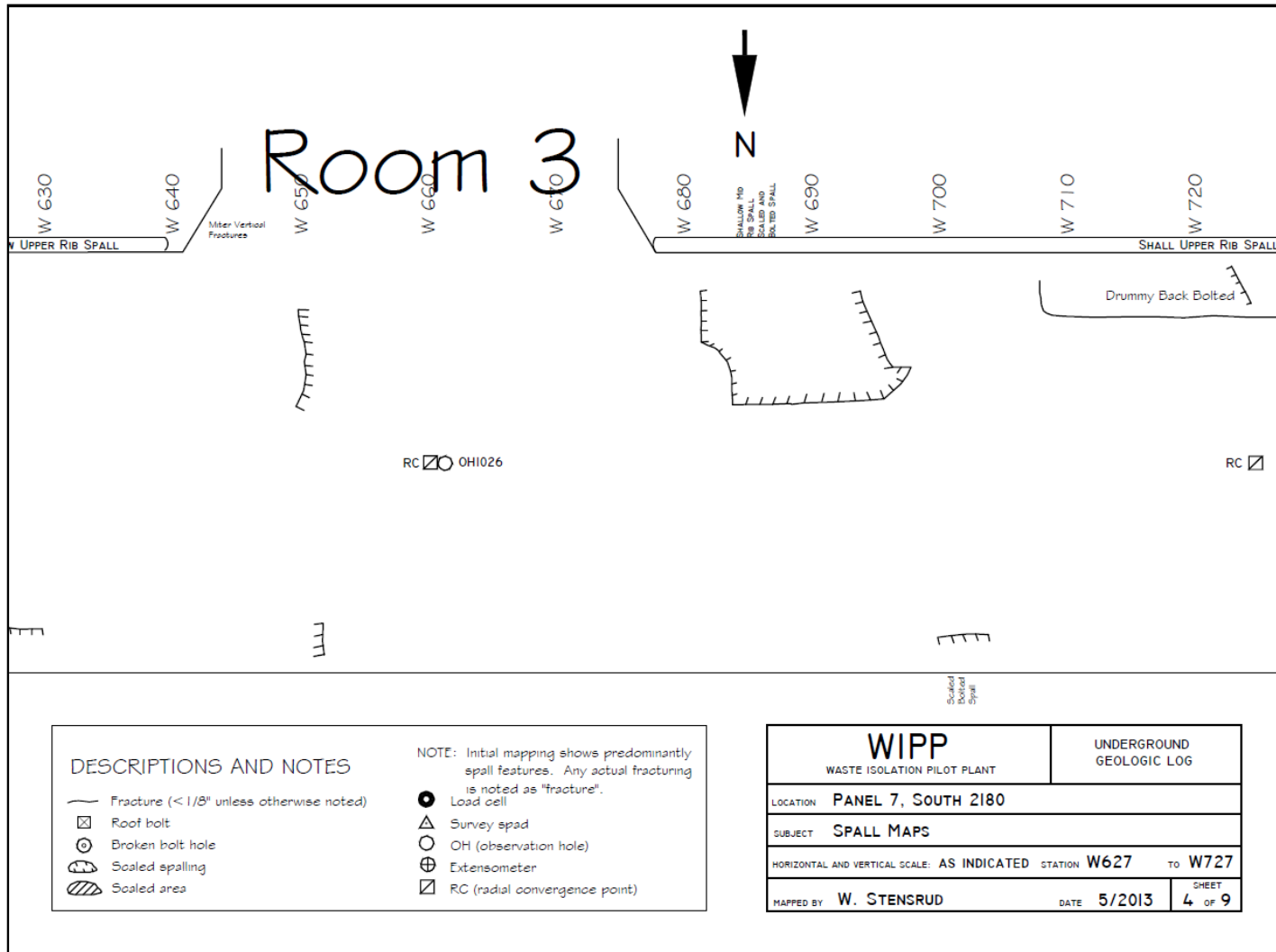
Figure 7-32 Panel 7 South 2180, W627-W727 Roof Fractures
