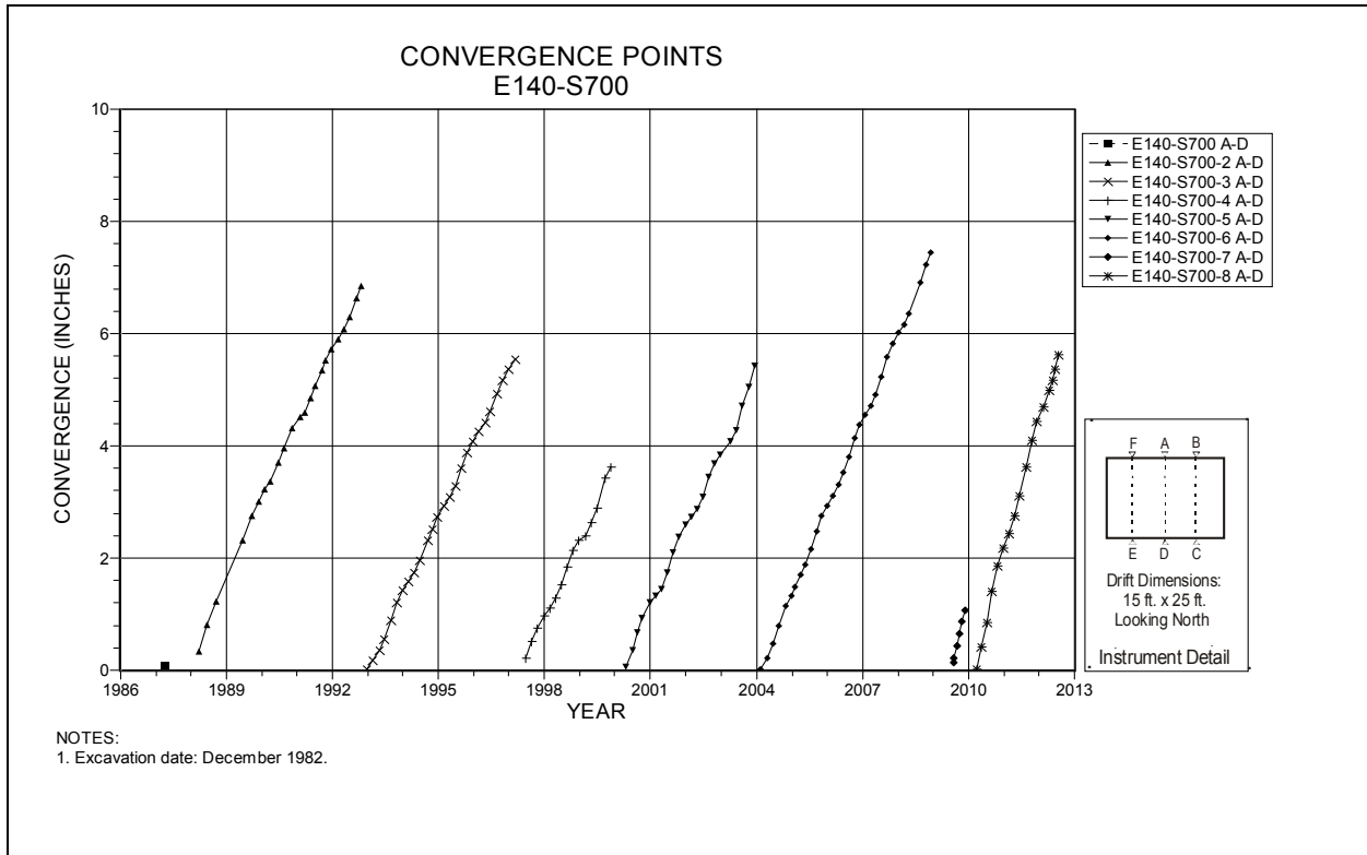
Figure 4-65 Convergence Point Array E140 S700 – Roof to Floor – Centerline
