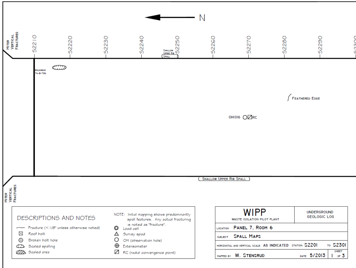
Figure 7-23 Panel 7 Room 6, S2201-S2301 Roof Fractures
