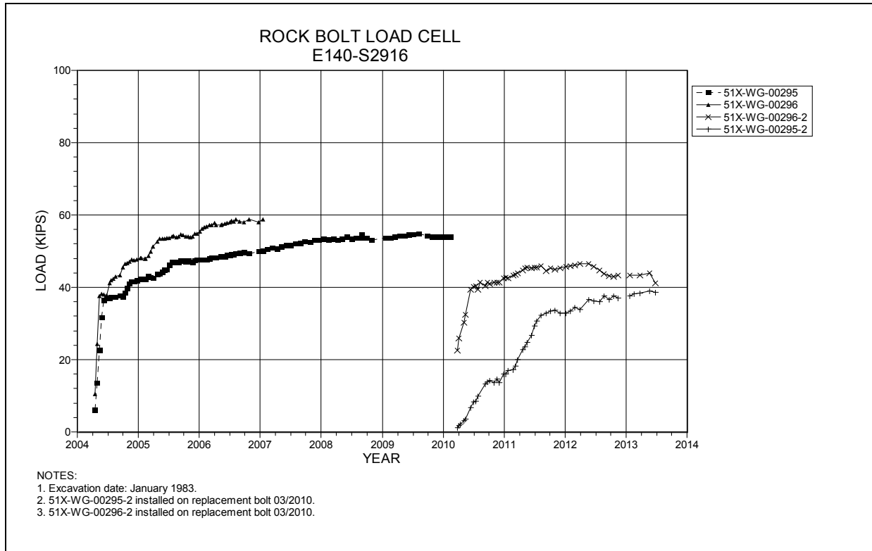
Figure 4-277 Rock Bolt Load Cells E140 S2916
