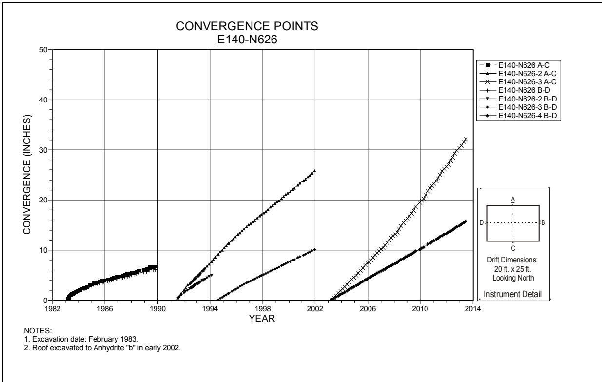
Figure 4-54 Convergence Point Array E140 N626 – All Chords
