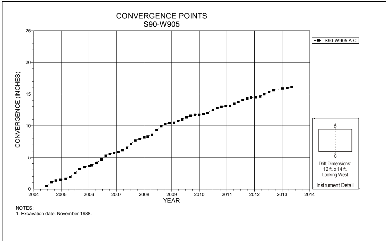
Figure 4-163 Convergence Point Array S90 W905 – Roof to Floor
