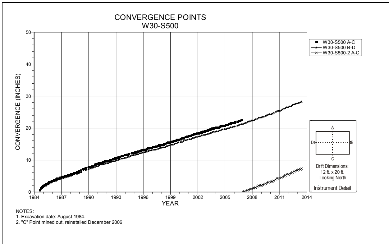
Figure 4-202 Convergence Point Array W30 S500 – All Chords
