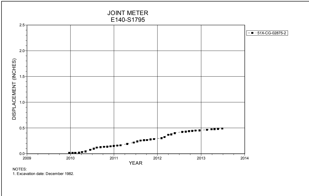
Figure 4-269 Joint Meter E140 S1795
