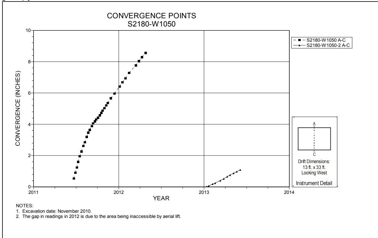
Figure 5-85 Convergence Point Array S2180 W1050 Intersection (Room 6, Panel 7) – Roof to Floor
