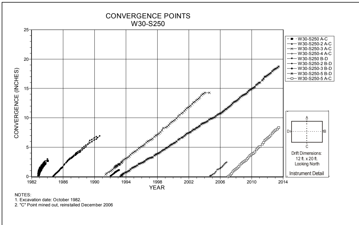
Figure 4-200 Convergence Point Array W30 S250 – All Chords
