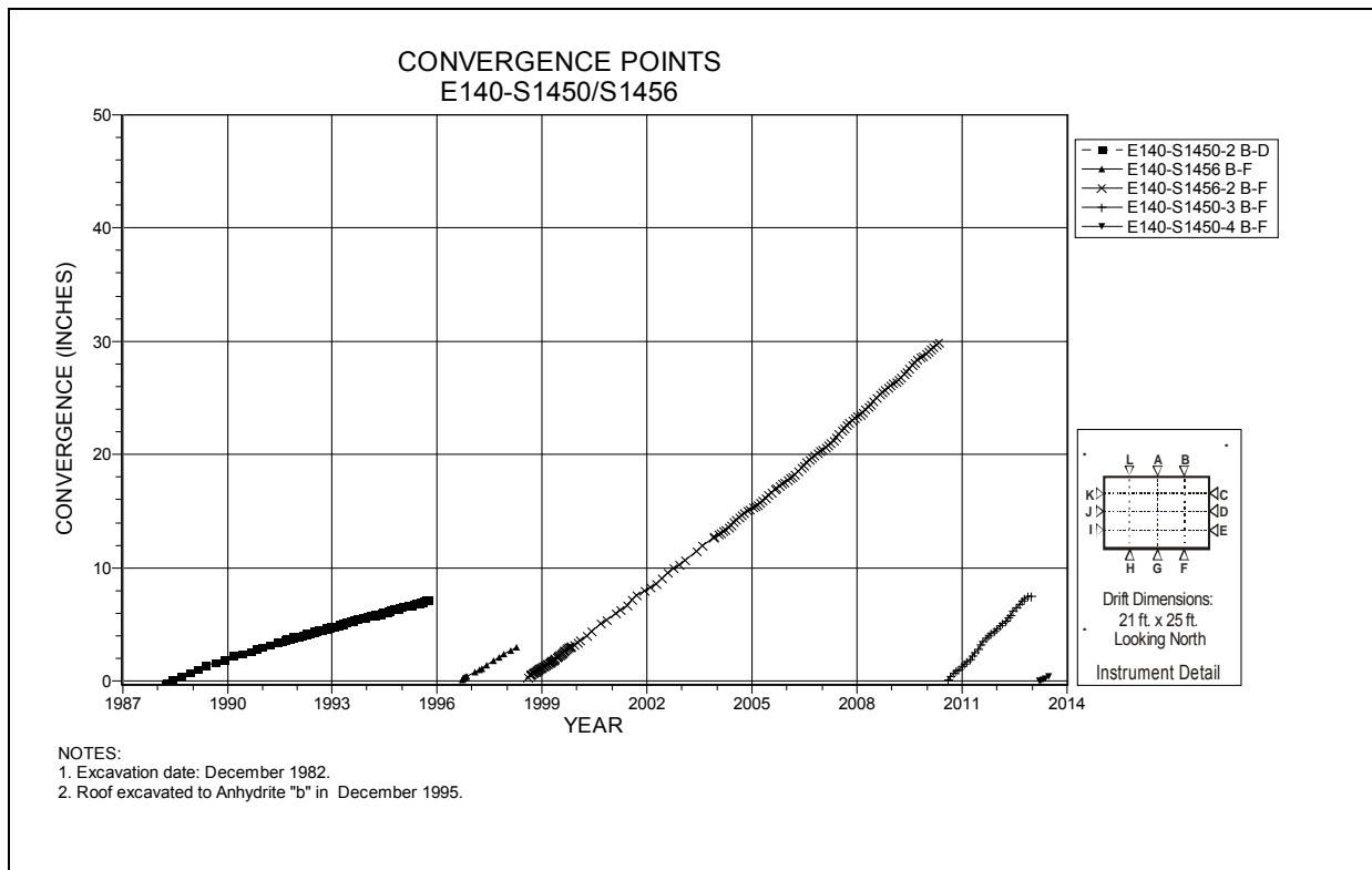
Figure 4-86 Convergence Point Array E140 S1450/S1456 – Roof to Floor – East Quarter Point
