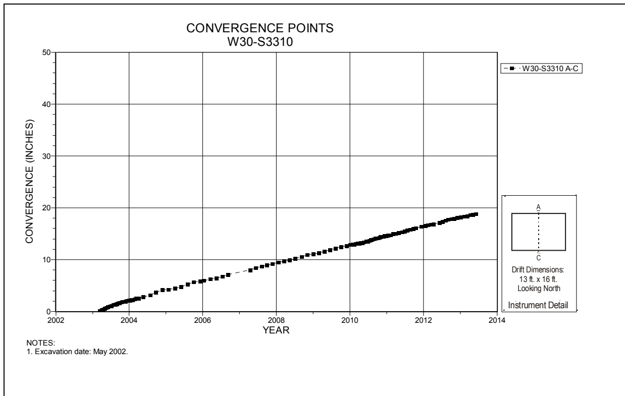
Figure 4-226 Convergence Point Array W30 S3310 – Roof to Floor
