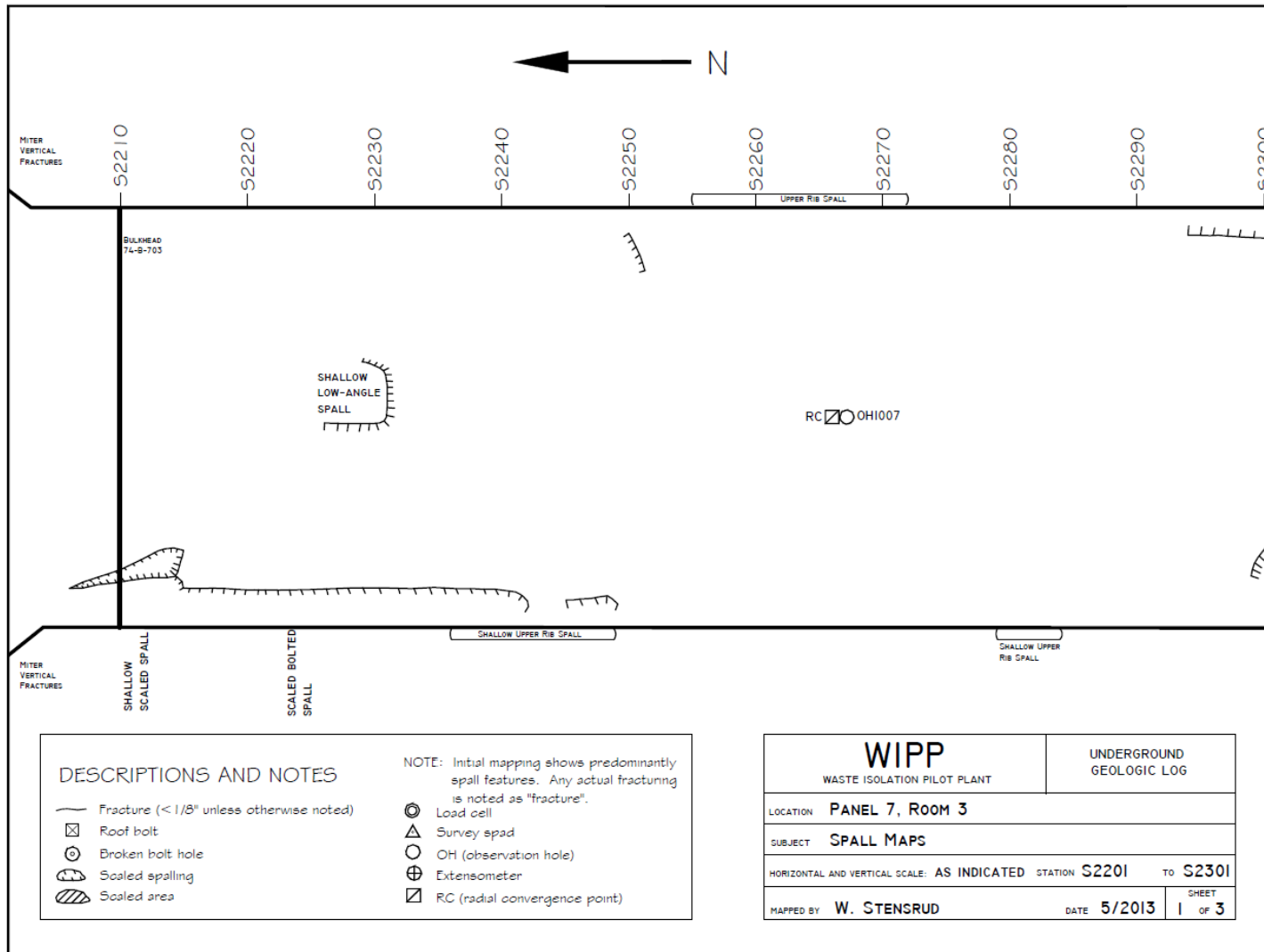
Figure 7-14 Panel 7 Room 3, S2201-S2301 Roof Fractures
