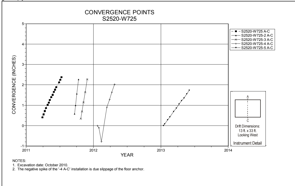
Figure 5-115 Convergence Point Array S2520 W725 – Roof to Floor
