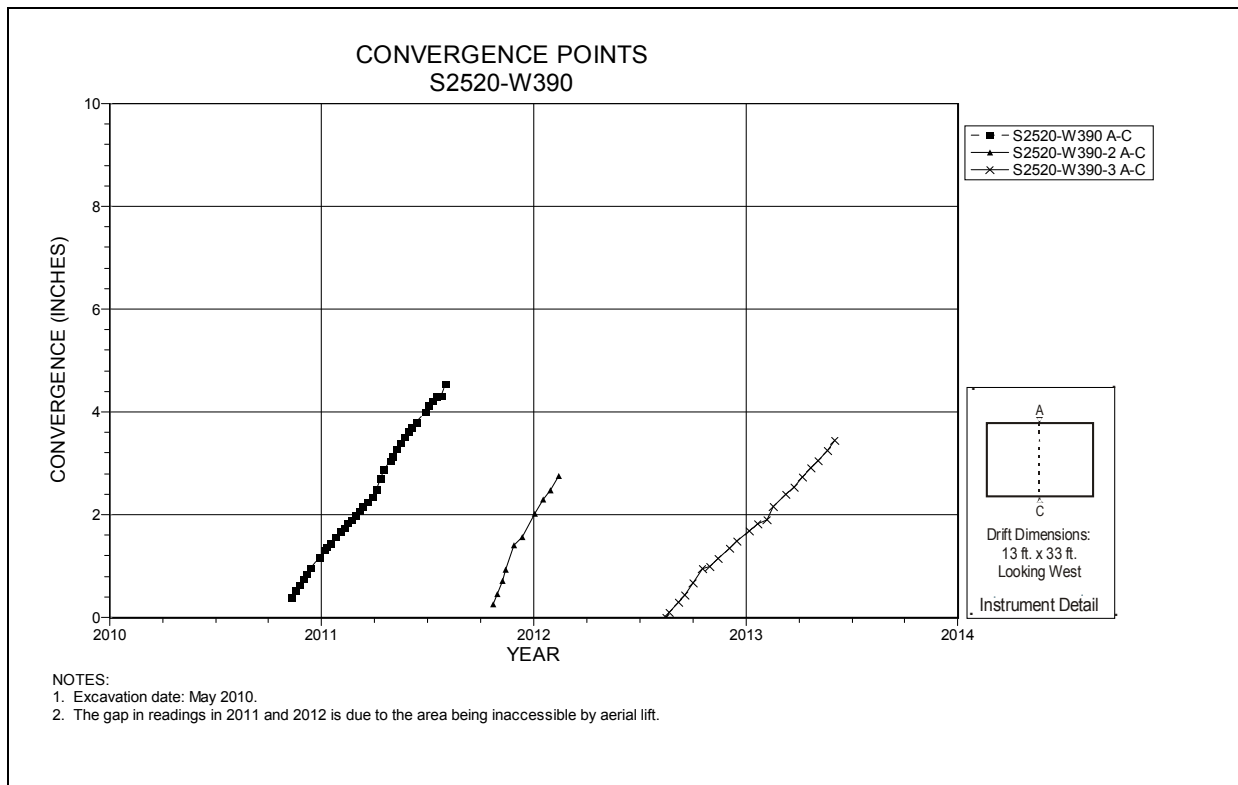
Figure 5-110 Convergence Point Array S2520 W390 Intersection (Room 1, Panel 7) – Roof to Floor
