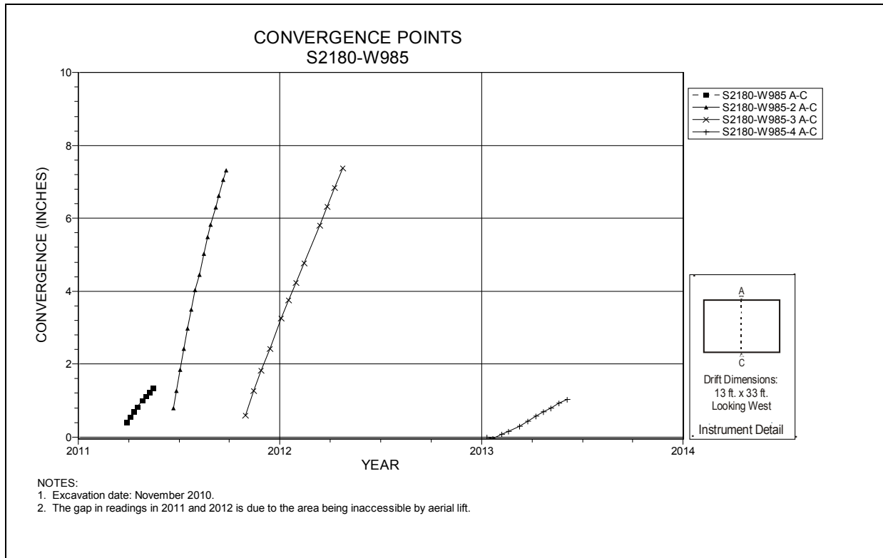
Figure 5-84 Convergence Point Array S2180 W985 – Roof to Floor
