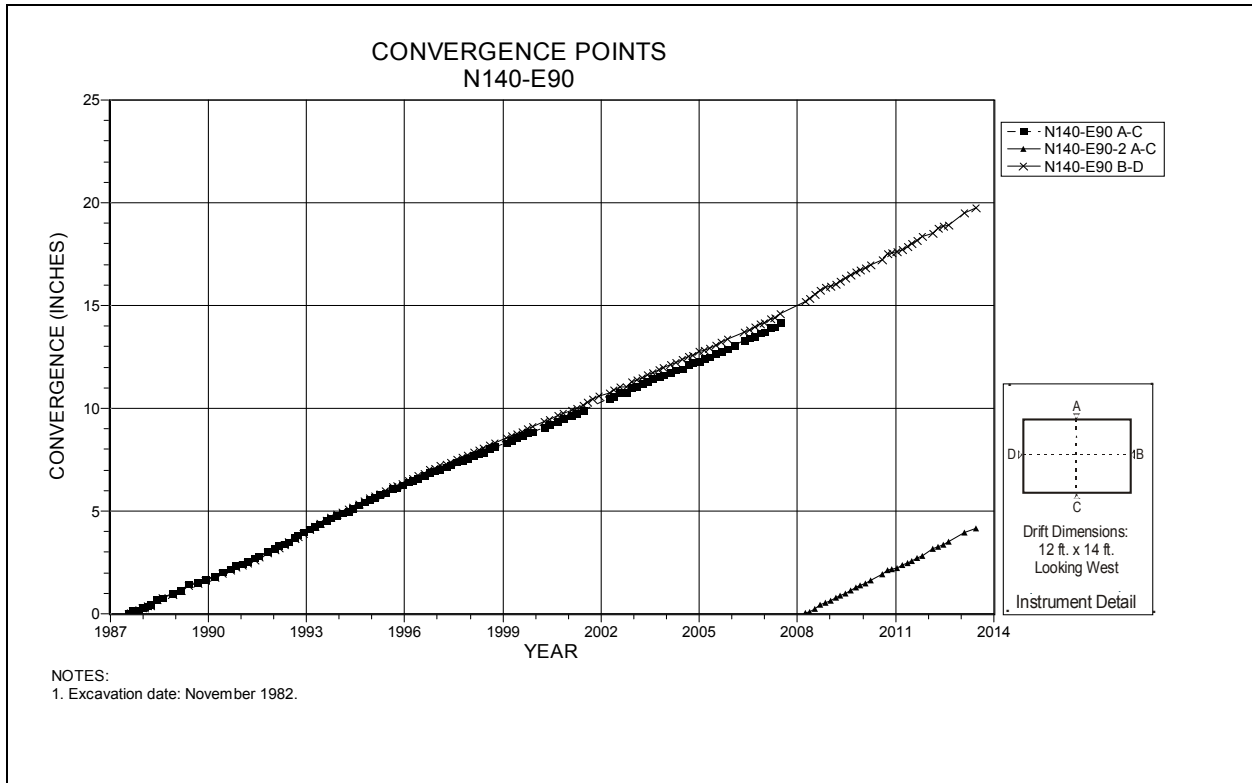
Figure 4-151 Convergence Point Array N140 E90 – All Chords
