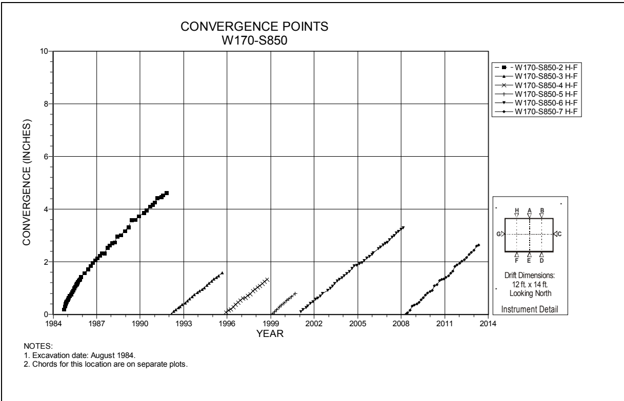
Figure 4-239 Convergence Point Array W170 S850 – Roof to Floor – West Quarter Point
