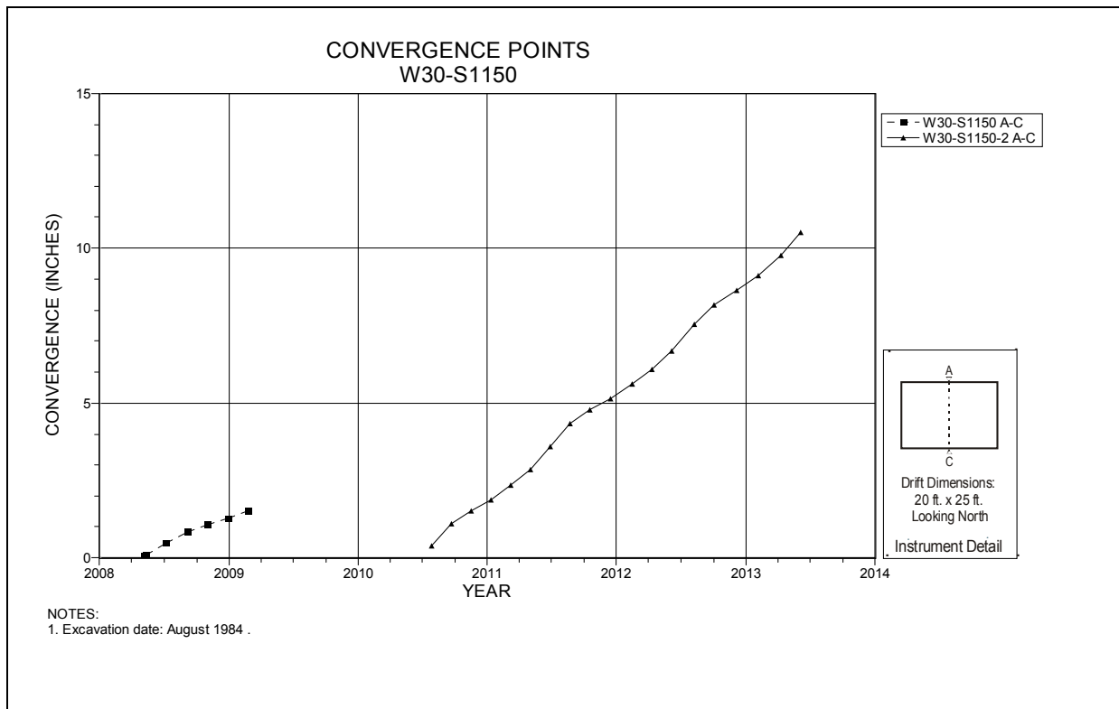
Figure 4-208 Convergence Point Array W30 S1150 – Roof to Floor
