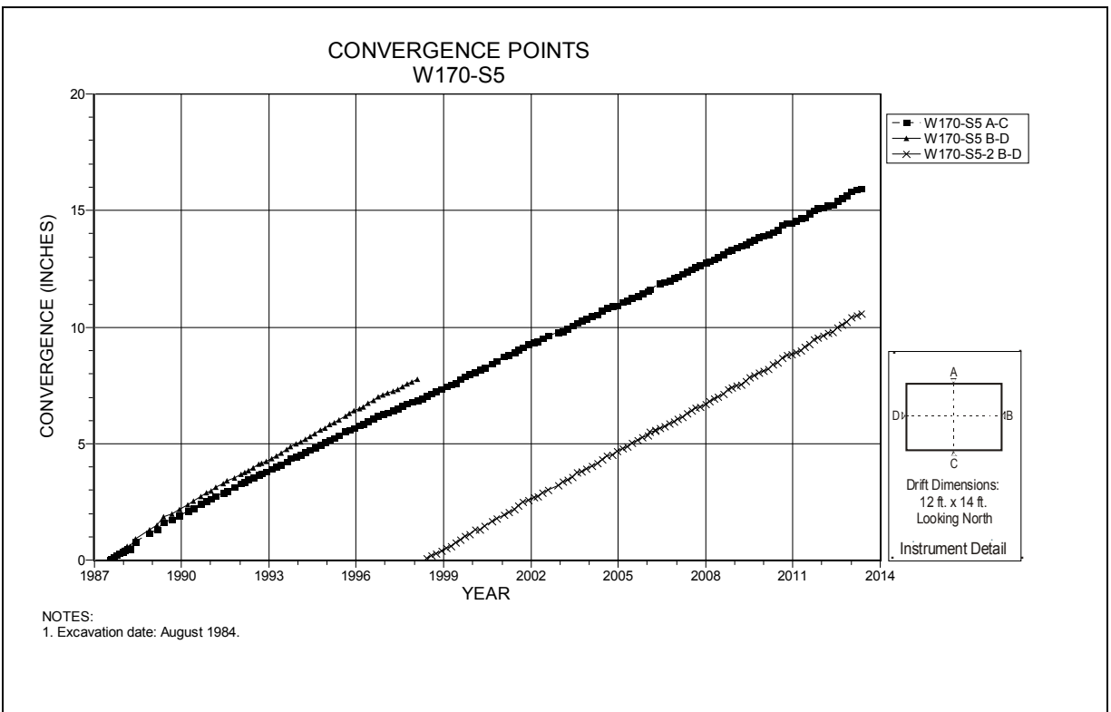
Figure 4-230 Convergence Point Array W170 S5 – All Chords
