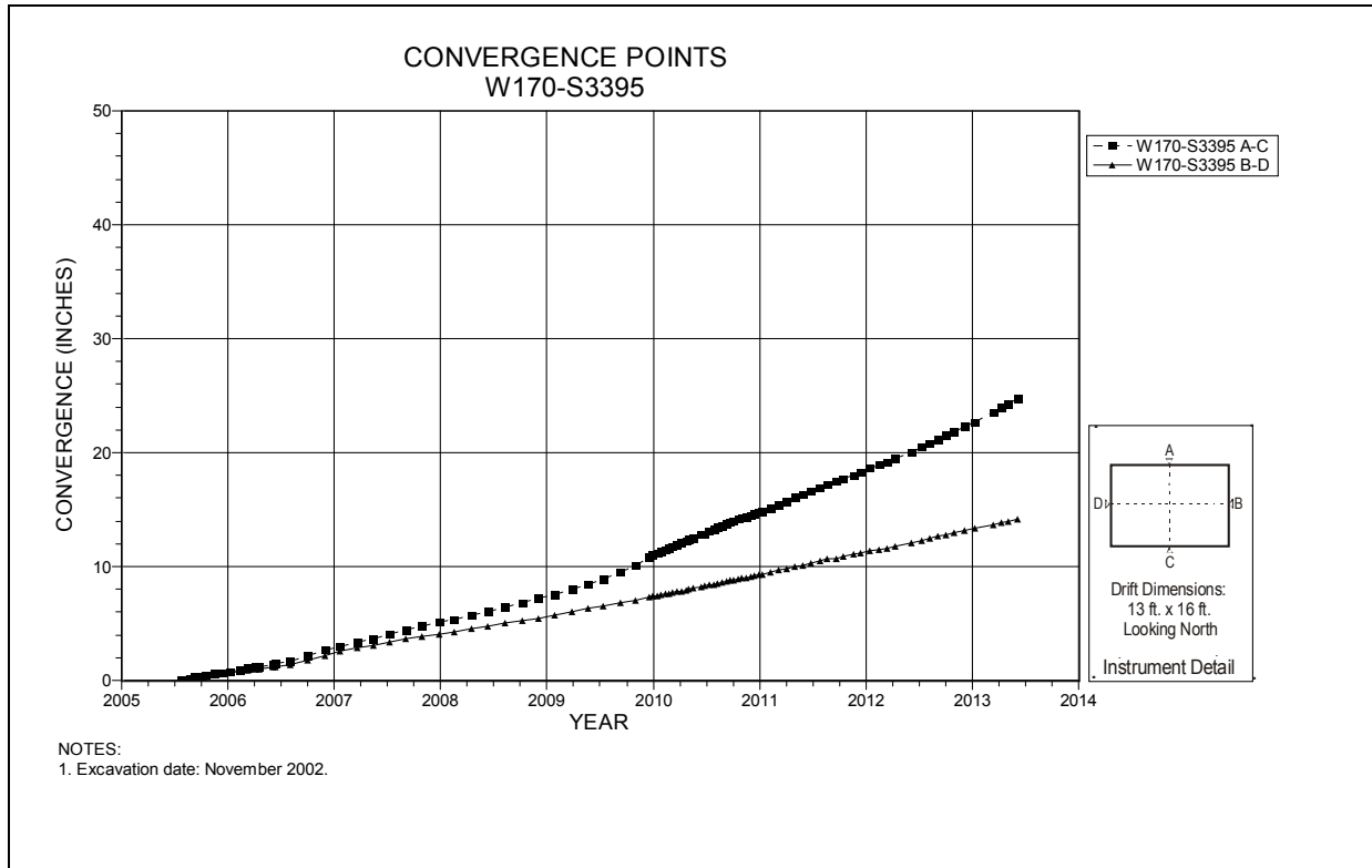
Figure 4-261 Convergence Point Array W170 S3395 – All Chords
