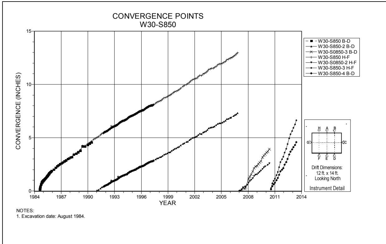
Figure 4-205 Convergence Point Array W30 S850 – Roof to Floor – Quarter Points
