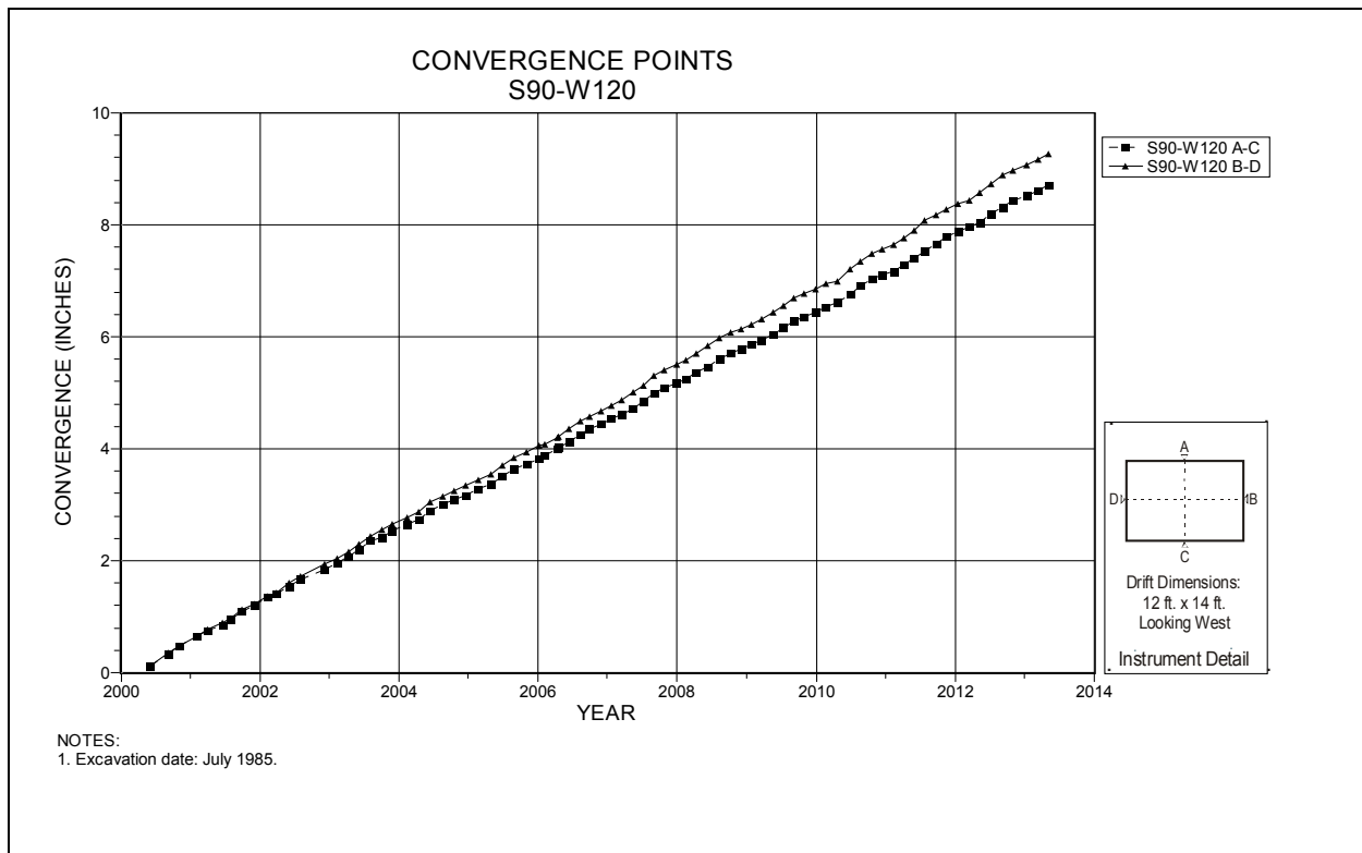
Figure 4-158 Convergence Point Array S90 W120 – All Chords
