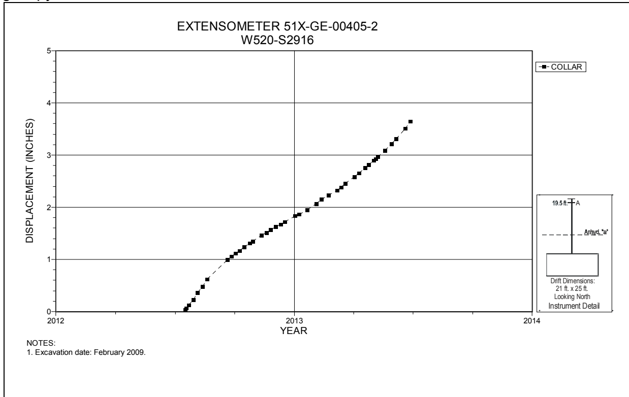
Figure 5-26 Extensometer 51X-GE-00405-2 Room 2, Panel 6 at W520 S2916 – Room Center – Roof
