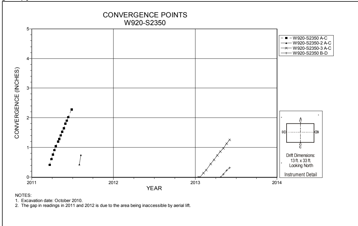
Figure 5-101 Convergence Point Array Room 5, Panel 7 at W920 S2350 – Room Center – All Chords
