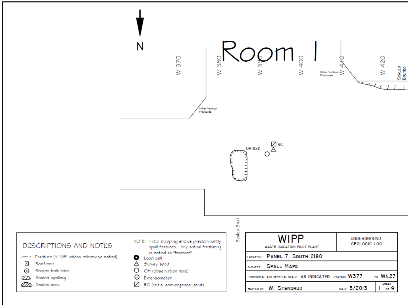
Figure 7-29 Panel 7 South 2180, W377-W427 Roof Fractures
