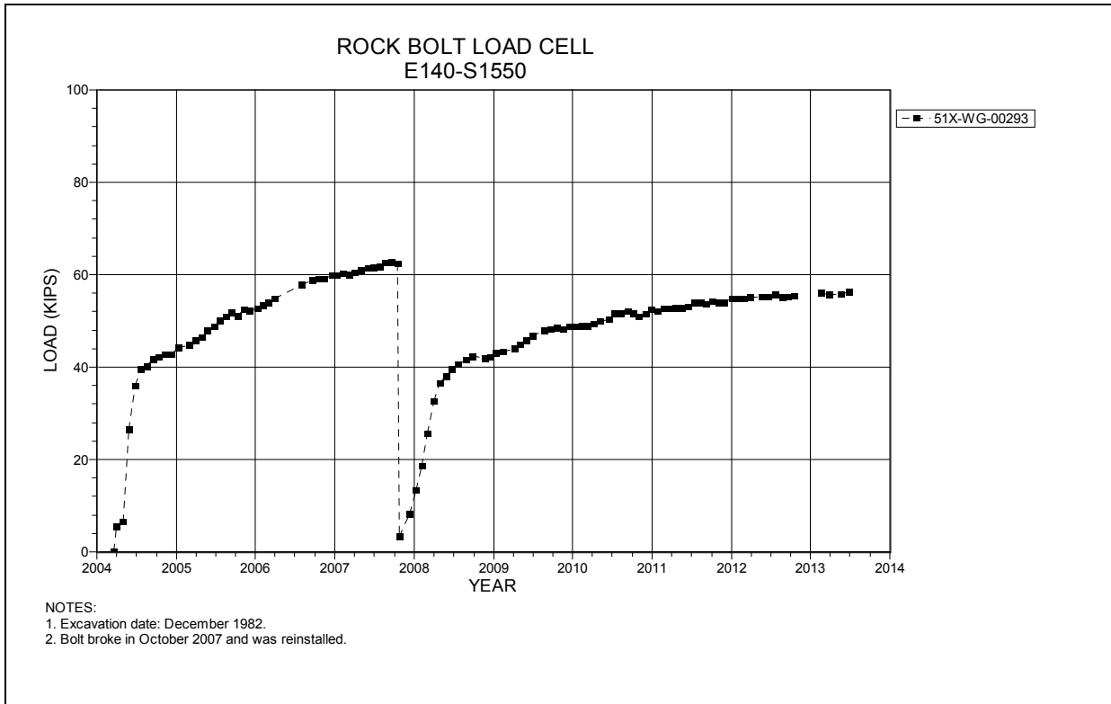
Figure 4-275 Rock Bolt Load Cell E140 S1550
