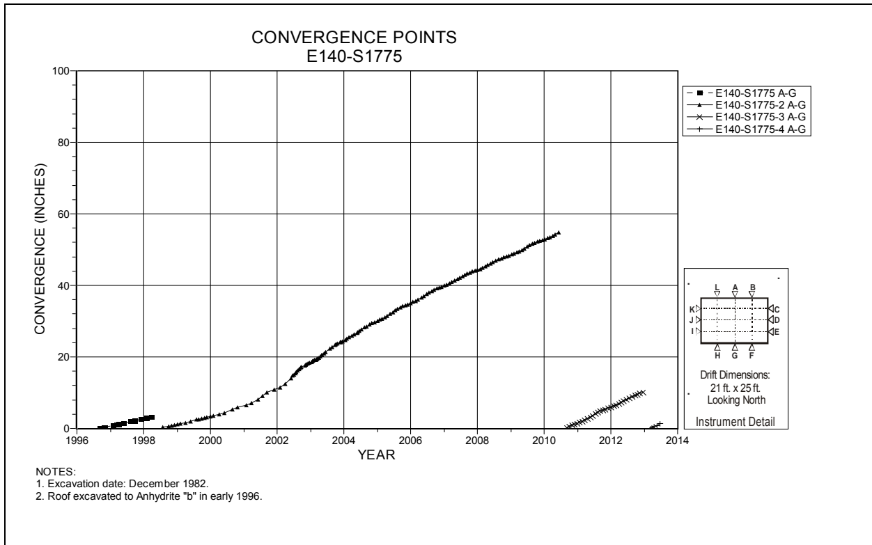
Figure 4-96 Convergence Point Array E140 S1775 – Roof to Floor – Centerline
