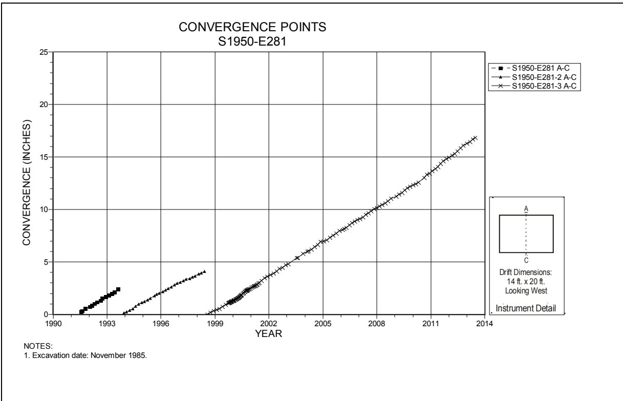
Figure 4-180 Convergence Point Array S1950 E281 – Roof to Floor
