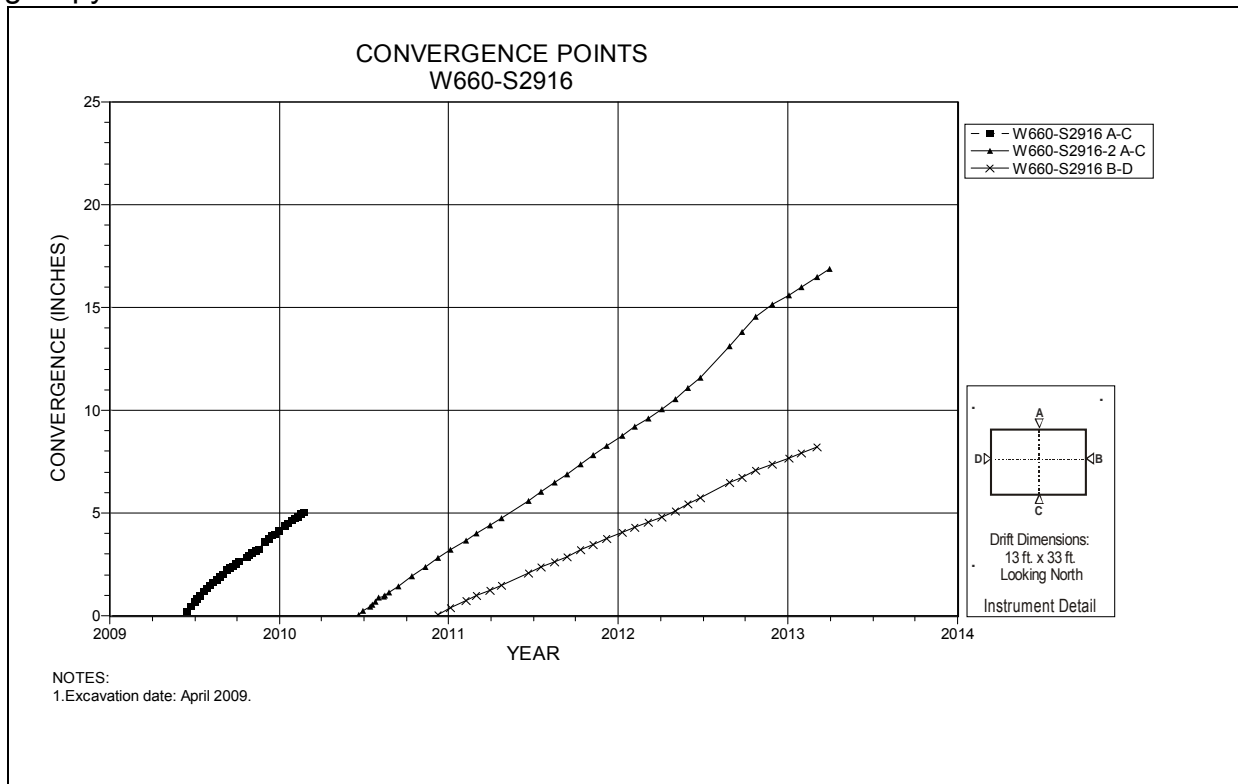
Figure 5-50 Convergence Point Array Room 3, Panel 6 at W660 S2916 – Room Center – All Chords
