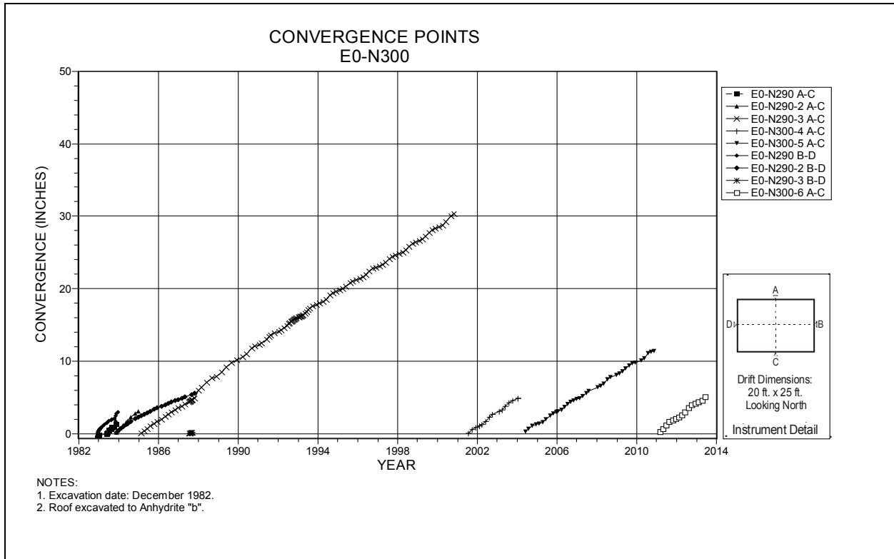
Figure 4-39 Convergence Point Array E0 N300 – All Chords
