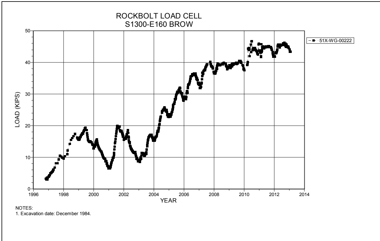
Figure 4-279 Rock Bolt Load Cell S1300 E160
