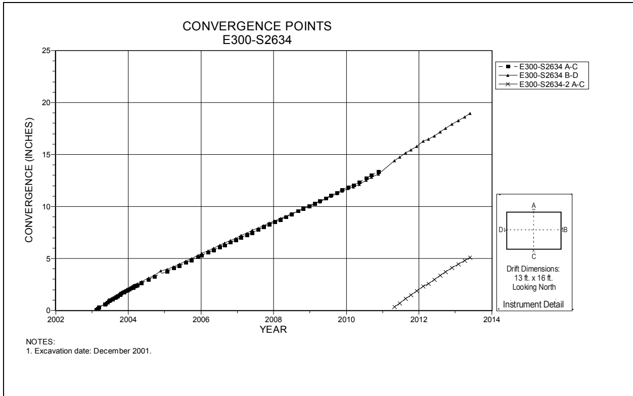
Figure 4-145 Convergence Point Array E300 S2634 – All Chords
