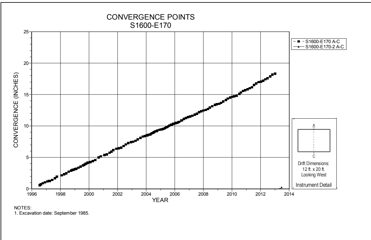
Figure 4-178 Convergence Point Array S1600 E170 – Roof to Floor
