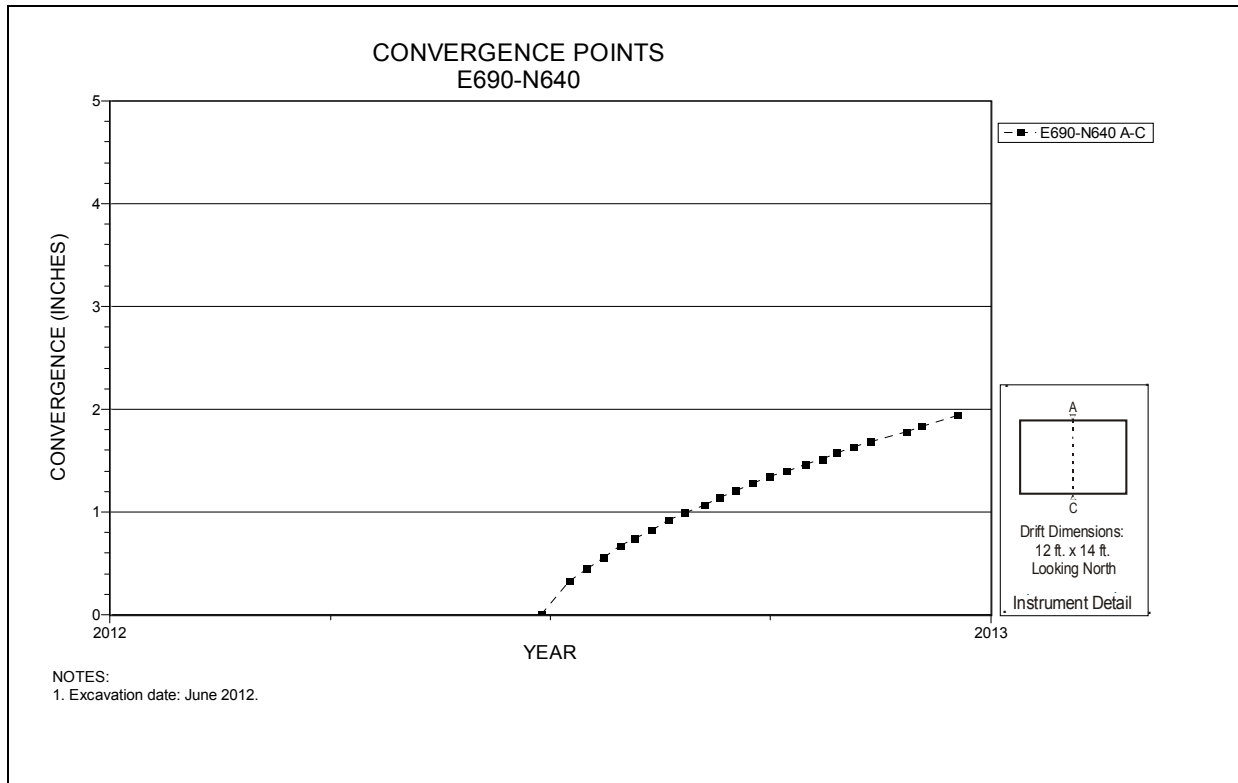
Figure 6-23 Convergence Point Array E690 N640 – Roof to Floor
