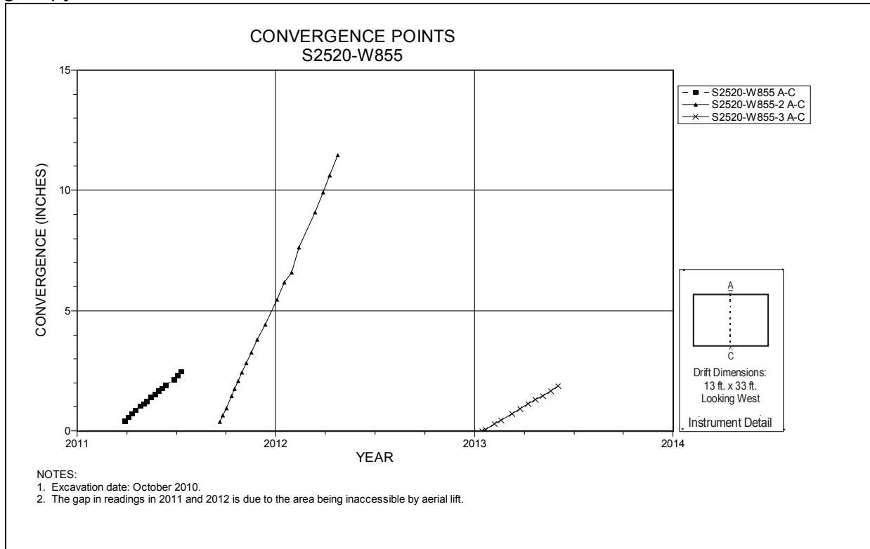
Figure 5-117 Convergence Point Array S2520 W855 – Roof to Floor
