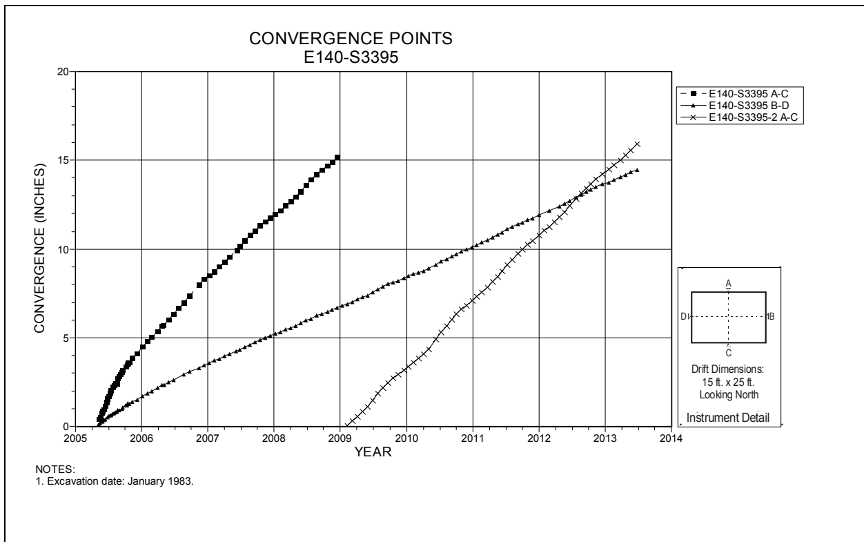
Figure 4-118 Convergence Point Array E140 S3395 – All Chords
