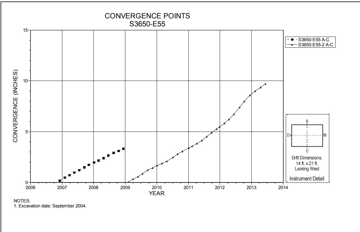
Figure 4-196 Convergence Point Array S3650 E55 – Roof to Floor
