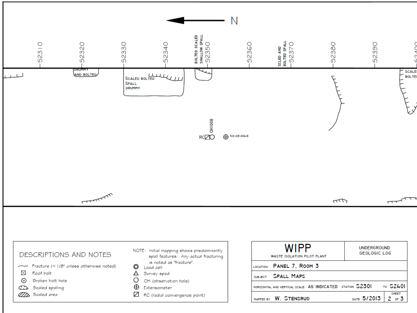
Figure 7-15 Panel 7 Room 3, S2301-S2401 Roof Fractures
