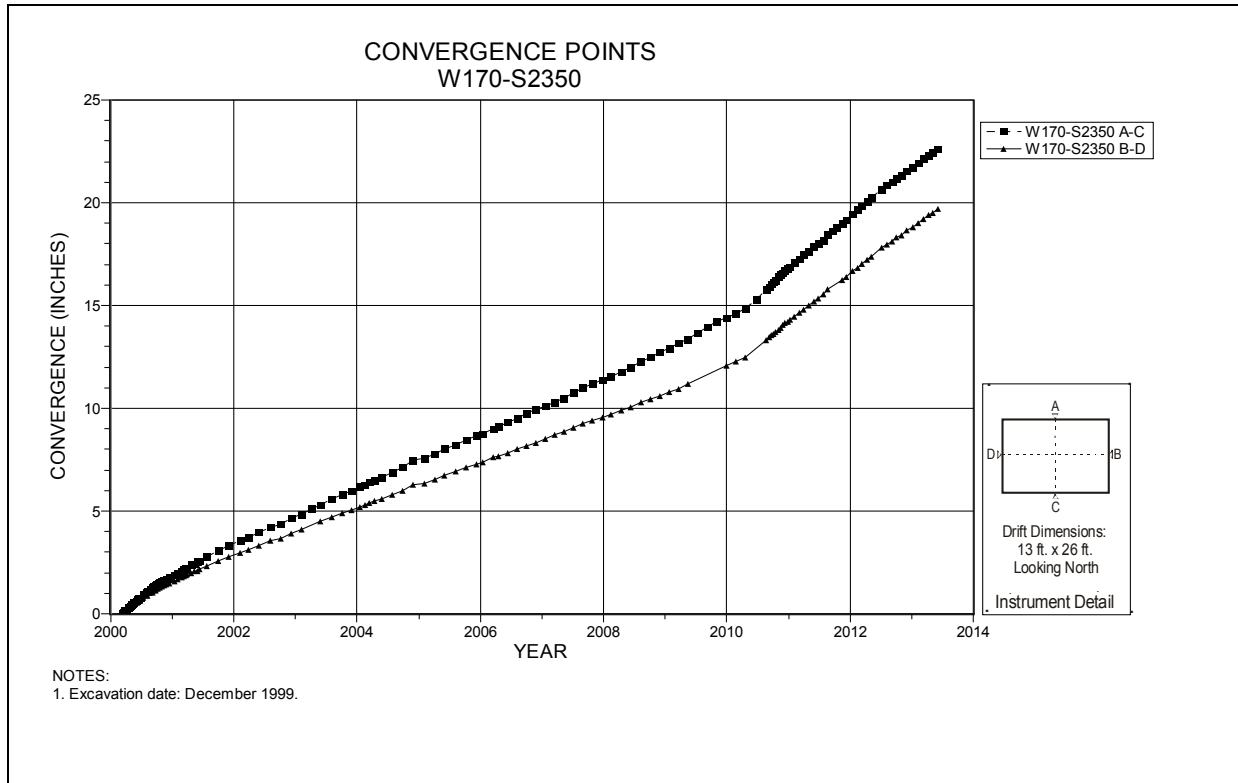
Figure 4-251 Convergence Point Array W170 S2350 – All Chords
