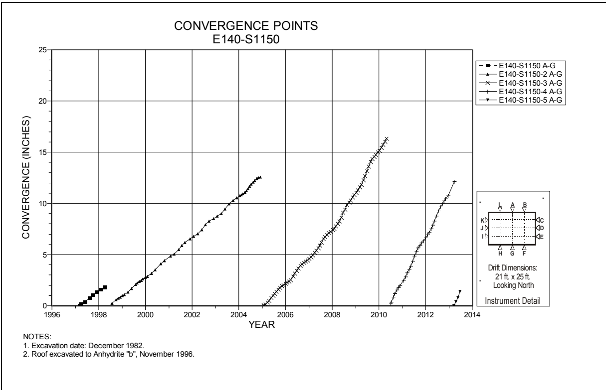
Figure 4-75 Convergence Point Array E140 S1150 – Roof to Floor – Centerline
