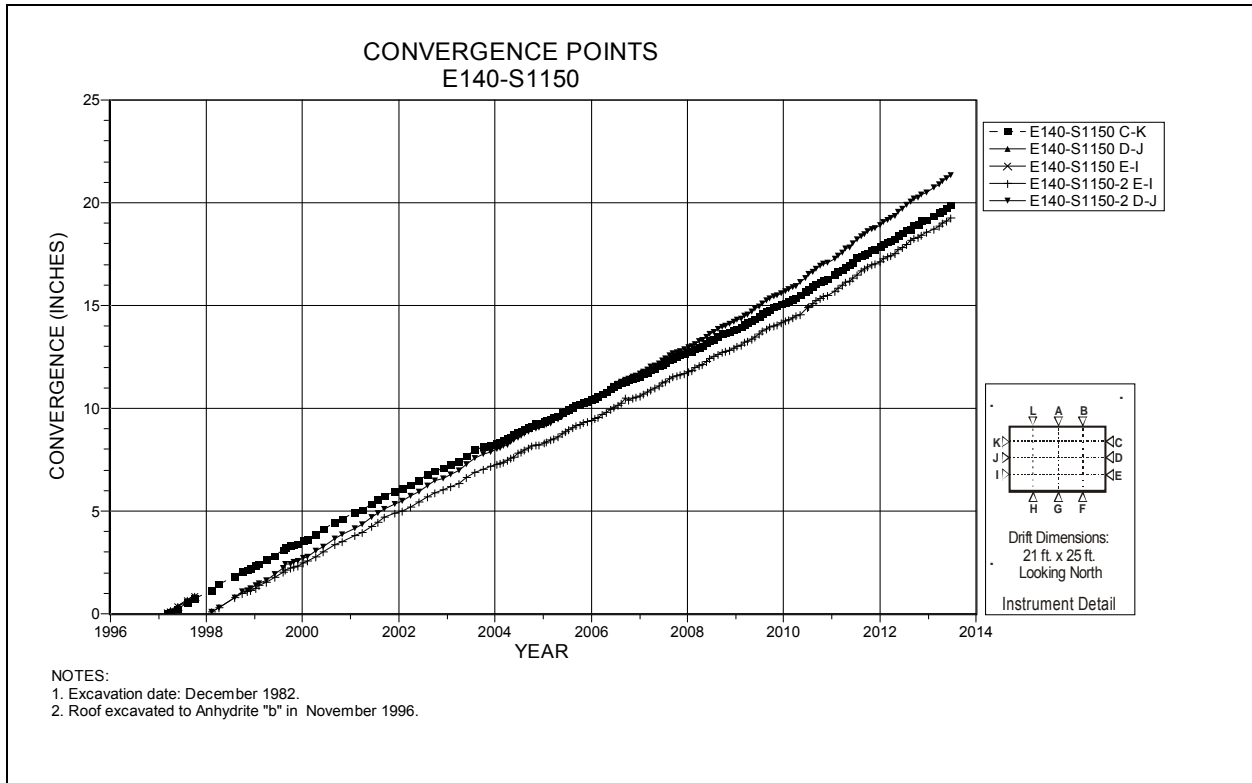
Figure 4-77 Convergence Point Array E140 S1150 – Rib to Rib
