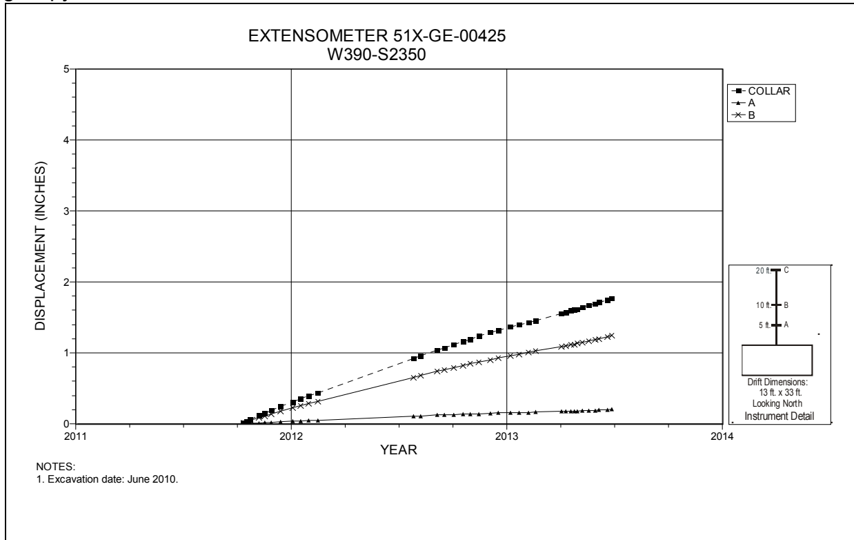
Figure 5-65 Extensometer 51X-GE-00425 Room 1, Panel 7 at W390 S2350 – Room Center – Roof
