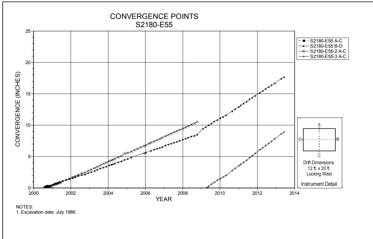
Figure 4-182 Convergence Point Array S2180 E55 – All Chords
