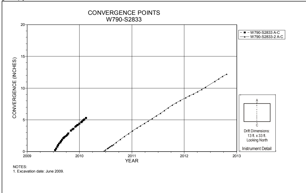
Figure 5-52 Convergence Point Array Room 4, Panel 6 at W790 S2833 – Roof to Floor
