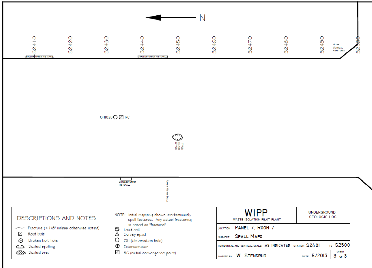
Figure 7-28 Panel 7 Room 7, S2401-S2500 Roof Fractures
