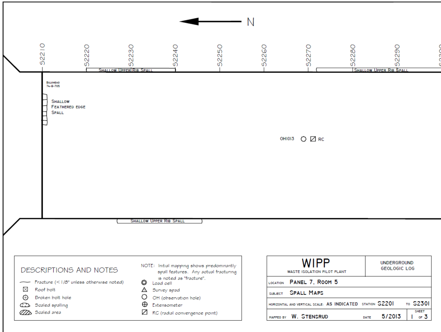
Figure 7-20 Panel 7 Room 5, S2201-S2301 Roof Fractures
