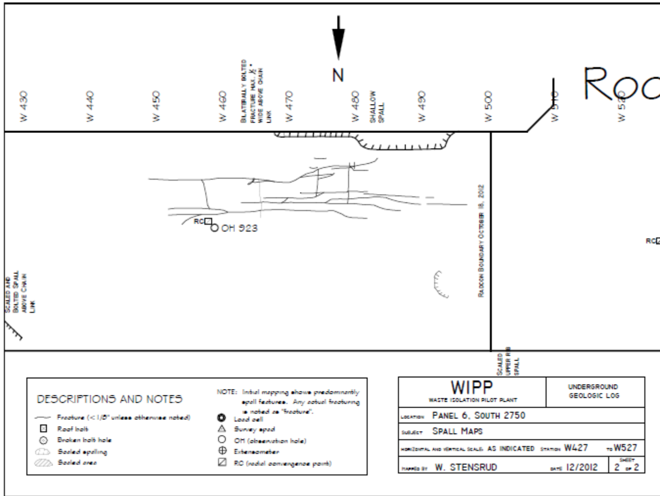
Figure 7-5 Panel 6 South 2750, W427-W527 Roof Fractures
