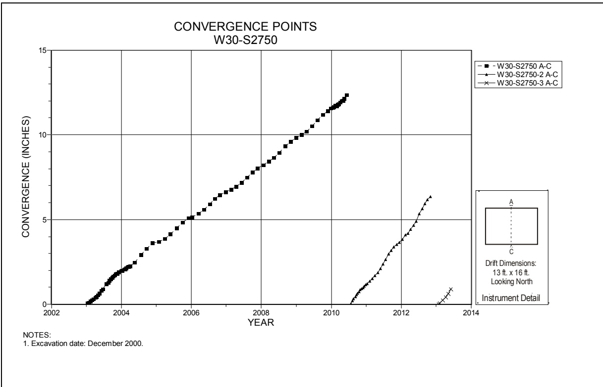
Figure 4-220 Convergence Point Array W30 S2750 – Roof to Floor
