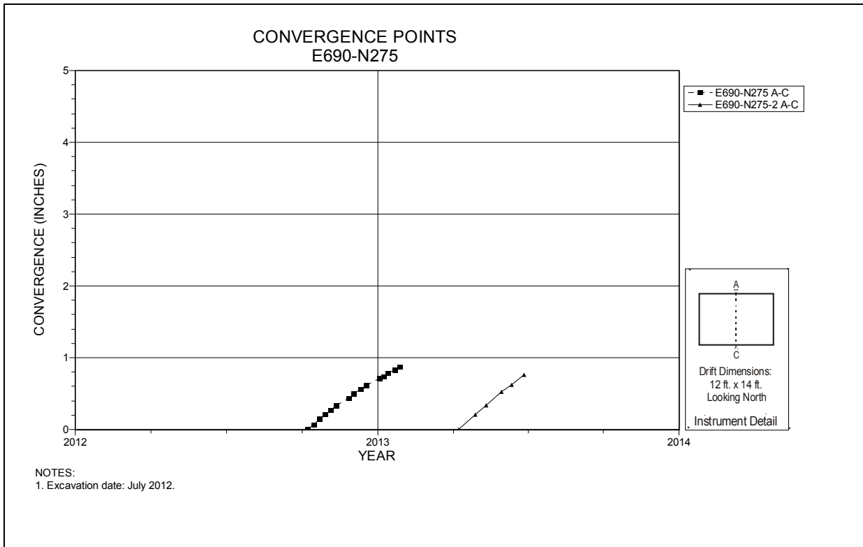
Figure 6-19 Convergence Point Array E690 N275 – Roof to Floor
