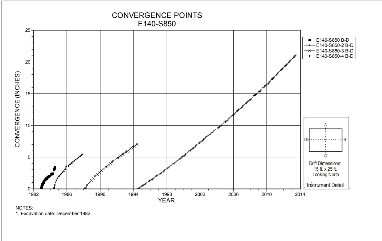
Figure 4-69 Convergence Point Array E140 S850 – Rib to Rib
