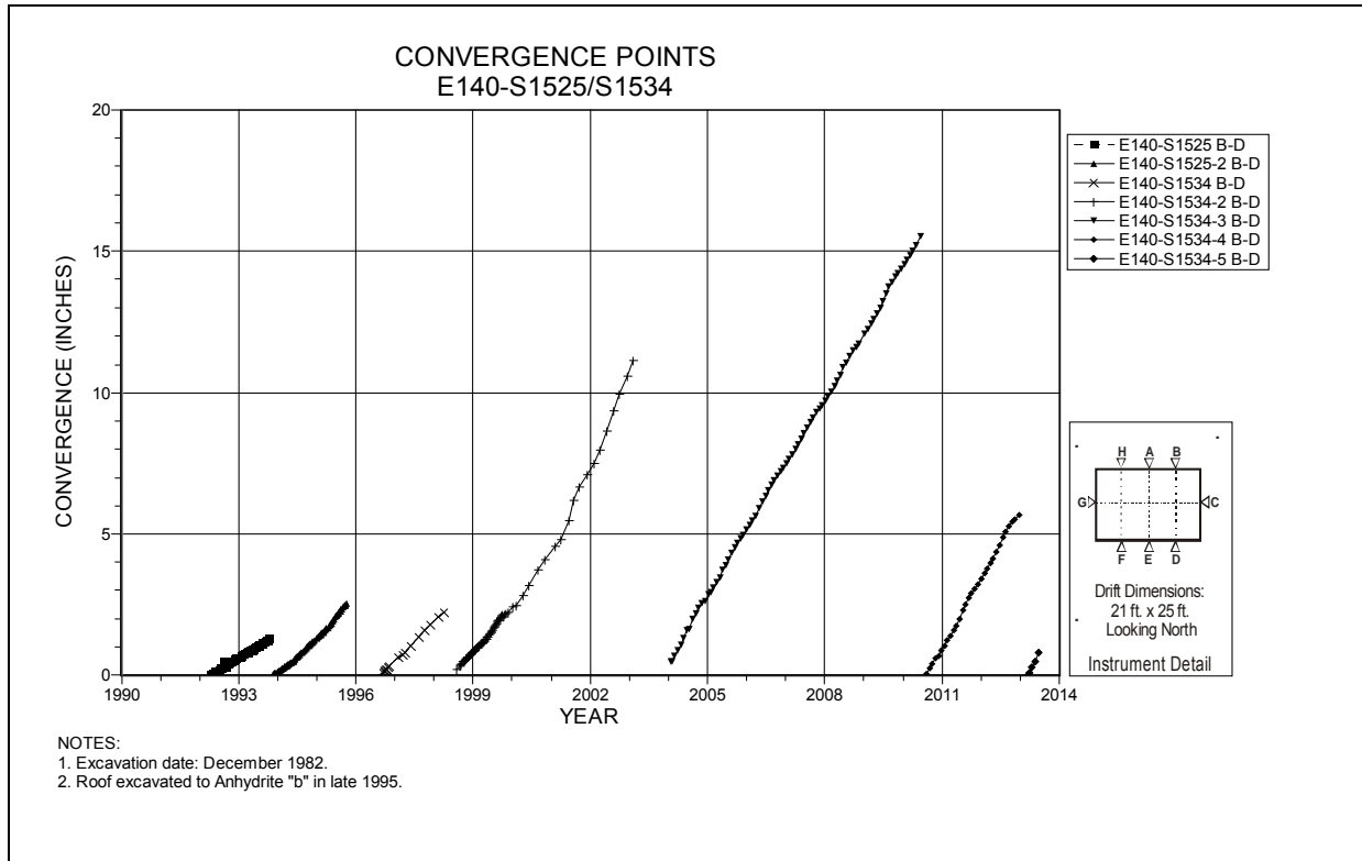
Figure 4-91 Convergence Point Array E140 S1525/S1534 – Roof to Floor – East Quarter Point
