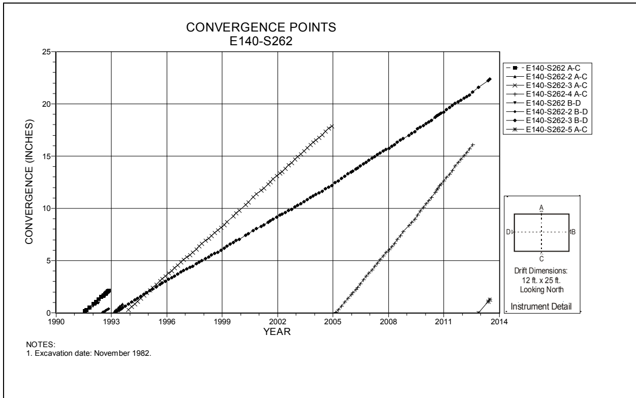
Figure 4-62 Convergence Point Array E140 S262 – All Chords
