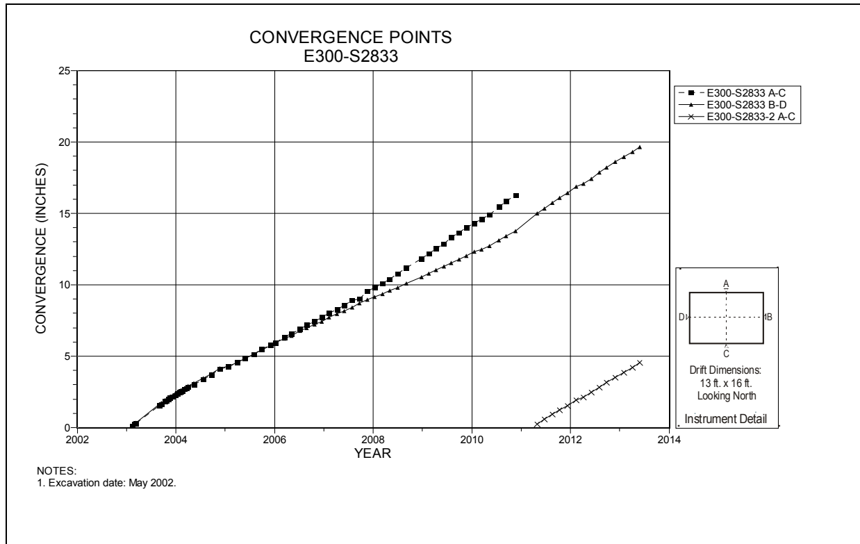
Figure 4-146 Convergence Point Array E300 S2833 – All Chords
