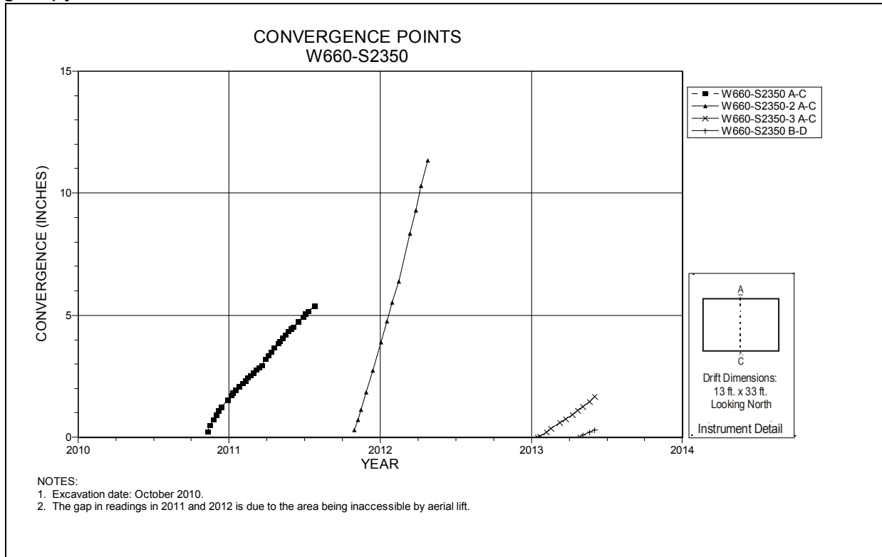
Figure 5-95 Convergence Point Array Room 3, Panel 7 at W660 S2350 – Room Center – All Chords
