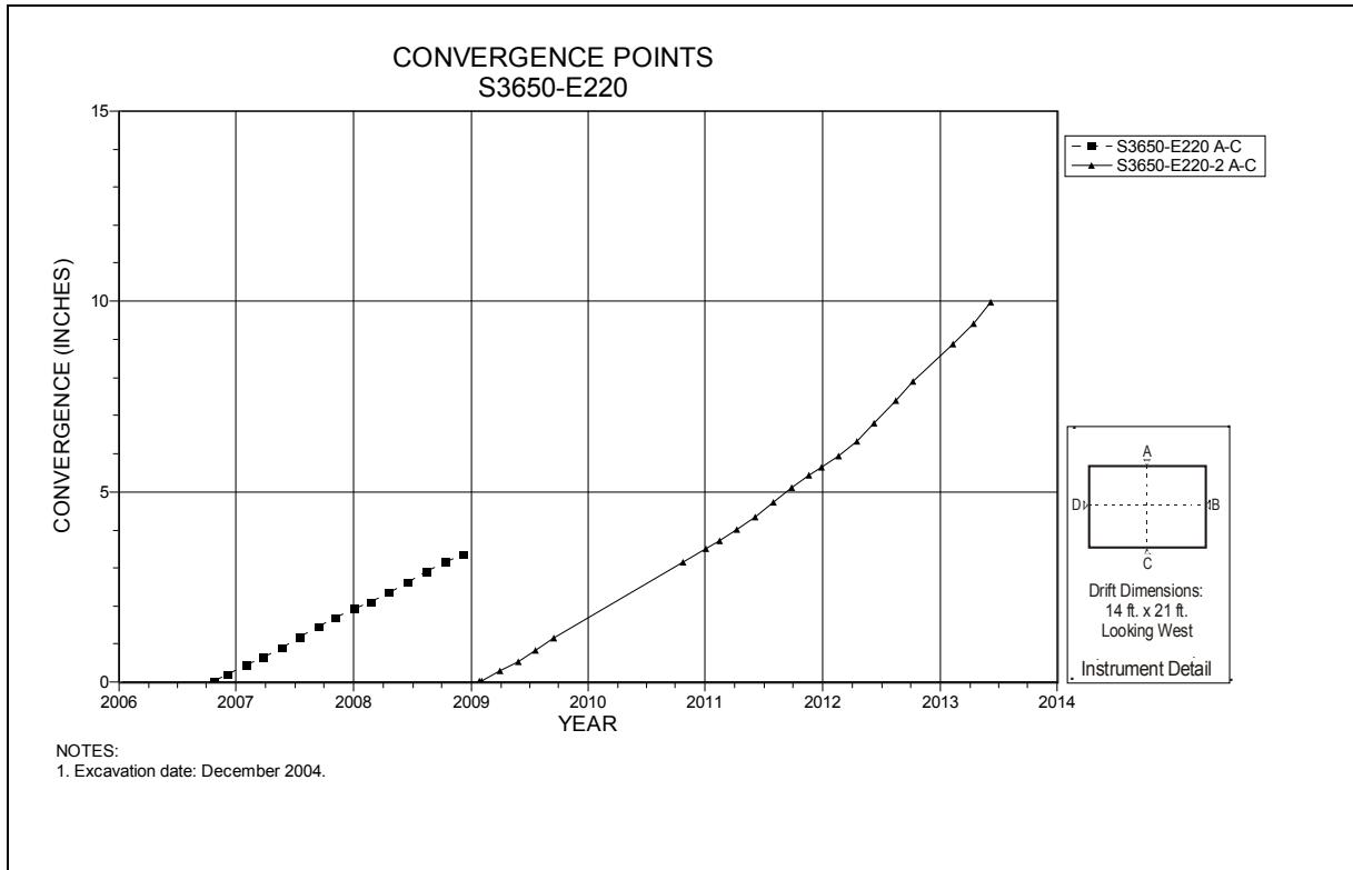
Figure 4-197 Convergence Point Array S3650 E220 – Roof to Floor
