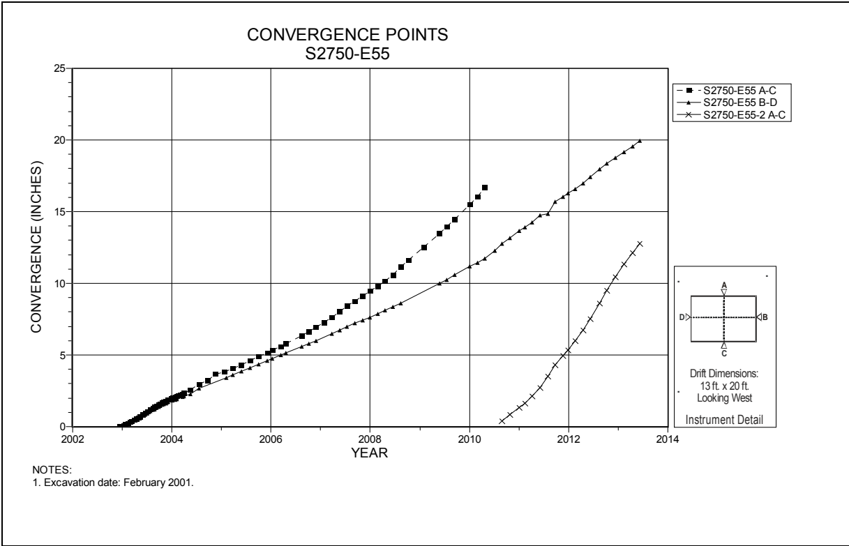
Figure 4-187 Convergence Point Array S2750 E55 – All Chords
