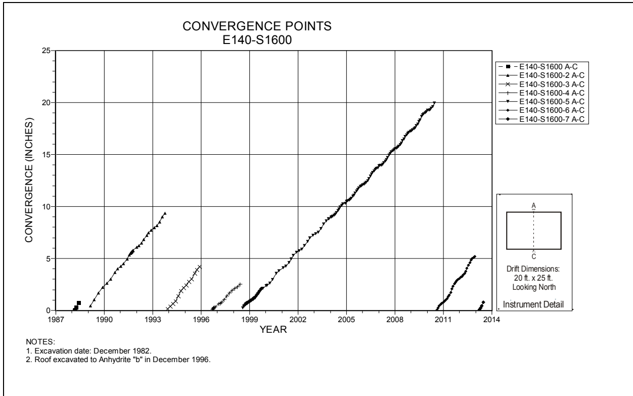
Figure 4-93 Convergence Point Array E140 S1600 – Roof to Floor
