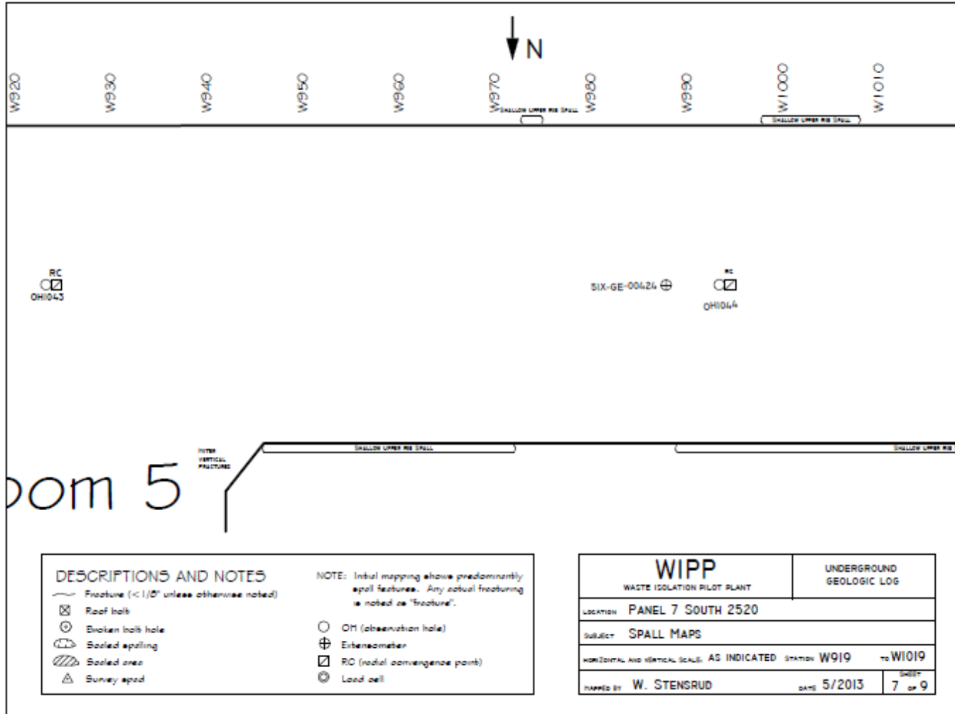
Figure 7-44 Panel 7 South 2520, W919-W1019 Roof Fractures
