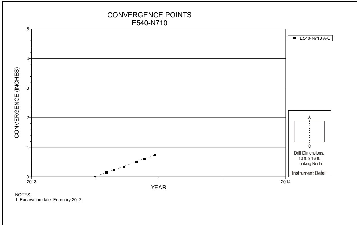
Figure 6-12 Convergence Point Array E540 N710 – Roof to Floor
