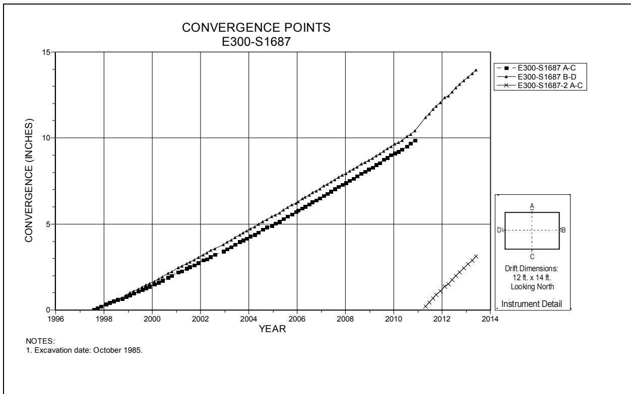
Figure 4-138 Convergence Point Array E300 S1687 – All Chords
