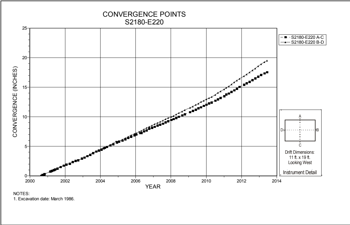
Figure 4-183 Convergence Point Array S2180 E220 – All Chords
