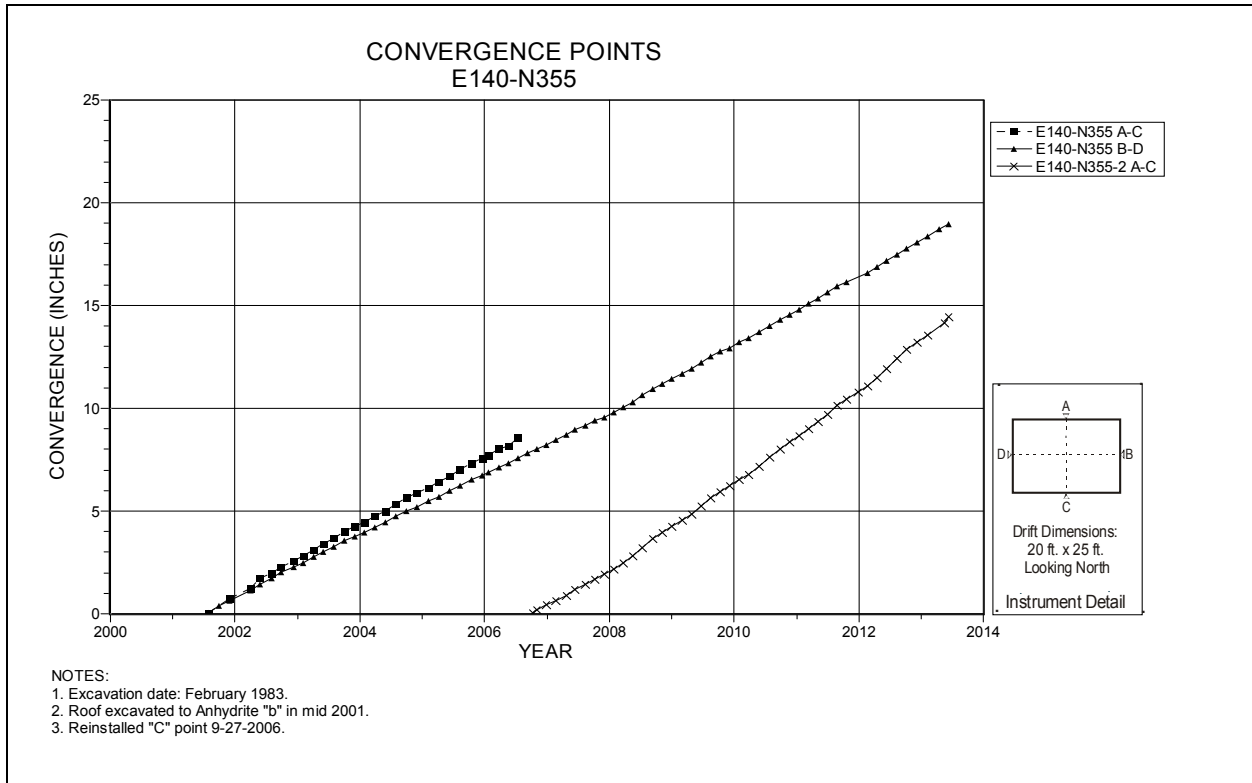
Figure 4-51 Convergence Point Array E140 N355 – All Chords
