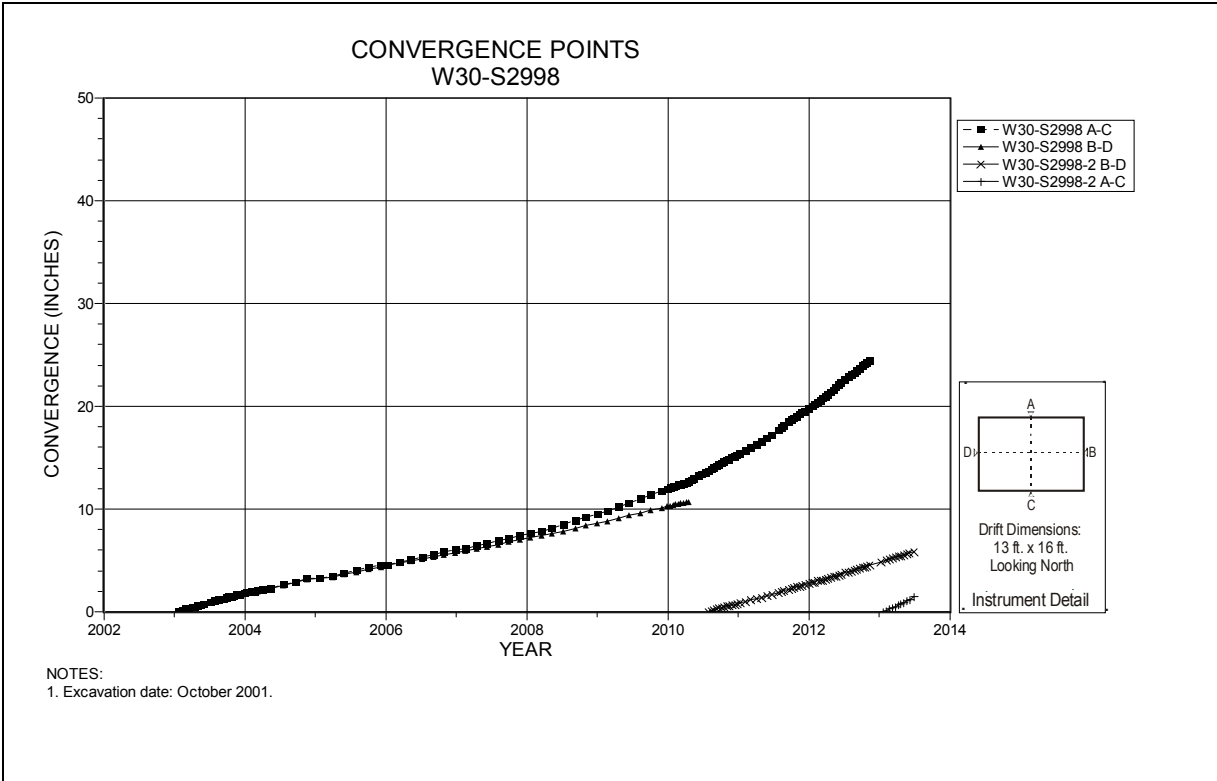
Figure 4-223 Convergence Point Array W30 S2998 – All Chords
