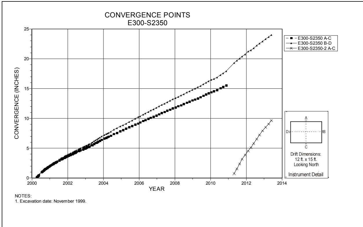
Figure 4-143 Convergence Point Array E300 S2350 – All Chords
