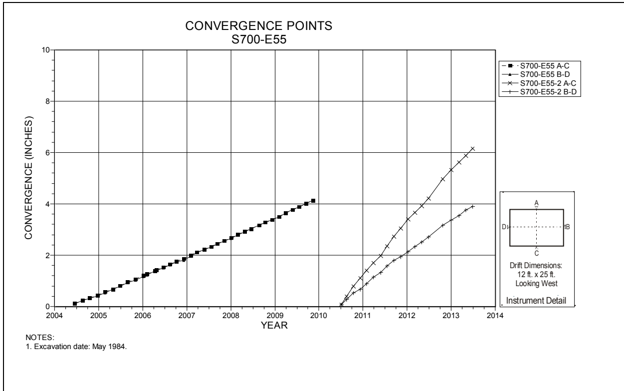
Figure 4-165 Convergence Point Array S700 E55 – All Chords
