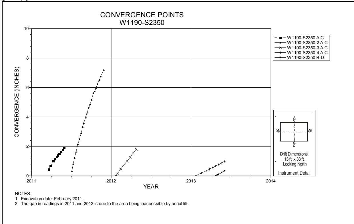
Figure 5-107 Convergence Point Array Room 7, Panel 7 at W1190 S2350 – Room Center – All Chords
