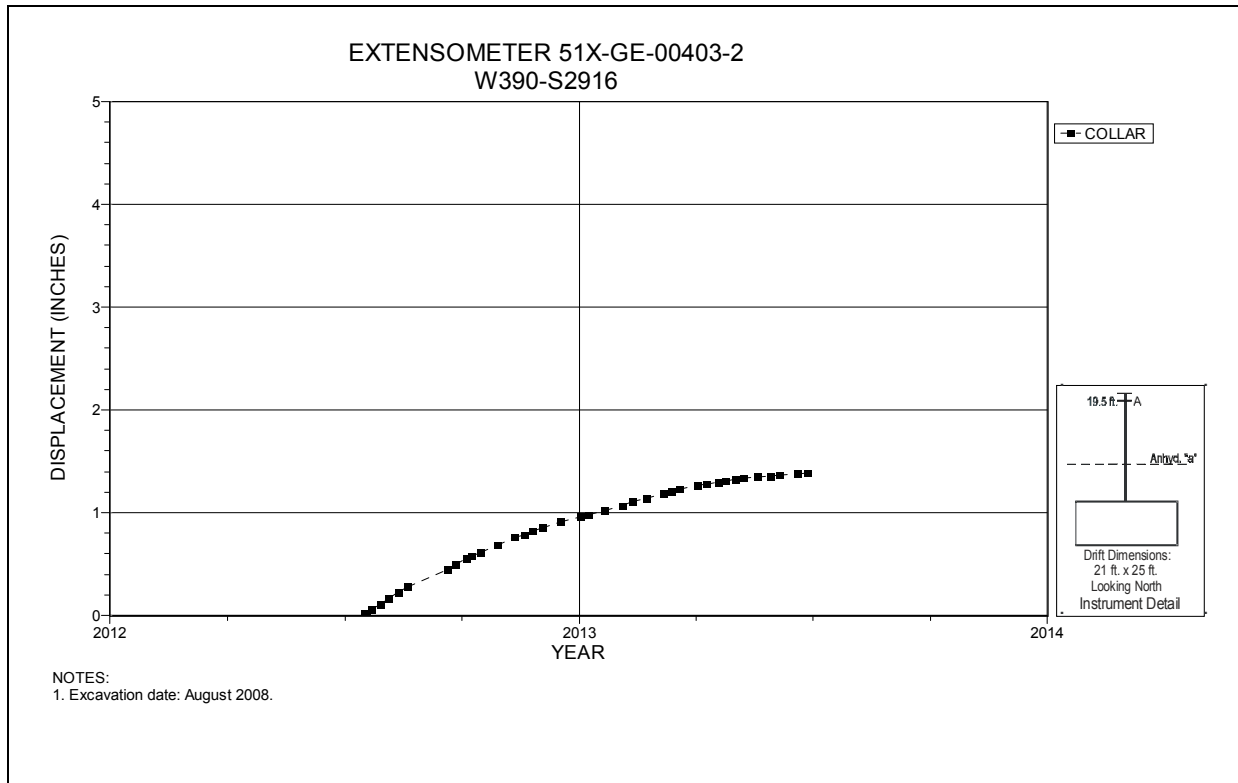
Figure 5-25 Extensometer 51X-GE-00403-2 Room 1, Panel 6 at W390 S2916 – Roof
