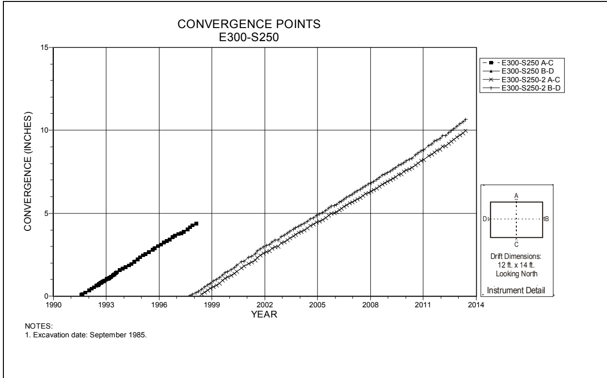
Figure 4-129 Convergence Point Array E300 S250 – All Chords
