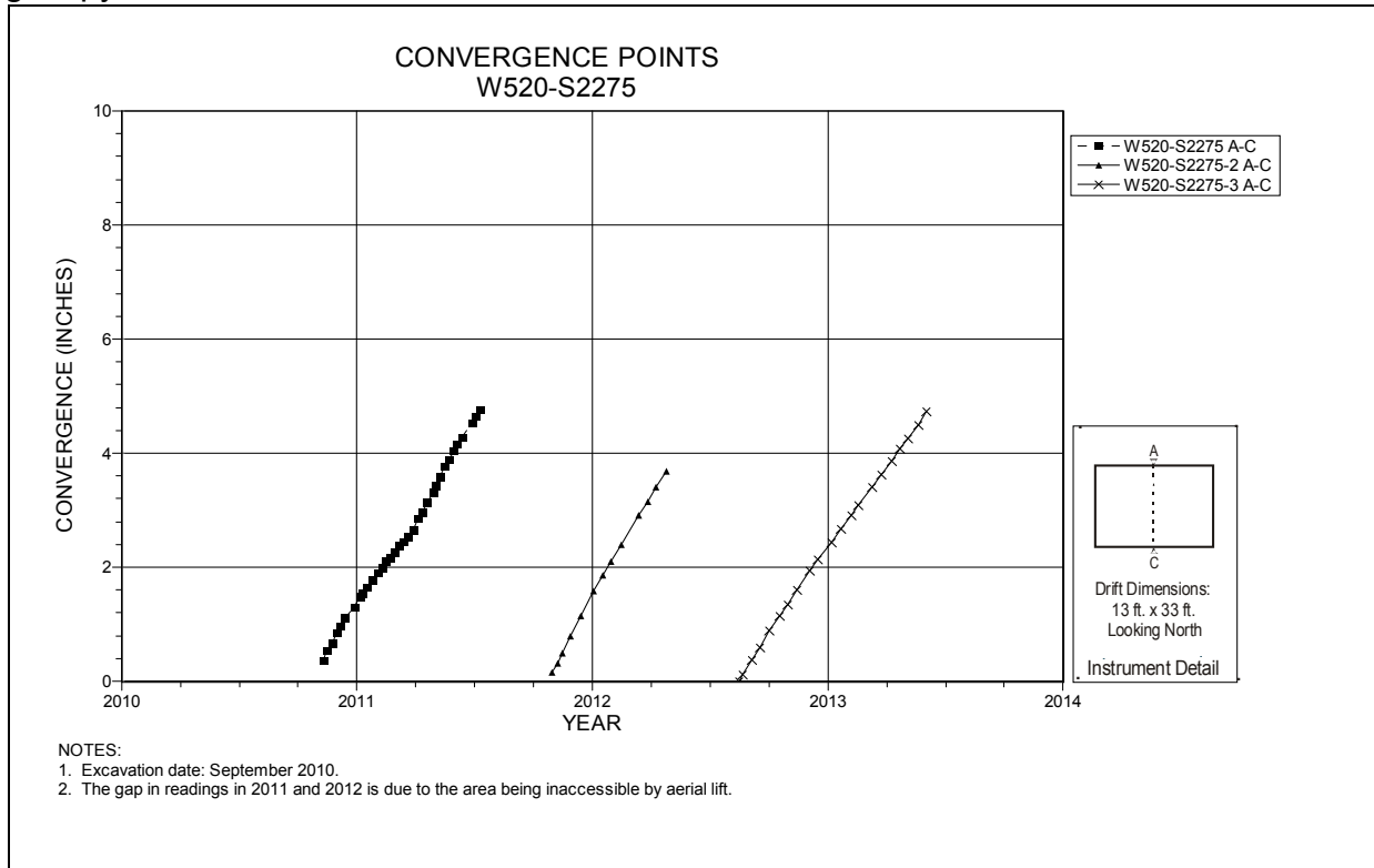
Figure 5-91 Convergence Point Array Room 2, Panel 7 at W520 S2275 – Roof to Floor
