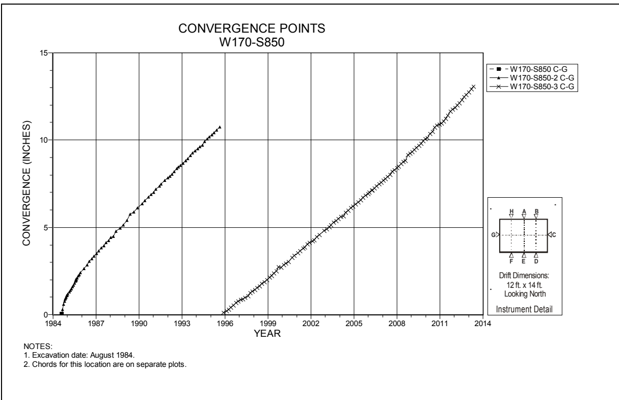
Figure 4-238 Convergence Point Array W170 S850 – Rib to Rib
