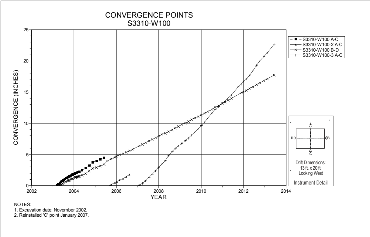
Figure 4-195 Convergence Point Array S3310 W100 – All Chords
