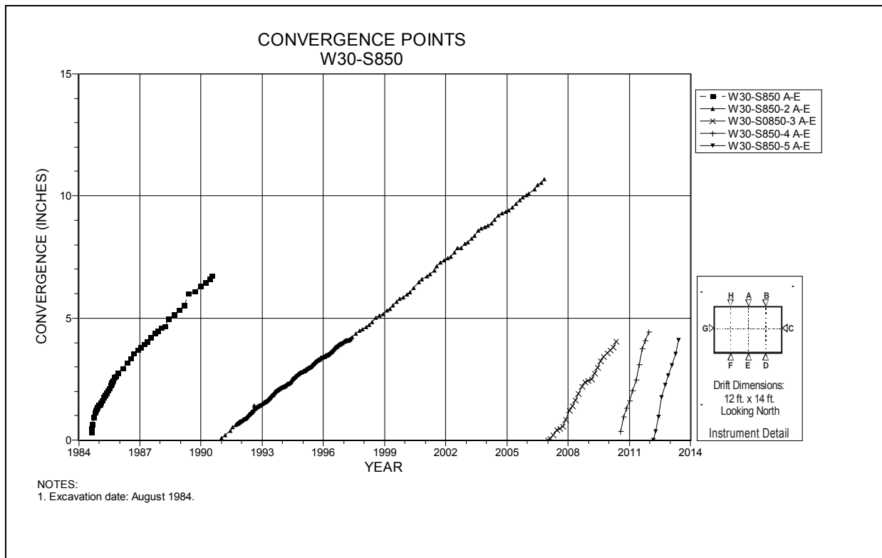
Figure 4-204 Convergence Point Array W30 S850 – Roof to Floor – Centerline
