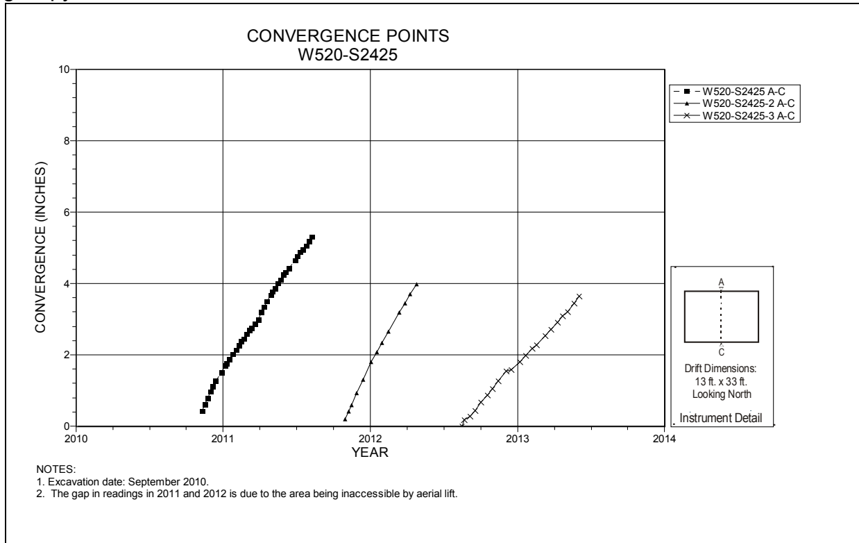
Figure 5-93 Convergence Point Array Room 2, Panel 7 at W520 S2425 – Roof to Floor
