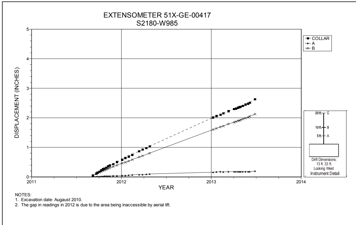
Figure 5-64 Extensometer 51X-GE-00417 S2180 W985 – Roof
