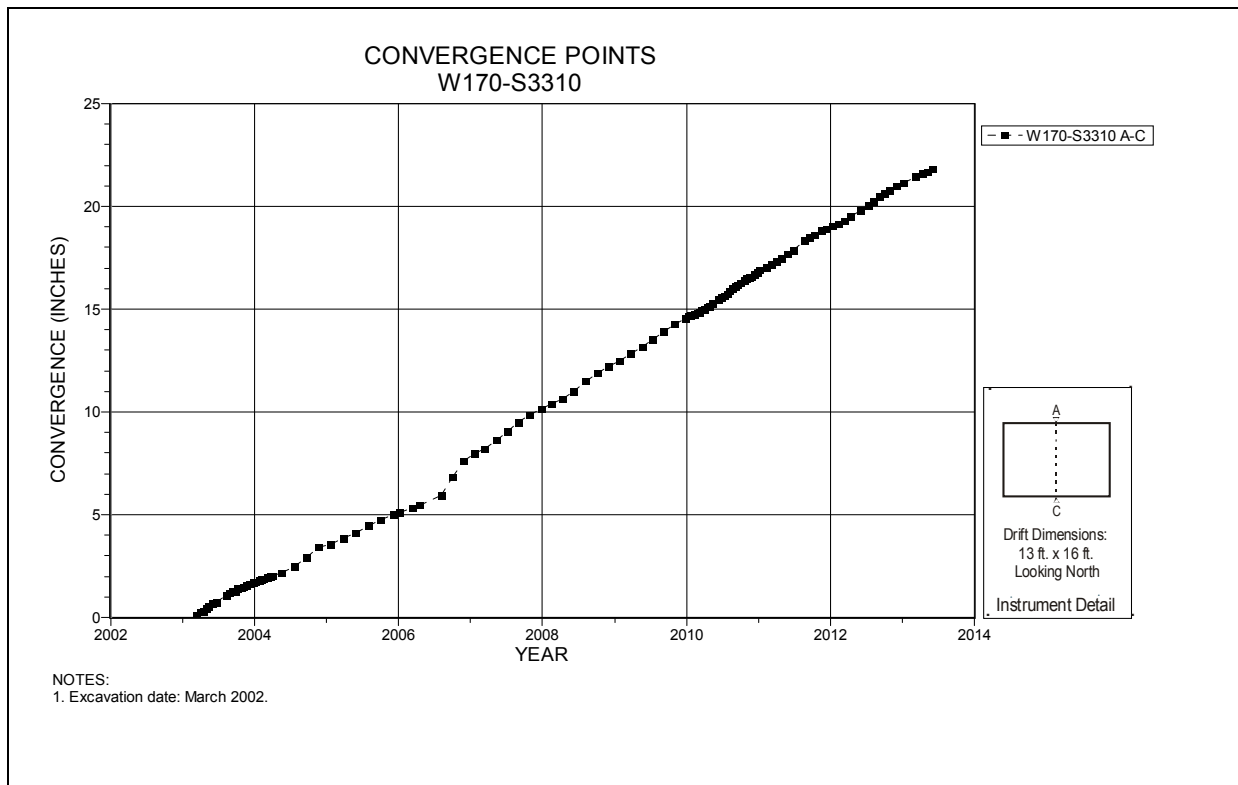
Figure 4-260 Convergence Point Array W170 S3310 – Roof to Floor
