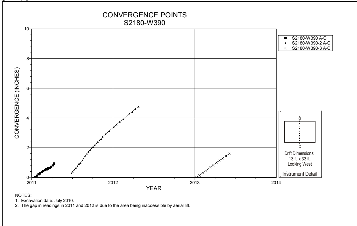
Figure 5-75 Convergence Point Array S2180 W390 Intersection (Room 1, Panel 7) – Roof to Floor
