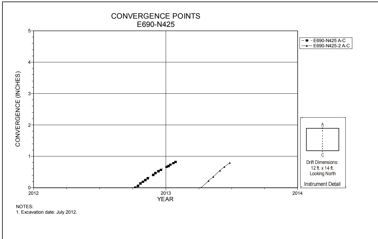
Figure 6-21 Convergence Point Array E690 N425 – Roof to Floor
