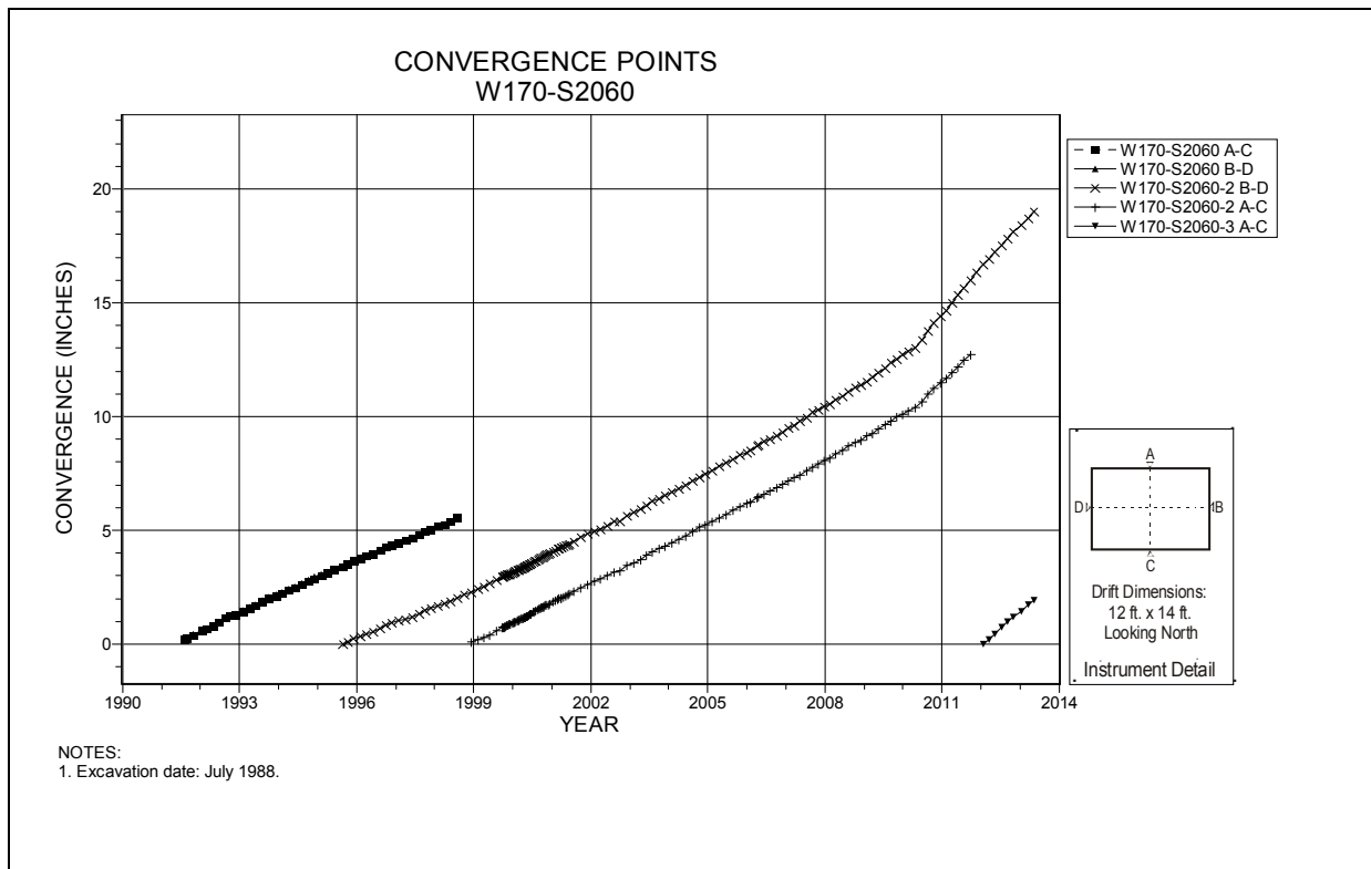
Figure 4-248 Convergence Point Array W170 S2060 – All Chords
