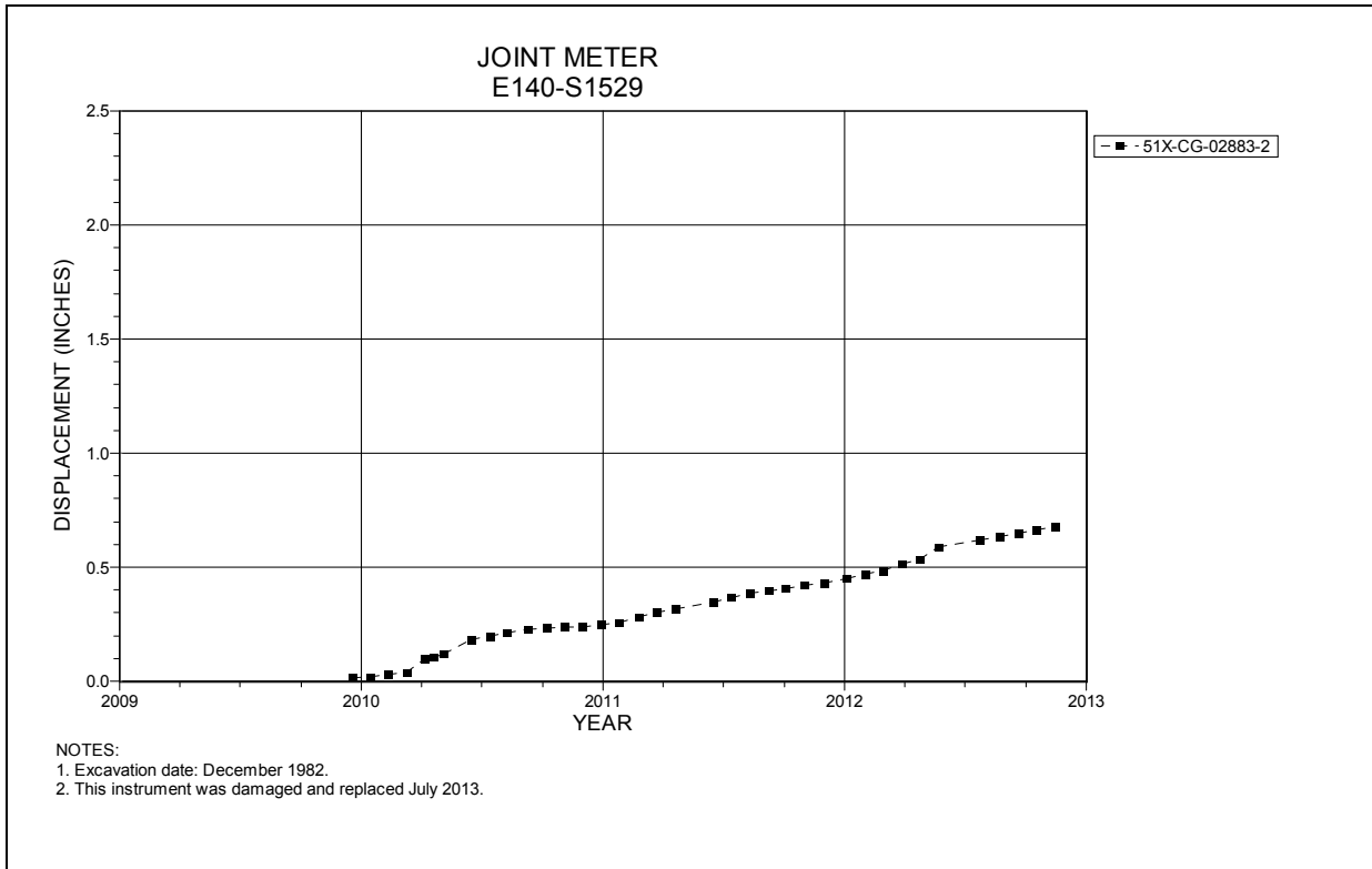
Figure 4-267 Joint Meter E140 S1529
