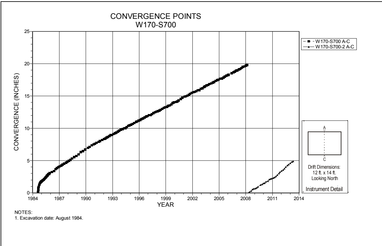
Figure 4-235 Convergence Point Array W170 S700 – Roof to Floor
