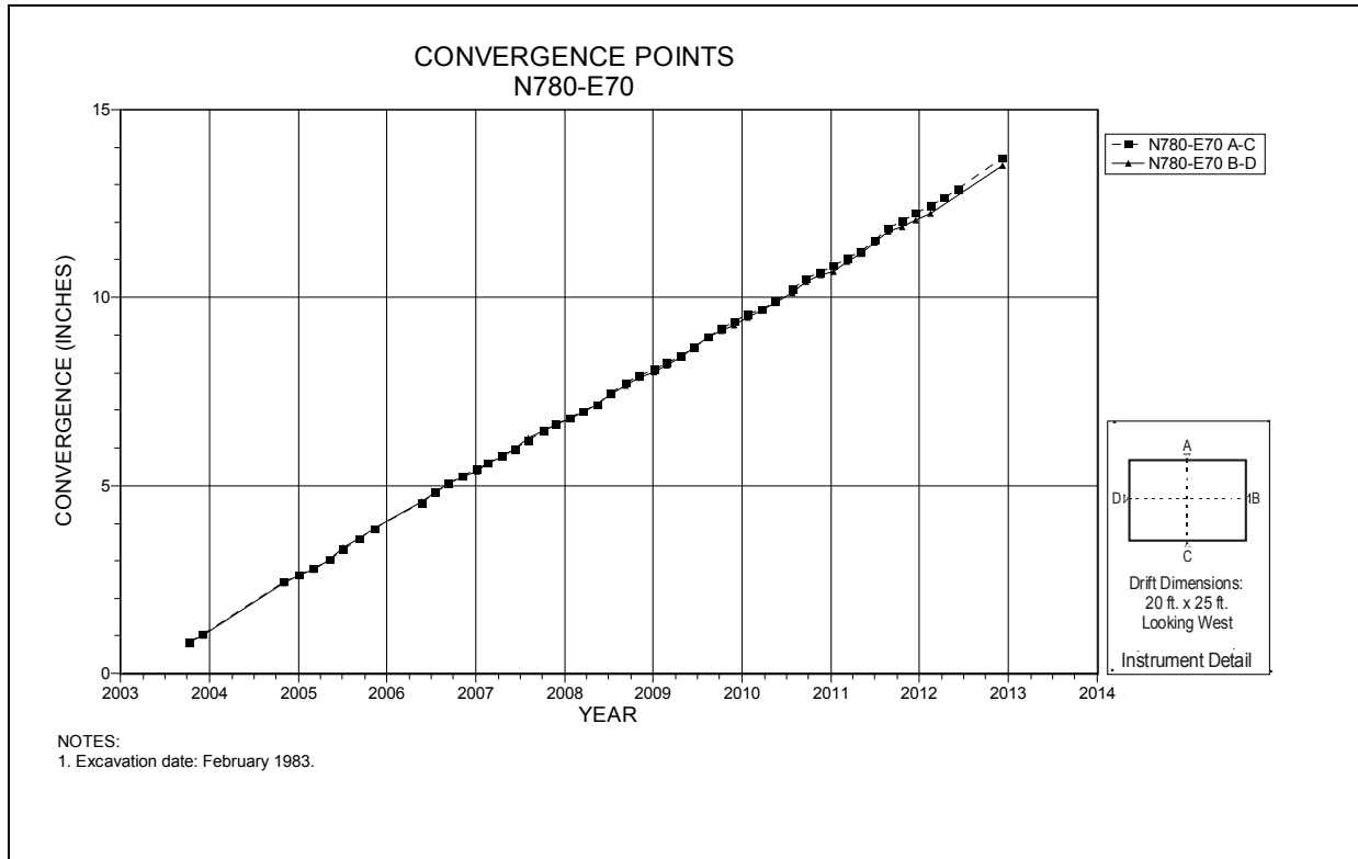
Figure 4-157 Convergence Point Array N780 E70 – All Chords
