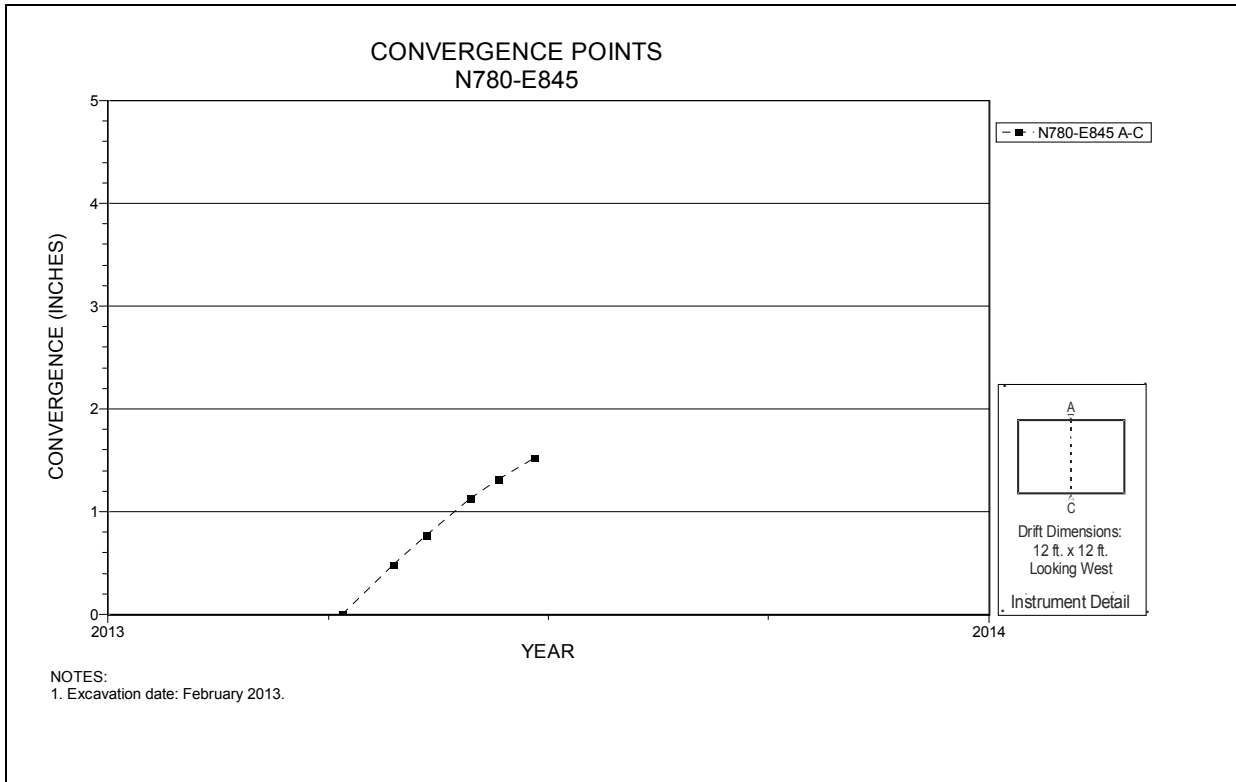
Figure 6-32 Convergence Point Array N780 E845 – Roof to Floor
