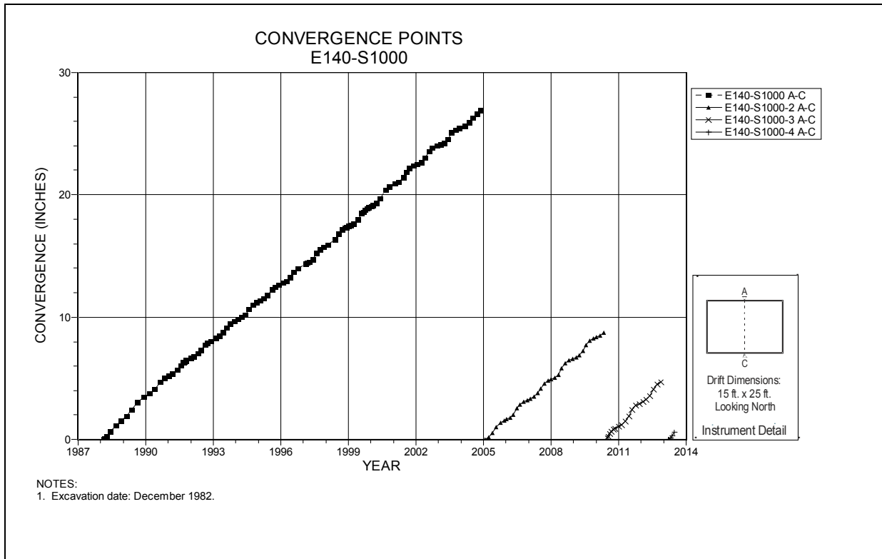
Figure 4-70 Convergence Point Array E140 S1000 – Roof to Floor
