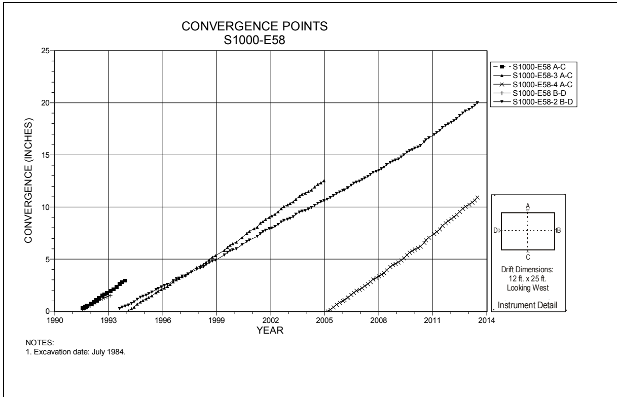
Figure 4-169 Convergence Point Array S1000 E58 – All Chords
