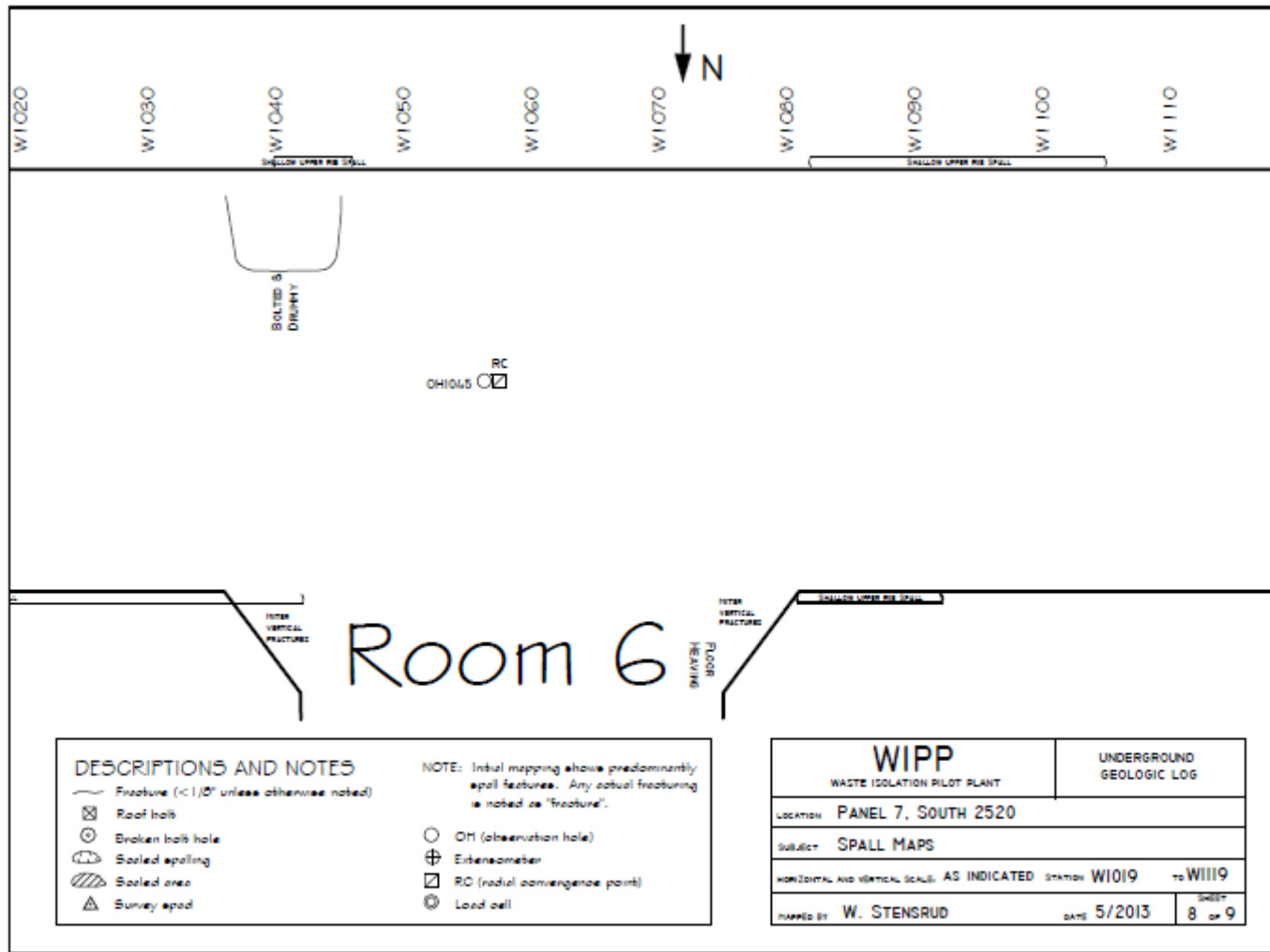
Figure 7-45 Panel 7 South 2520, W1019-W1119 Roof Fractures
