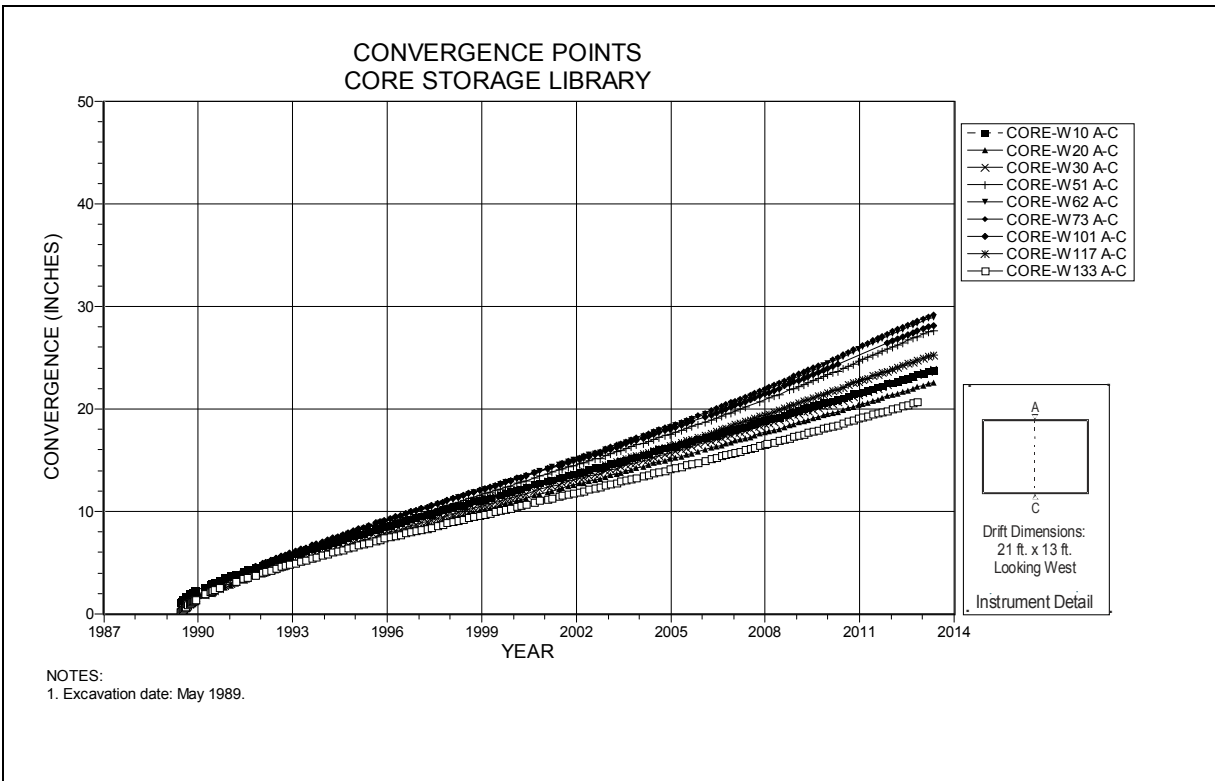
Figure 4-36 Convergence Point Array Core Storage Library – Roof to Floor
