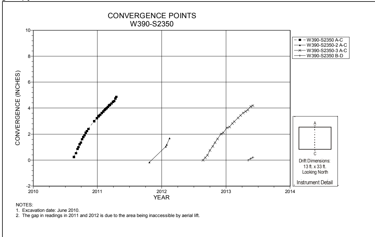
Figure 5-89 Convergence Point Array Room 1, Panel 7 at W390 S2350– Room Center – All Chords
