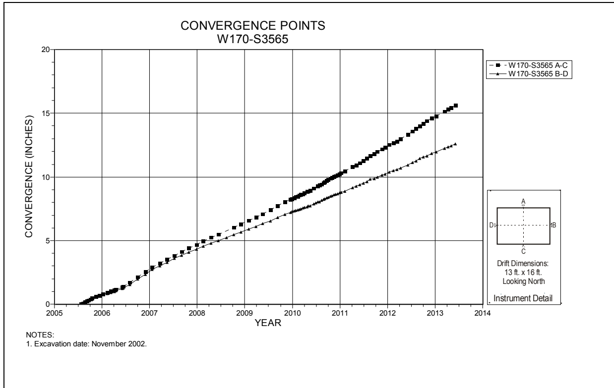
Figure 4-263 Convergence Point Array W170 S3565 – All Chords
