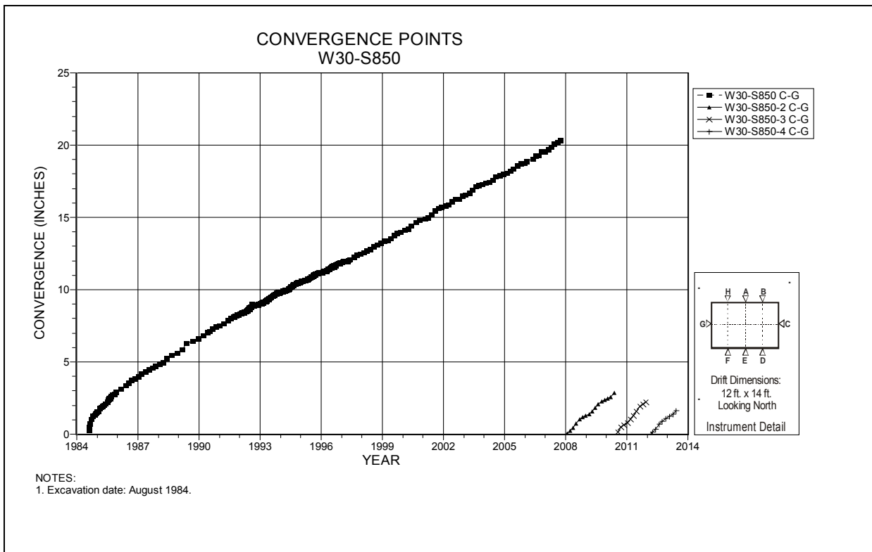
Figure 4-206 Convergence Point Array W30 S850 – Rib to Rib
