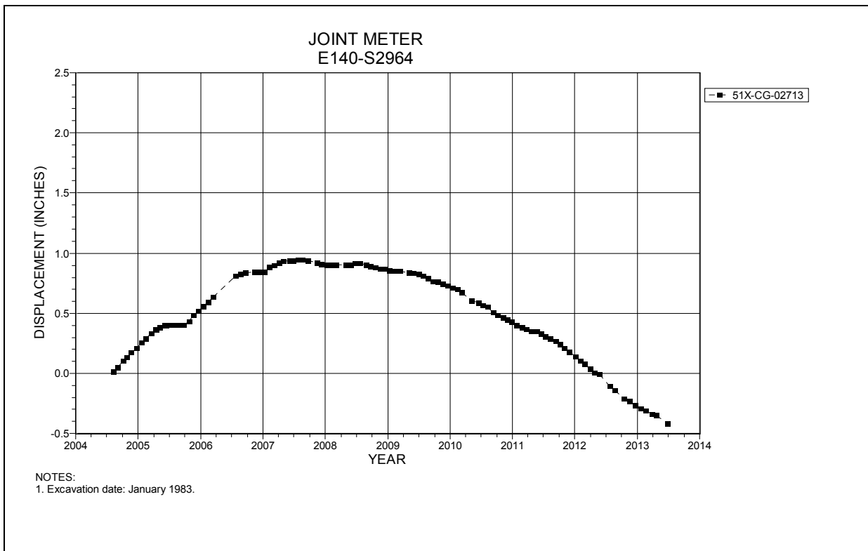
Figure 4-270 Joint Meter E140 S2964
