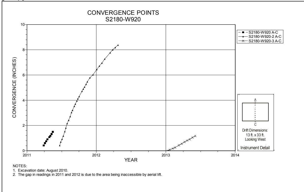
Figure 5-83 Convergence Point Array S2180 W920 Intersection (Room 5, Panel 7) – Roof to Floor
