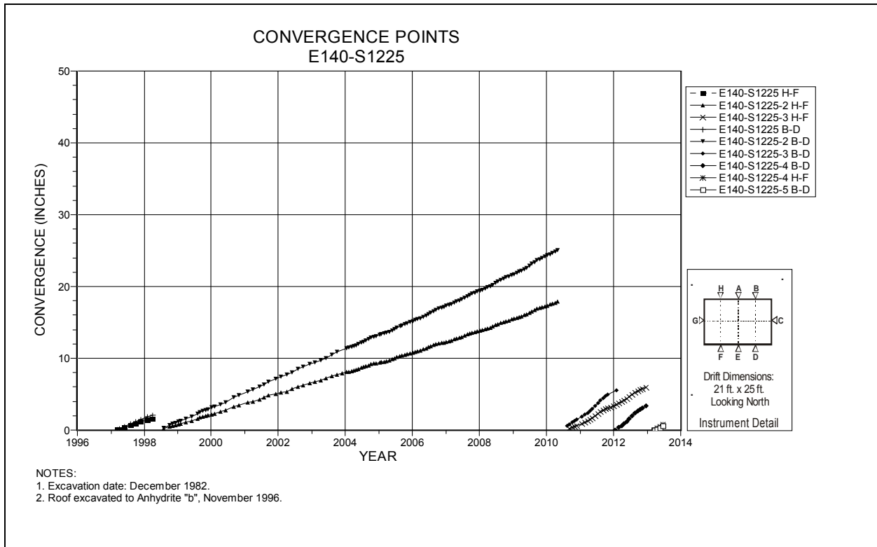
Figure 4-80 Convergence Point Array E140 S1225 – Roof to Floor – Quarter Points
