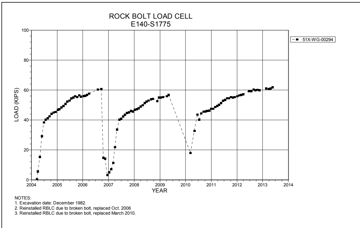
Figure 4-276 Rock Bolt Load Cell E140 S1775
