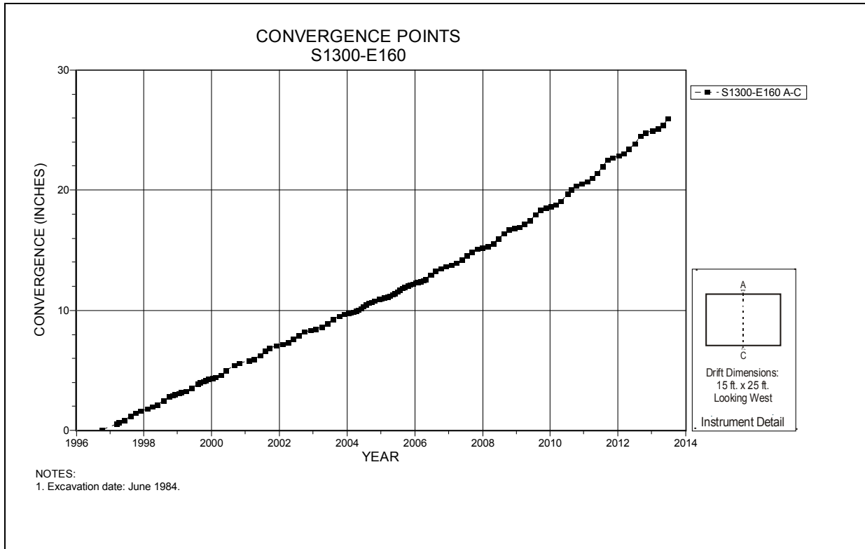
Figure 4-175 Convergence Point Array S1300 E160 – Roof to Floor
