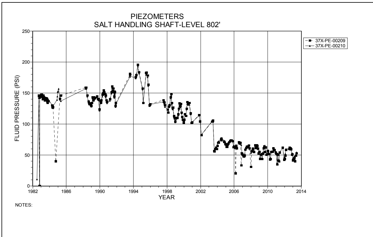
Figure 2-4 Piezometers Salt Handling Shaft – Level 802 at the Los Medaños Member
