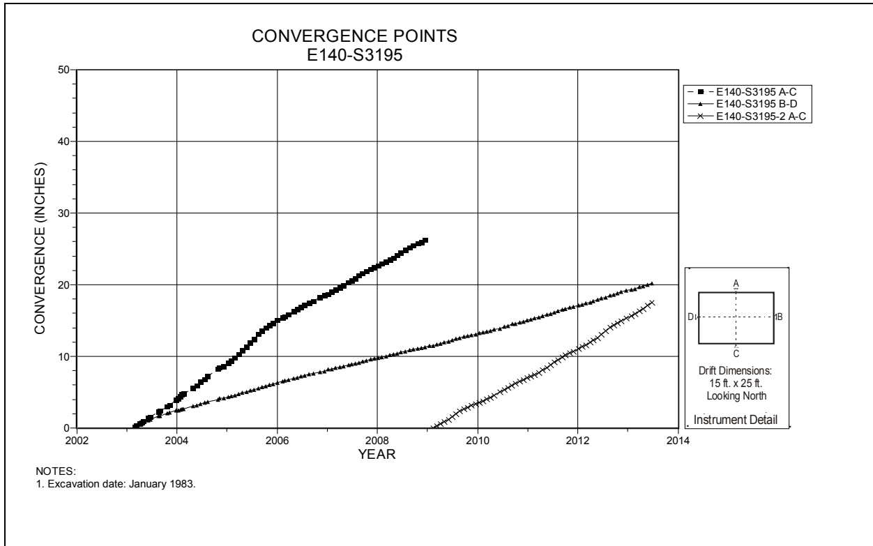
Figure 4-115 Convergence Point Array E140 S3195 – All Chords
