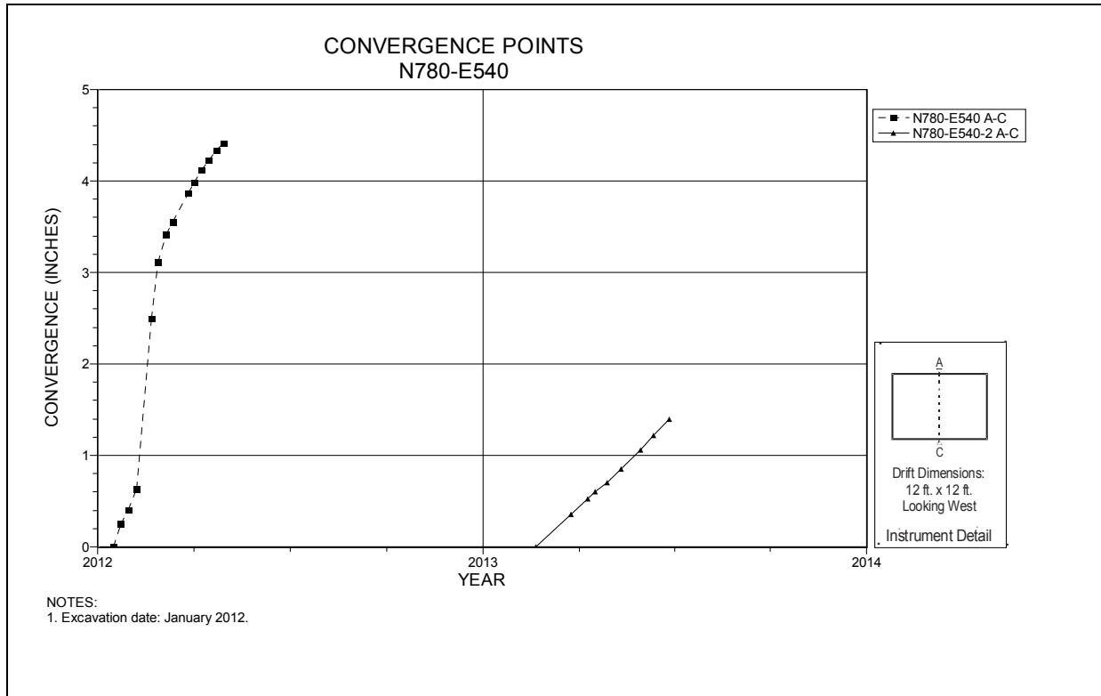
Figure 6-28 Convergence Point Array N780 E540 – Roof to Floor
