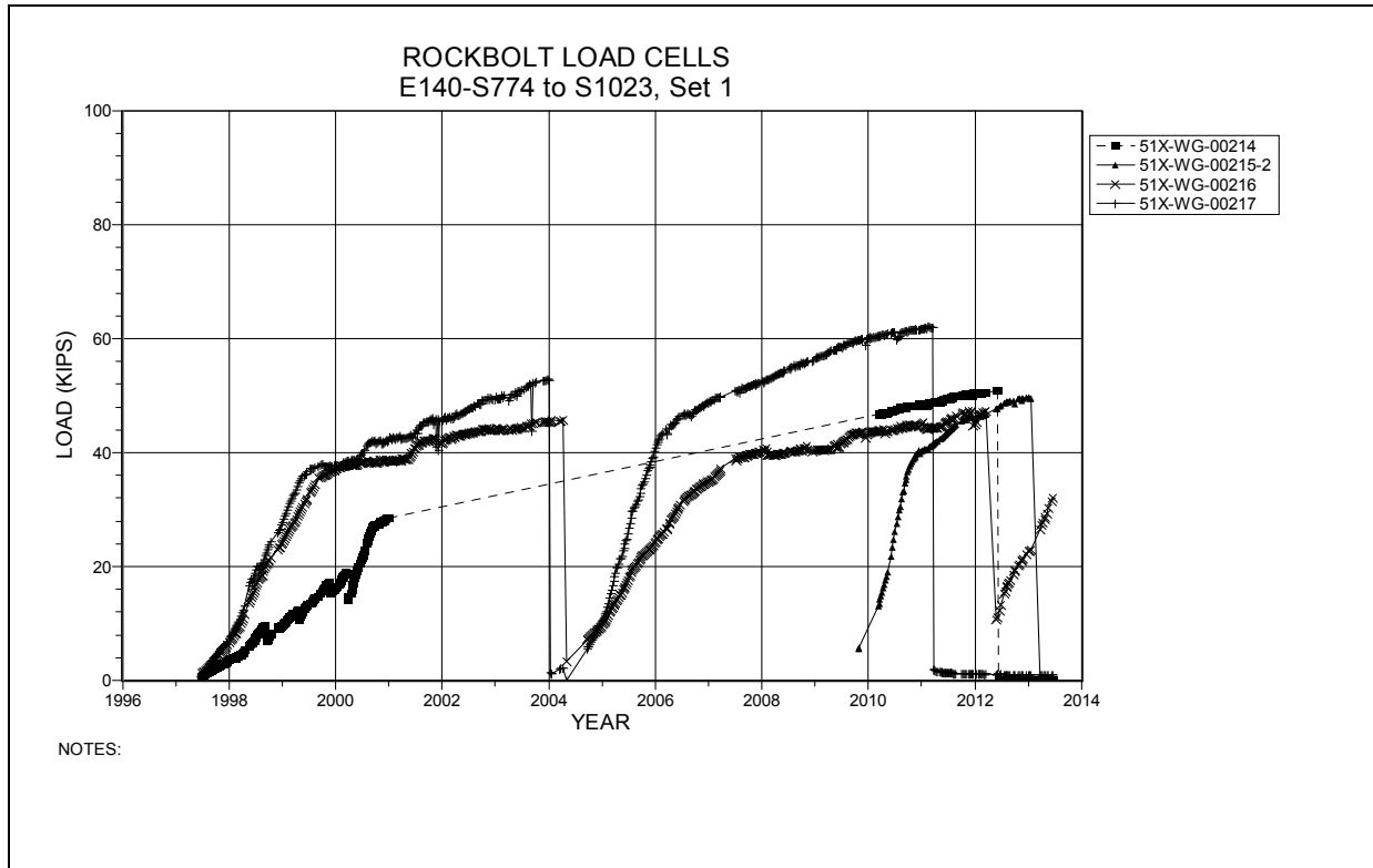
Figure 4-273 Rock Bolt Load Cells E140 S774 – S1023
