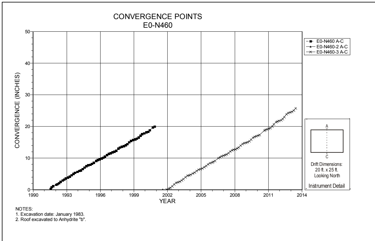
Figure 4-40 Convergence Point Array E0 N460 – Roof to Floor
