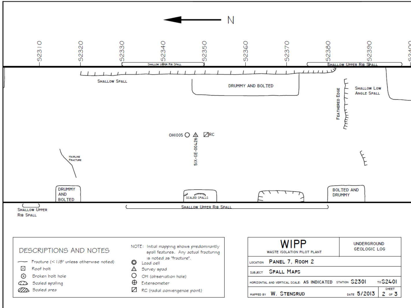
Figure 7-12 Panel 7 Room 2, S2301-S2401 Roof Fractures
