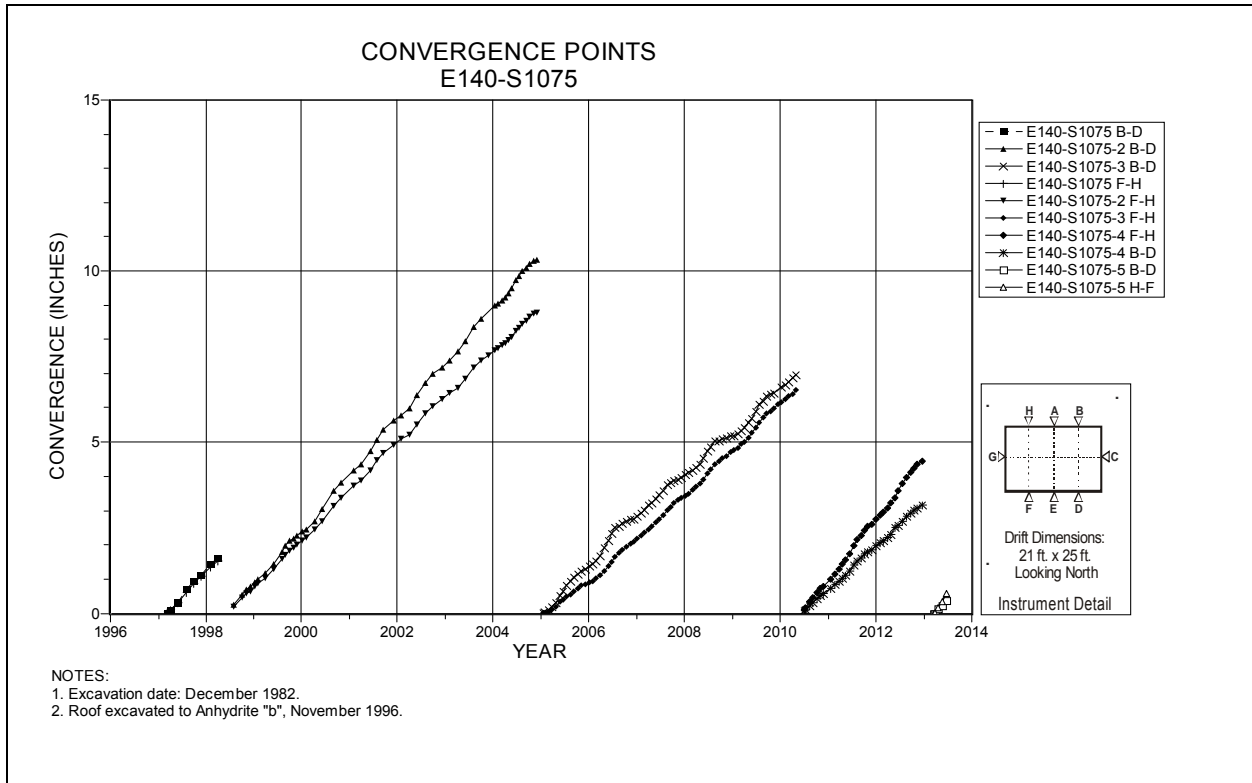
Figure 4-73 Convergence Point Array E140 S1075 – Roof to Floor – Quarter Points
