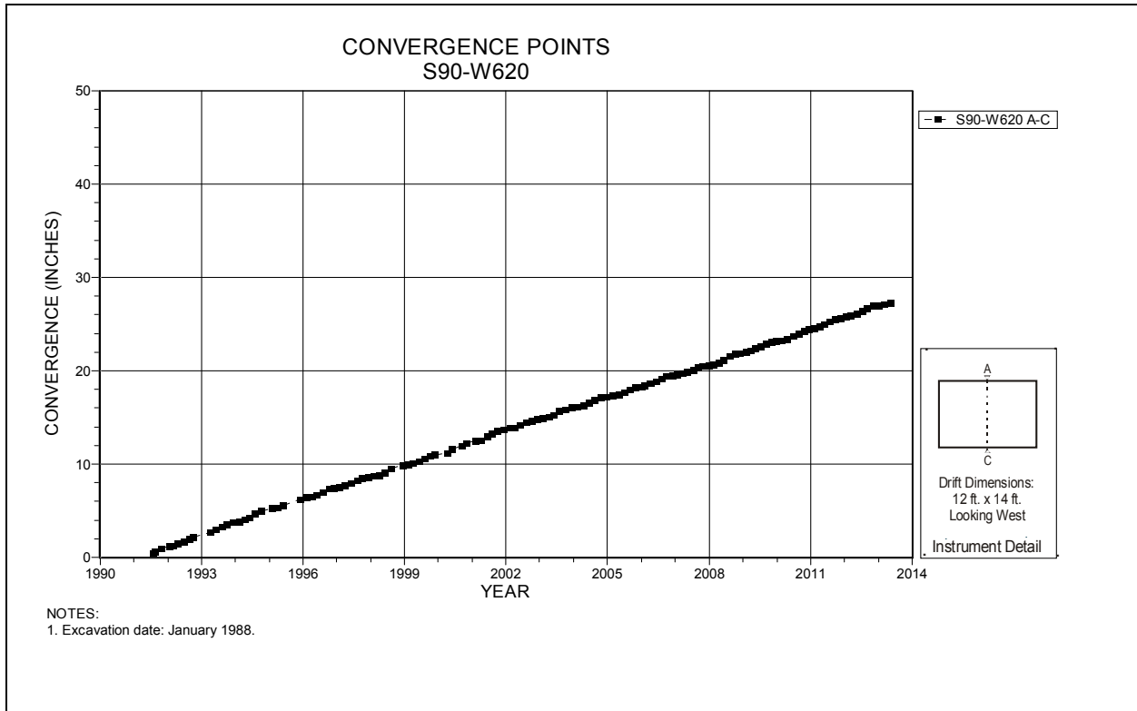
Figure 4-161 Convergence Point Array S90 W620 – Roof to Floor
