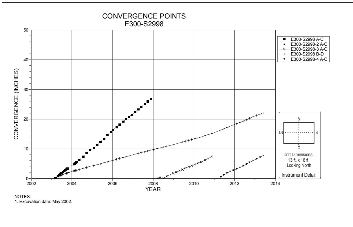
Figure 4-148 Convergence Point Array E300 S2998 – All Chords
