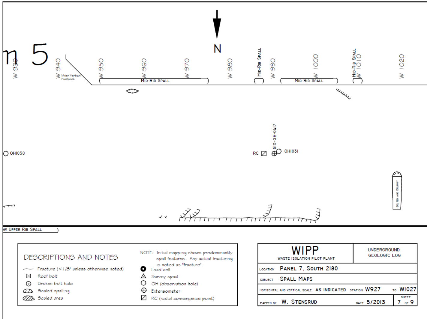
Figure 7-35 Panel 7 South 2180, W927-W1027 Roof Fractures
