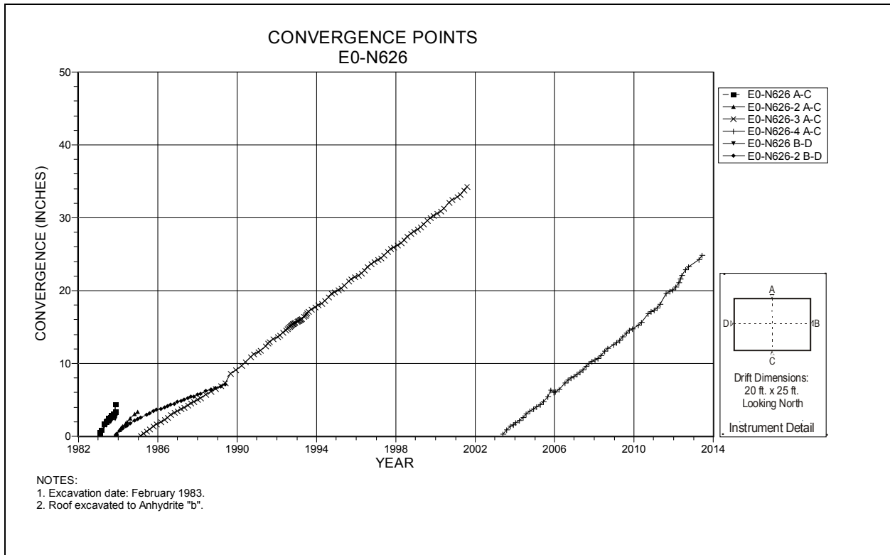
Figure 4-42 Convergence Point Array E0 N626 – All Chords
