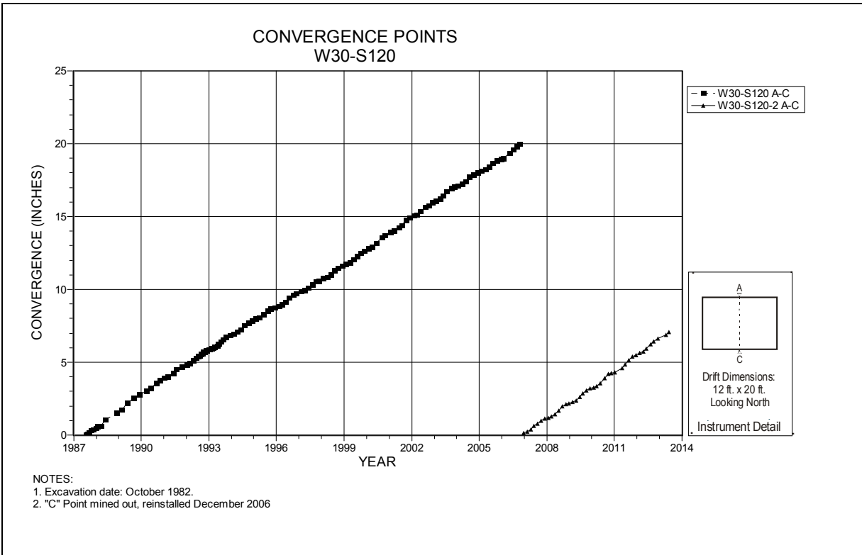
Figure 4-199 Convergence Point Array W30 S120 – Roof to Floor
