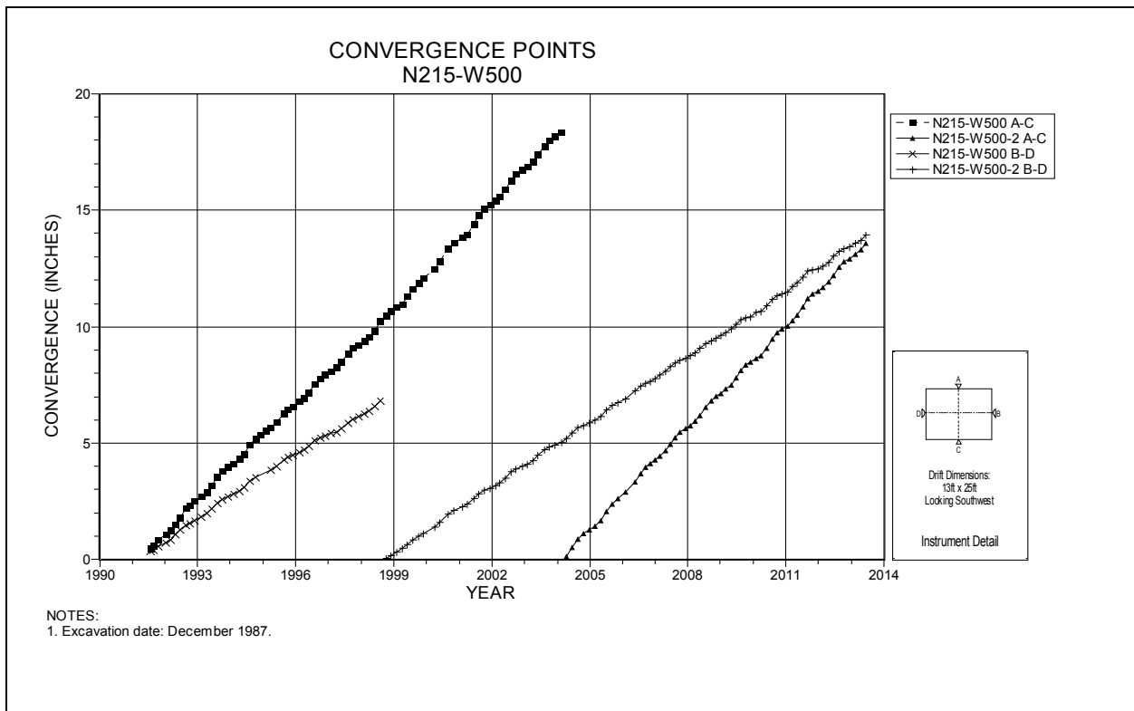
Figure 4-152 Convergence Point Array N215 W500 – All Chords
