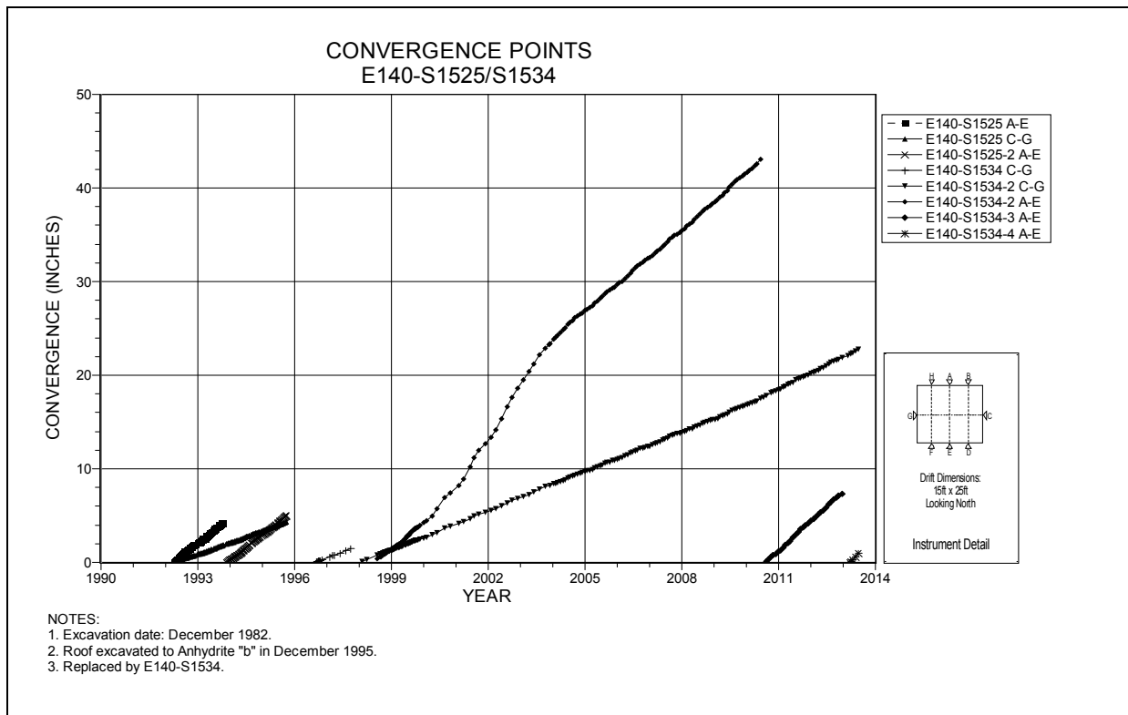
Figure 4-90 Convergence Point Array E140 S1525/S1534 – Roof to Floor – Centerline and Rib to Rib
