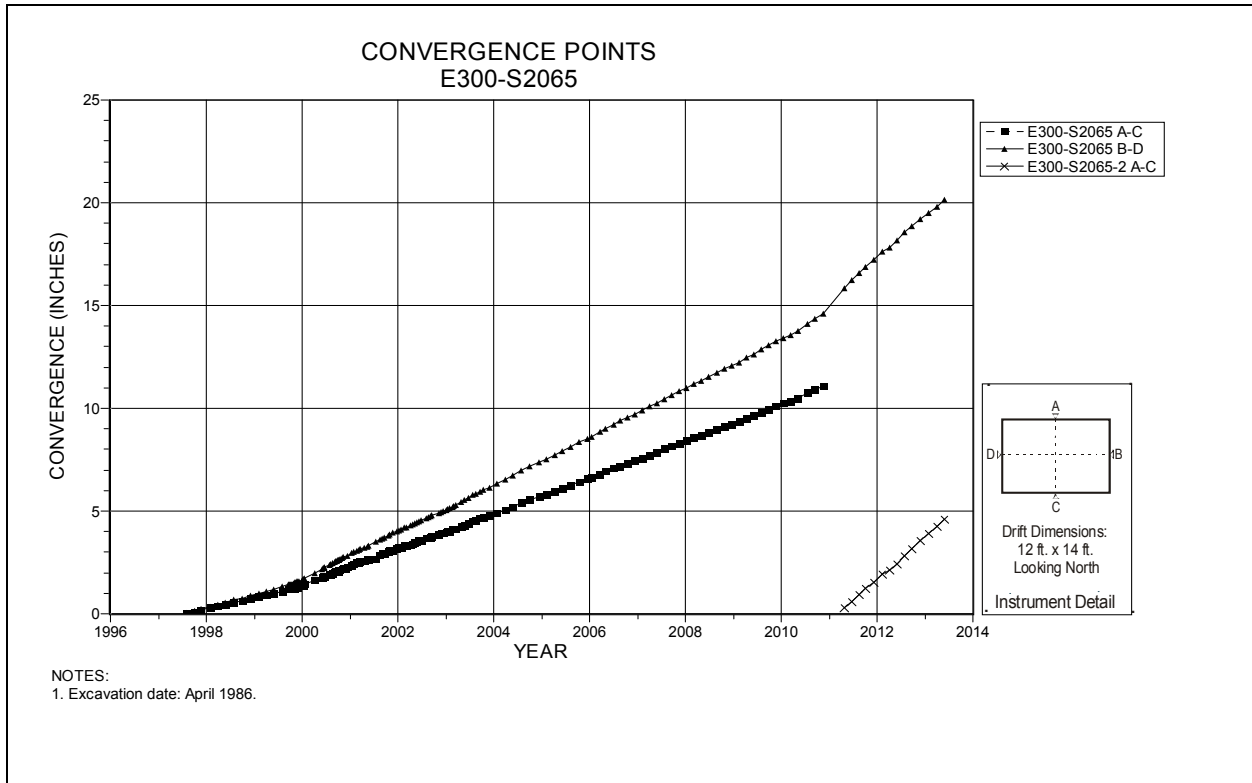
Figure 4-141 Convergence Point Array E300 S2065 – All Chords
