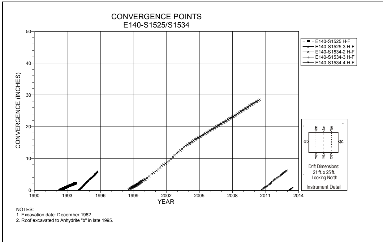
Figure 4-92 Convergence Point Array E140 S1525/S1534 – Roof to Floor – West Quarter Point
