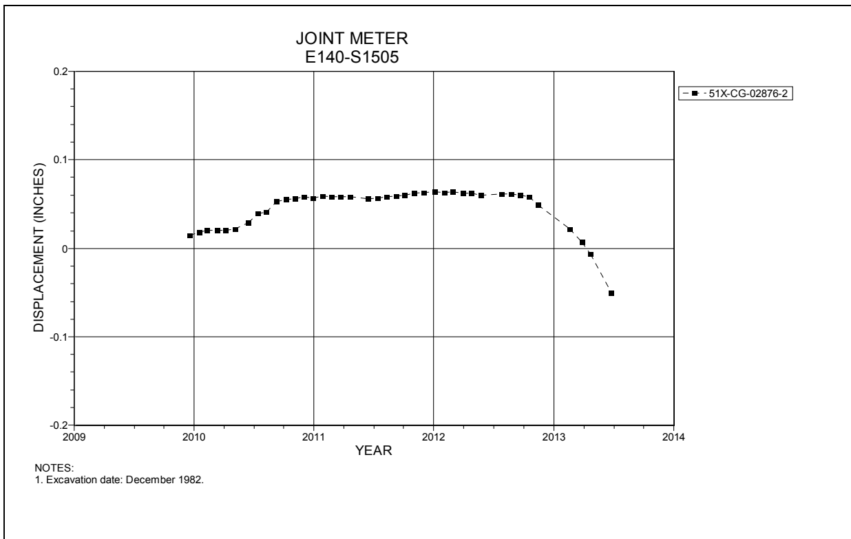
Figure 4-266 Joint Meter E140 S1505
