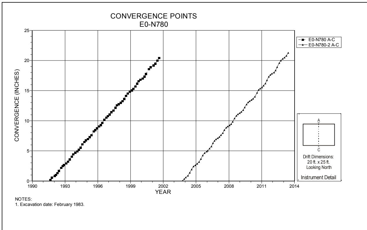
Figure 4-44 Convergence Point Array E0 N780 – Roof to Floor
