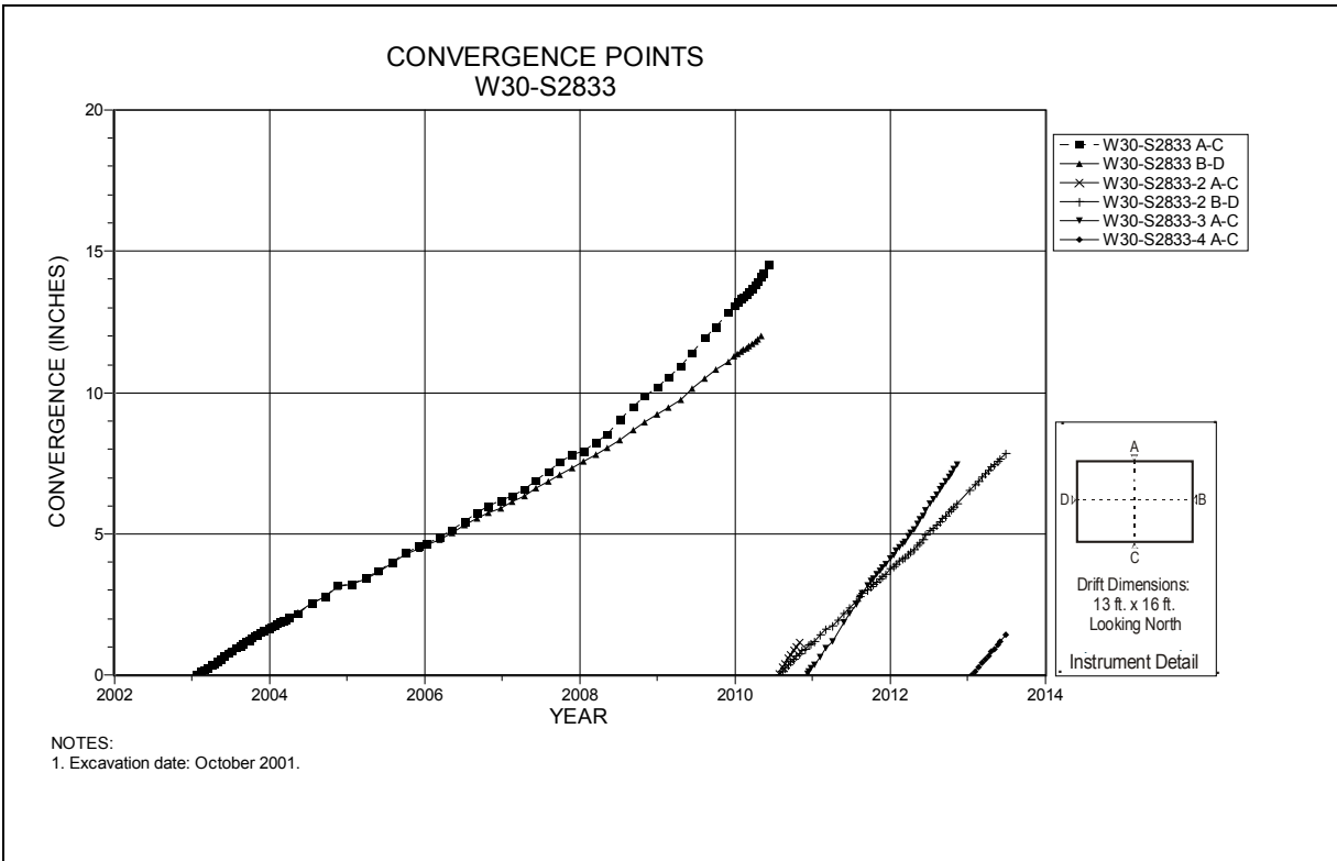
Figure 4-221 Convergence Point Array W30 S2833 – All Chords
