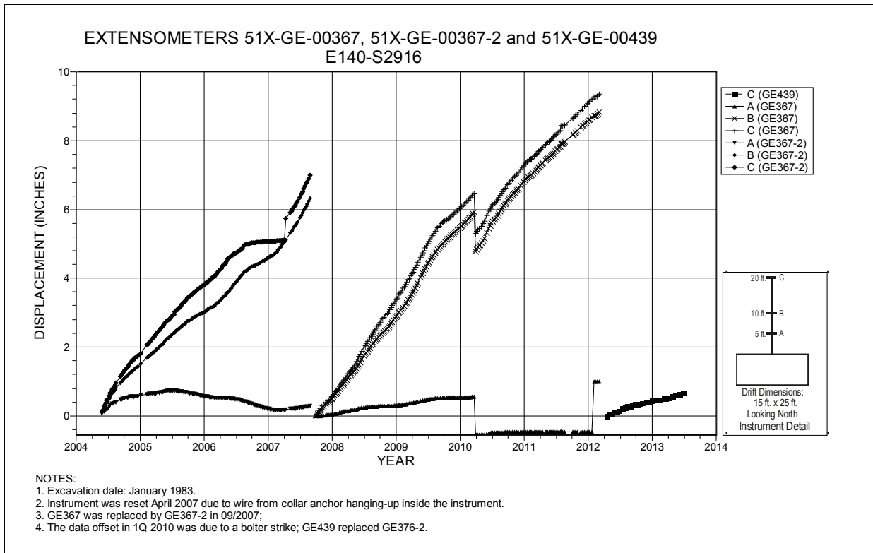
Figure 4-22 Extensometers 51X-GE-00367, 51X-GE-00367-2 and 51X-GE-00439 E140 S2916 – Roof
