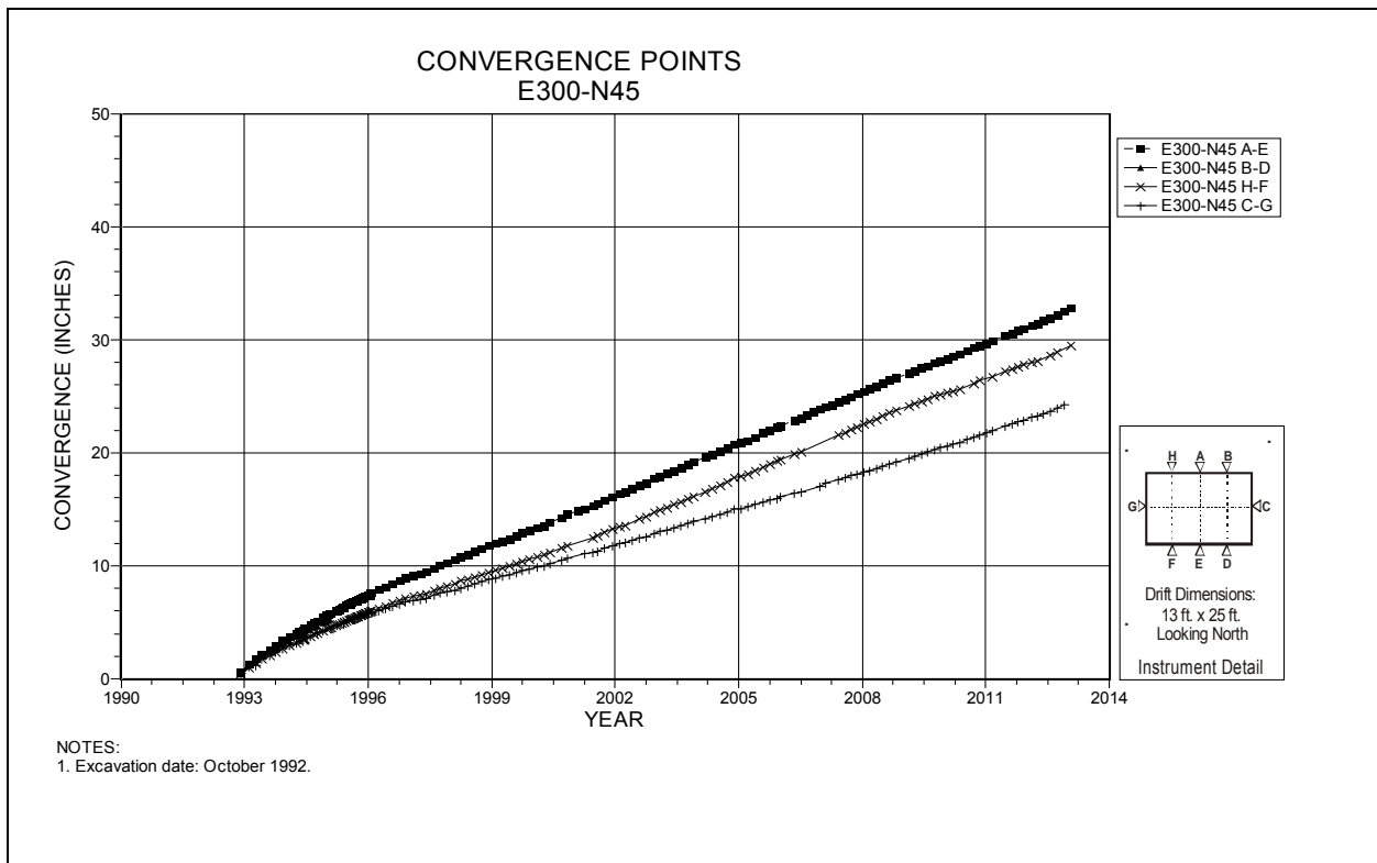
Figure 4-122 Convergence Point Array E300 N45 – All Chords
