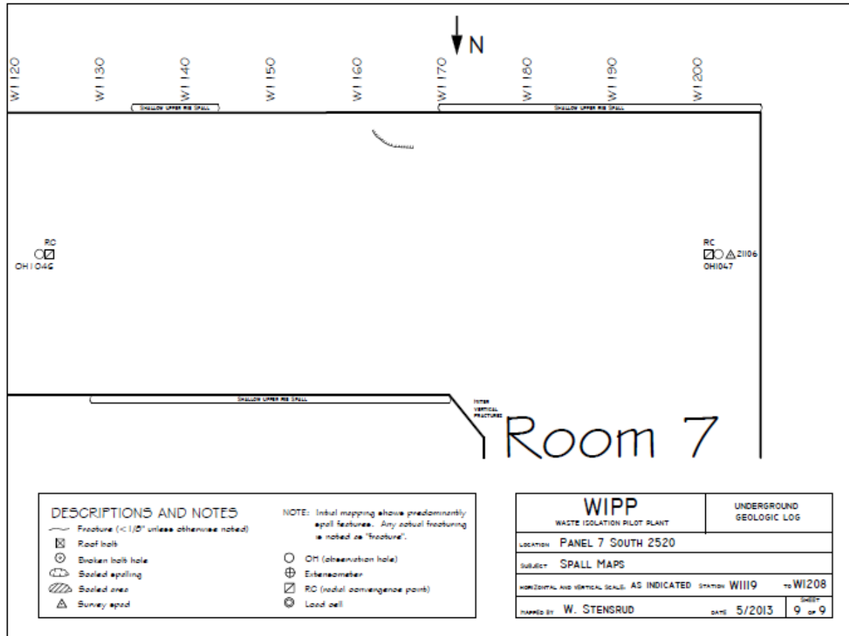
Figure 7-46 Panel 7 South 2520, W1119-W1208 Roof Fractures
