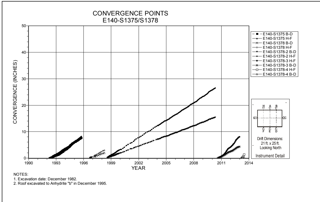
Figure 4-83 Convergence Point Array E140 S1375/S1378 – Roof to Floor – Quarter Points
