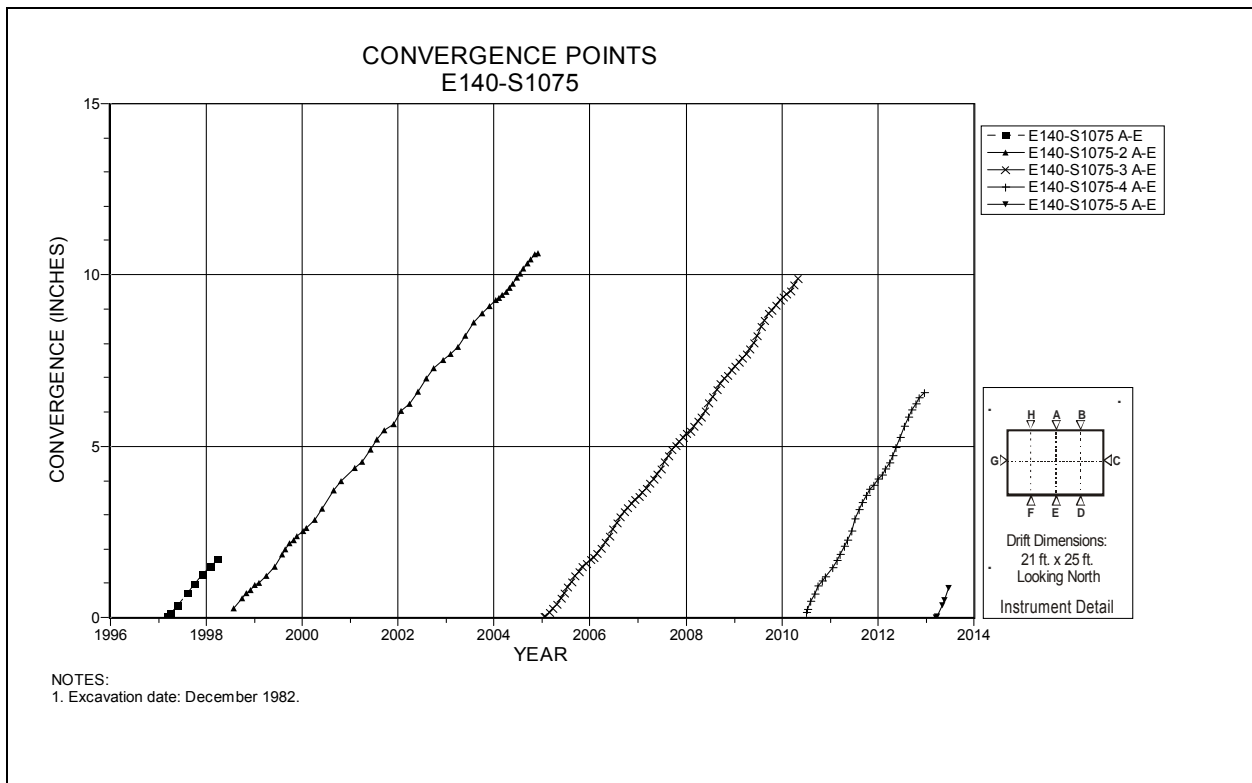
Figure 4-72 Convergence Point Array E140 S1075 – Roof to Floor – Centerline
