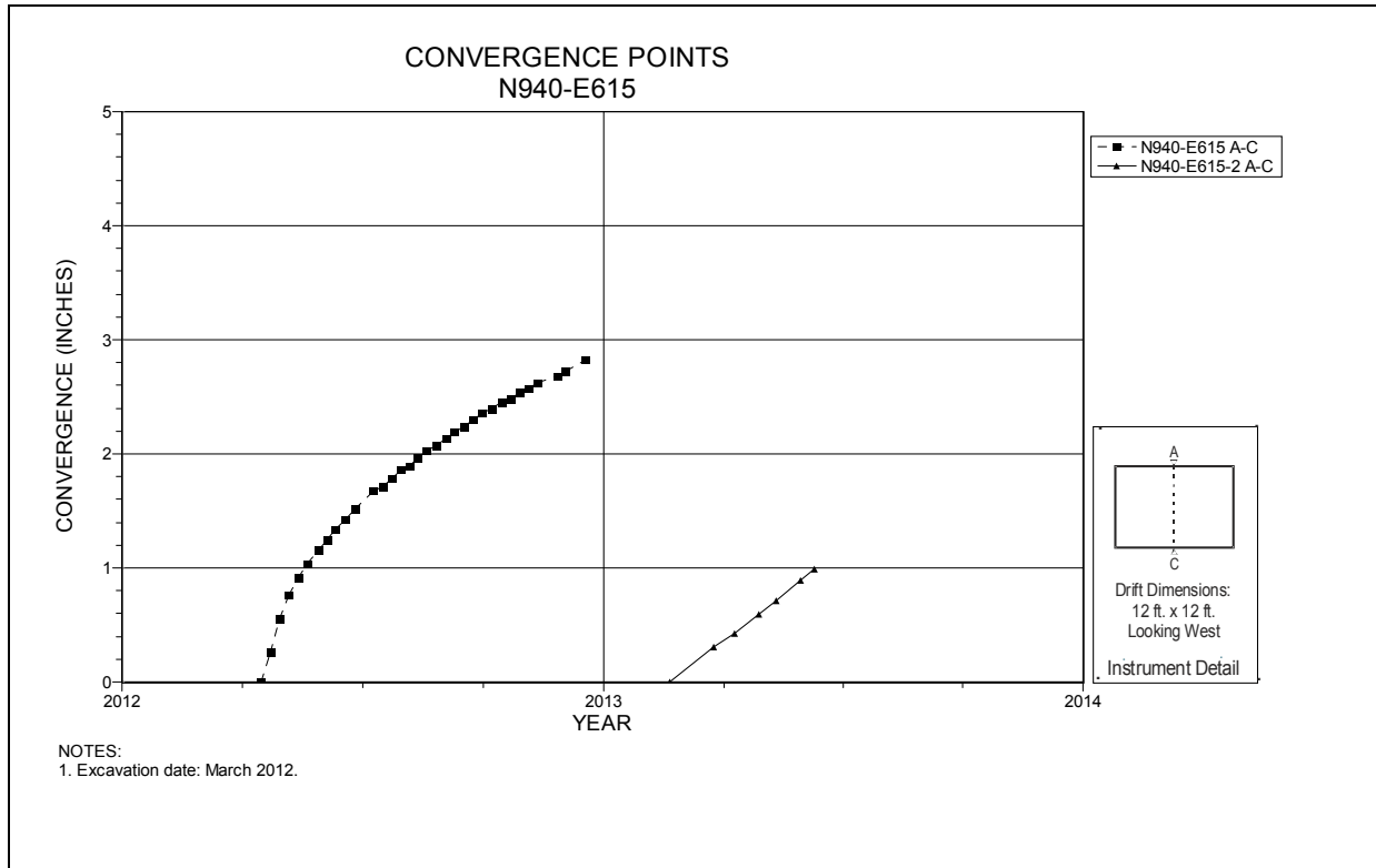
Figure 6-44 Convergence Point Array N940 E615 – Roof to Floor
