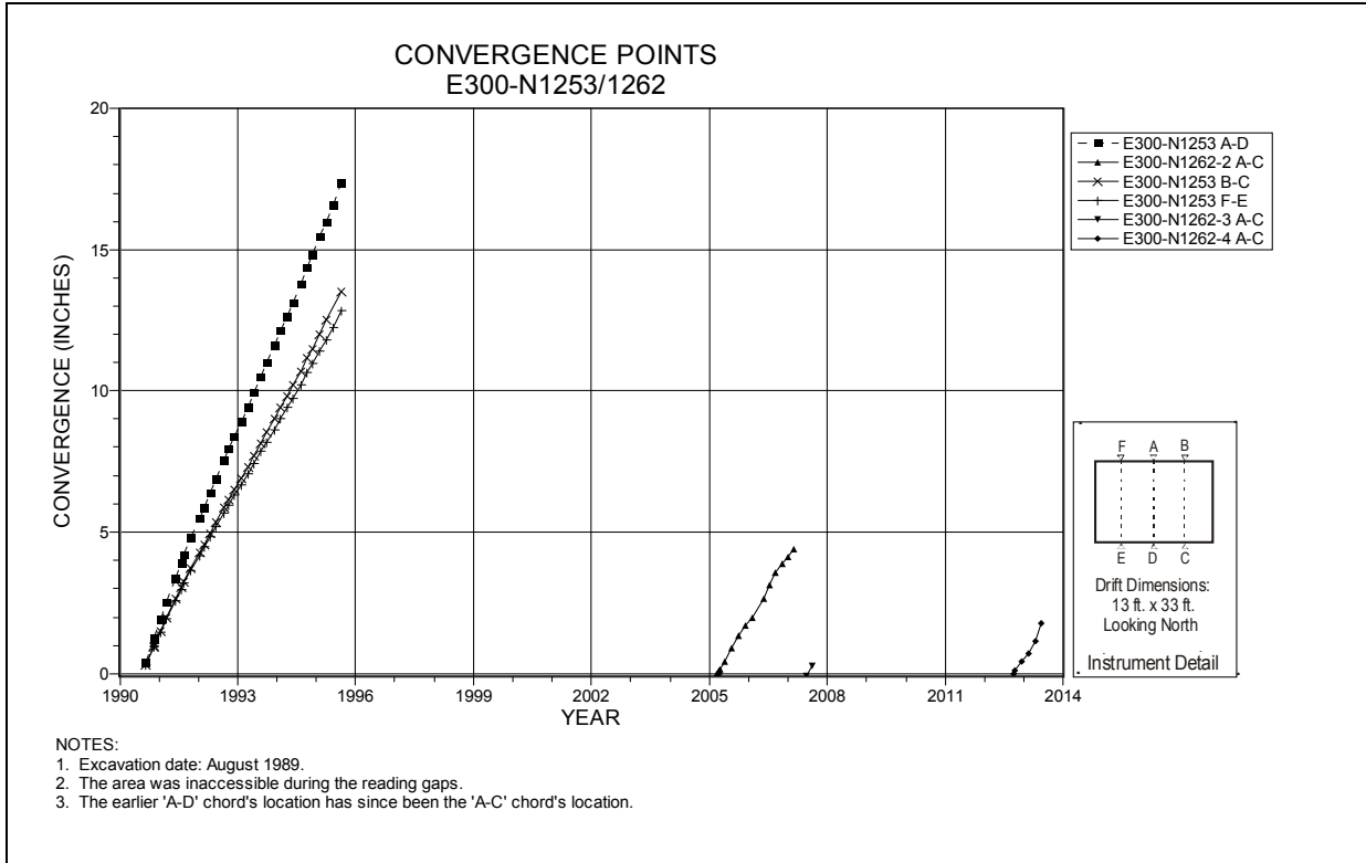
Figure 4-125 Convergence Point Array E300 N1253/N1262 – Roof to Floor
