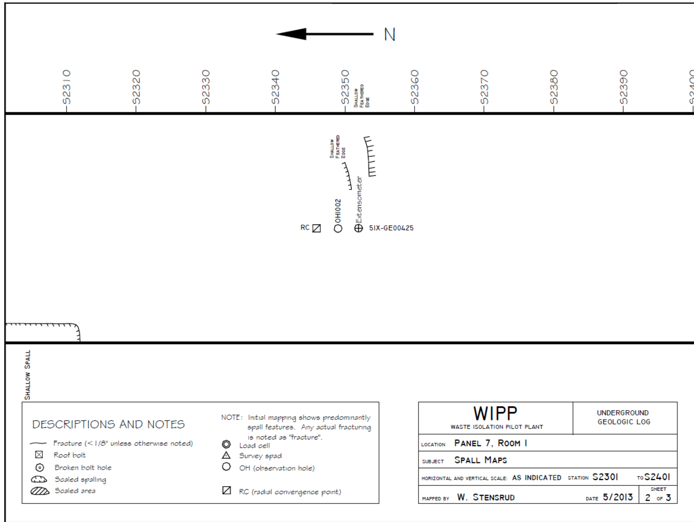
Figure 7-9 Panel 7 Room 1, S2301-S2401 Roof Fractures
