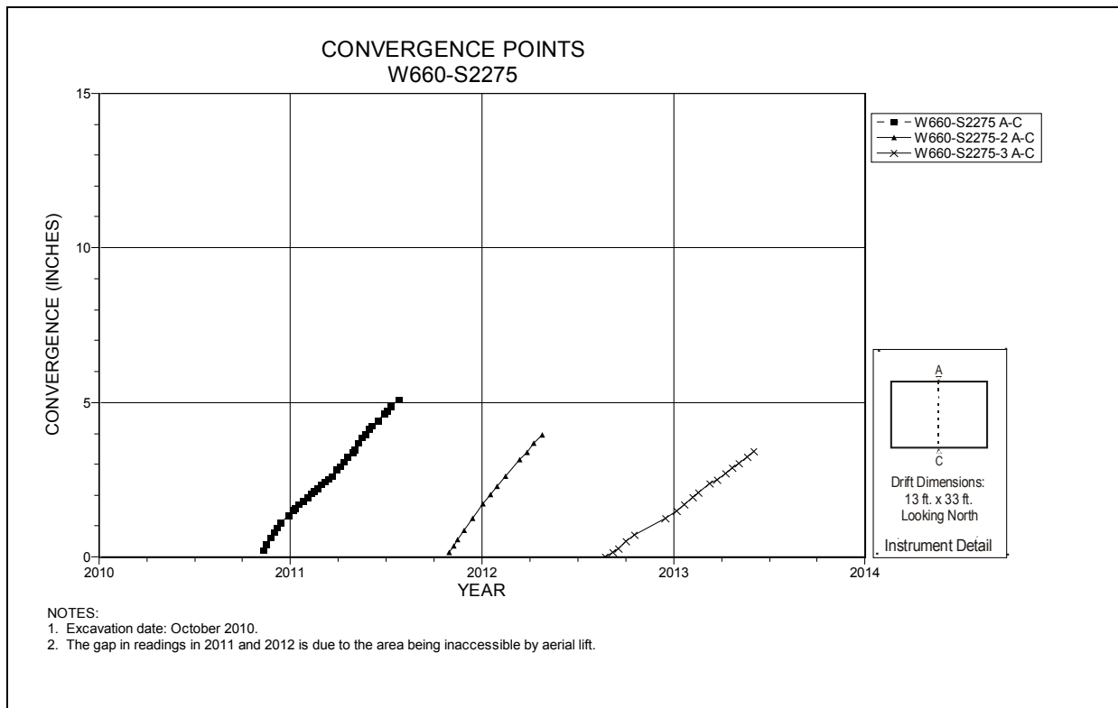
Figure 5-94 Convergence Point Array Room 3, Panel 7 at W660 S2275 – Roof to Floor
