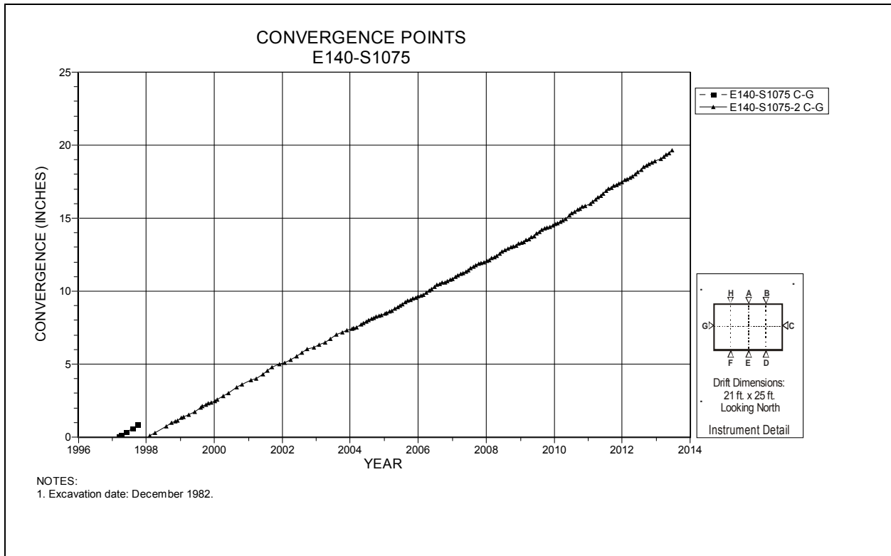
Figure 4-74 Convergence Point Array E140 S1075 – Rib to Rib
