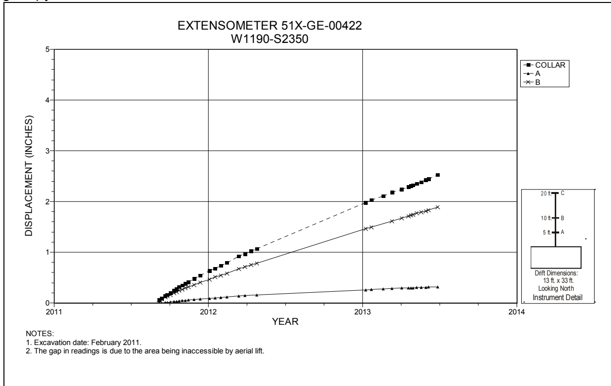
Figure 5-71 Extensometer 51X-GE-00422 Room 7, Panel 7 at W1190 S2350 – Room Center – Roof
