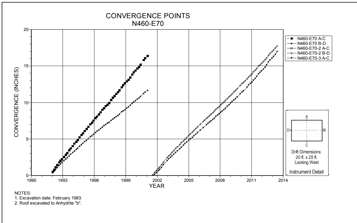
Figure 4-156 Convergence Point Array N460 E70 – All Chords
