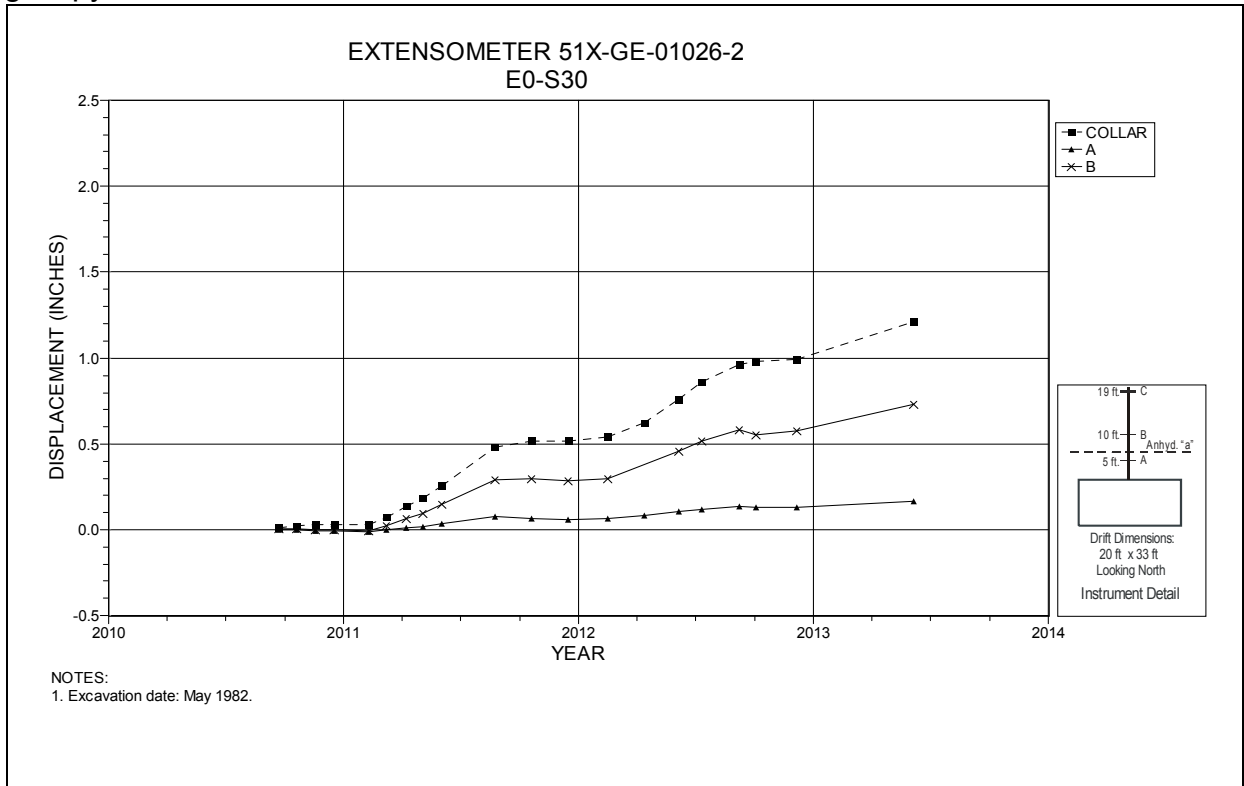
Figure 3-5 Extensometer 51X-GE-001026-2 Salt Handling Shaft Station at S30 – Roof
