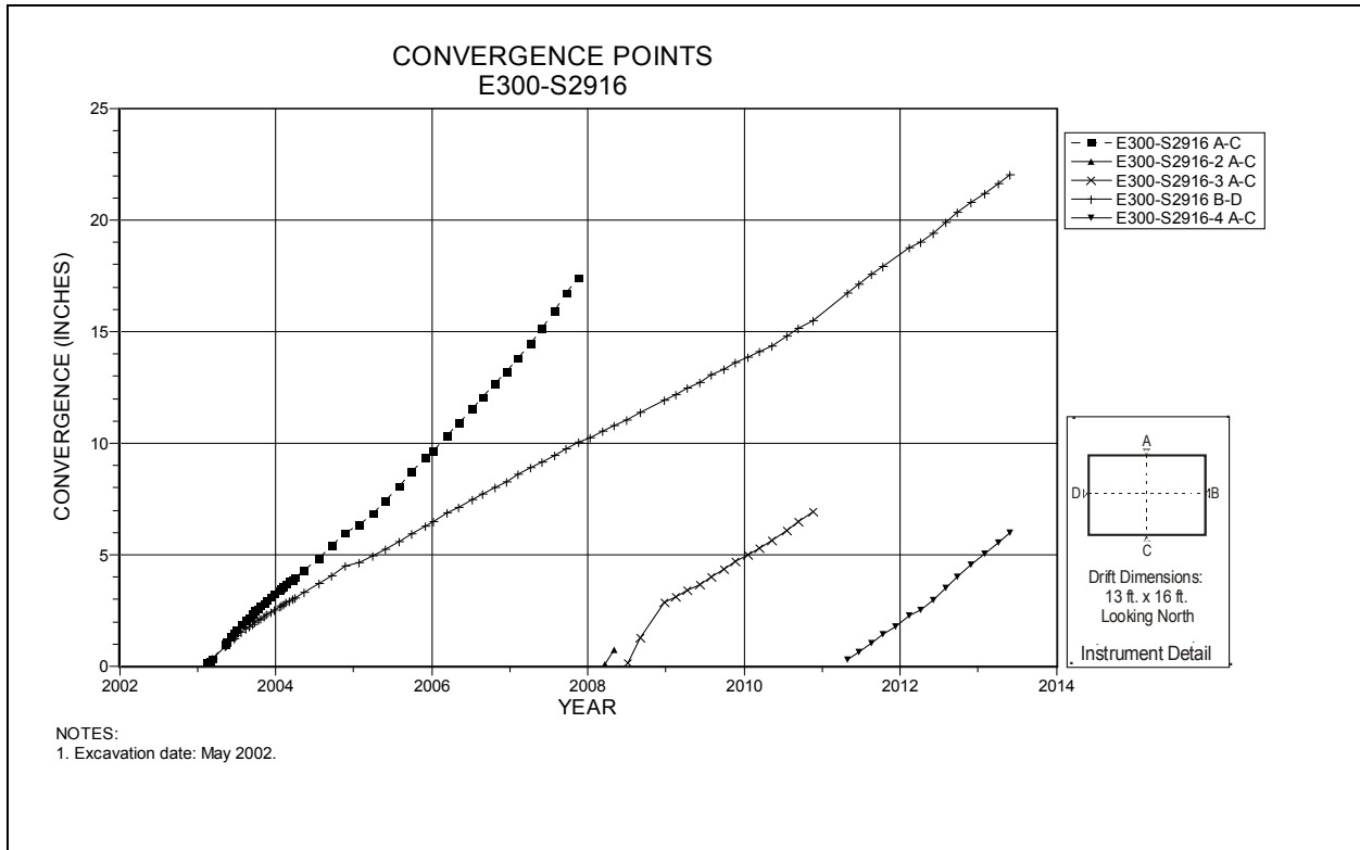
Figure 4-147 Convergence Point Array E300 S2916 – All Chords
