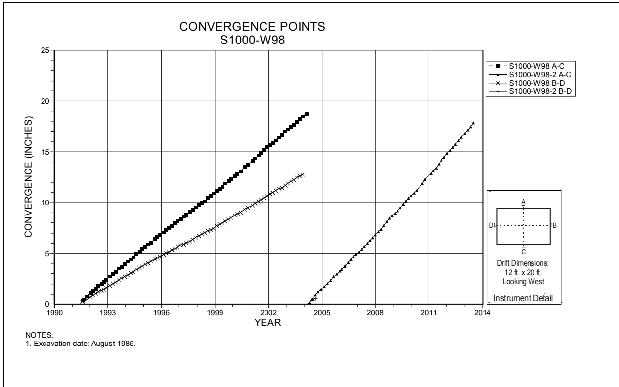
Figure 4-172 Convergence Point Array S1000 W98 – All Chords
