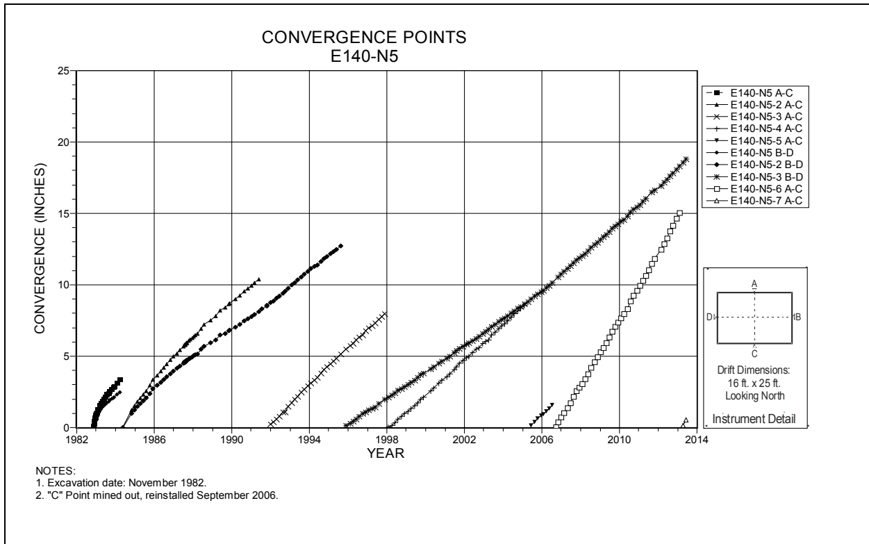
Figure 4-48 Convergence Point Array E140 N5 – All Chords
