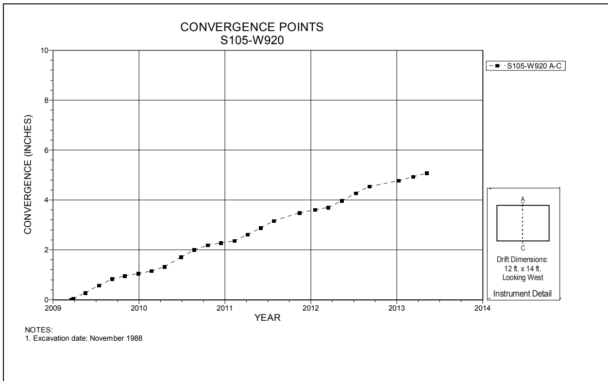
Figure 4-164 Convergence Point Array S105 W920 – Roof to Floor
