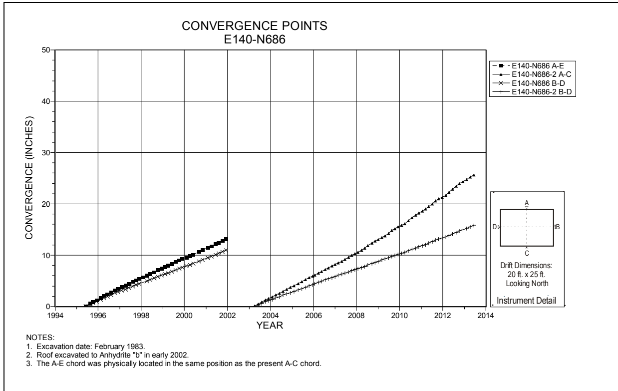
Figure 4-55 Convergence Point Array E140 N686 – All Chords
