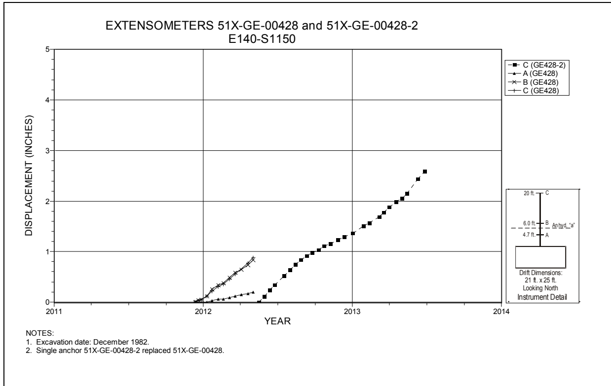
Figure 4-11 Extensometers 51X-GE-00428 and 51X-GE-00428-2 E140 S1150 – Roof
