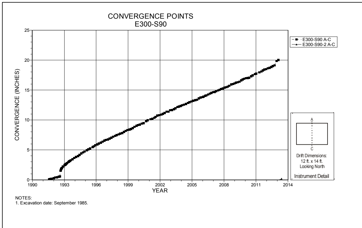
Figure 4-128 Convergence Point Array E300 S90 – Roof to Floor
