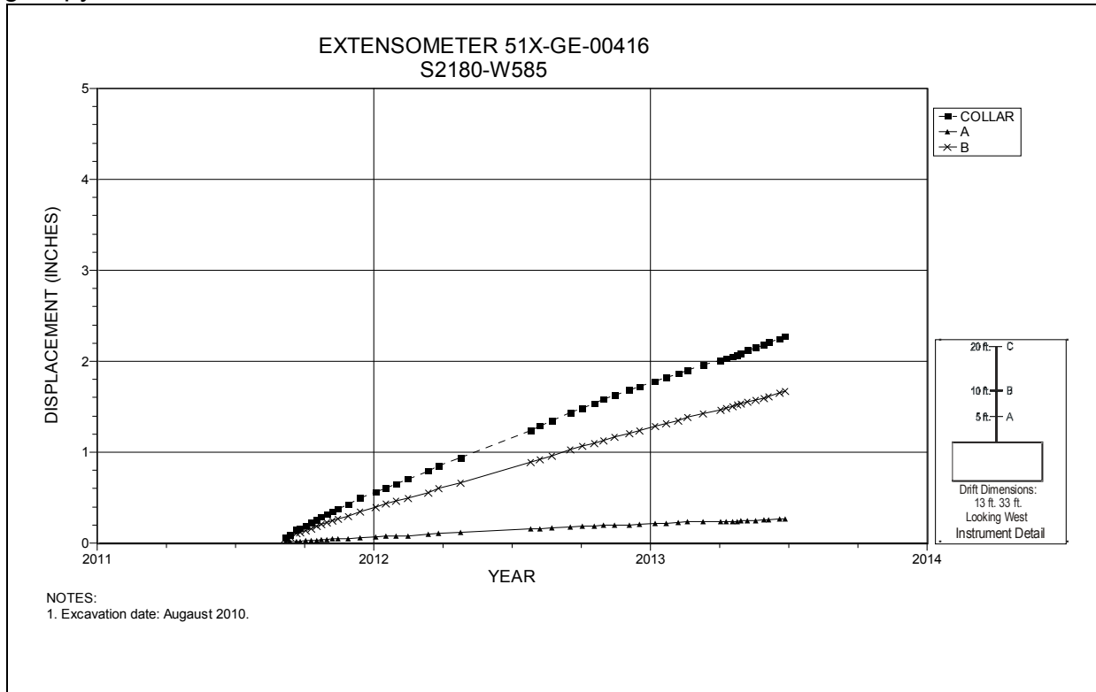
Figure 5-63 Extensometer 51X-GE-00416 S2180 W585 – Roof
