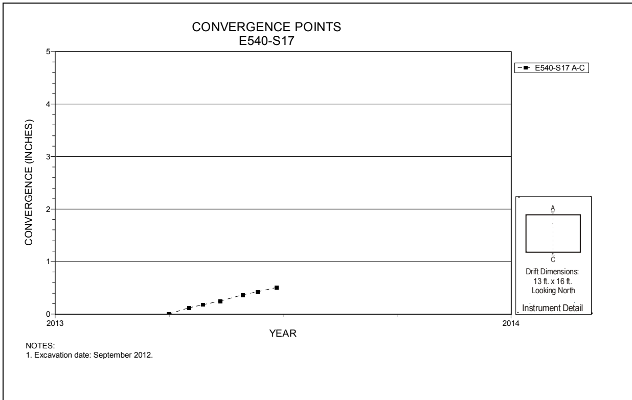
Figure 6-1 Convergence Point Array E540 S17 – Roof to Floor
