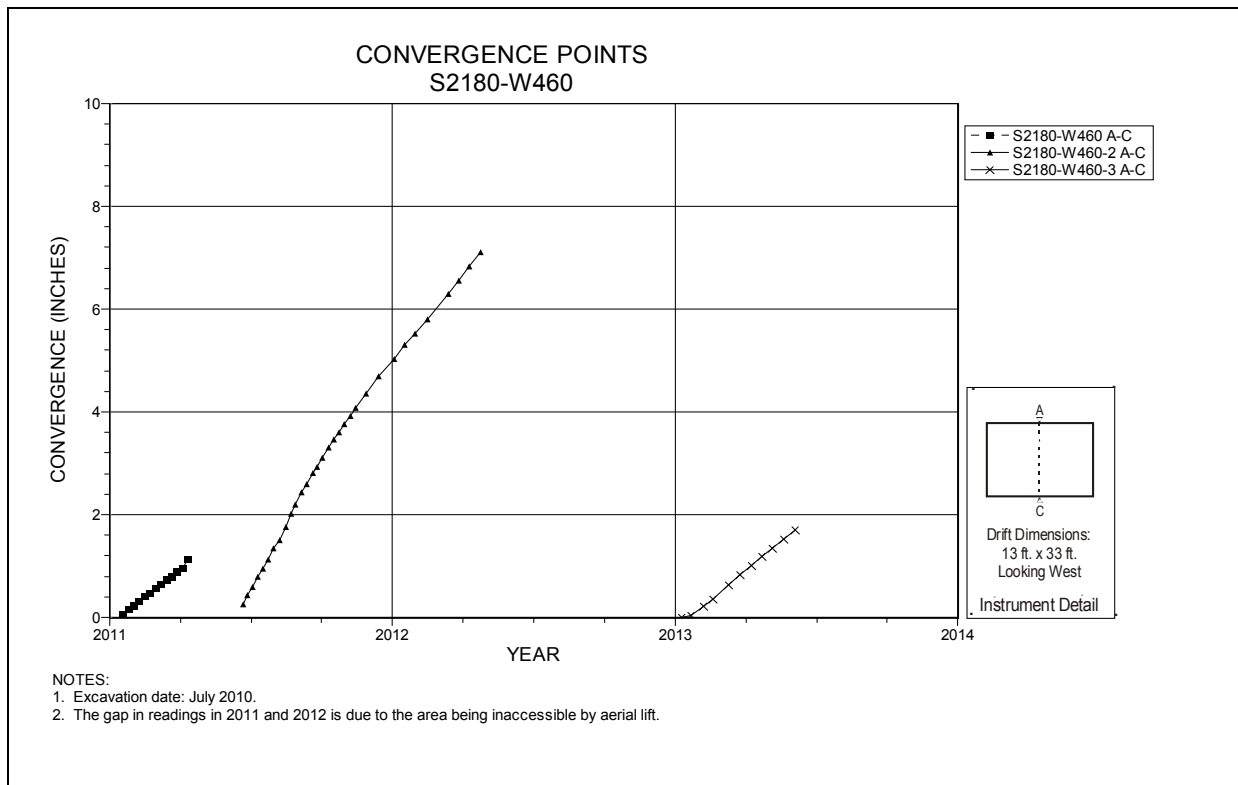
Figure 5-76 Convergence Point Array S2180 W460 – Roof to Floor
