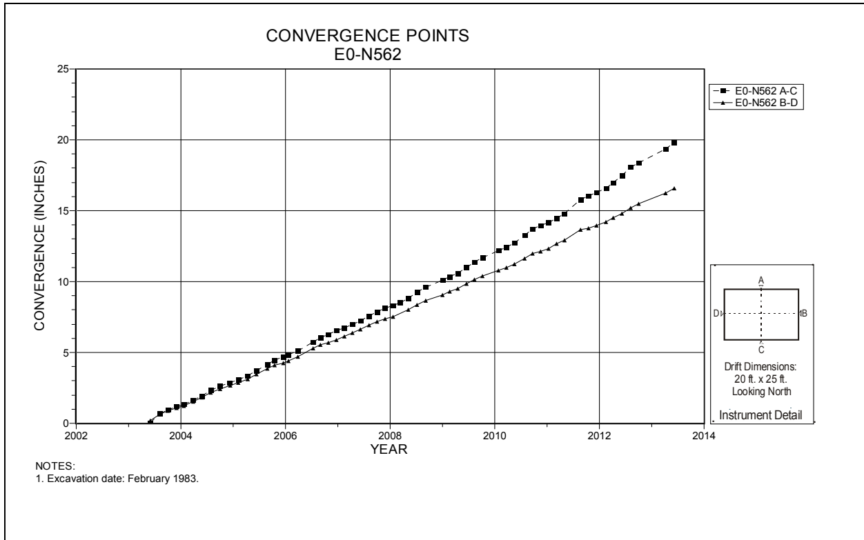
Figure 4-41 Convergence Point Array E0 N562 – All Chords
