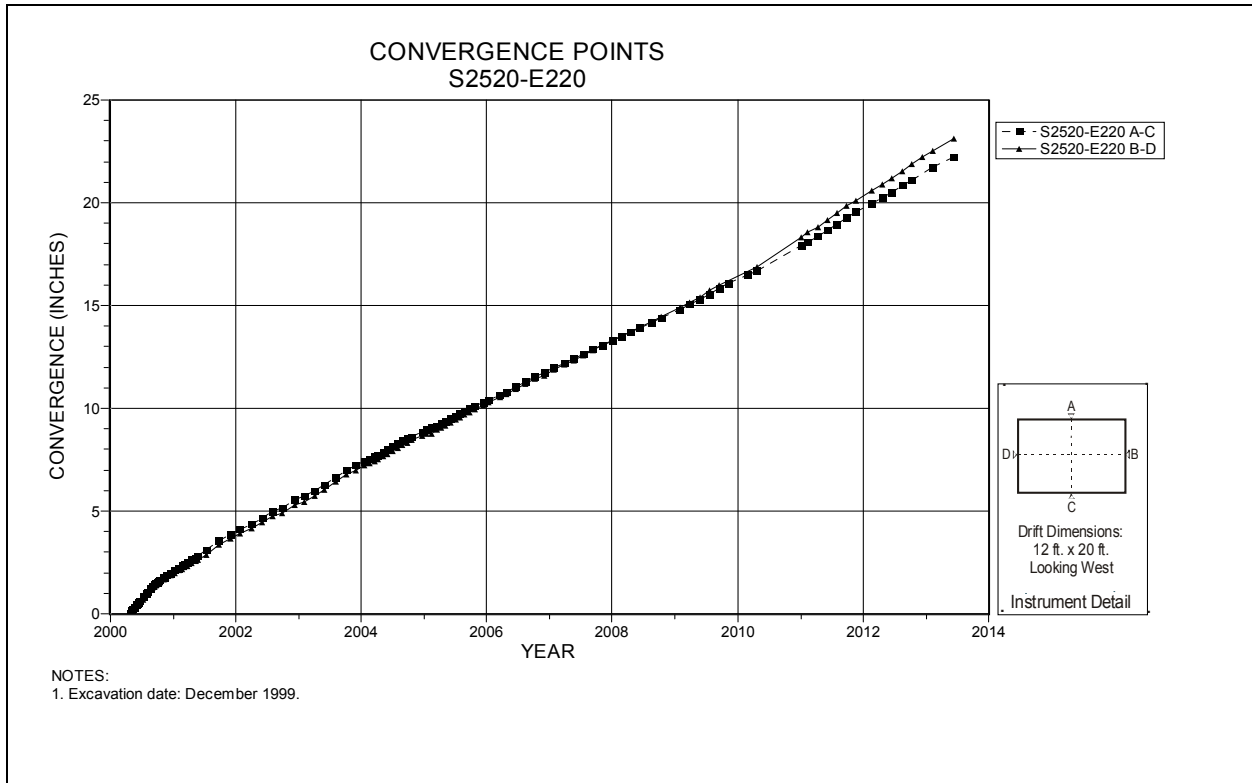
Figure 4-185 Convergence Point Array S2520 E220 – All Chords
