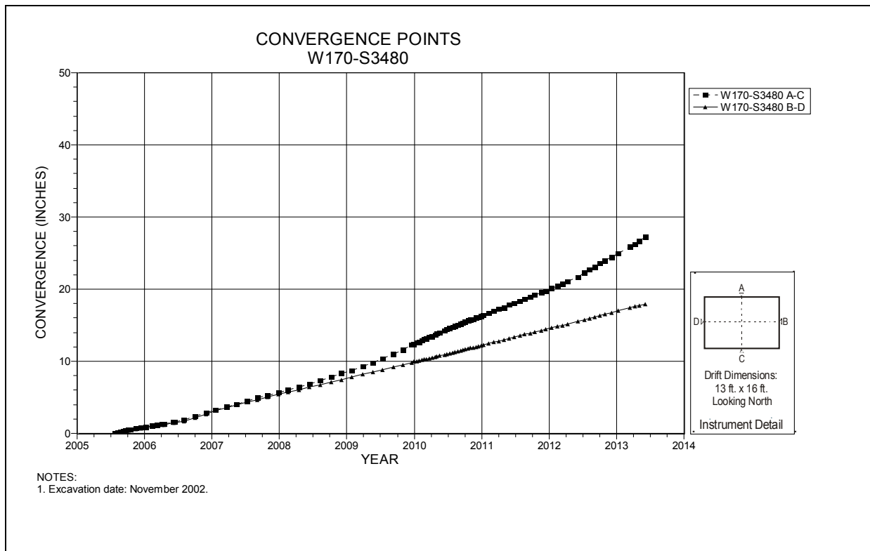
Figure 4-262 Convergence Point Array W170 S3480 – All Chords
