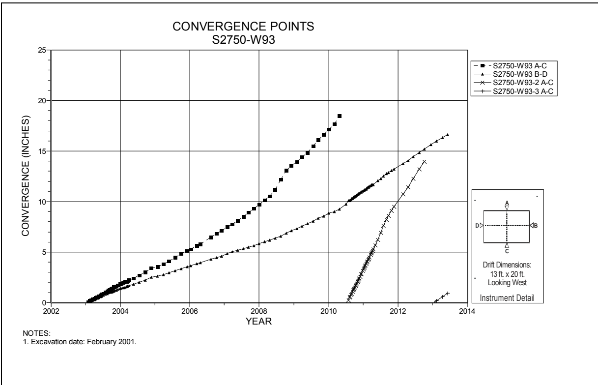
Figure 4-190 Convergence Point Array S2750 W93 – All Chords
