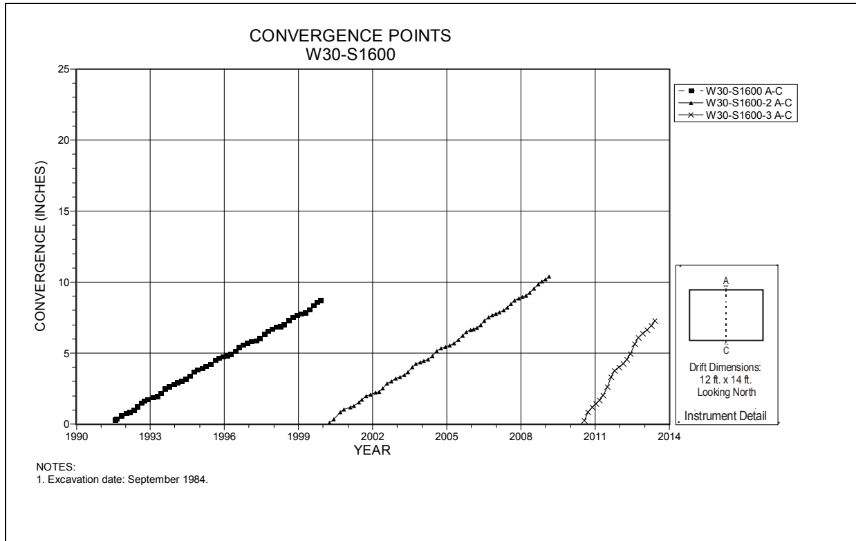
Figure 4-211 Convergence Point Array W30 S1600 – Roof to Floor
