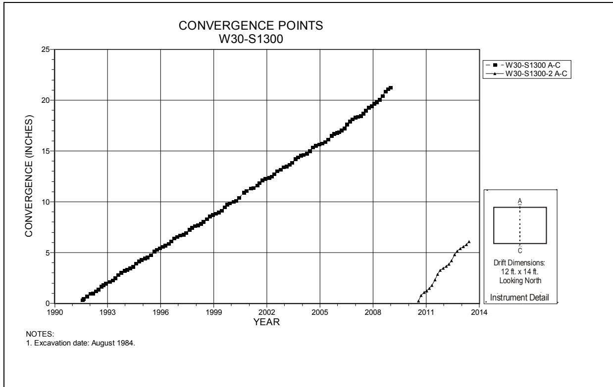
Figure 4-209 Convergence Point Array W30 S1300 – Roof to Floor
