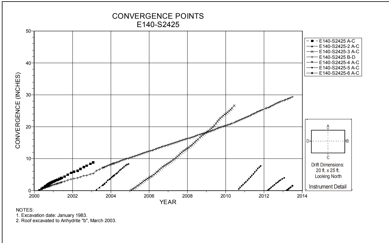
Figure 4-107 Convergence Point Array E140 S2425 – All Chords
