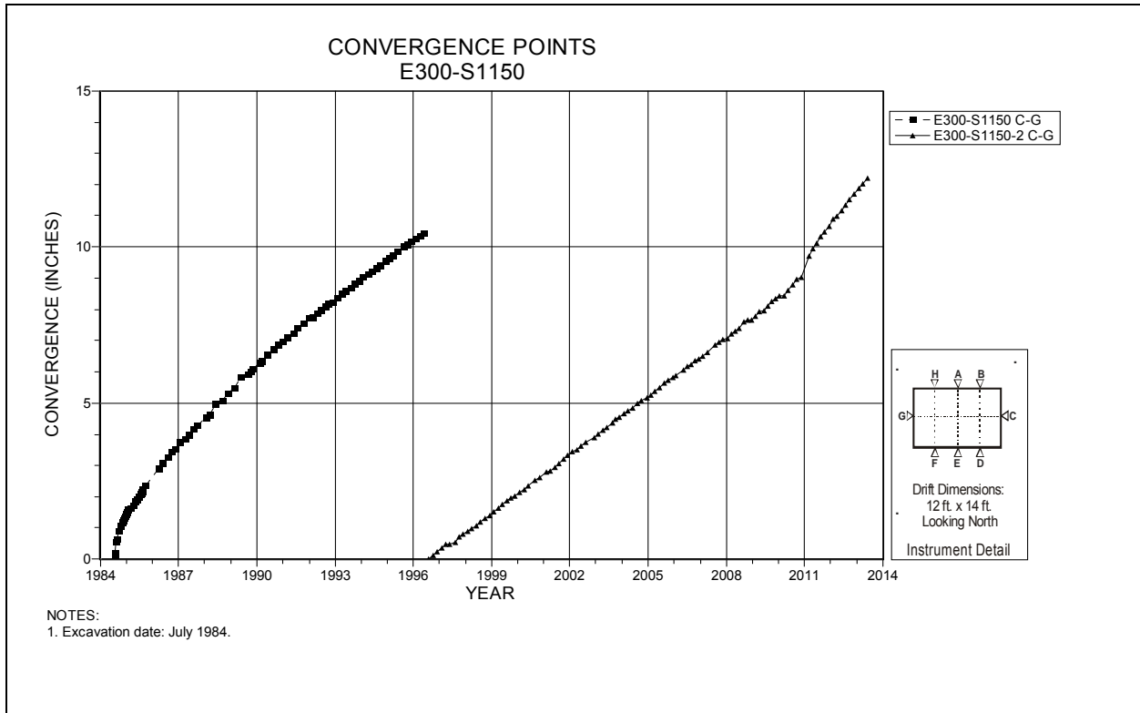
Figure 4-135 Convergence Point Array E300 S1150 – Rib to Rib
