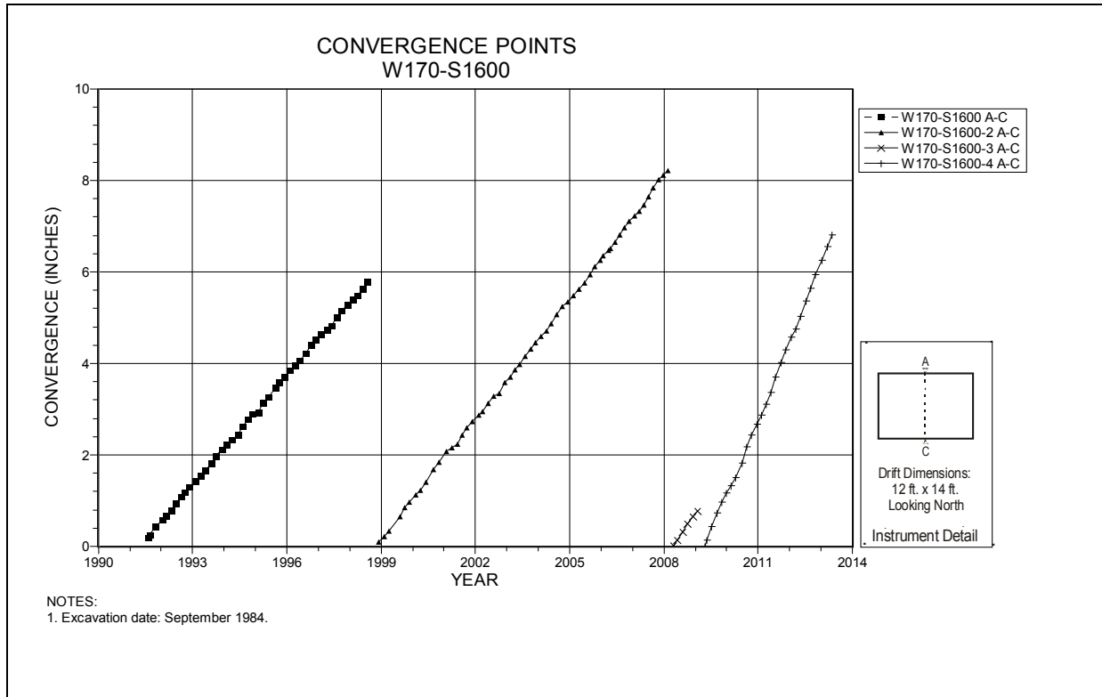
Figure 4-245 Convergence Point Array W170 S1600 – Roof to Floor
