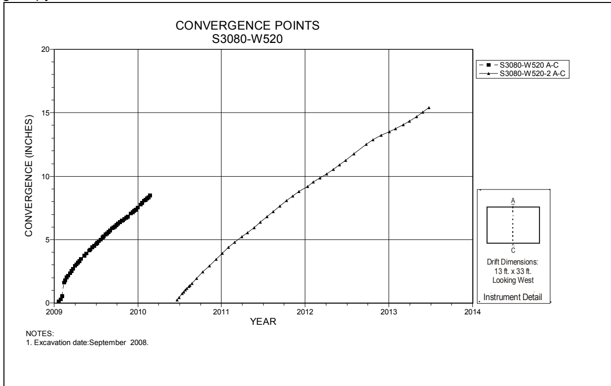
Figure 5-58 Convergence Point Array S3080 W520 Intersection (Room 2, Panel 6) – Roof to Floor
