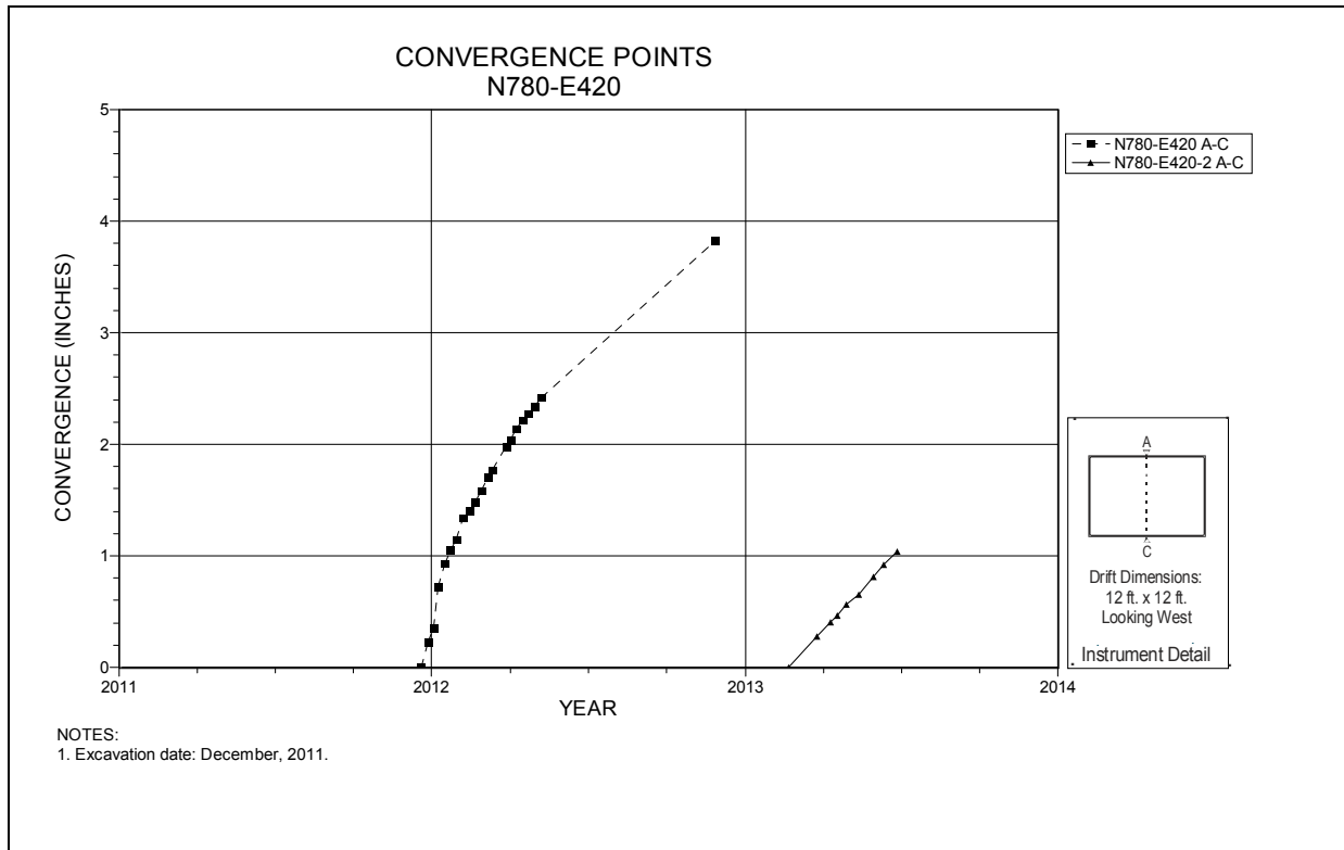
Figure 6-27 Convergence Point Array N780 E420 – Roof to Floor
