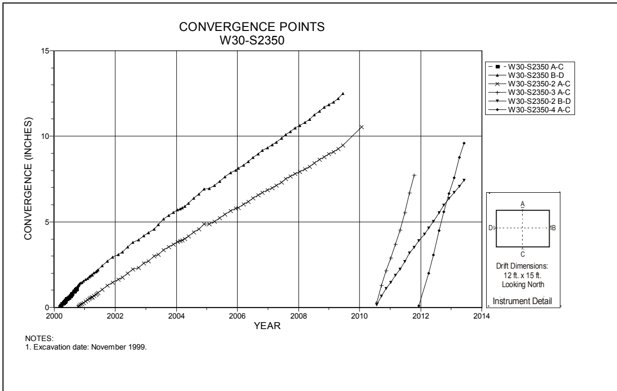
Figure 4-216 Convergence Point Array W30 S2350 – All Chords
