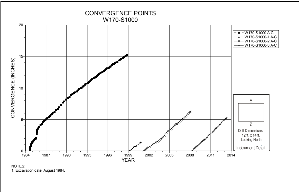
Figure 4-240 Convergence Point Array W170 S1000 – Roof to Floor
