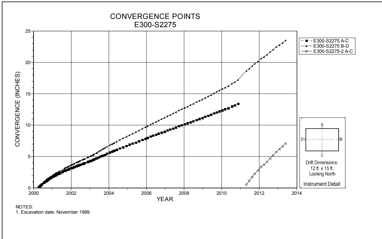
Figure 4-142 Convergence Point Array E300 S2275 – All Chords
