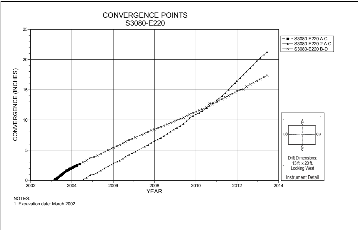
Figure 4-191 Convergence Point Array S3080 E220 – All Chords
