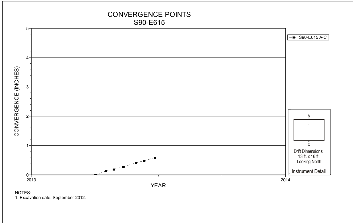
Figure 6-46 Convergence Point Array S90 E615 – Roof to Floor
