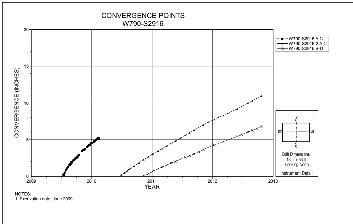
Figure 5-53 Convergence Point Array Room 4, Panel 6 at W790 S2916 – Room Center – All Chords
