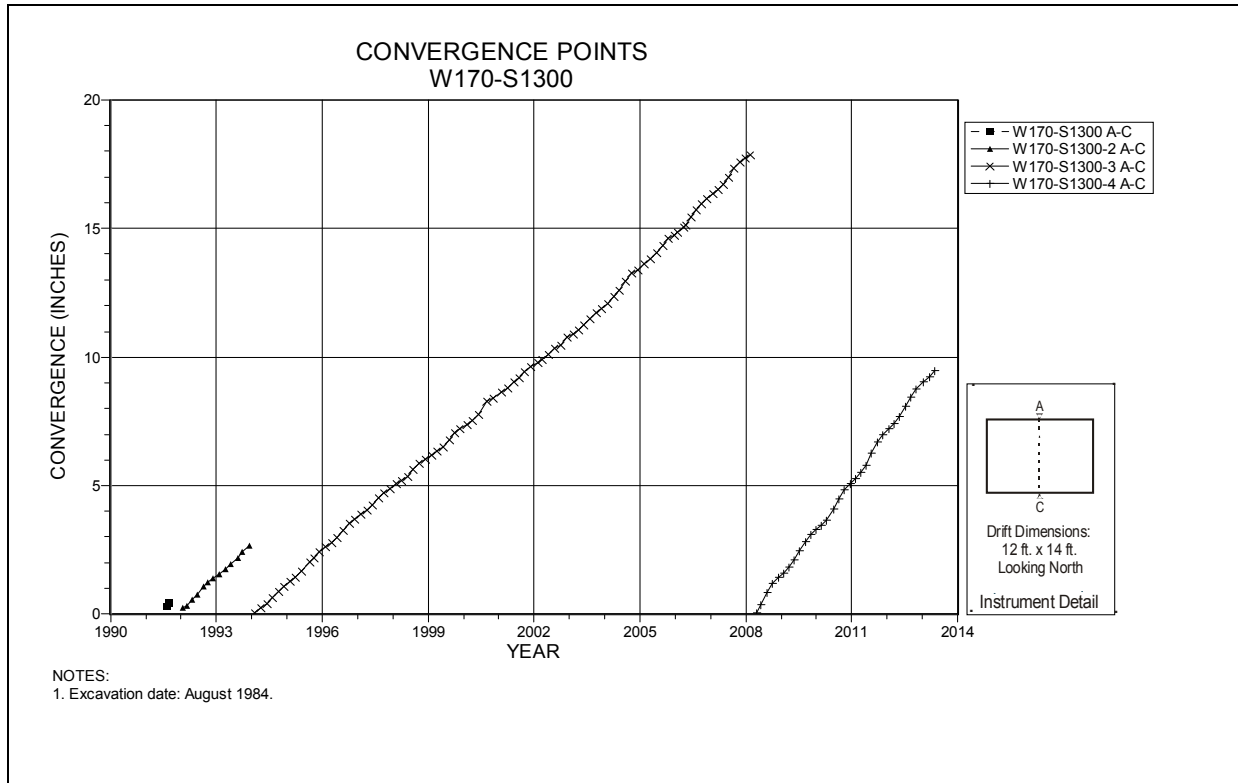
Figure 4-243 Convergence Point Array W170 S1300 – Roof to Floor
