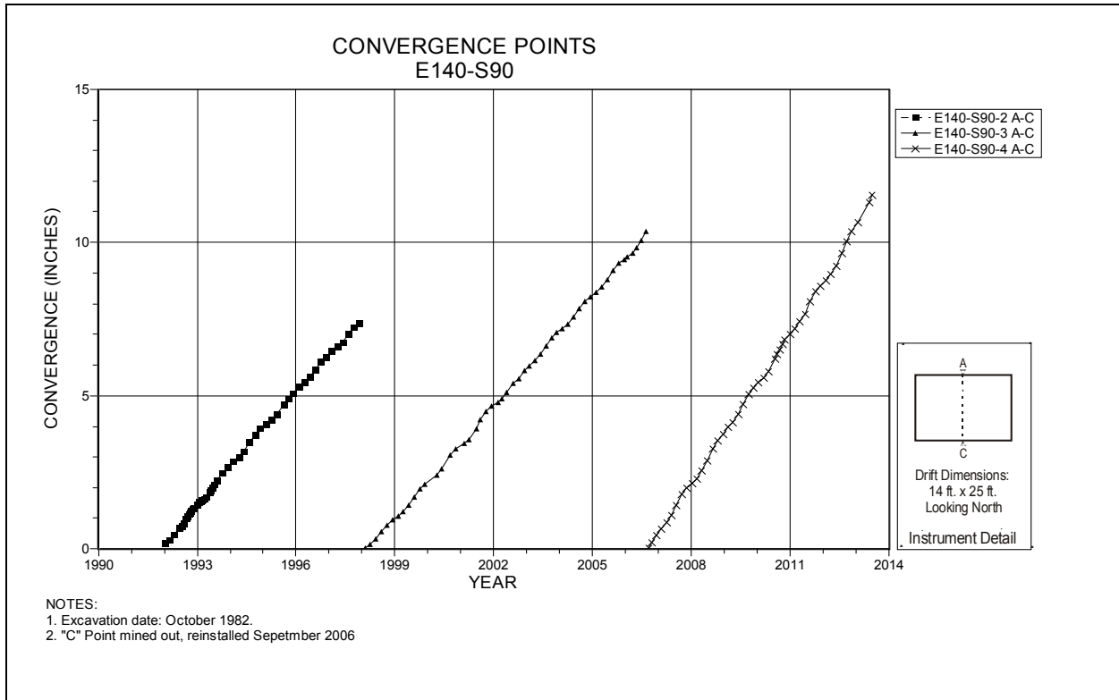
Figure 4-61 Convergence Point Array E140 S90 – Roof to Floor
