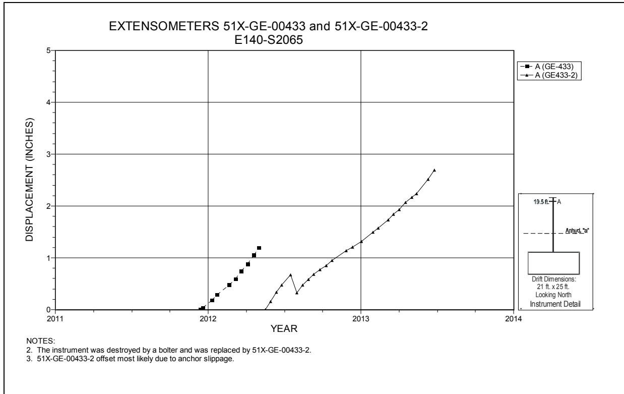
Figure 4-17 Extensometers 51X-GE-00433 and 51X-GE-00433-2 E140 S2065 – Roof
