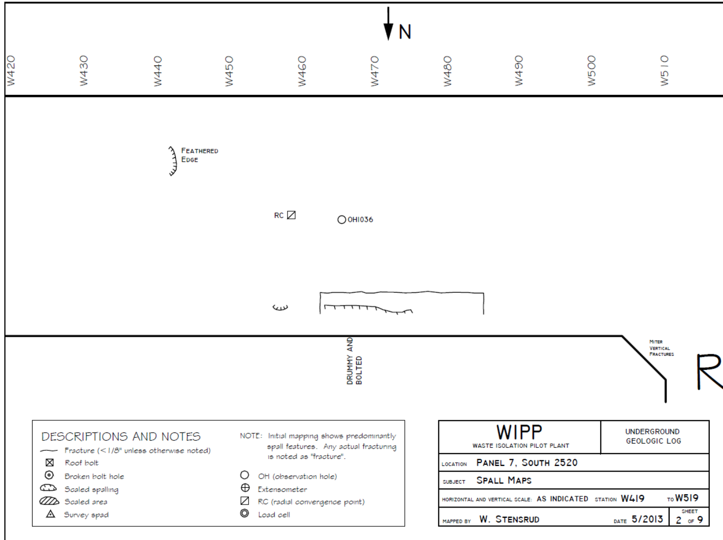
Figure 7-39 Panel 7 South 2520, W419-W519 Roof Fractures
