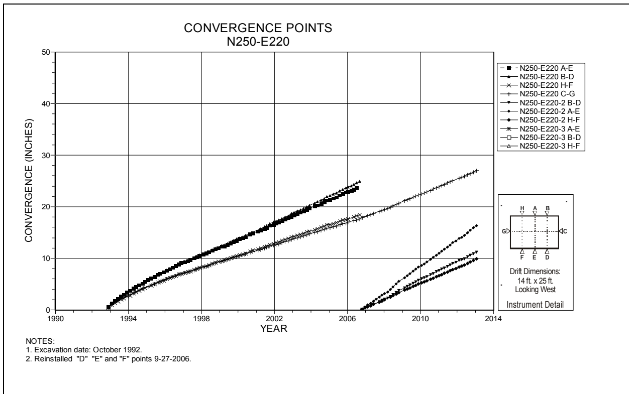
Figure 4-154 Convergence Point Array N250 E220 – All Chords
