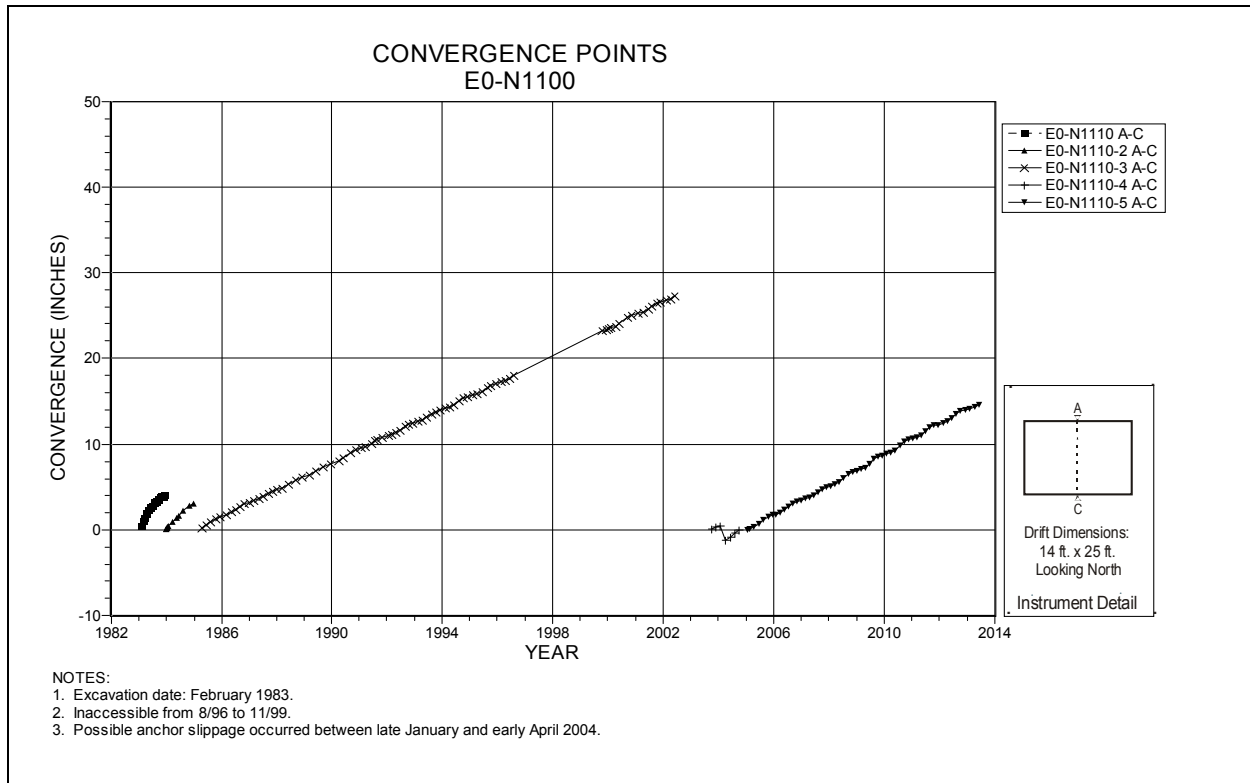
Figure 4-46 Convergence Point Array E0 N1100 – Roof to Floor
