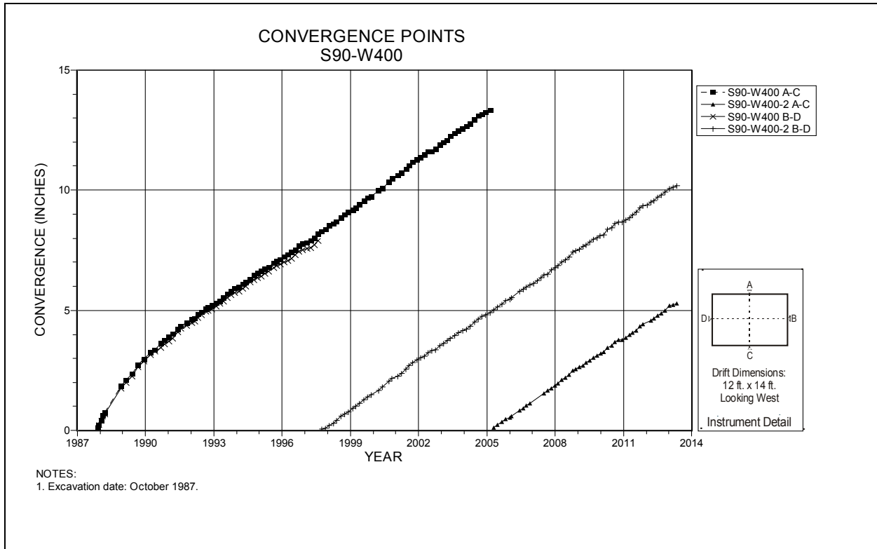
Figure 4-159 Convergence Point Array S90 W400 – All Chords
