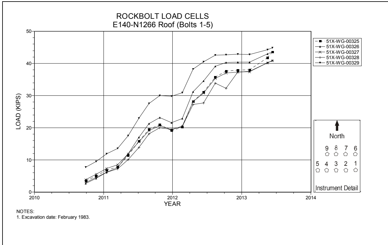
Figure 4-271 Rock Bolt Load Cells, Bolts 1-5 E140 N1266
