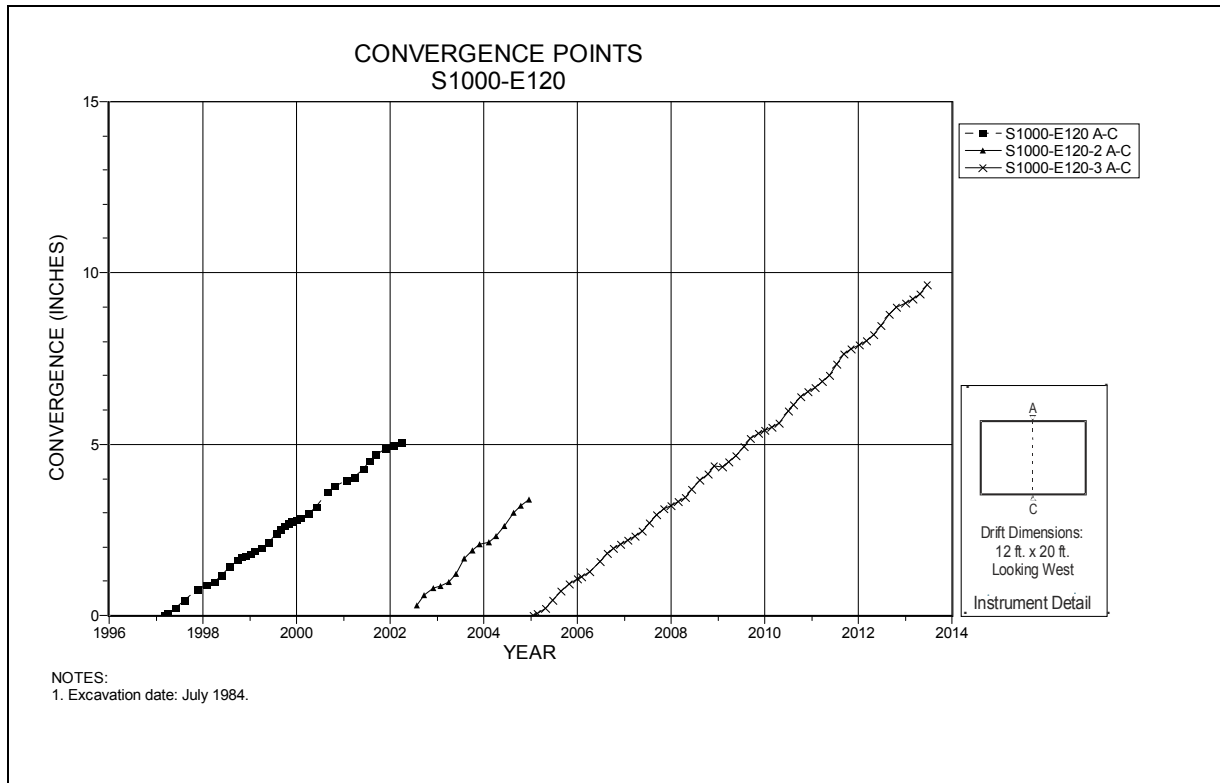
Figure 4-170 Convergence Point Array S1000 E120 – Roof to Floor
