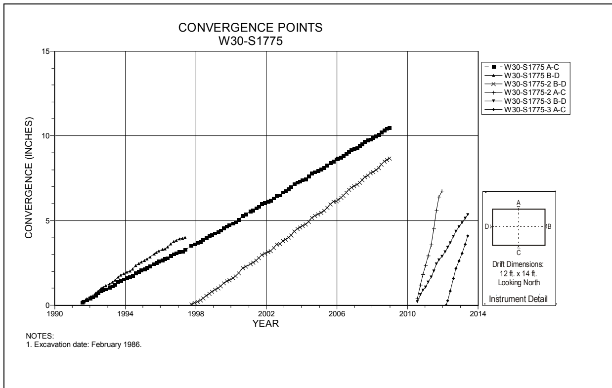
Figure 4-212 Convergence Point Array W30 S1775 – All Chords
