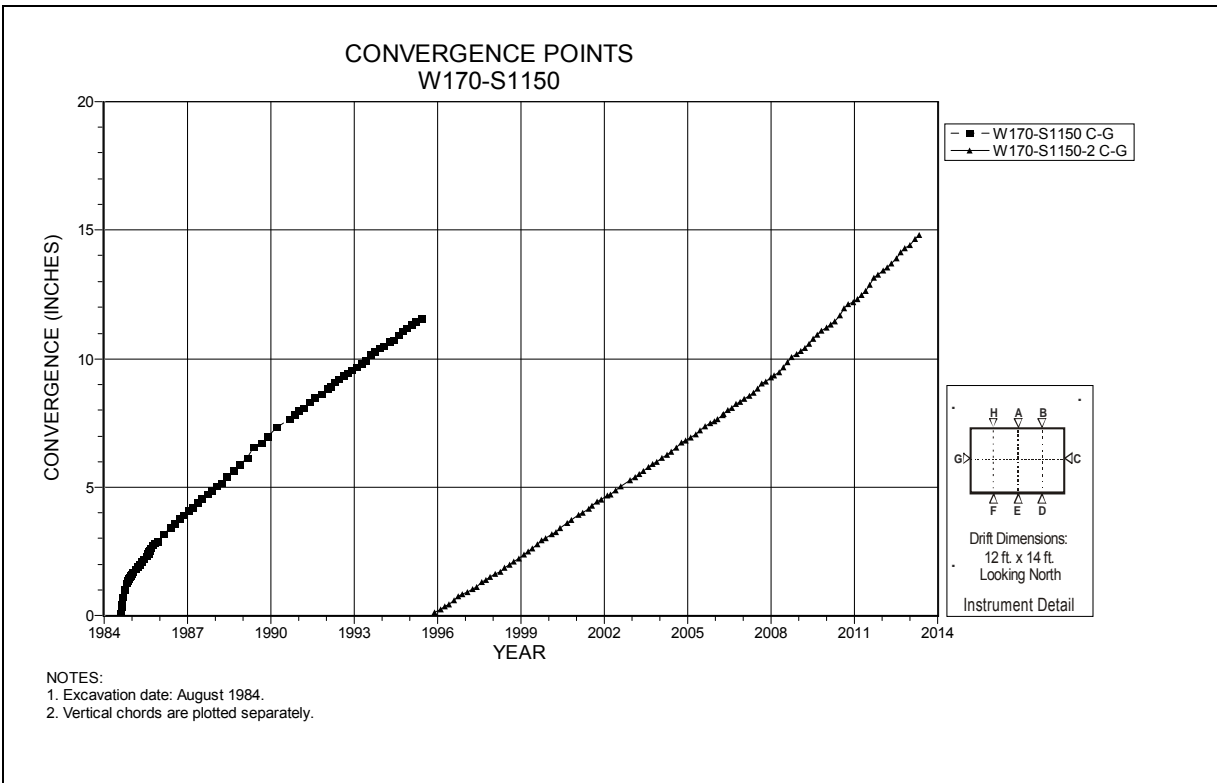
Figure 4-242 Convergence Point Array W170 S1150 – Rib to Rib
