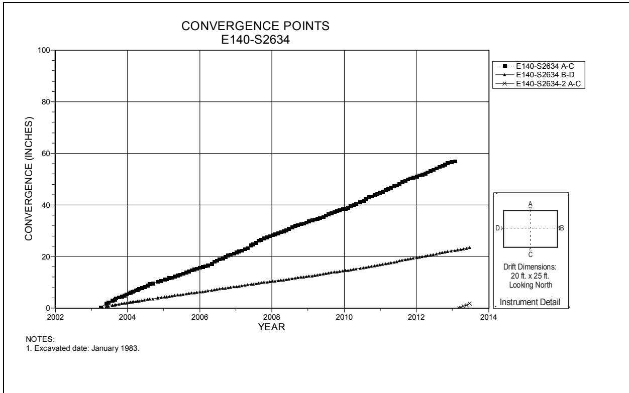
Figure 4-109 Convergence Point Array E140 S2634 – All Chords
