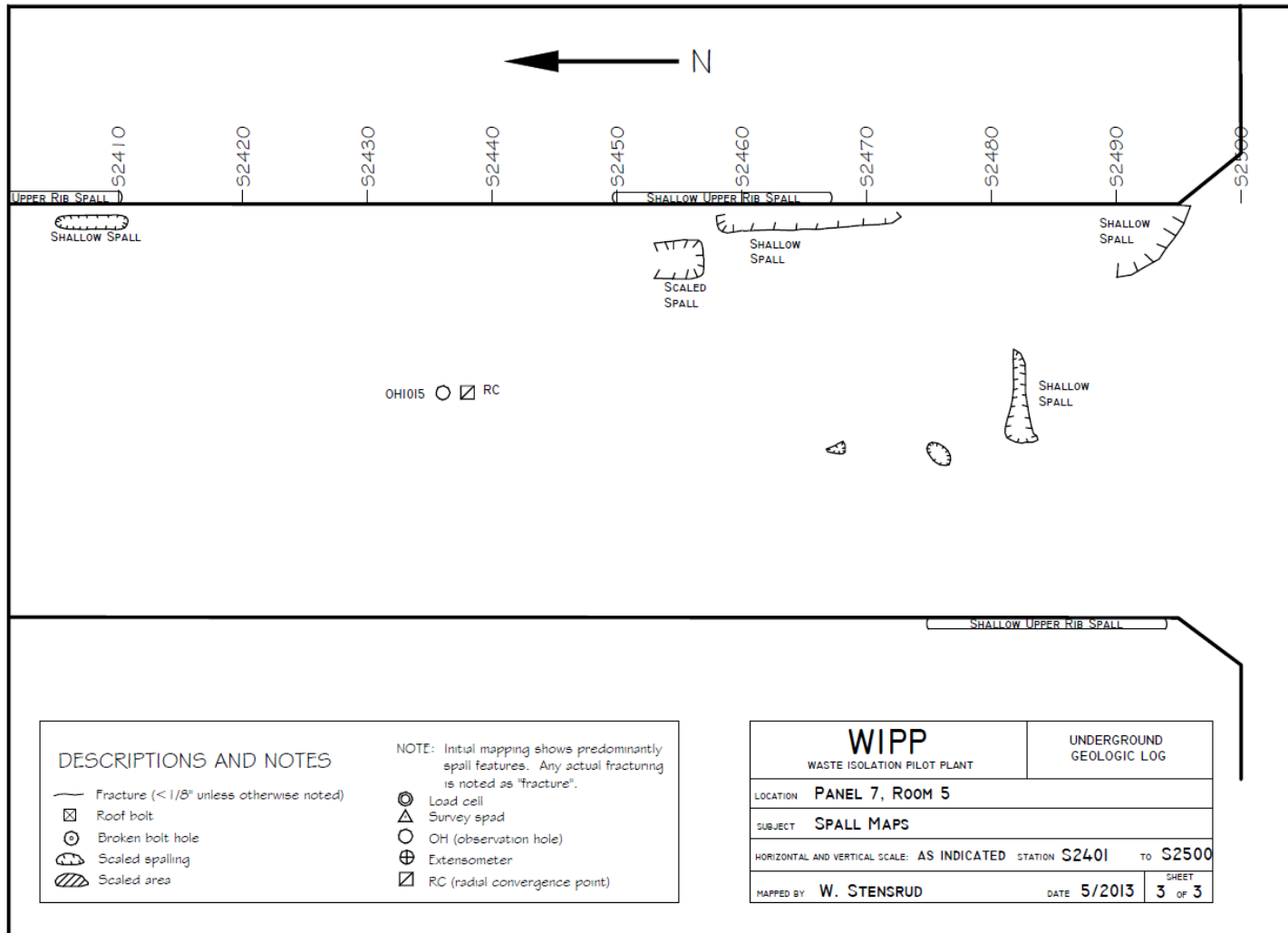
Figure 7-22 Panel 7 Room 5, S2401-S2500 Roof Fractures
