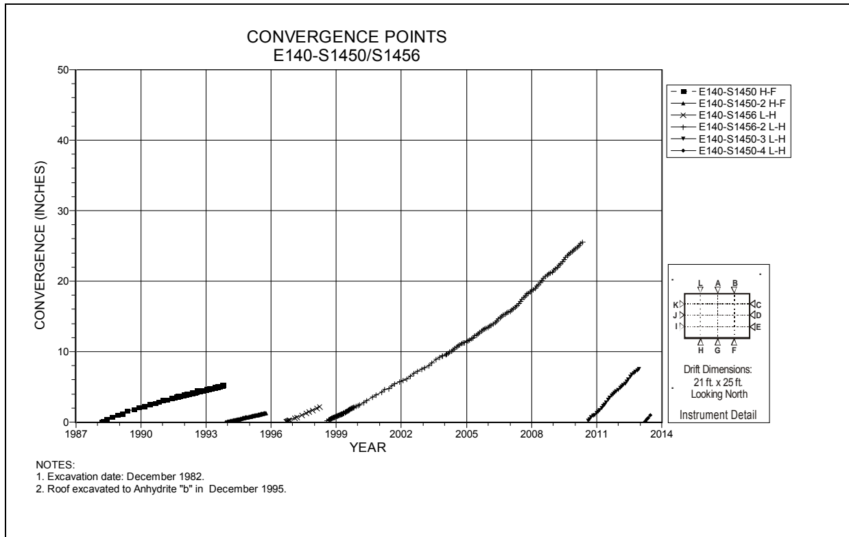
Figure 4-88 Convergence Point Array E140 S1450/S1456 – Roof to Floor – West Quarter Point
