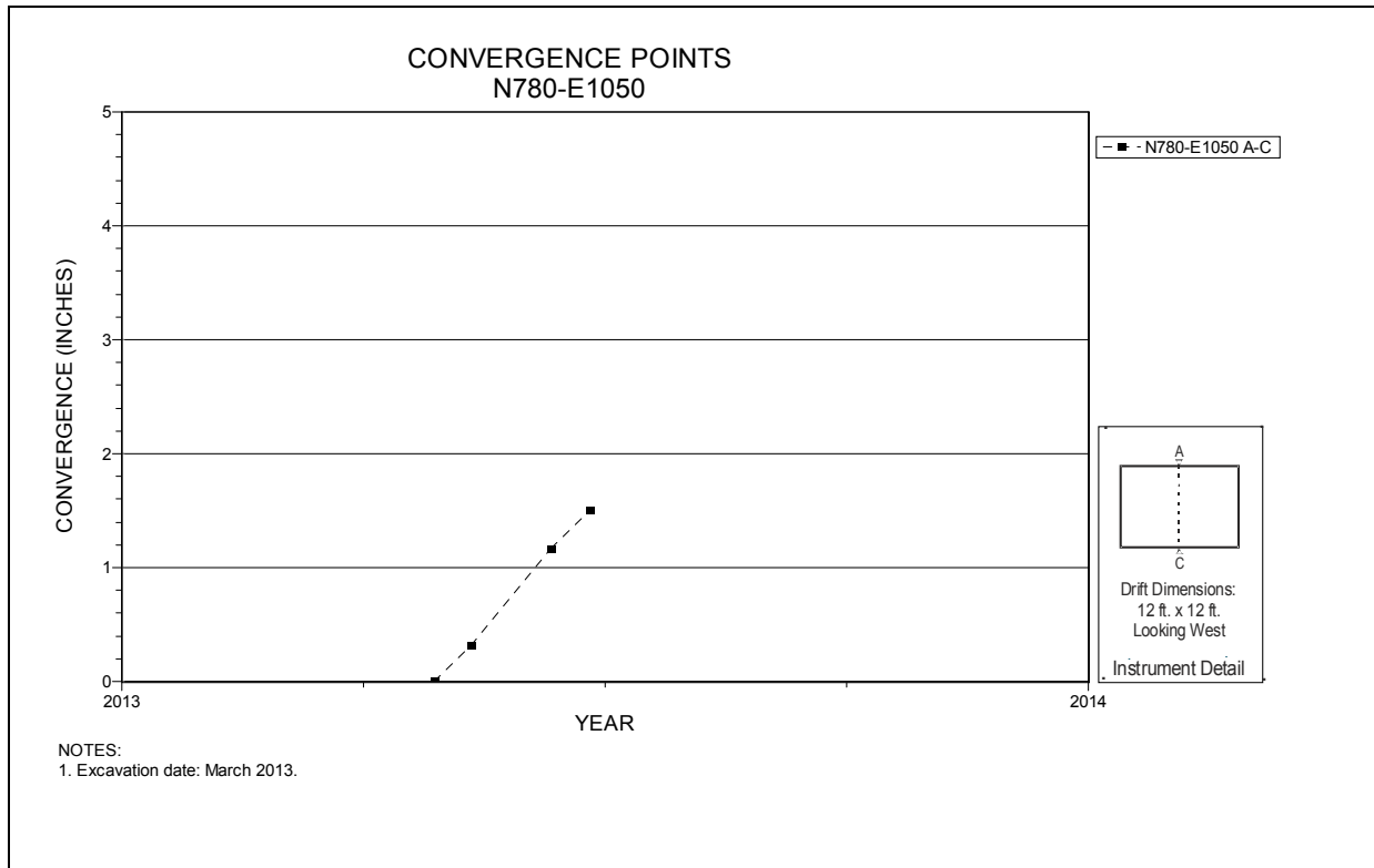
Figure 6-35 Convergence Point Array N780 E1050 – Roof to Floor
