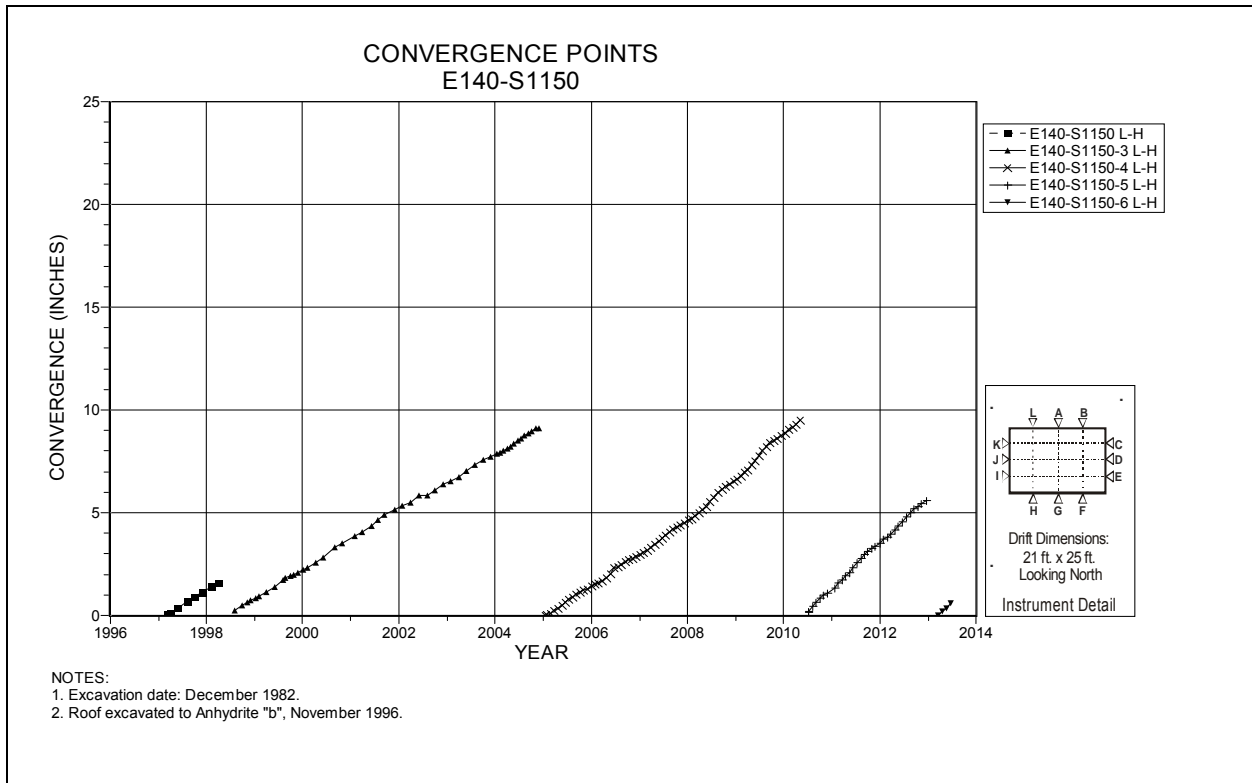
Figure 4-78 Convergence Point Array E140 S1150 – Roof to Floor – West Quarter Point
