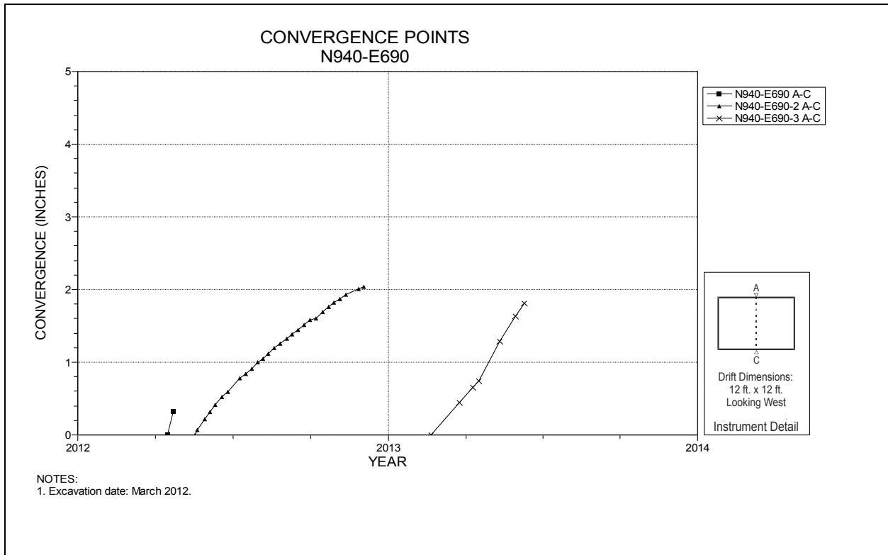
Figure 6-45 Convergence Point Array N940 E690 – Roof to Floor
