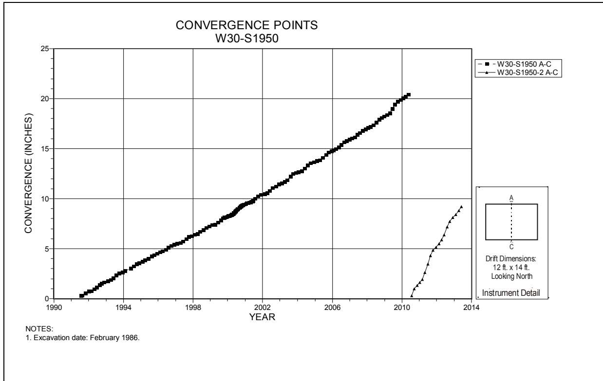
Figure 4-213 Convergence Point Array W30 S1950 – Roof to Floor
