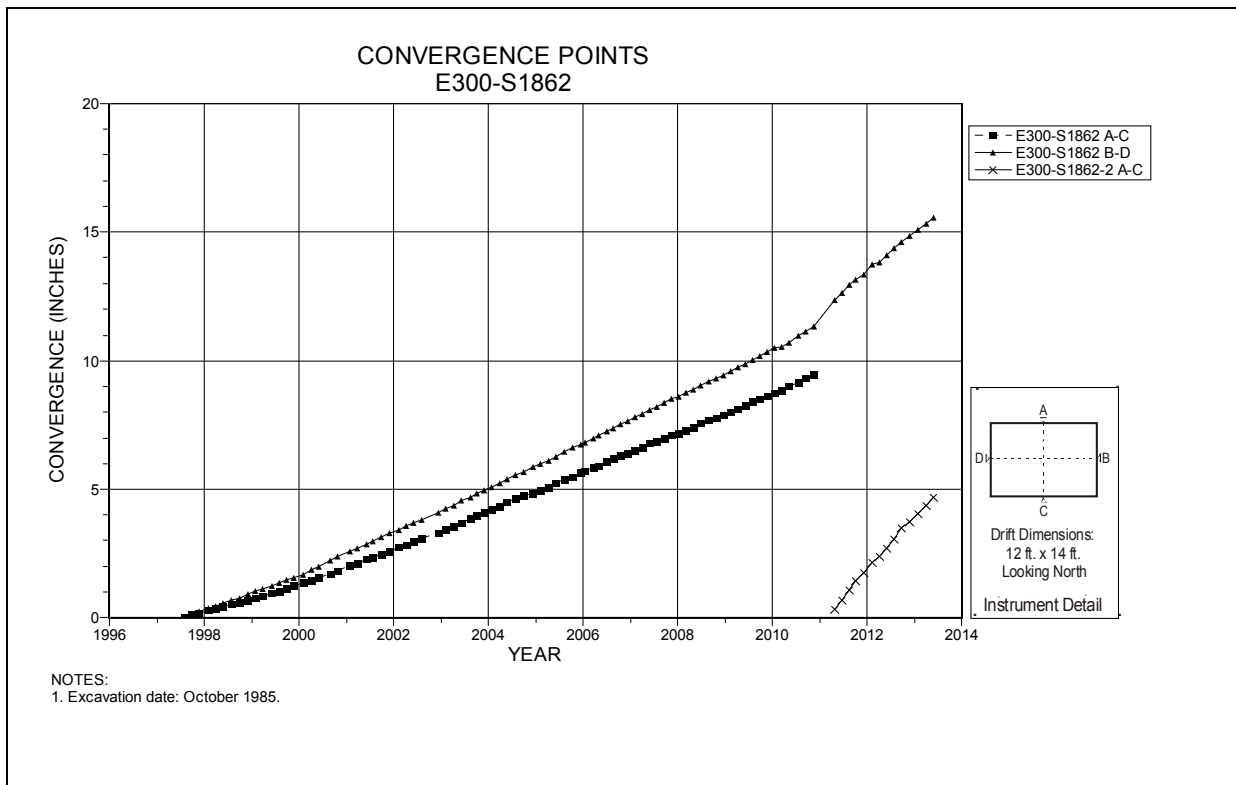
Figure 4-140 Convergence Point Array E300 S1862 – All Chords
