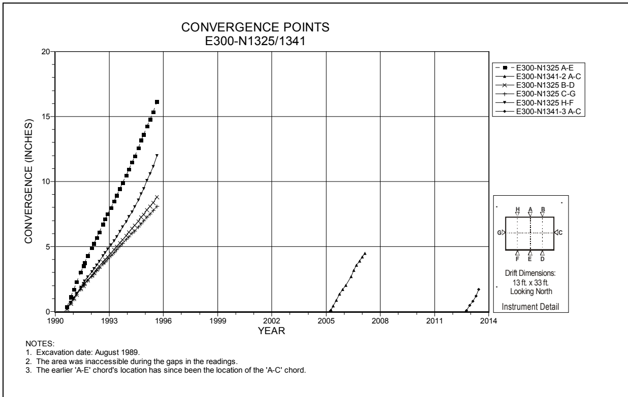
Figure 4-126 Convergence Point Array E300 N1325/N1341 – All Chords
