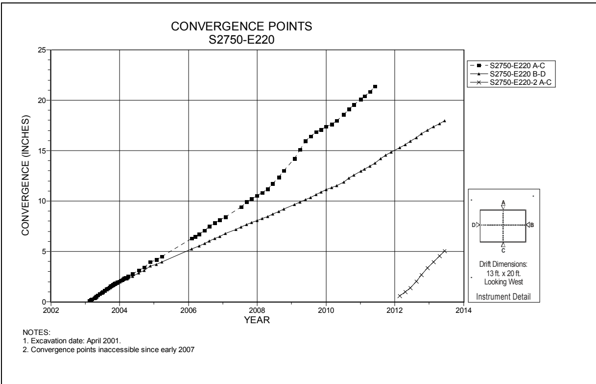
Figure 4-188 Convergence Point Array S2750 E220 – All Chords
