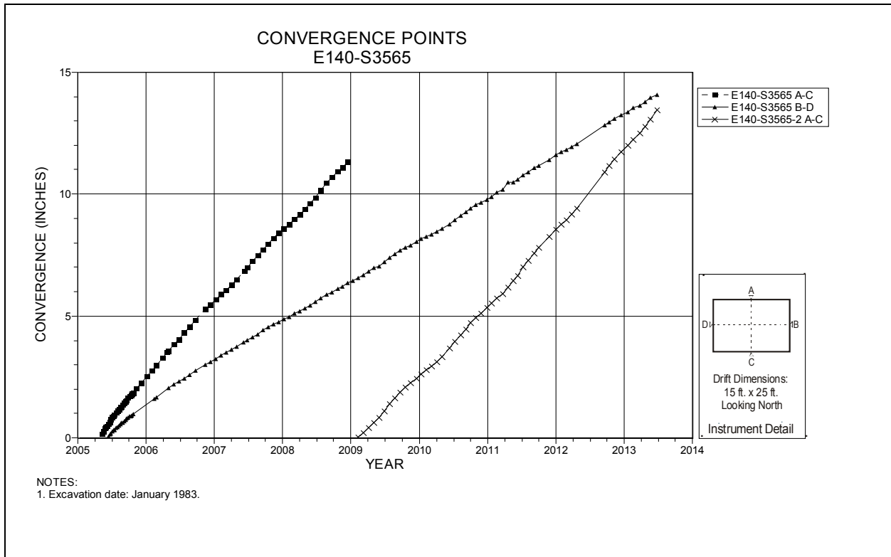
Figure 4-120 Convergence Point Array E140 S3565 – All Chords
