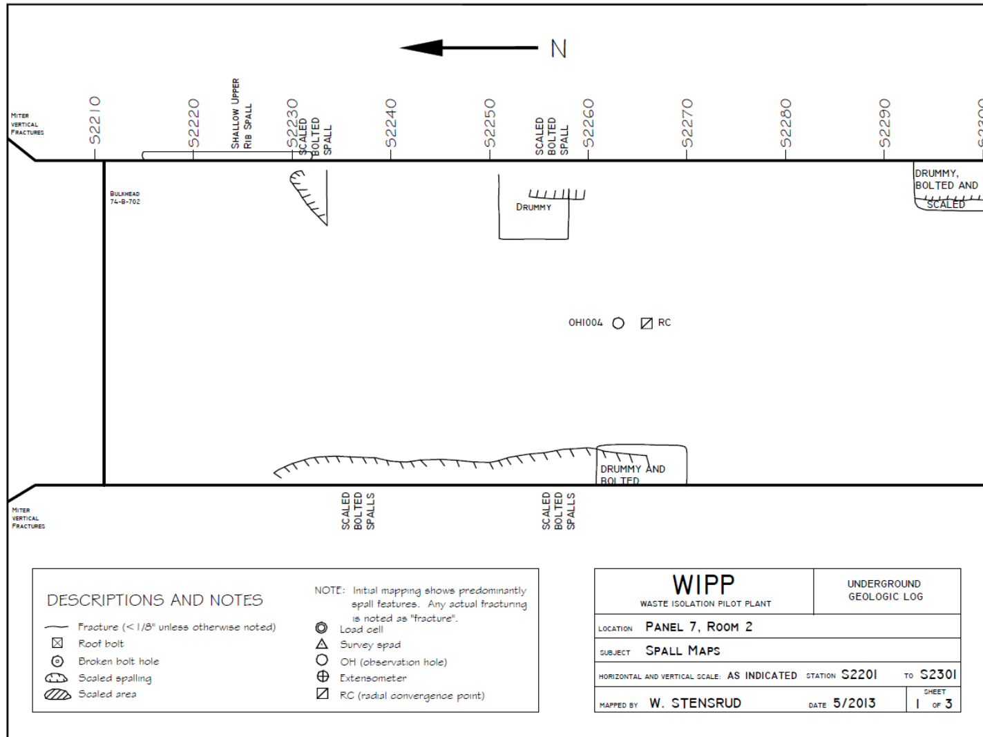
Figure 7-11 Panel 7 Room 2, S2201-S2301 Roof Fractures
