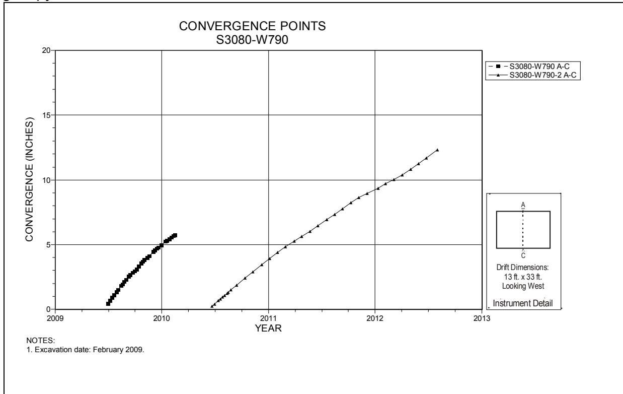
Figure 5-62 Convergence Point Array S3080 W790 Intersection (Room 4, Panel 6) – Roof to Floor
