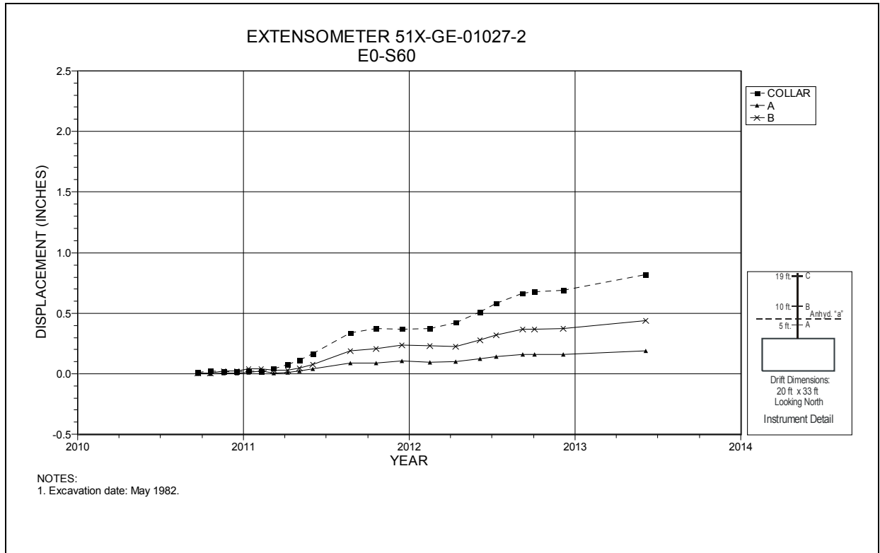
Figure 3-6 Extensometer 51X-GE-001027-2 Salt Handling Shaft Station at S60 – Roof
