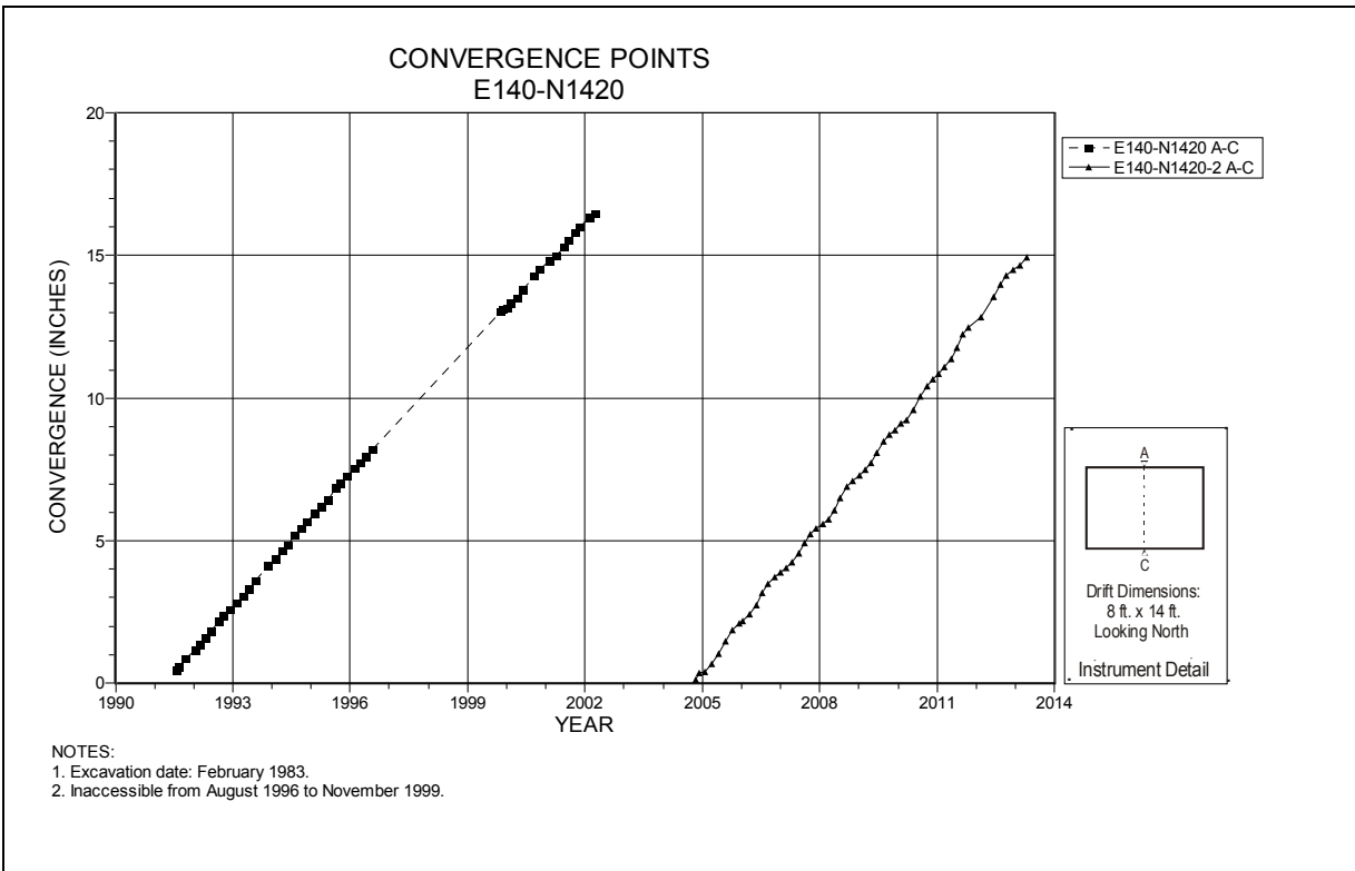
Figure 4-60 Convergence Point Array E140 N1420 – Roof to Floor
