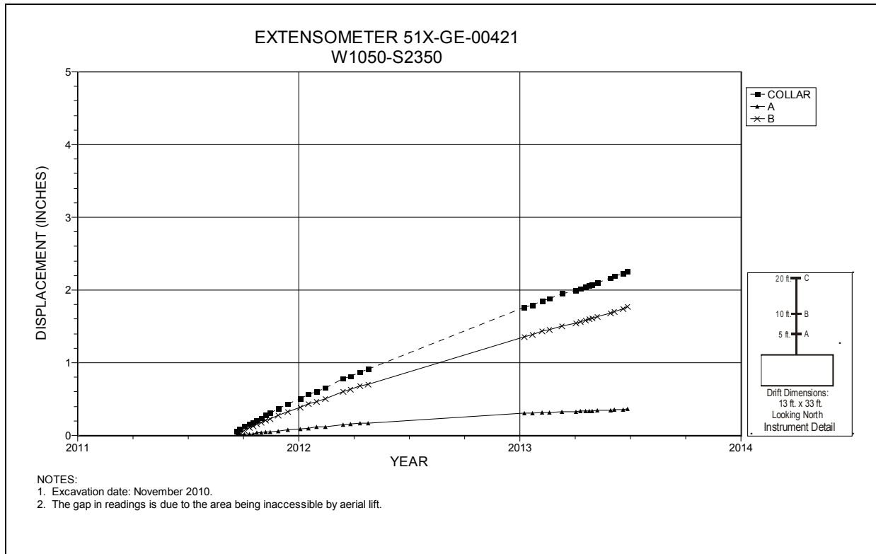
Figure 5-70 Extensometer 51X-GE-00421 Room 6, Panel 7 at W1050 S2350 – Room Center – Roof
