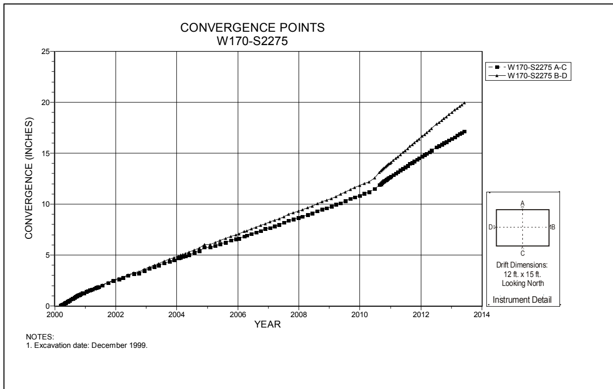
Figure 4-250 Convergence Point Array W170 S2275 – All Chords
