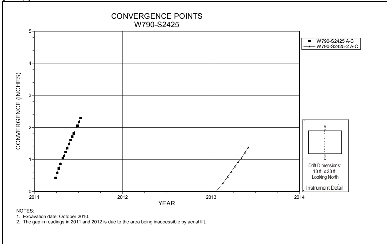
Figure 5-99 Convergence Point Array Room 4, Panel 7 at W790 S2425 – Roof to Floor
