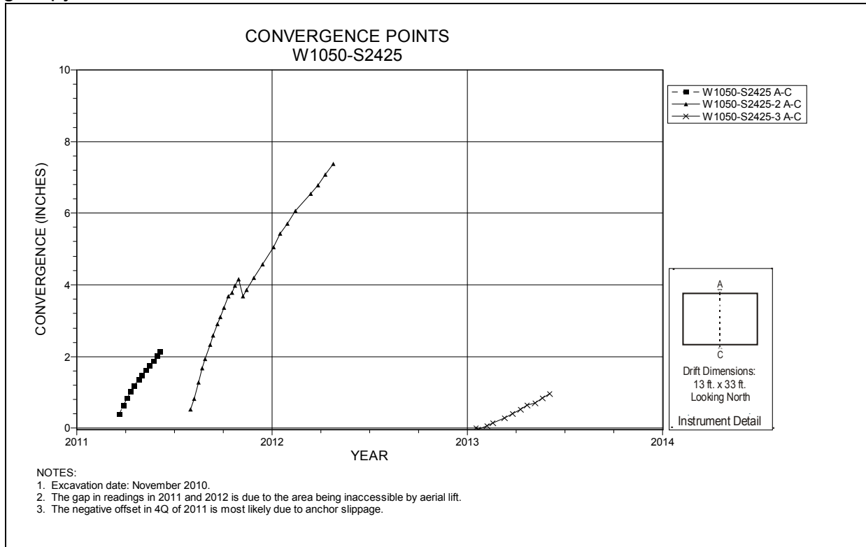
Figure 5-105 Convergence Point Array Room 6, Panel 7 at W1050 S2425 – Roof to Floor
