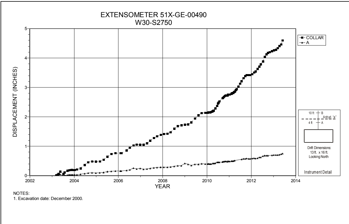
Figure 4-35 Extensometer 51X-GE-00490 W30 S2750 – Roof
