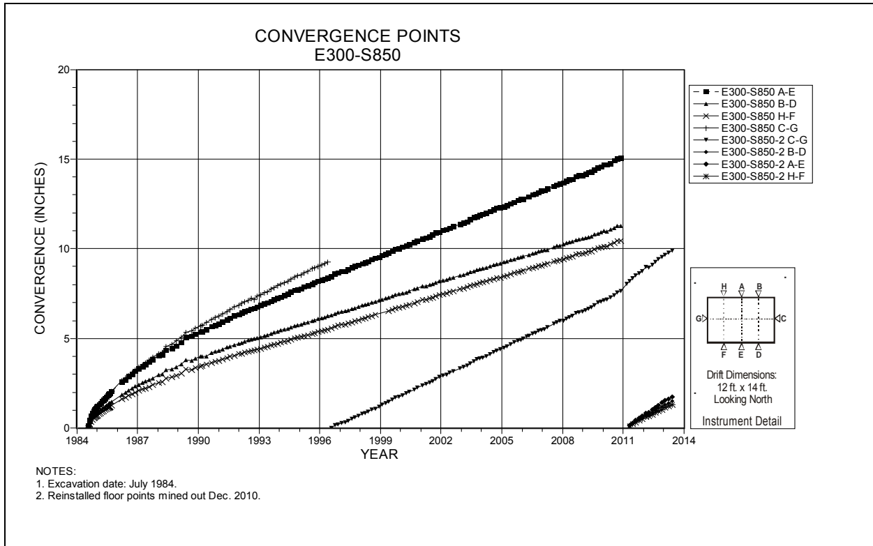
Figure 4-131 Convergence Point Array E300 S850 – All Chords
