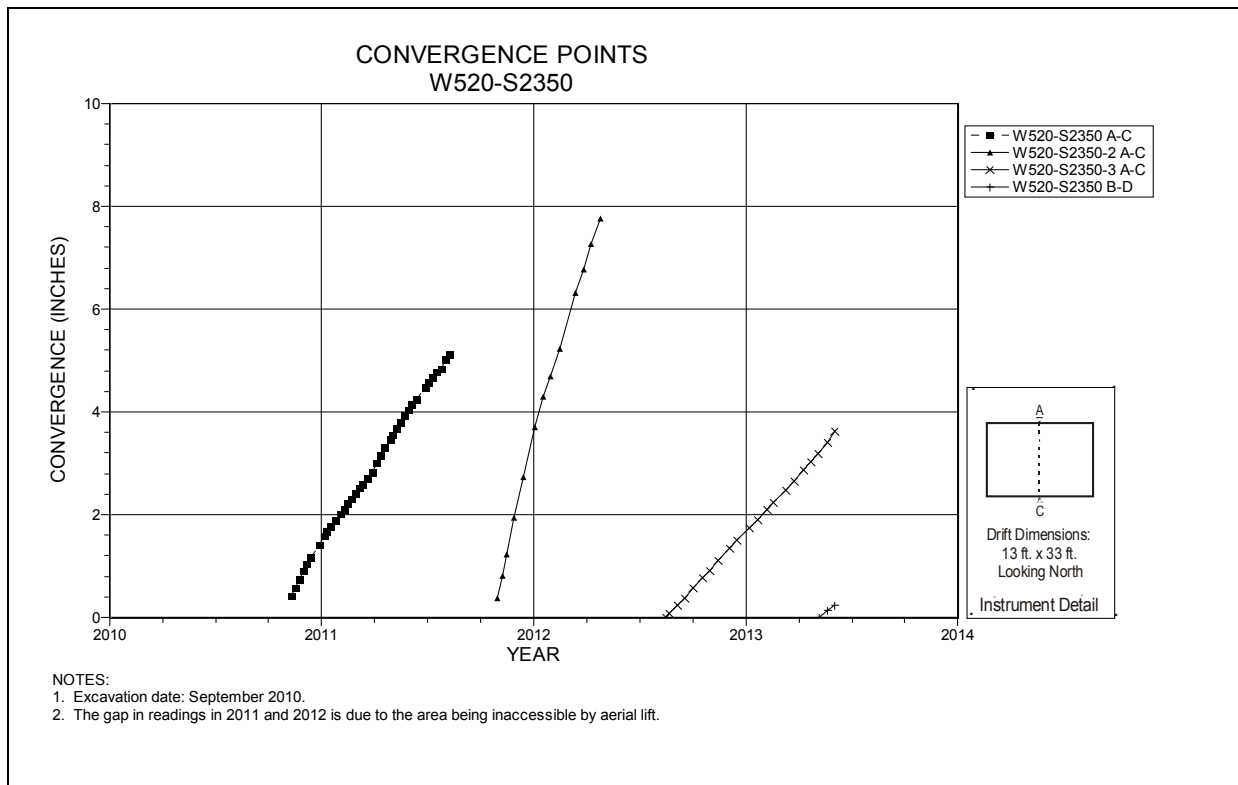
Figure 5-92 Convergence Point Array Room 2, Panel 7 at W520 S2350 – Room Center – All Chords
