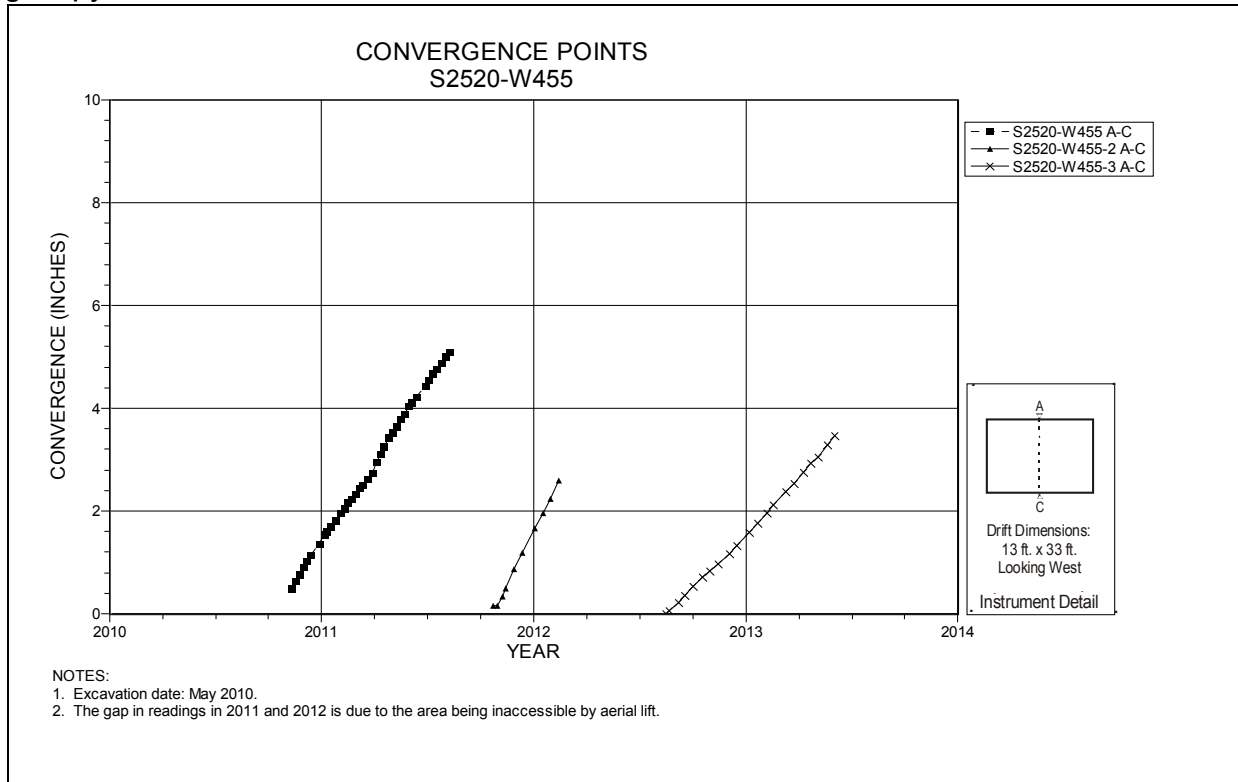
Figure 5-111 Convergence Point Array S2520 W455 – Roof to Floor
