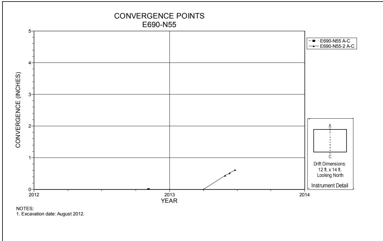
Figure 6-16 Convergence Point Array E690 N55 – Roof to Floor
