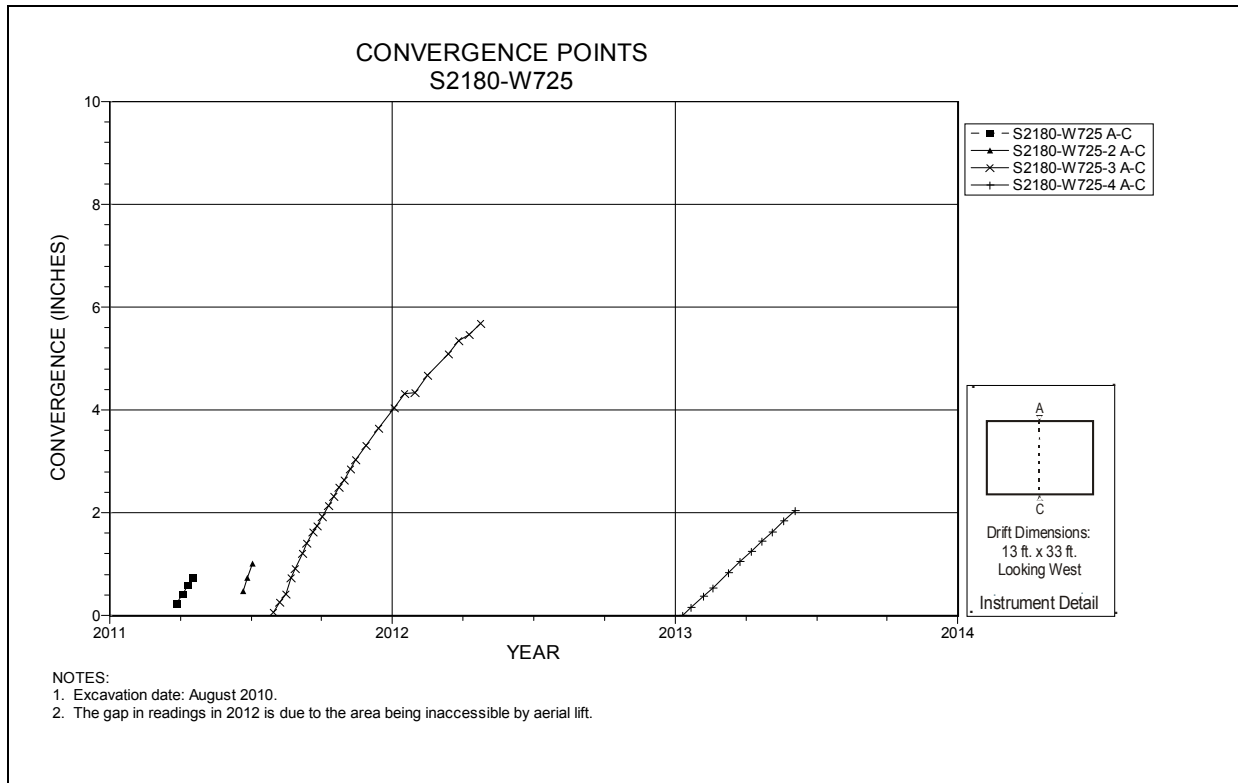
Figure 5-80 Convergence Point Array S2180 W725 – Roof to Floor
