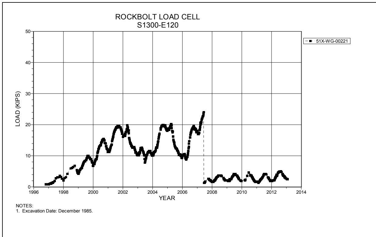
Figure 4-278 Rock Bolt Load Cell S1300 E120
