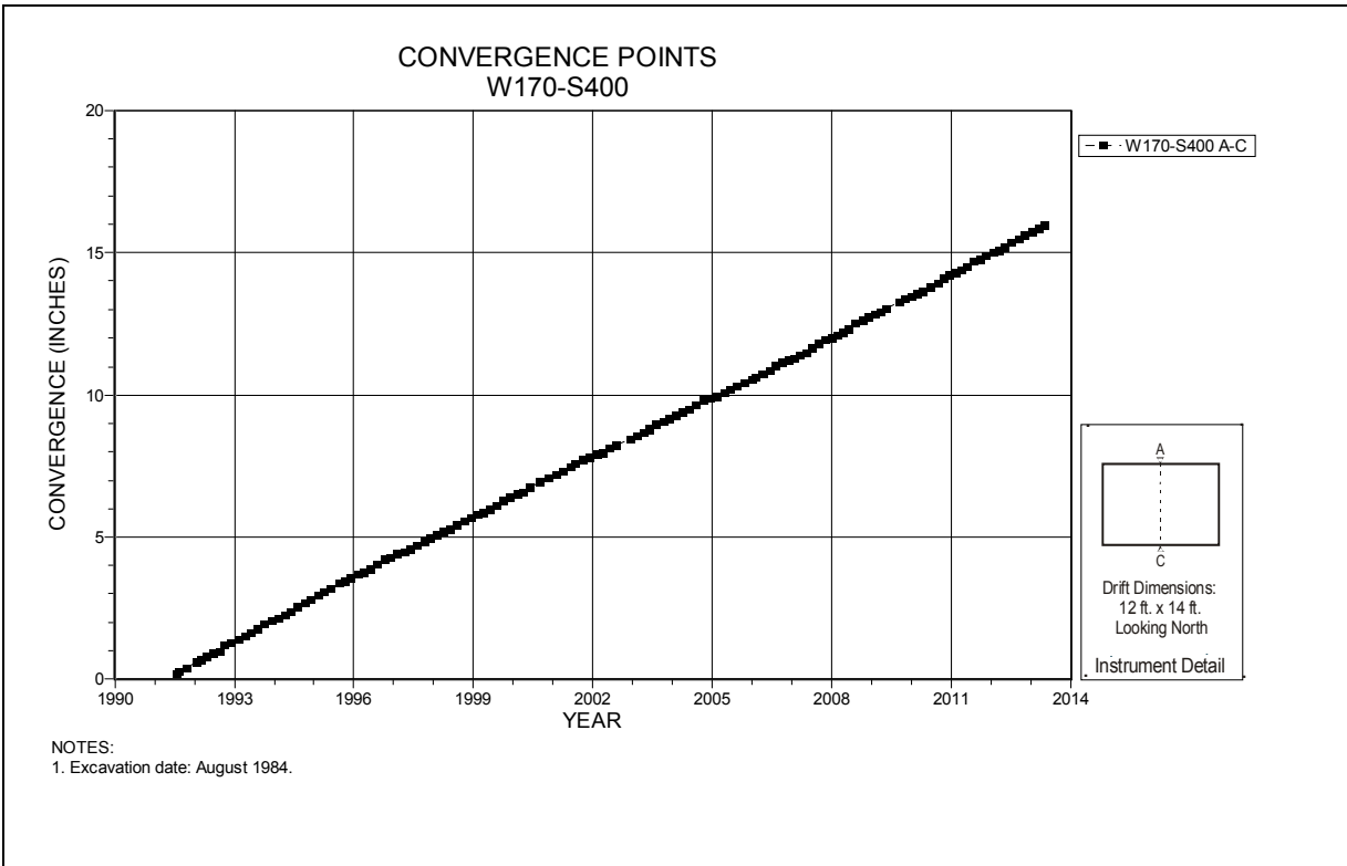
Figure 4-233 Convergence Point Array W170 S400 – Roof to Floor
