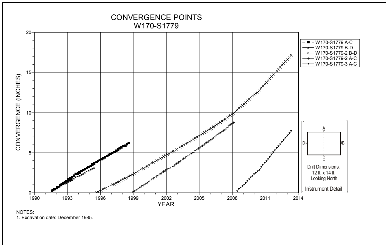
Figure 4-246 Convergence Point Array W170 S1779 – All Chords
