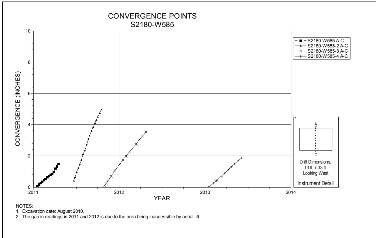
Figure 5-78 Convergence Point Array S2180 W585 – Roof to Floor
