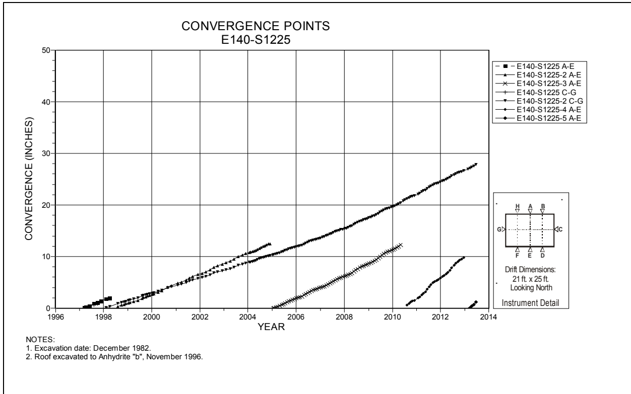
Figure 4-79 Convergence Point Array E140 S1225 – Roof to Floor – Centerline and Rib to Rib
