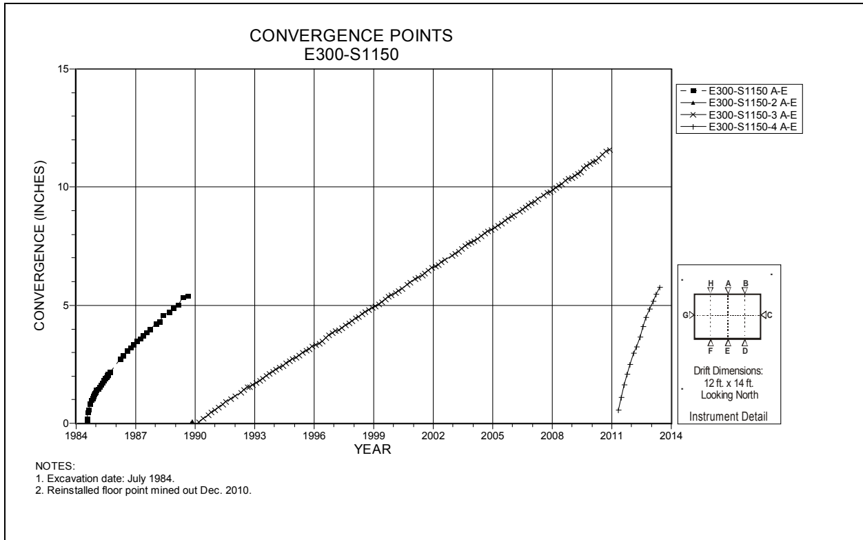
Figure 4-133 Convergence Point Array E300 S1150 – Roof to Floor
