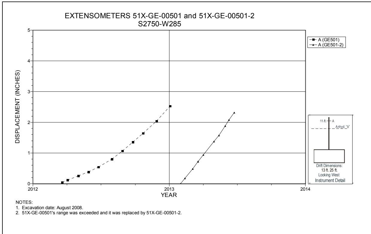
Figure 5-22 Extensometers 51X-GE-00501 and 51X-GE-00501-2 S2750 W285 – Roof
