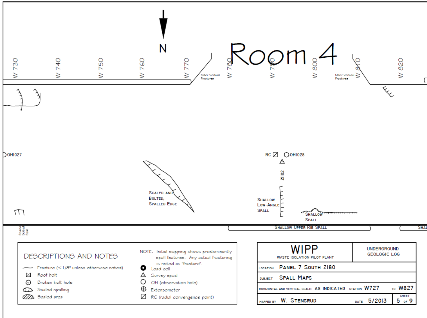
Figure 7-33 Panel 7 South 2180, W727-W827 Roof Fractures
