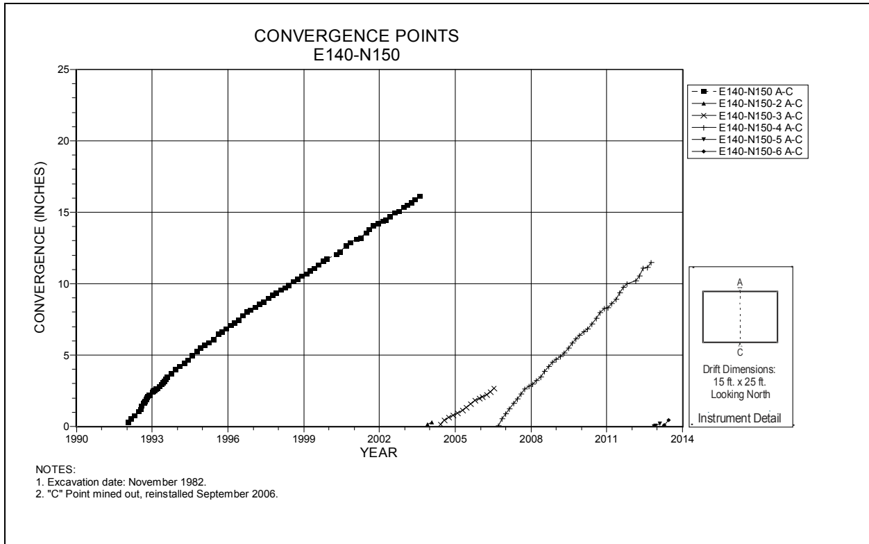
Figure 4-49 Convergence Point Array E140 N150 – Roof to Floor
