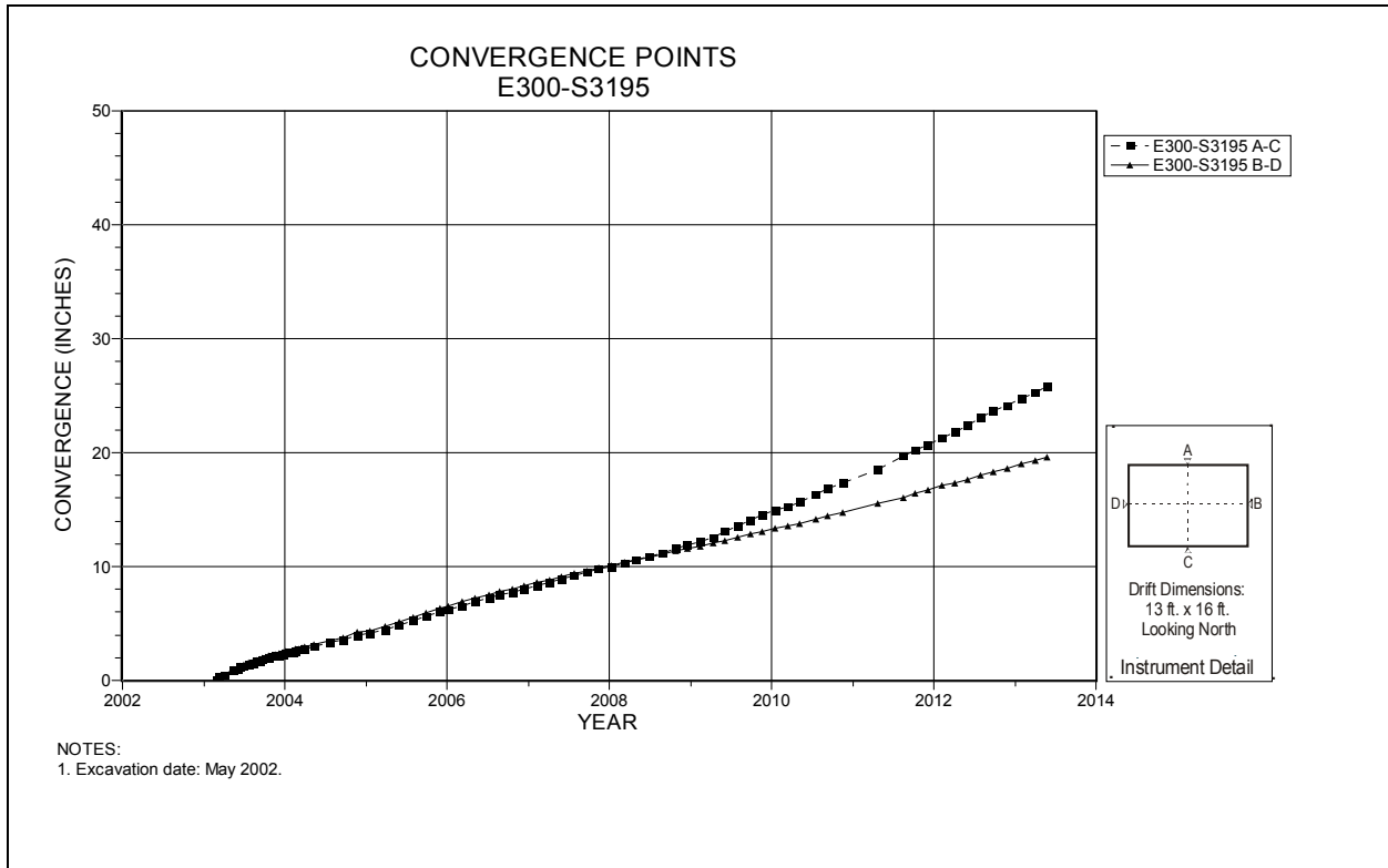
Figure 4-149 Convergence Point Array E300 S3195 – All Chords
