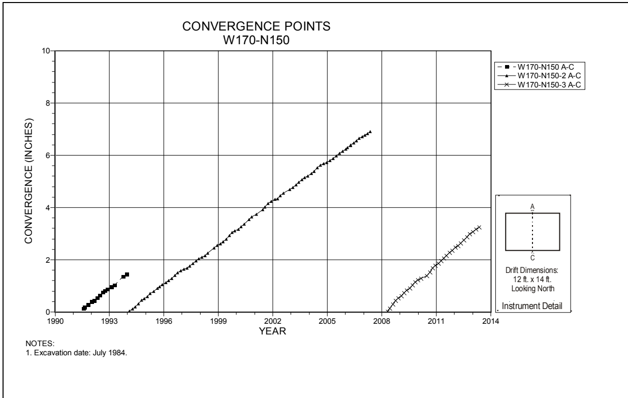
Figure 4-229 Convergence Point Array W170 N150 – Roof to Floor
