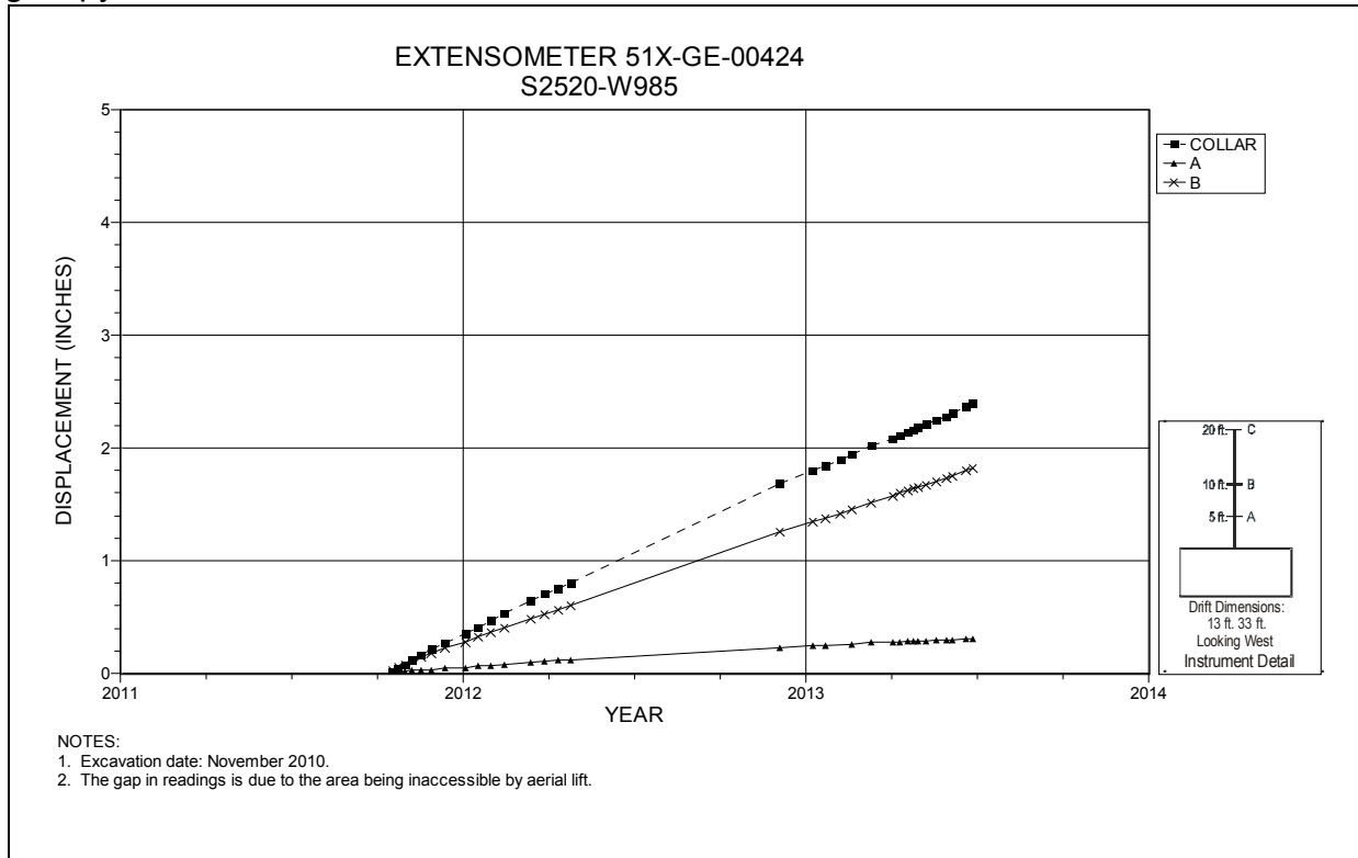
Figure 5-73 Extensometer 51X-GE-00424 S2520 W985 – Roof
