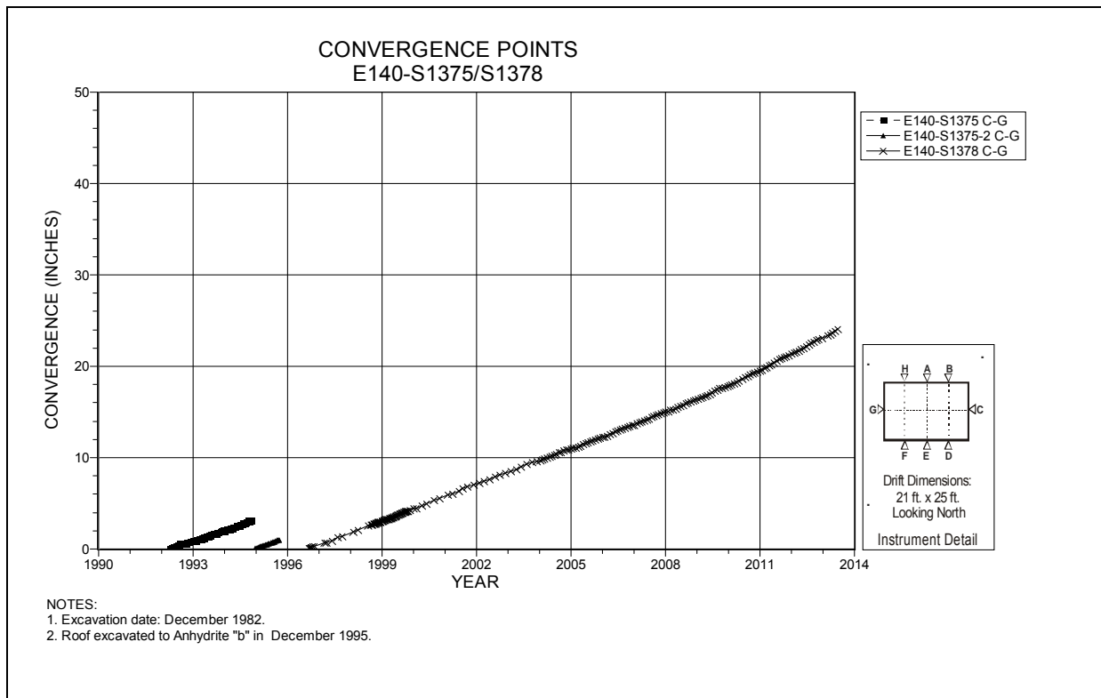
Figure 4-84 Convergence Point Array E140 S1375/S1378 – Rib to Rib
