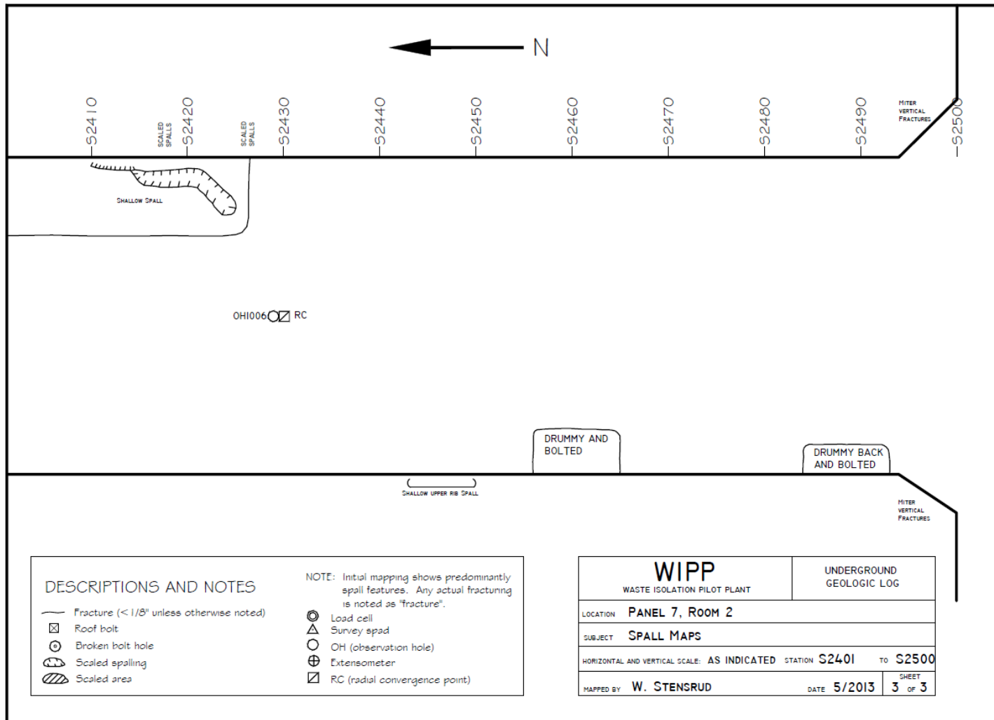
Figure 7-13 Panel 7 Room 2, S2401-S2500 Roof Fractures
