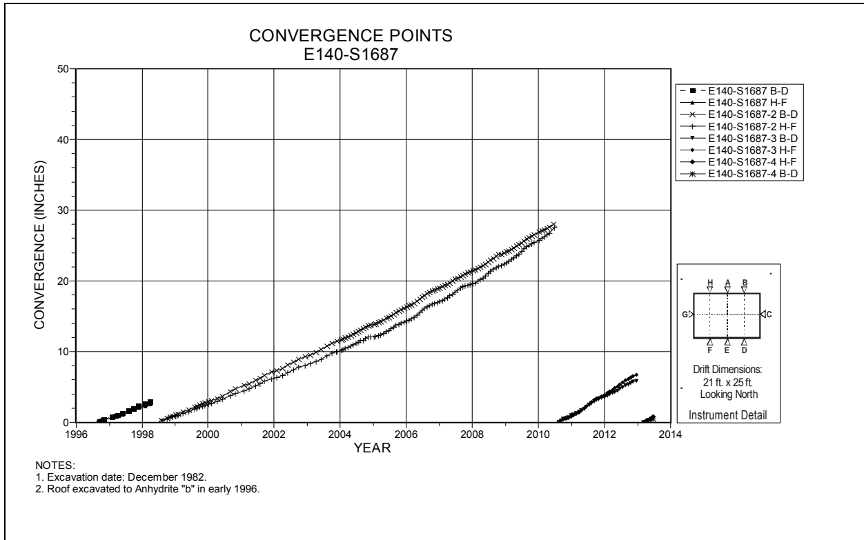
Figure 4-95 Convergence Point Array E140 S1687 – Roof to Floor – Quarter Points
