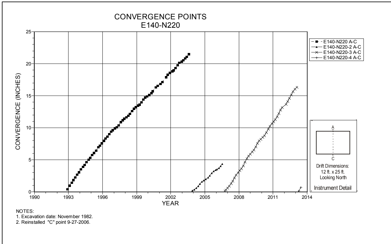
Figure 4-50 Convergence Point Array E140 N220 – Roof to Floor
