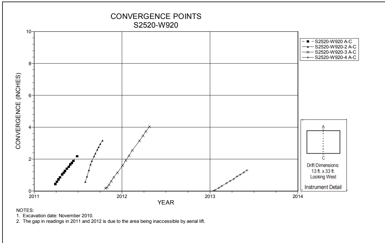
Figure 5-118 Convergence Point Array S2520 W920 Intersection (Room 5, Panel 7) – Roof to Floor
