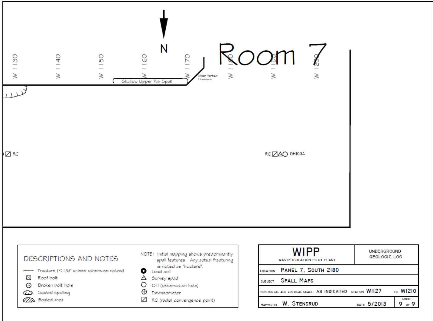
Figure 7-37 Panel 7 South 2180, W1127-W1210 Roof Fractures
