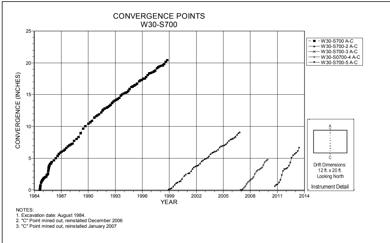
Figure 4-203 Convergence Point Array W30 S700 – Roof to Floor
