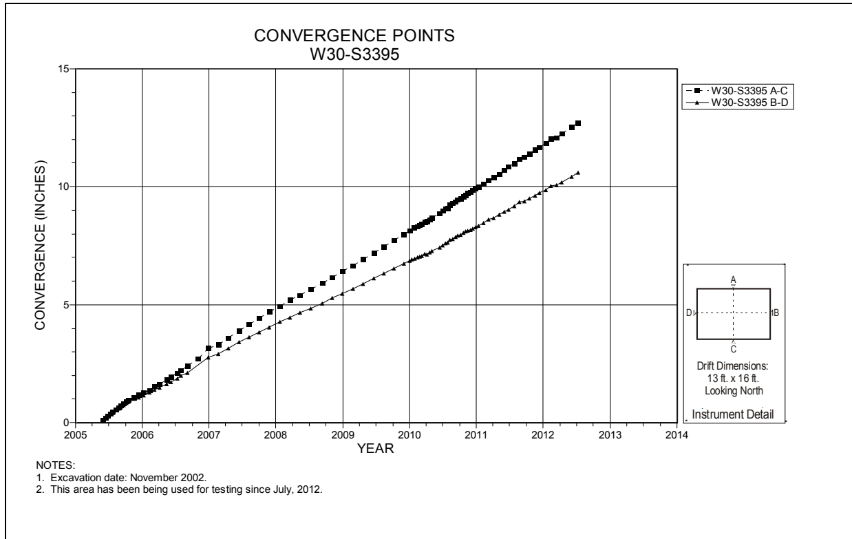
Figure 4-227 Convergence Point Array W30 S3395 – All Chords
