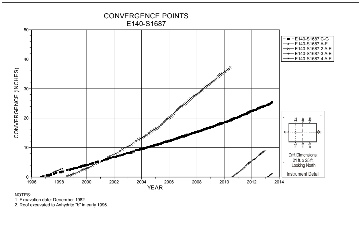
Figure 4-94 Convergence Point Array E140 S1687 – Roof to Floor – Centerline and Rib to Rib
