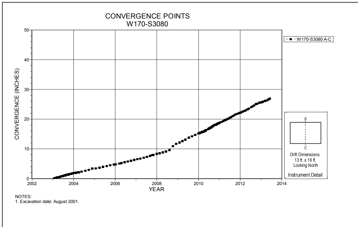
Figure 4-258 Convergence Point Array W170 S3080 – Roof to Floor
