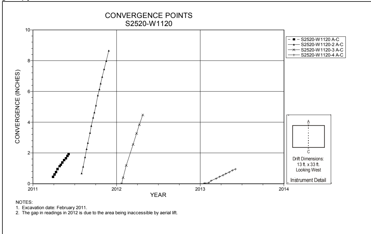
Figure 5-121 Convergence Point Array S2520 W1120 – Roof to Floor
