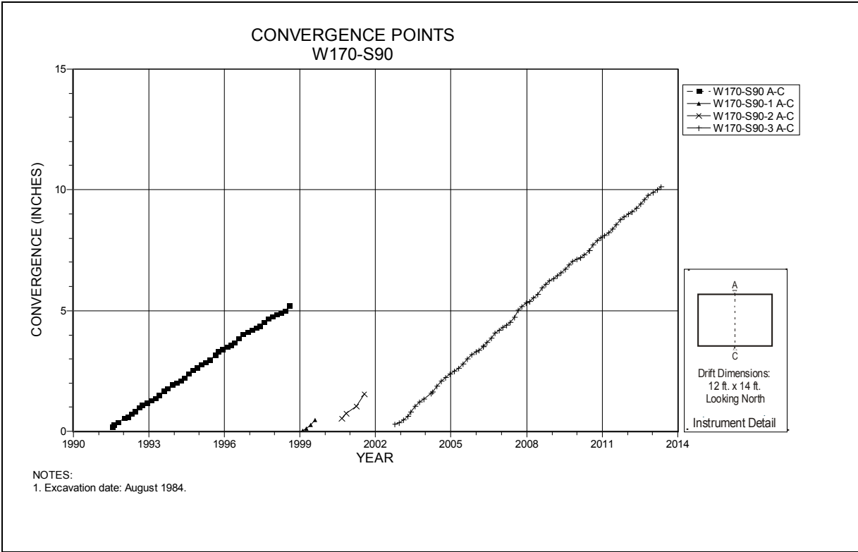
Figure 4-231 Convergence Point Array W170 S90 – Roof to Floor
