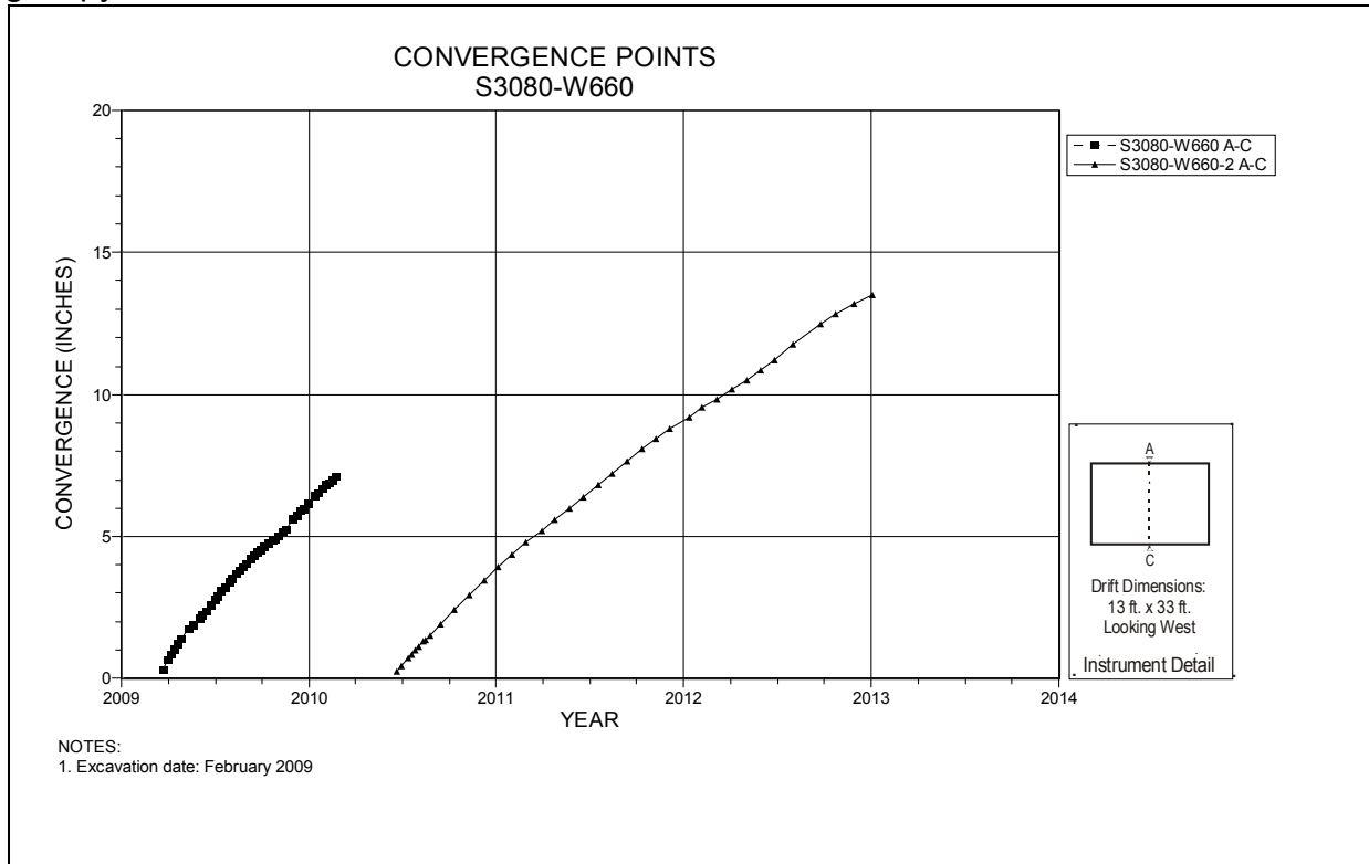
Figure 5-60 Convergence Point Array S3080 W660 Intersection (Room 3, Panel 6) – Roof to Floor
