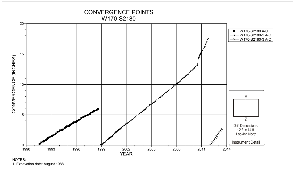
Figure 4-249 Convergence Point Array W170 S2180 – Roof to Floor
