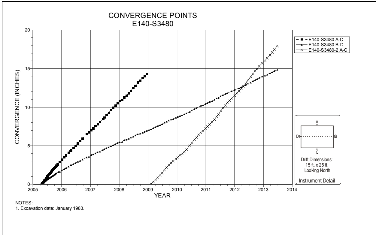
Figure 4-119 Convergence Point Array E140 S3480 – All Chords
