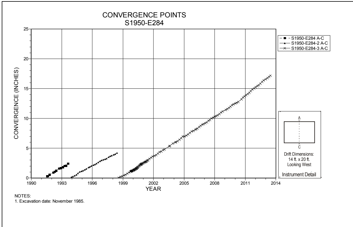
Figure 4-181 Convergence Point Array S1950 E284 – Roof to Floor
