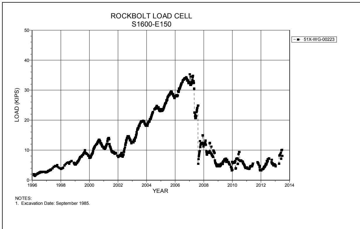
Figure 4-280 Rock Bolt Load Cell S1600 E150
