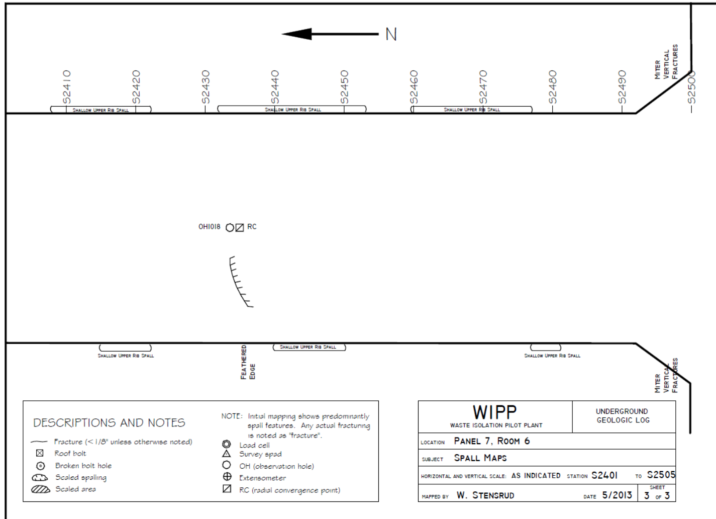
Figure 7-25 Panel 7 Room 6, S2401-S2505 Roof Fractures
