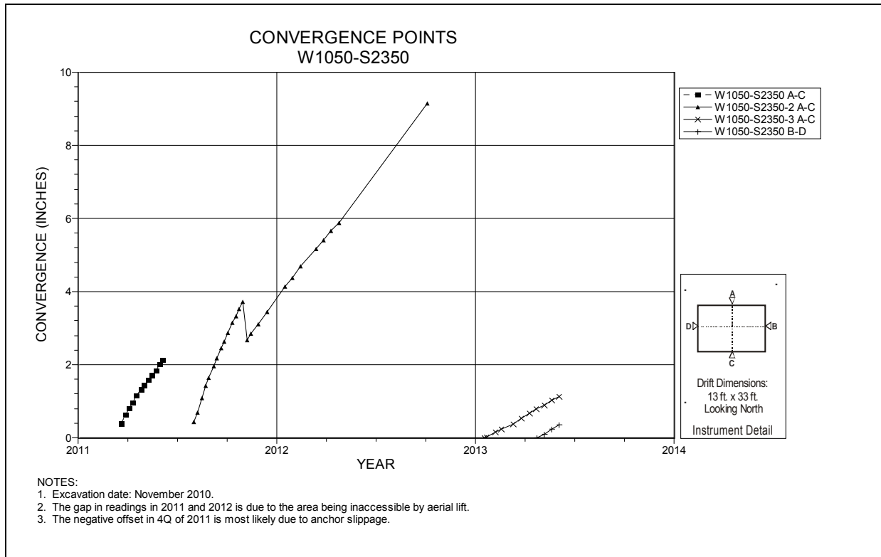
Figure 5-104 Convergence Point Array Room 6, Panel 7 at W1050 S2350 – Room Center – All Chords
