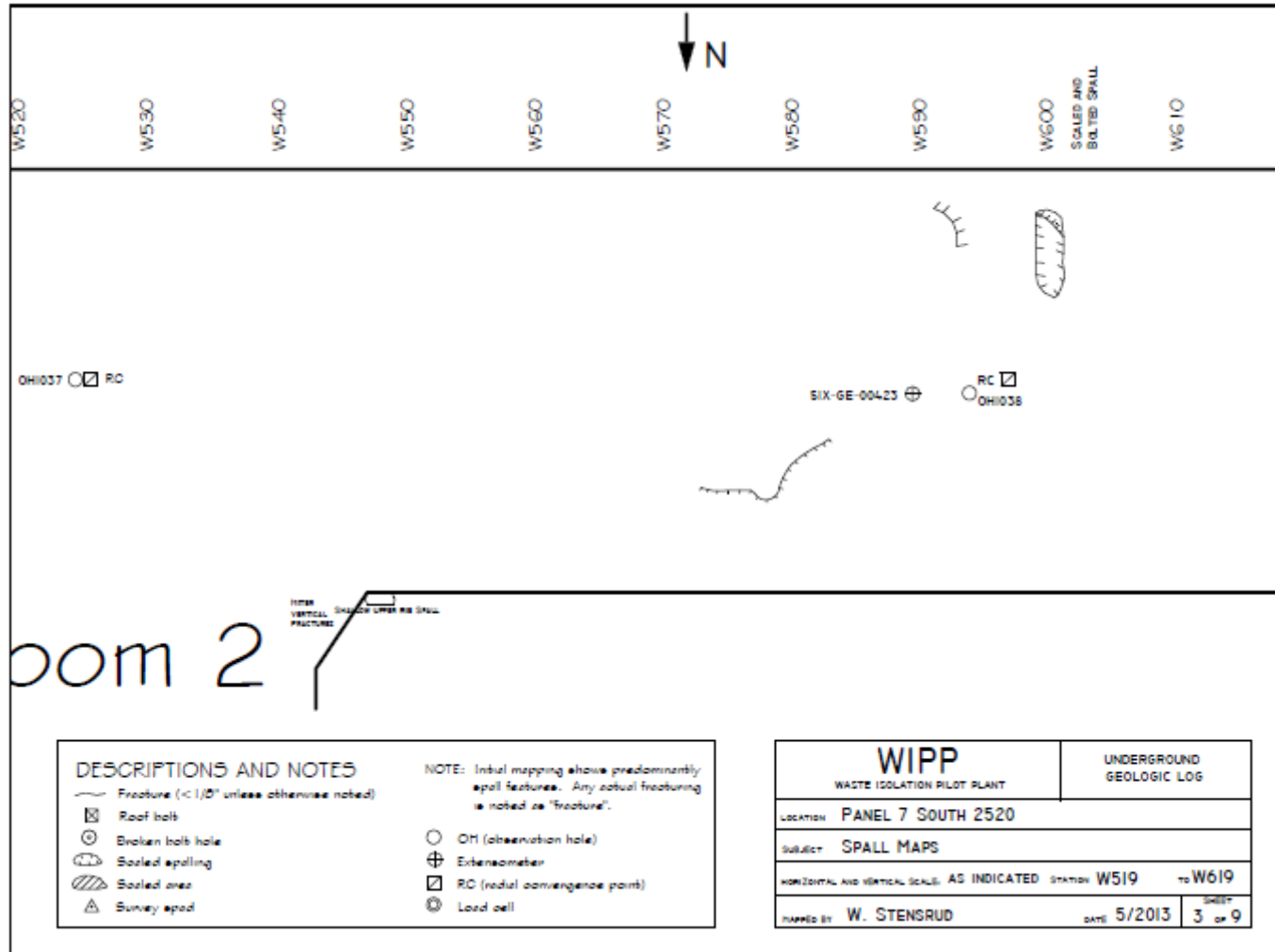
Figure 7-40 Panel 7 South 2520, W519-W619 Roof Fractures
