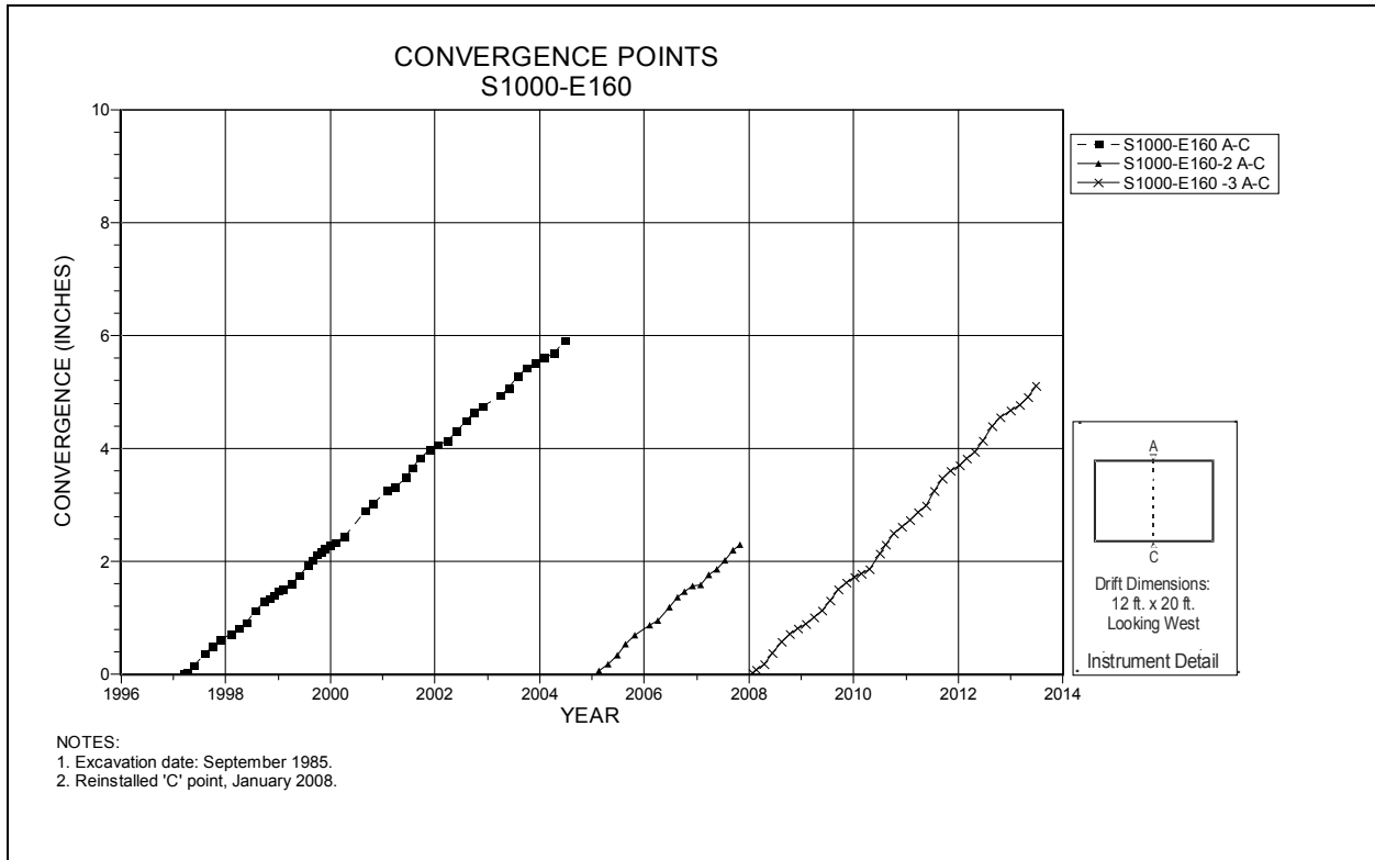
Figure 4-171 Convergence Point Array S1000 E160 – Roof to Floor
