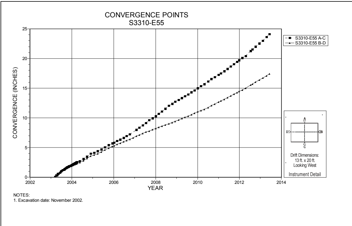
Figure 4-193 Convergence Point Array S3310 E55 – All Chords
