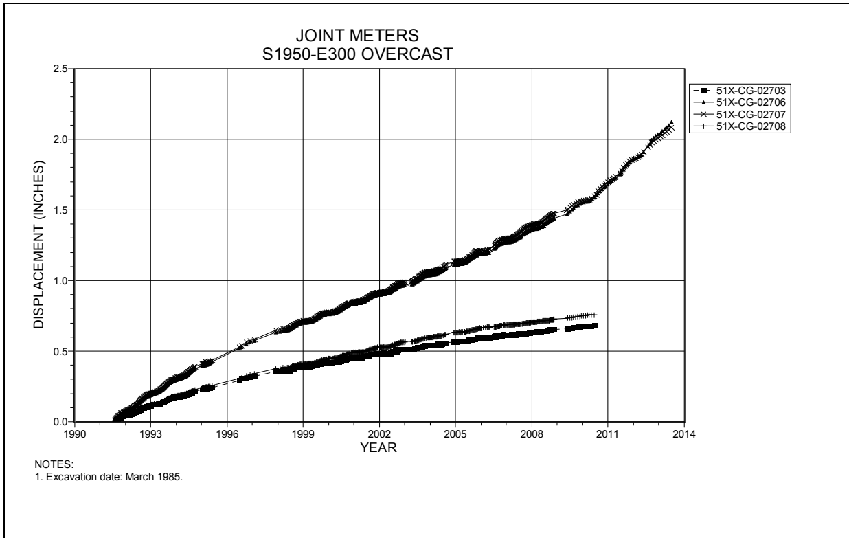
Figure 4-265 Joint Meters S1950 E300 Overcast
