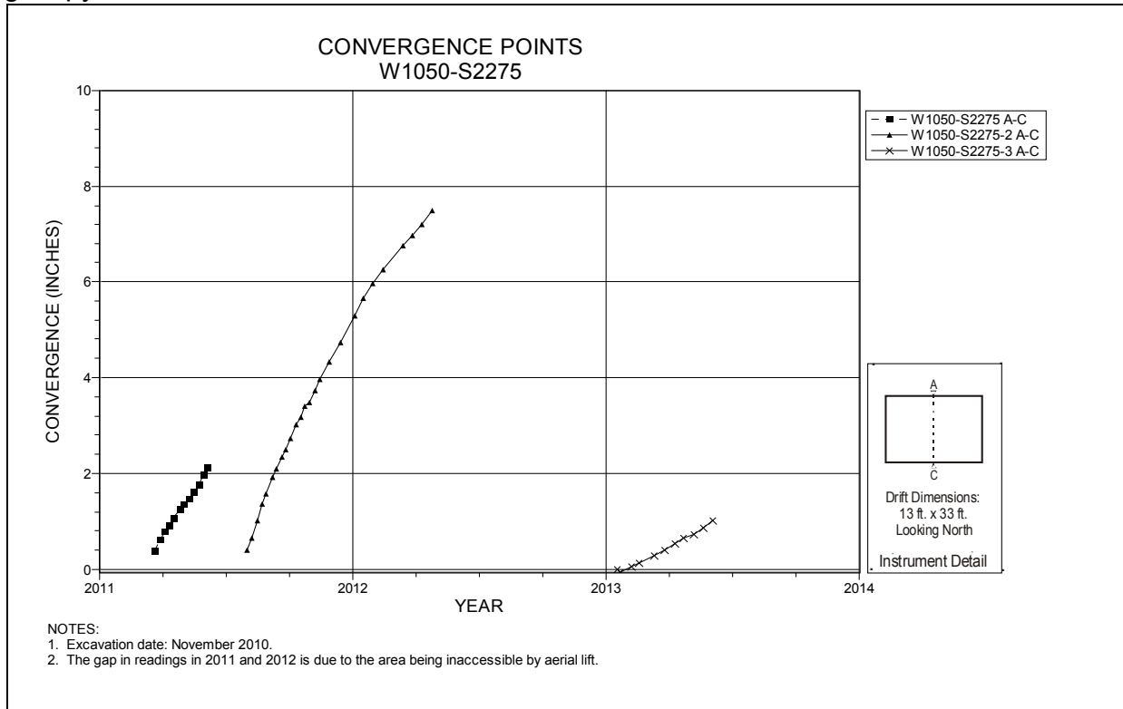
Figure 5-103 Convergence Point Array Room 6, Panel 7 at W1050 S2275 – Roof to Floor
