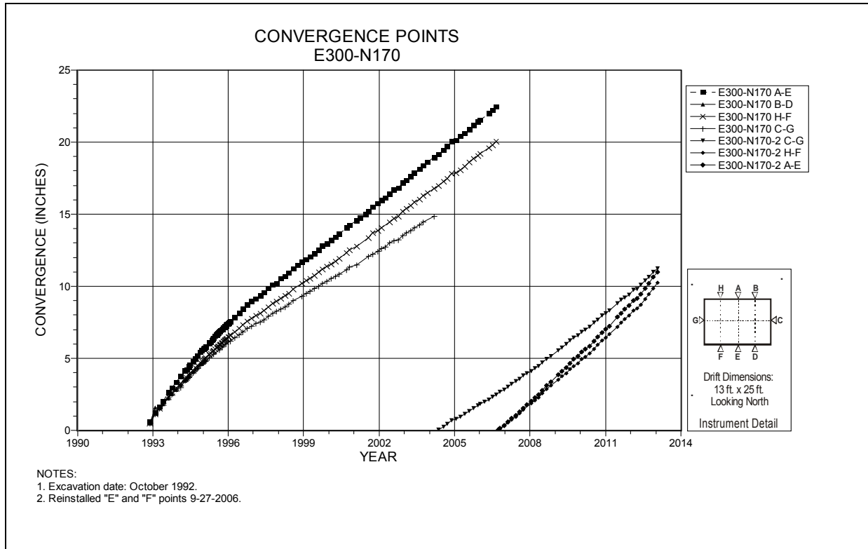
Figure 4-123 Convergence Point Array E300 N170 – All Chords
