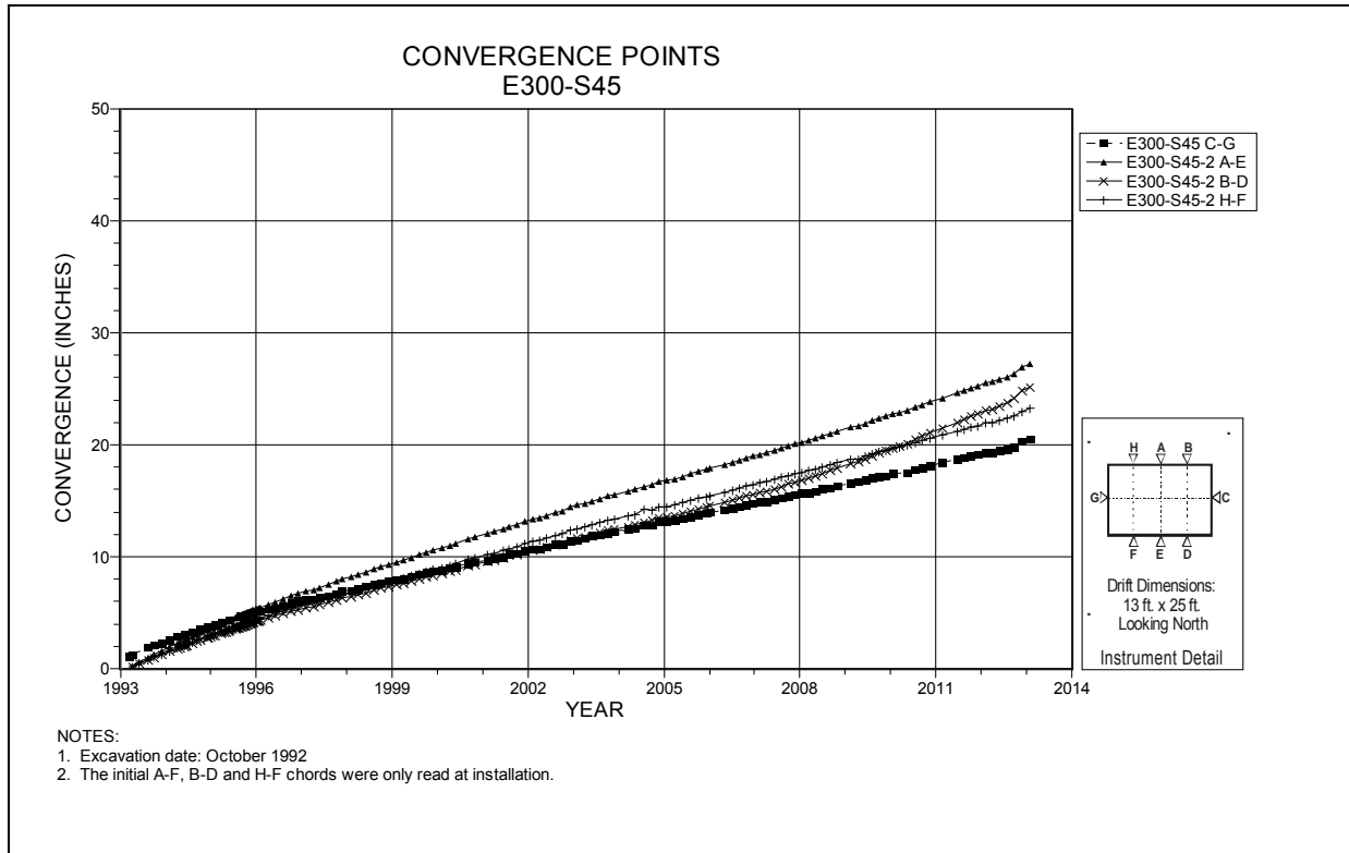
Figure 4-127 Convergence Point Array E300 S45 – All Chords
