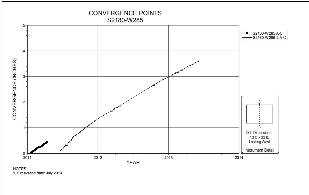
Figure 5-74 Convergence Point Array S2180 W285 – Roof to Floor
