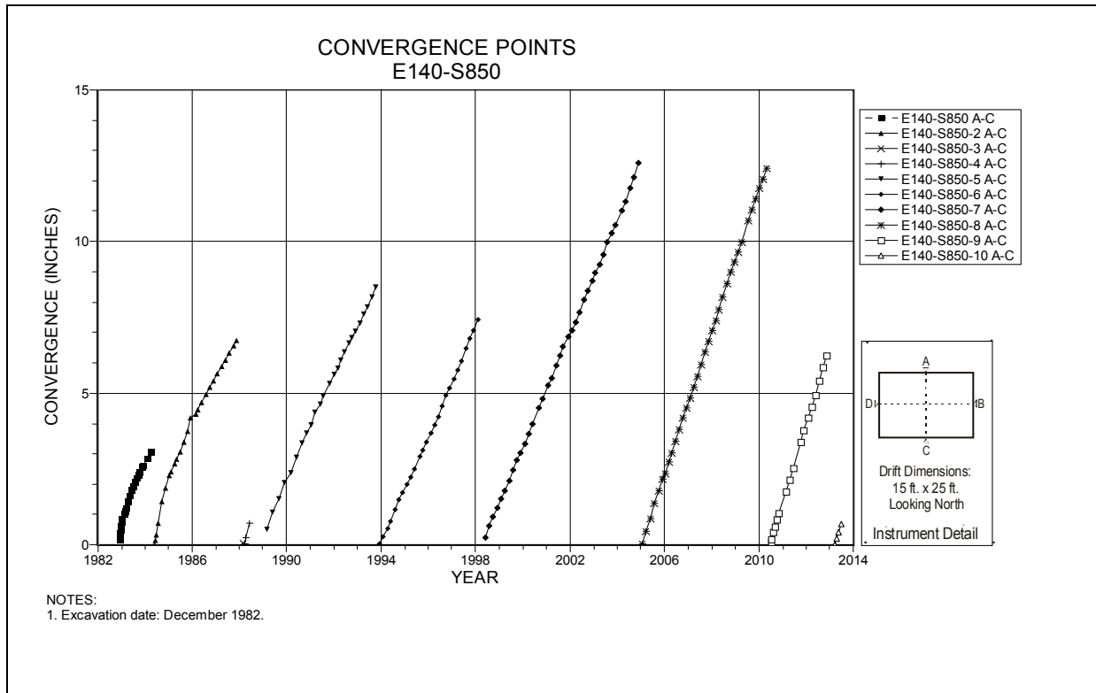
Figure 4-68 Convergence Point Array E140 S850 – Roof to Floor
