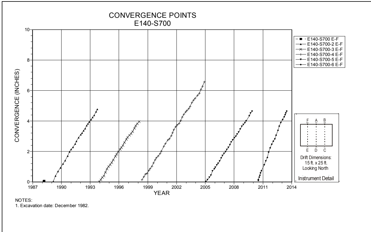
Figure 4-67 Convergence Point Array E140 S700 – Roof to Floor – West Quarter Point
