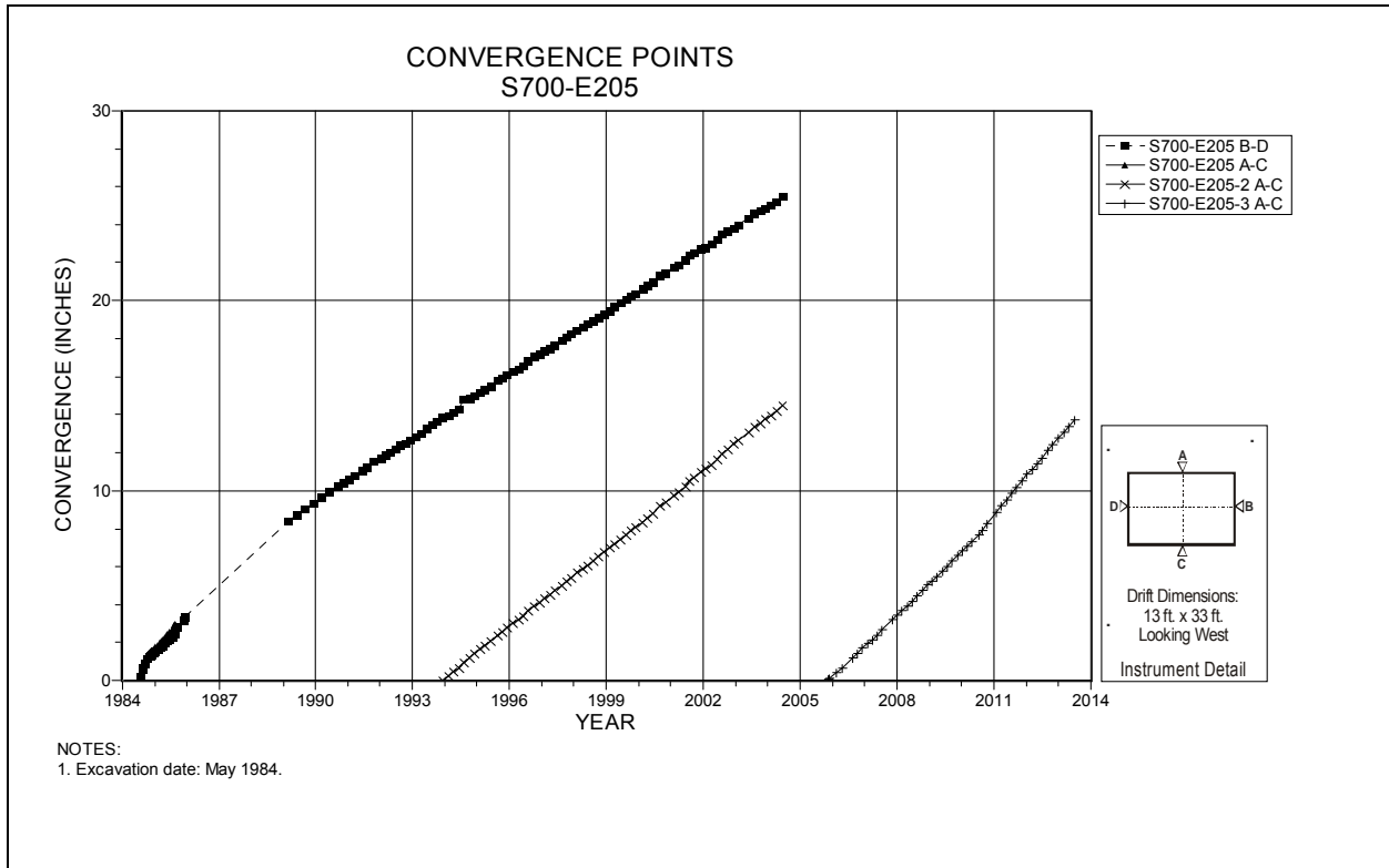
Figure 4-167 Convergence Point Array S700 E205 – All Chords
