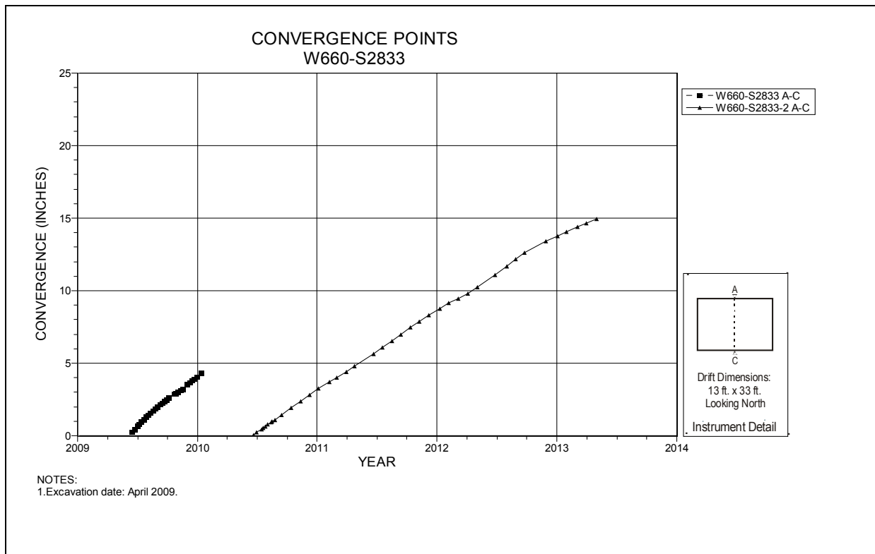
Figure 5-49 Convergence Point Array Room 3, Panel 6 at W660 S2833 – Roof to Floor
