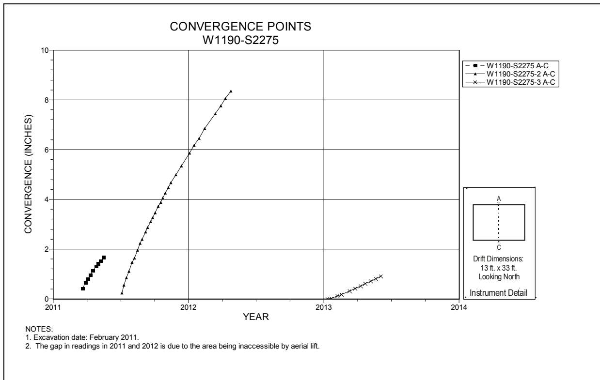
Figure 5-106 Convergence Point Array Room 7, Panel 7 at W1190 S2275 – Roof to Floor
