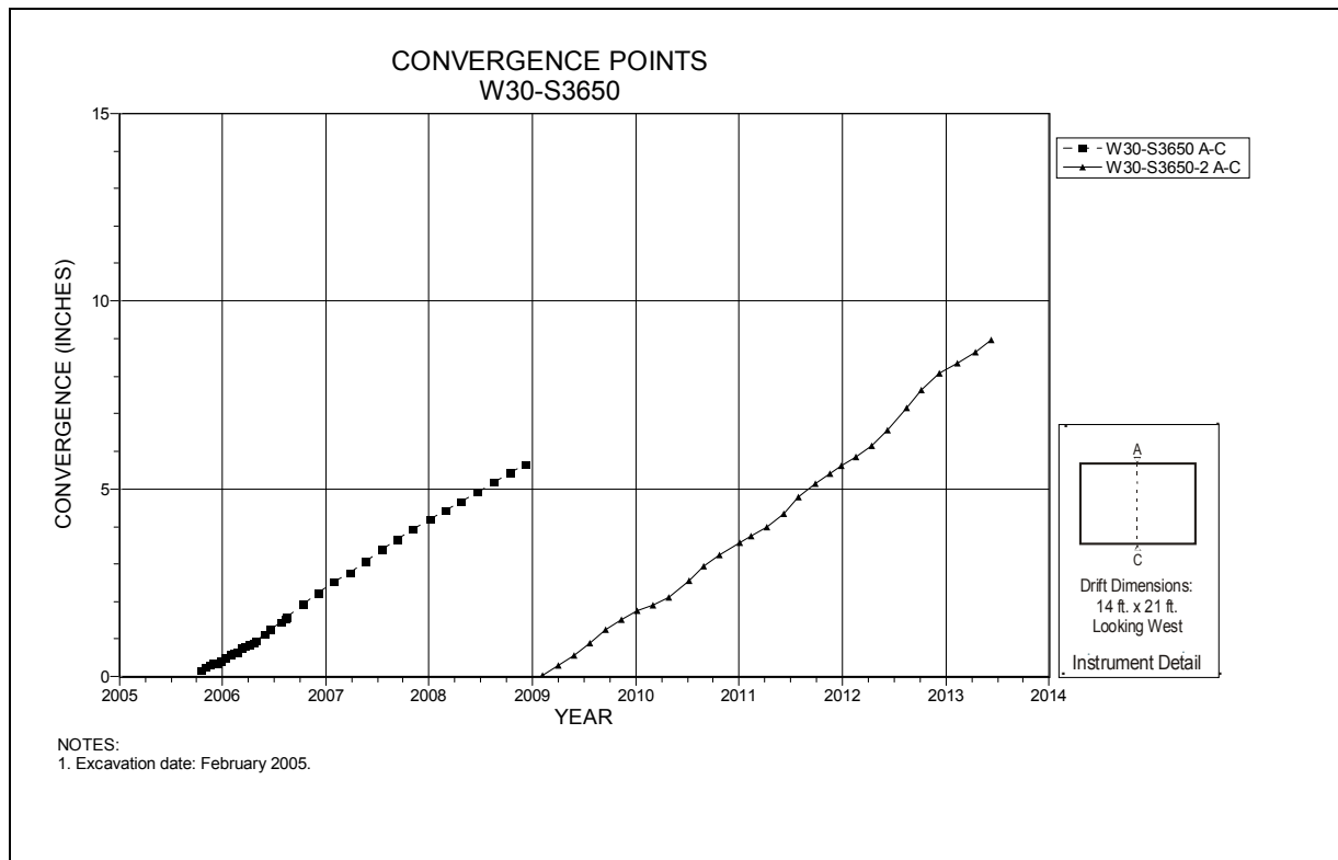
Figure 4-228 Convergence Point Array W30 S3650 – Roof to Floor
