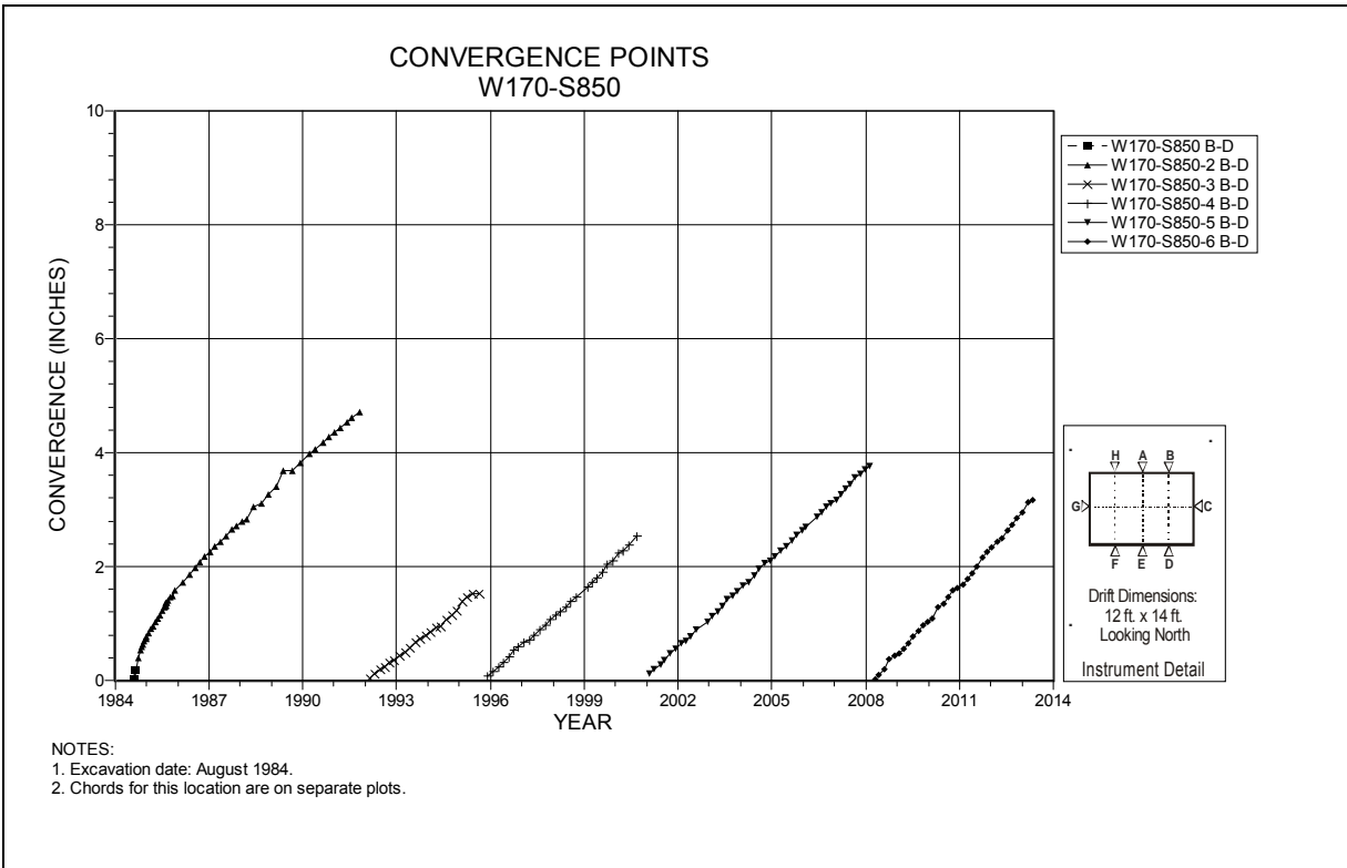
Figure 4-237 Convergence Point Array W170 S850 – Roof to Floor – East Quarter Point
