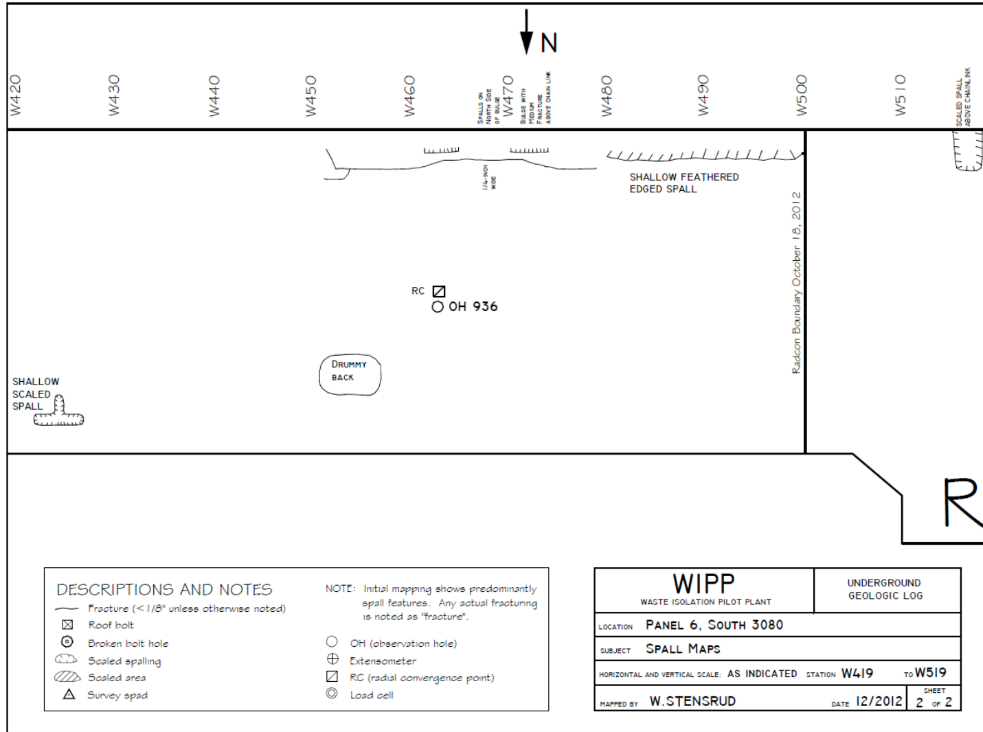
Figure 7-7 Panel 6 South 3080, W419-W519 Roof Fractures
