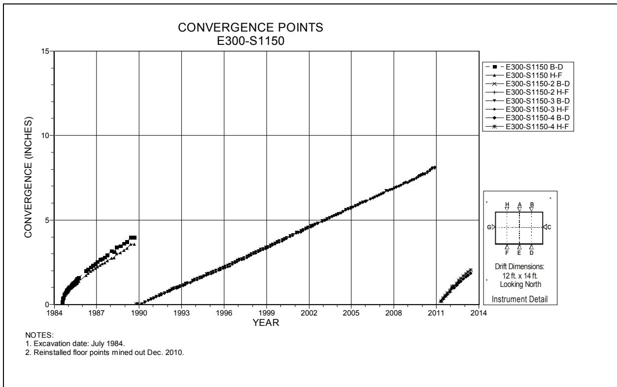
Figure 4-134 Convergence Point Array E300 S1150 – Roof to Floor – Quarter Points
