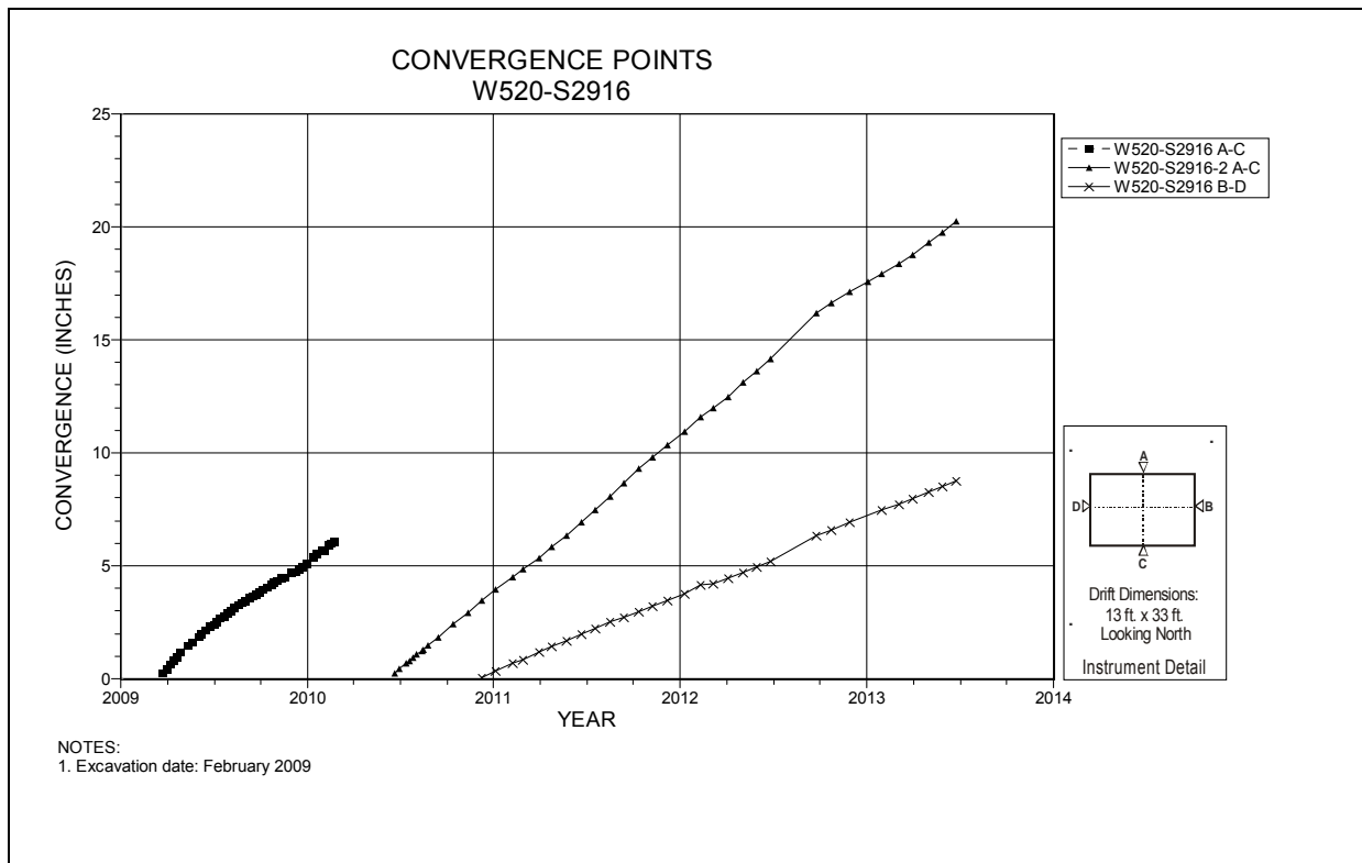
Figure 5-47 Convergence Point Array Room 2, Panel 6 at W520 S2916 – Room Center – All Chords
