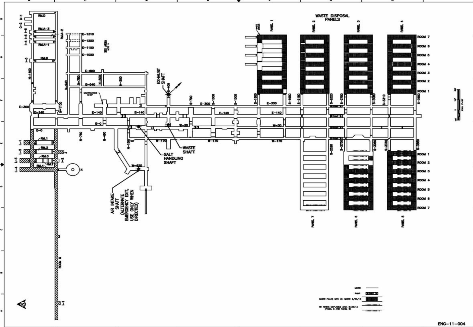
Figure 1 - 2 Underground Mining and Waste Disposal Configuration as of June 30, 2013
