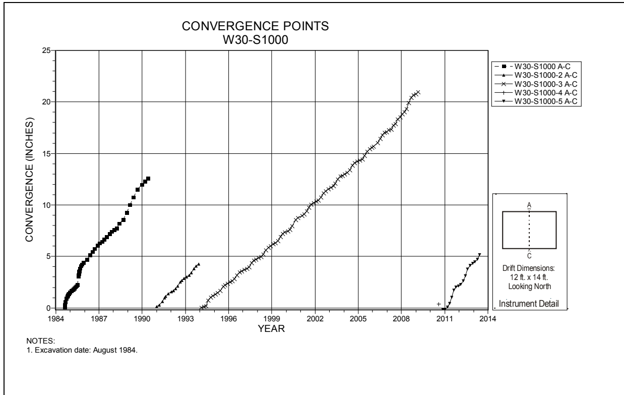
Figure 4-207 Convergence Point Array W30 S1000 – Roof to Floor
