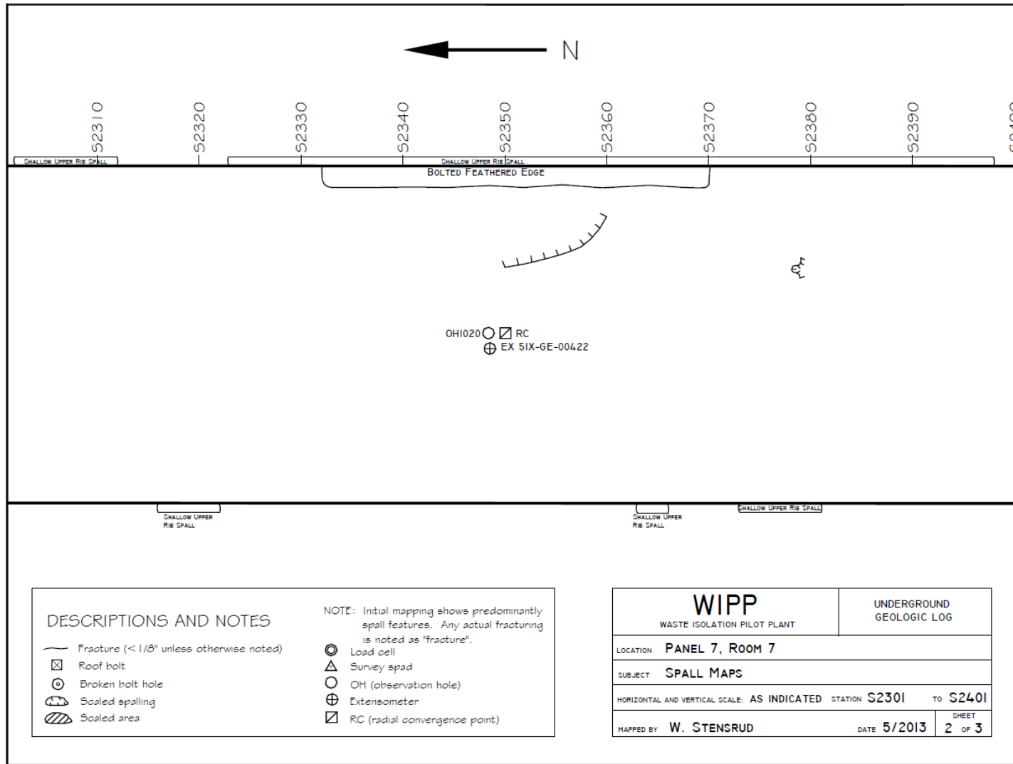
Figure 7-27 Panel 7 Room 7, S2301-S2401 Roof Fractures
