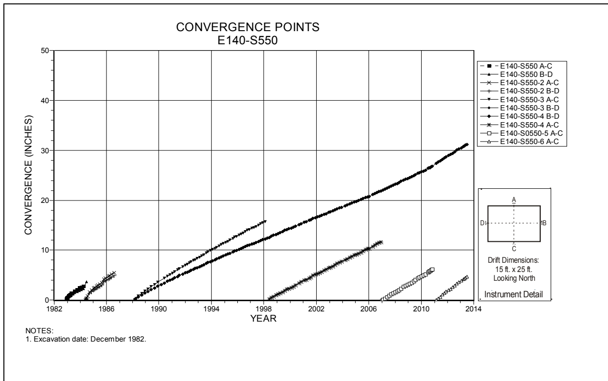
Figure 4-64 Convergence Point Array E140 S550 – All Chords
