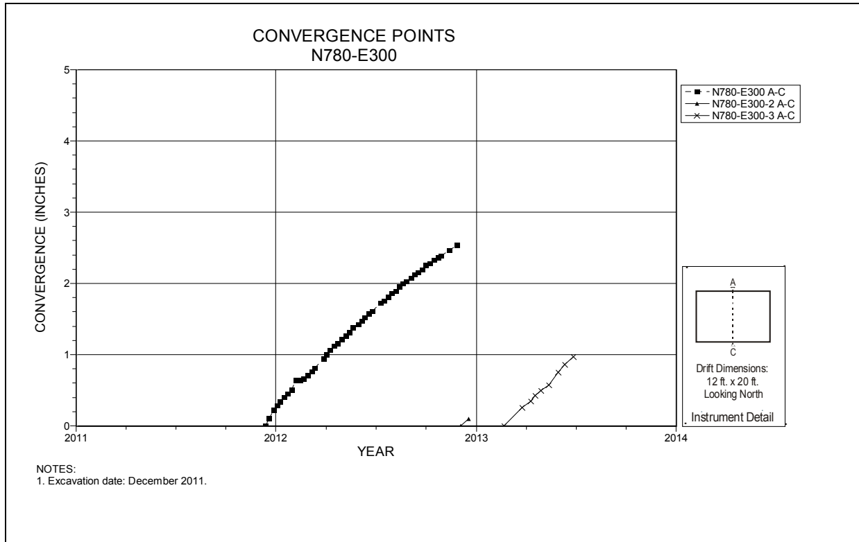
Figure 6-26 Convergence Point Array N780 E300 – Roof to Floor
