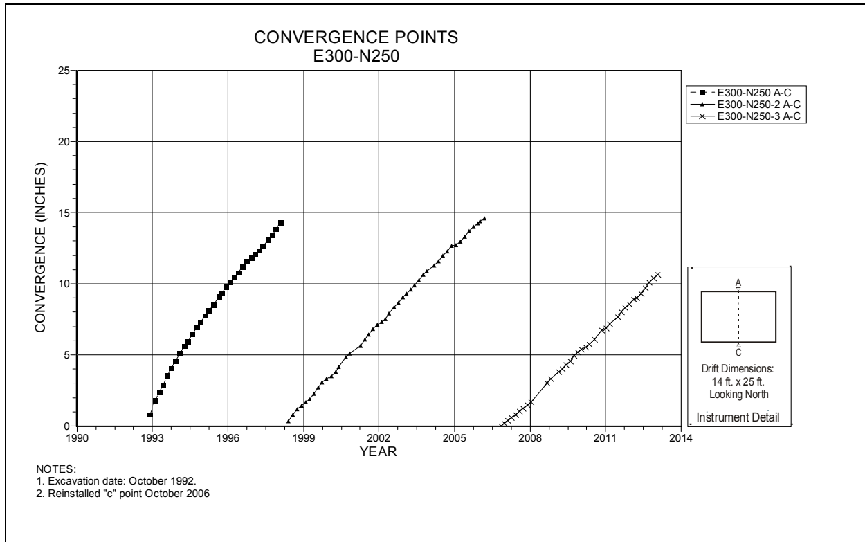
Figure 4-124 Convergence Point Array E300 N250 – Roof to Floor
