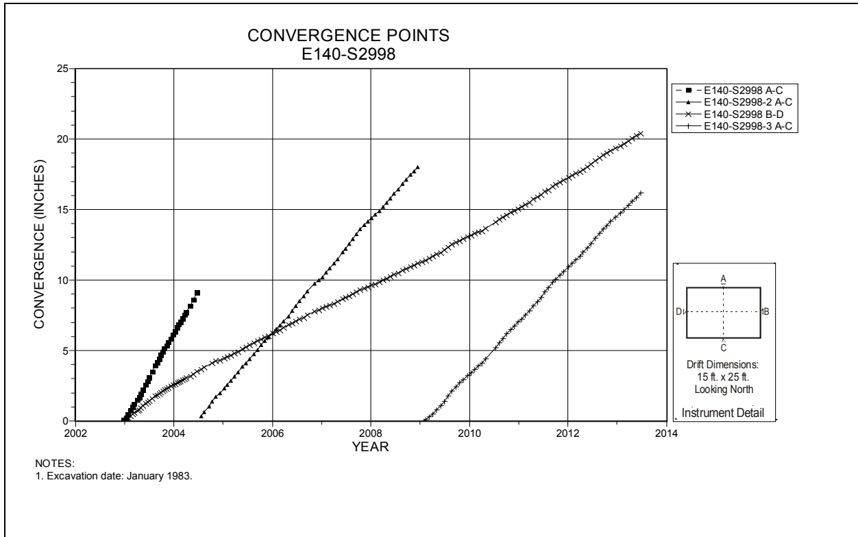
Figure 4-113 Convergence Point Array E140 S2998 – All Chords
