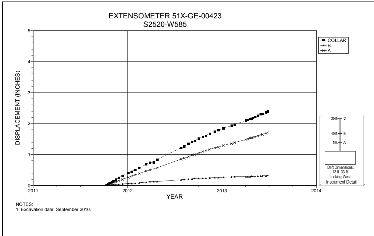
Figure 5-72 Extensometer 51X-GE-00423 S2520 W585 – Roof
