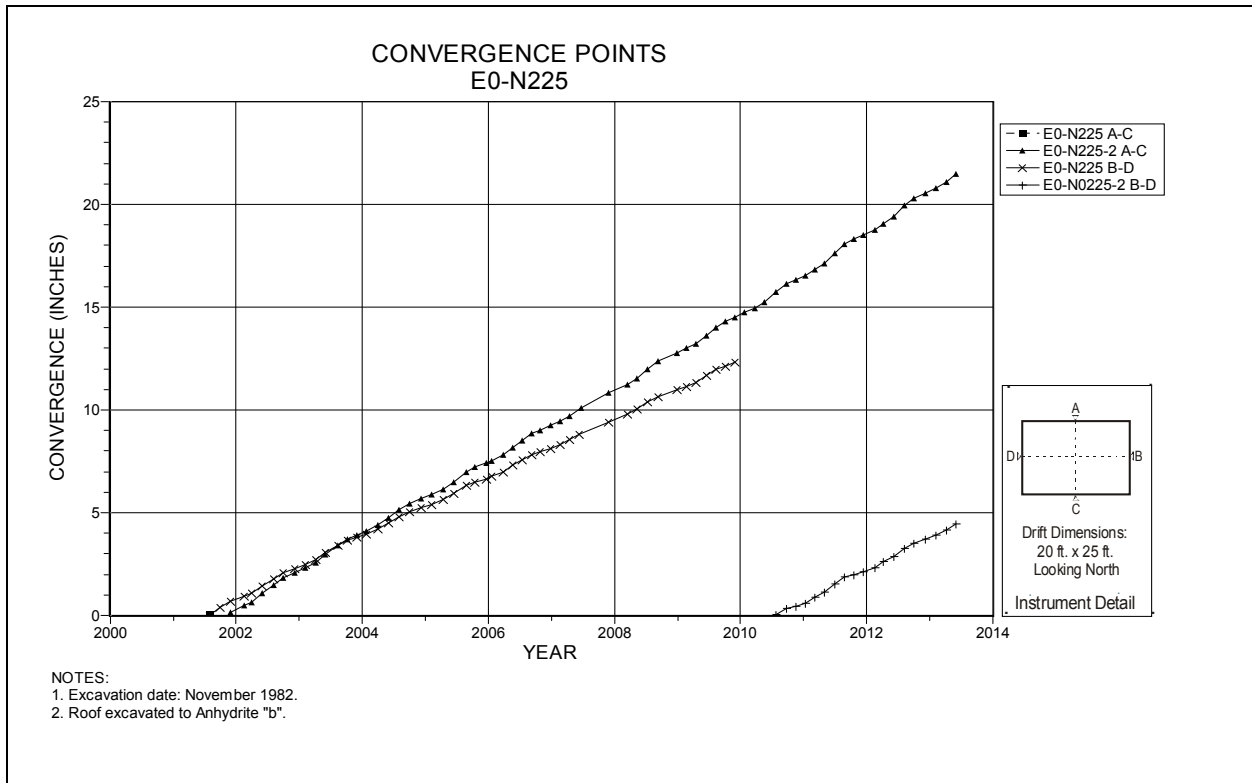
Figure 4-38 Convergence Point Array E0 N225 – All Chords
