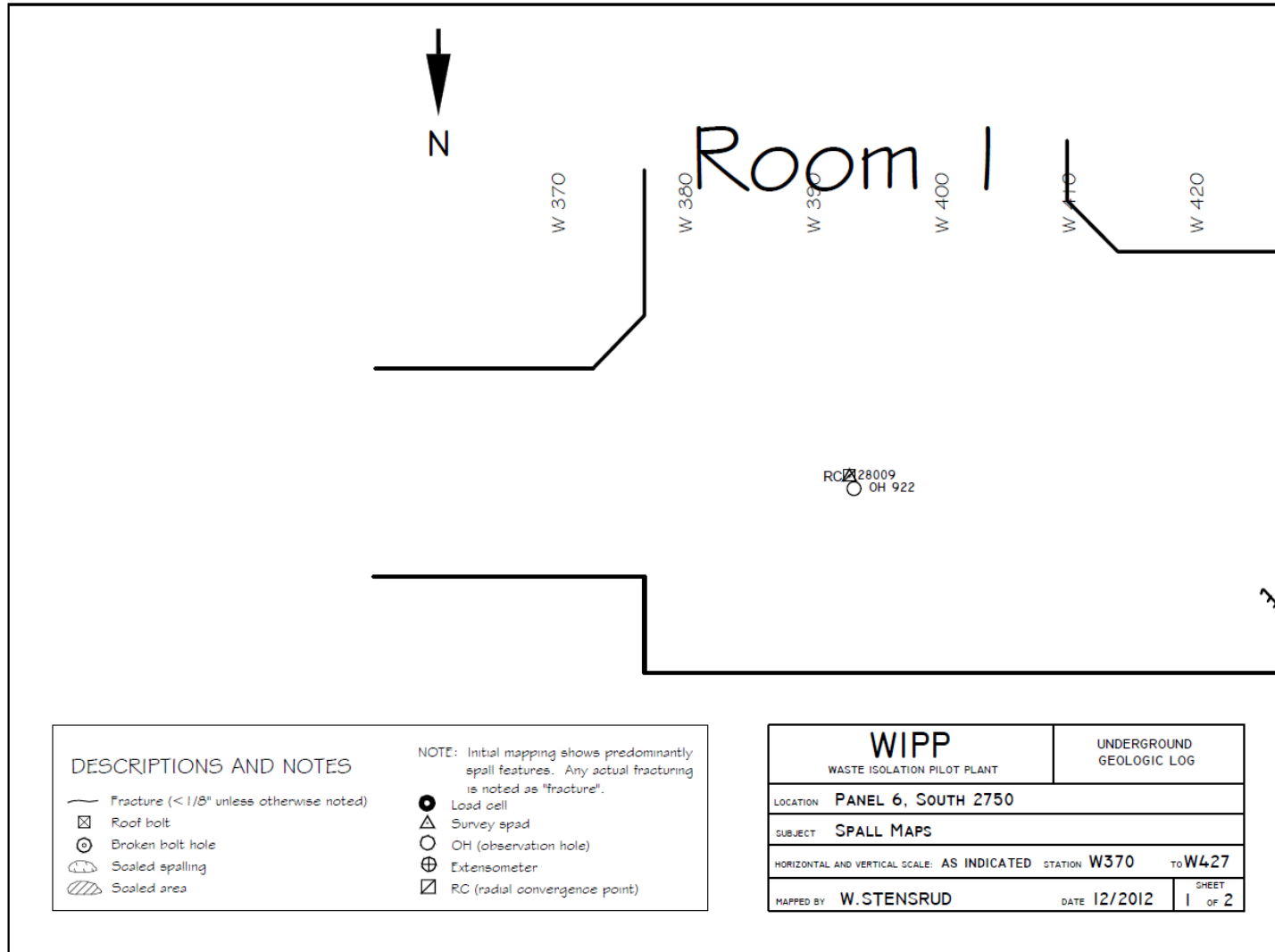
Figure 7-4 Panel 6 South 2750, W370-W427 Roof Fractures
