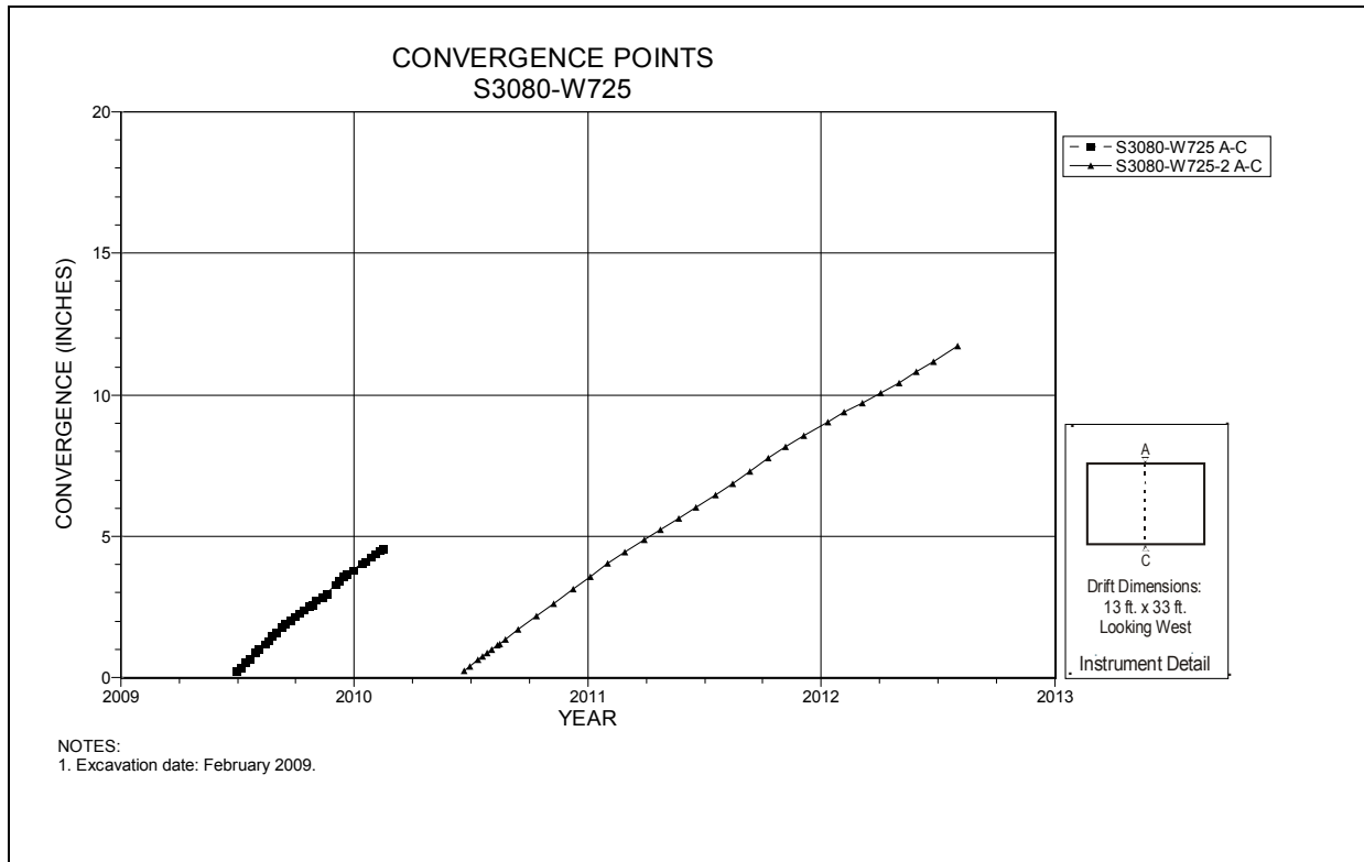
Figure 5-61 Convergence Point Array S3080 W725 – Roof to Floor
