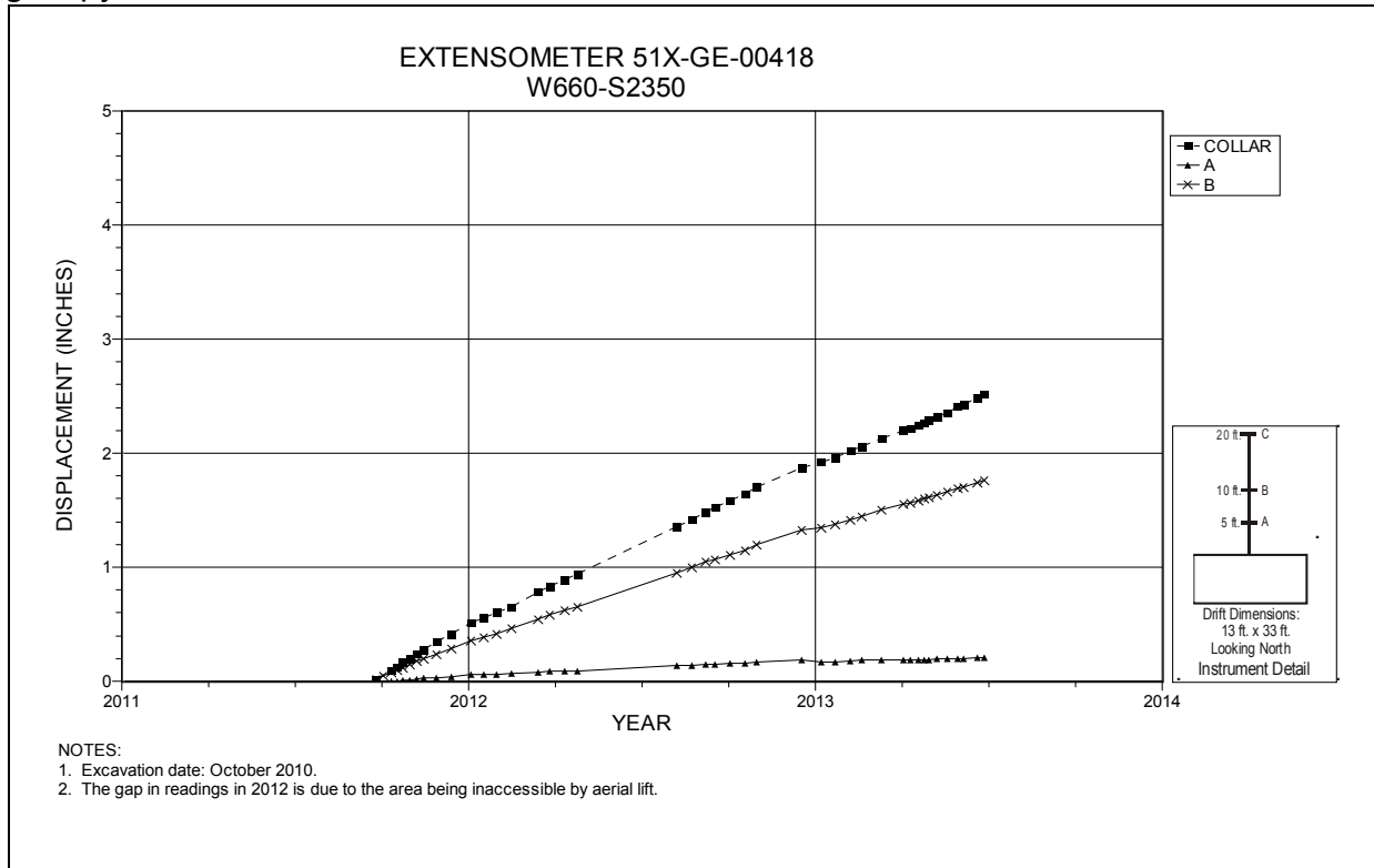
Figure 5-67 Extensometer 51X-GE-00418 Room 3, Panel 7 at W660 S2350 – Room Center – Roof
