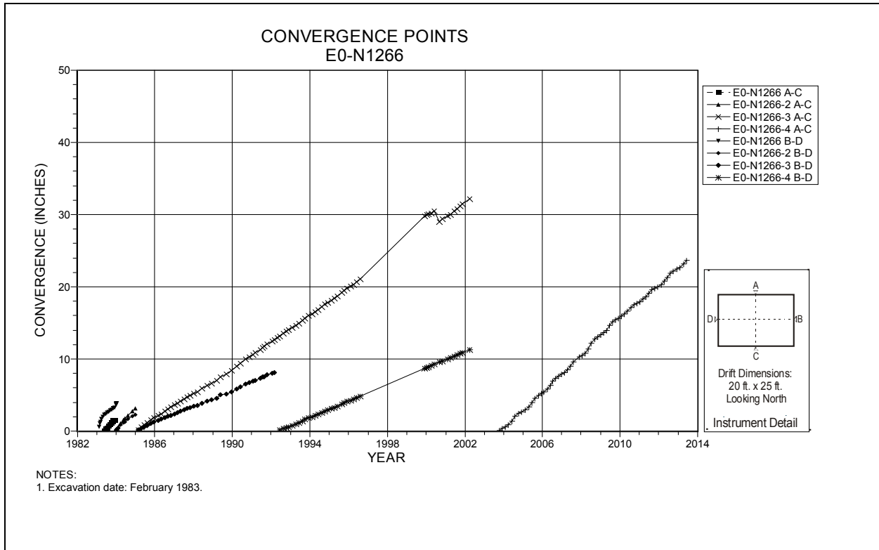
Figure 4-47 Convergence Point Array E0 N1266 – All Chords
