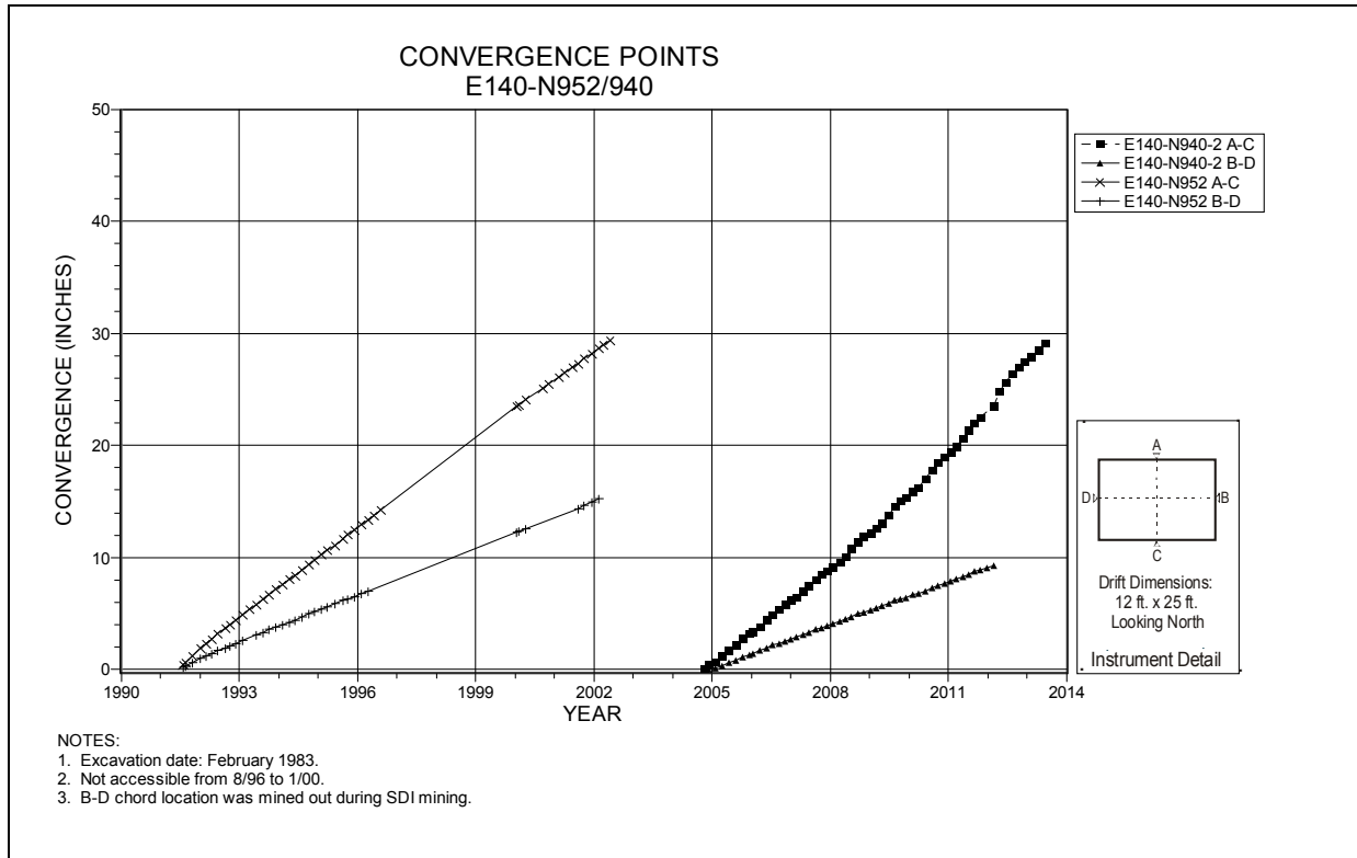
Figure 4-57 Convergence Point Array E140 N940/N952 – All Chords
