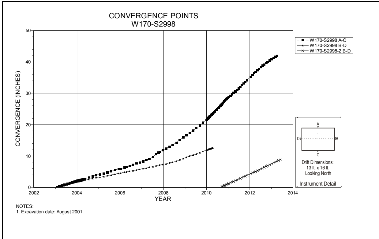
Figure 4-257 Convergence Point Array W170 S2998 – All Chords
