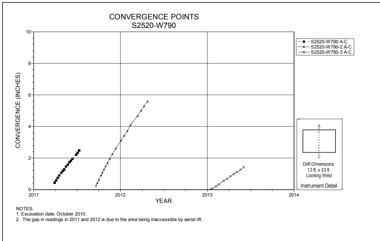
Figure 5-116 Convergence Point Array S2520 W790 Intersection (Room 4, Panel 7) – Roof to Floor
