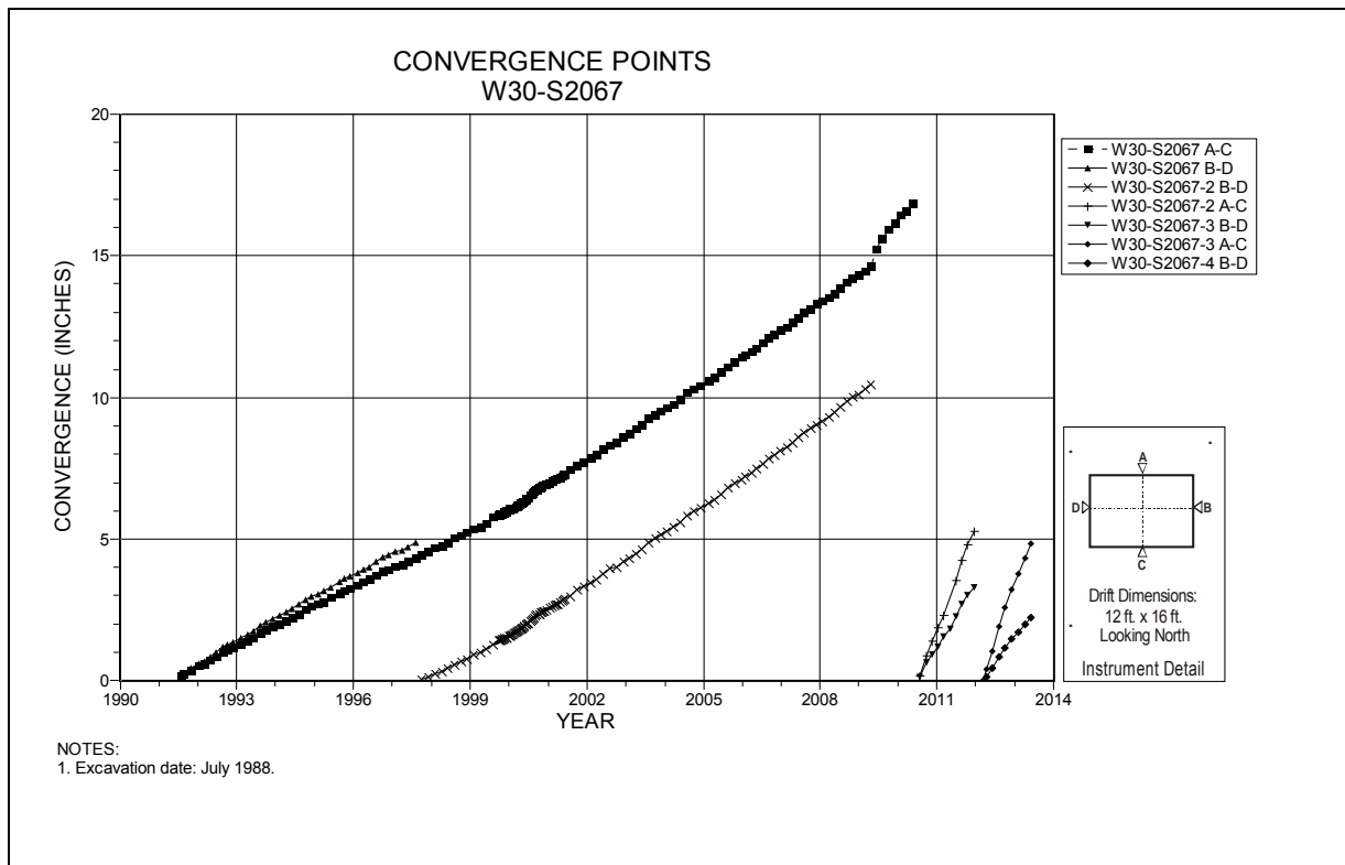
Figure 4-214 Convergence Point Array W30 S2067 – All Chords
