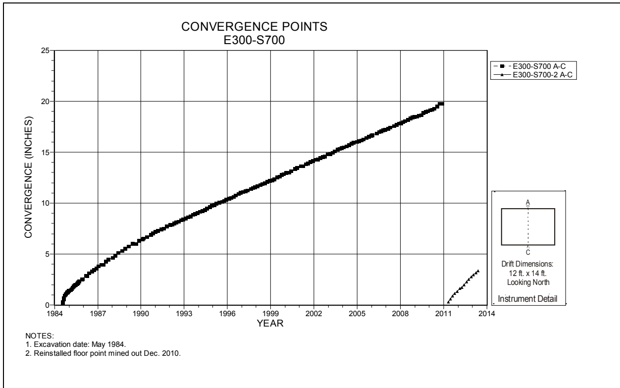
Figure 4-130 Convergence Point Array E300 S700 – Roof to Floor
