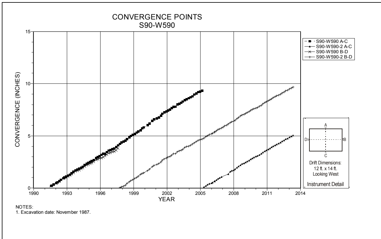
Figure 4-160 Convergence Point Array S90 W590 – All Chords
