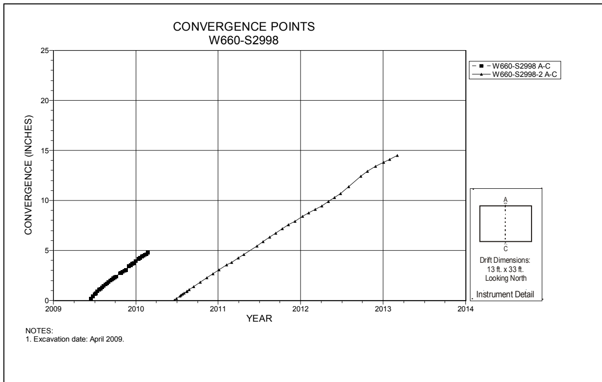
Figure 5-51 Convergence Point Array Room 3, Panel 6 at W660 S2998 – Roof to Floor
