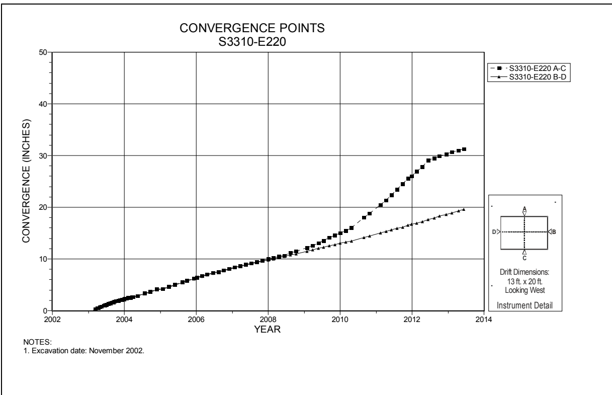
Figure 4-194 Convergence Point Array S3310 E220 – All Chords
