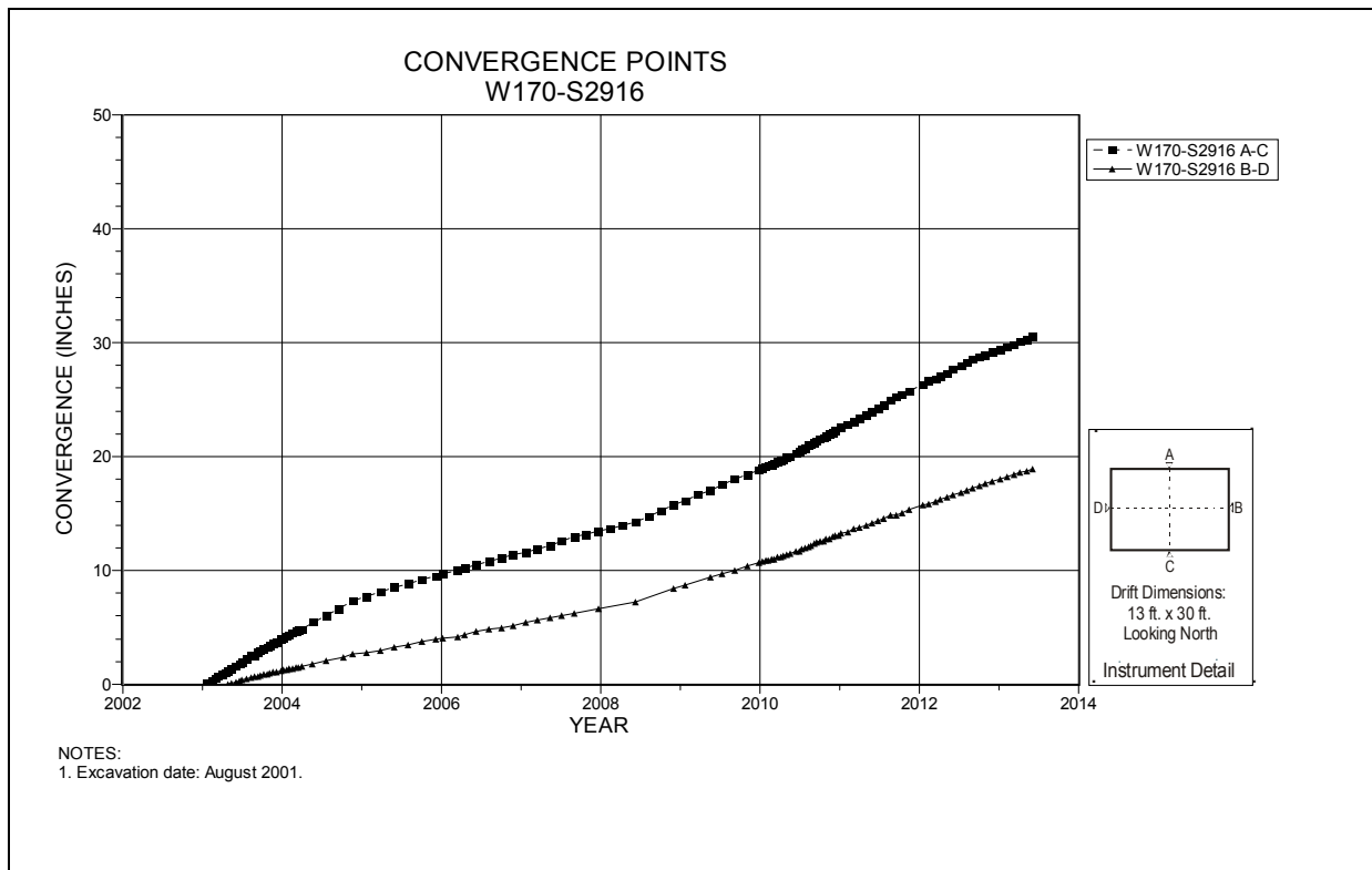
Figure 4-256 Convergence Point Array W170 S2916 – All Chords
