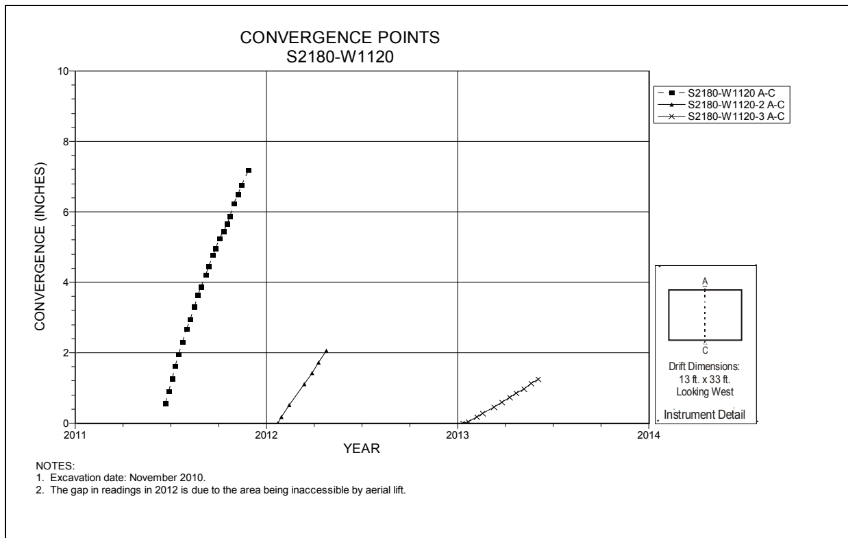
Figure 5-86 Convergence Point Array S2180 W1120 – Roof to Floor
