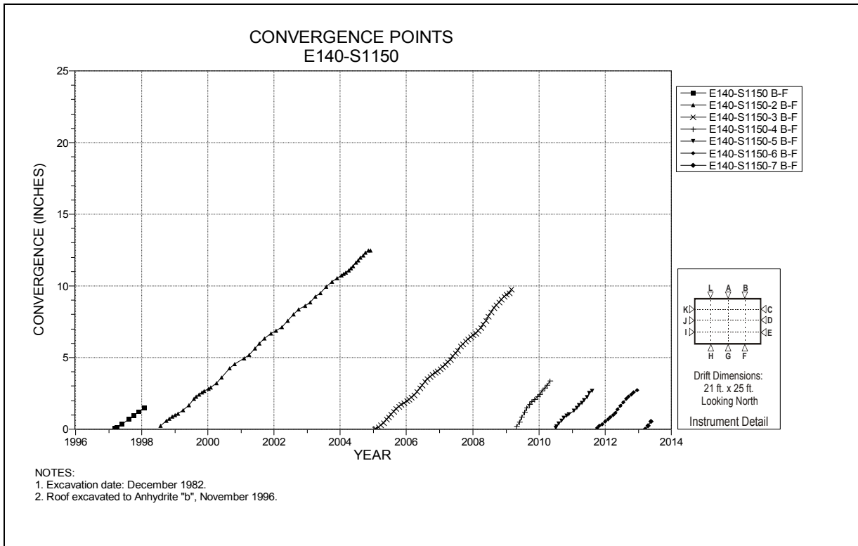
Figure 4-76 Convergence Point Array E140 S1150 – Roof to Floor – East Quarter Point
