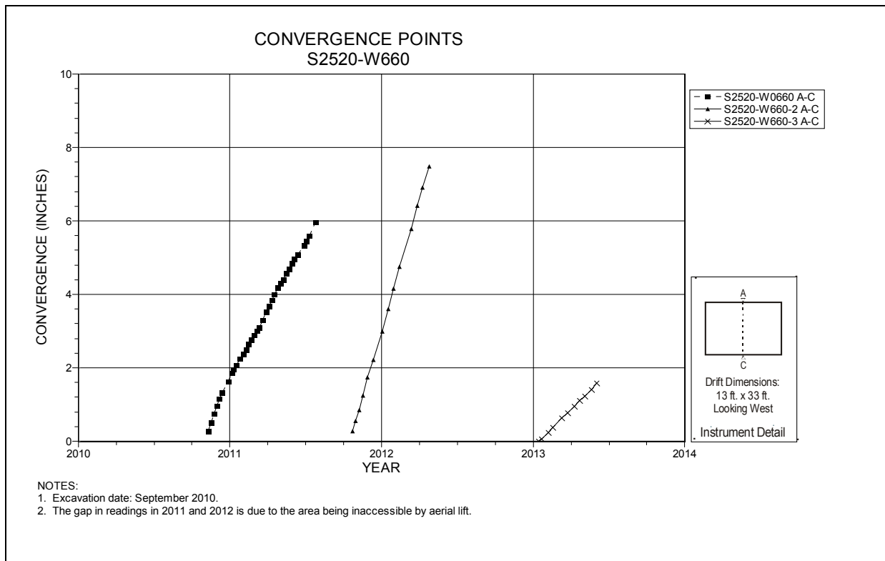
Figure 5-114 Convergence Point Array S2520 W660 Intersection (Room 3, Panel 7) – Roof to Floor
