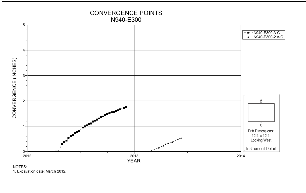
Figure 6-41 Convergence Point Array N940 E300 – Roof to Floor
