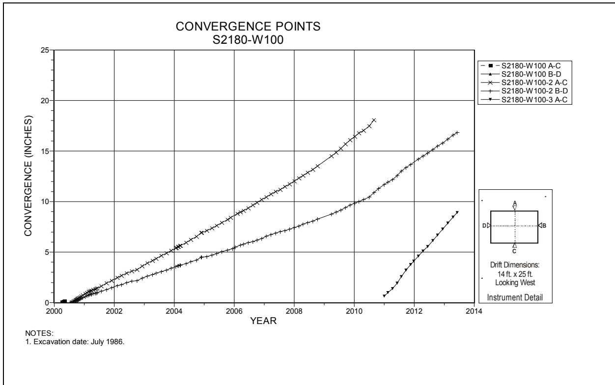
Figure 4-184 Convergence Point Array S2180 W100 – All Chords
