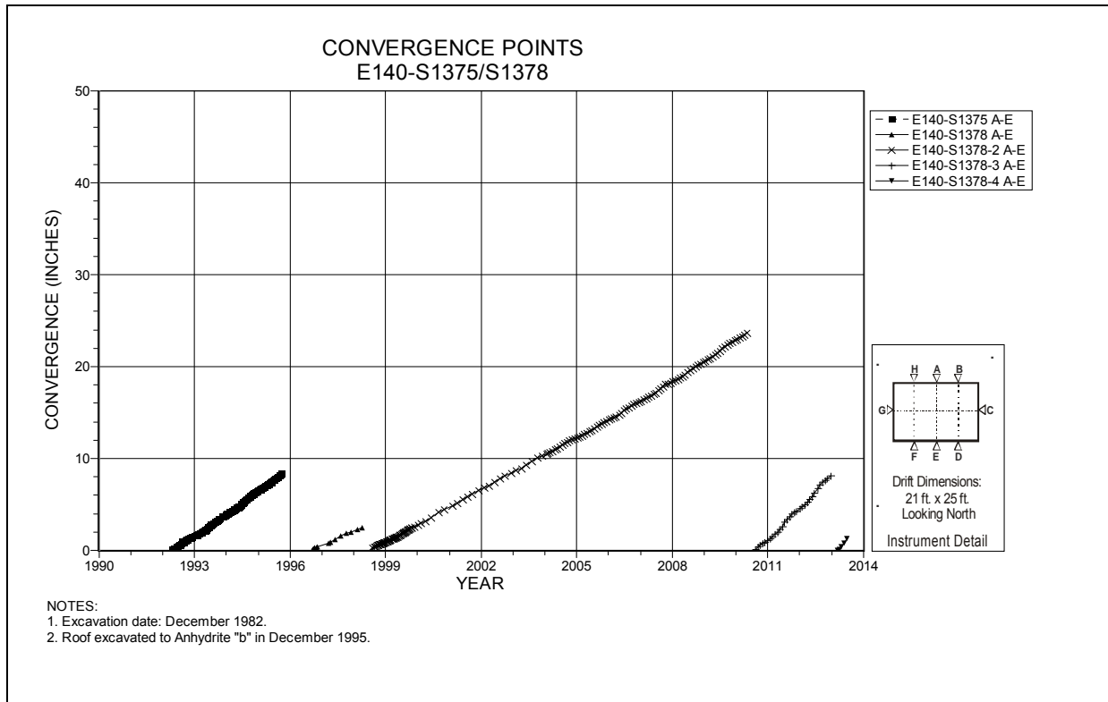
Figure 4-82 Convergence Point Array E140 S1375/S1378 – Roof to Floor – Centerline
