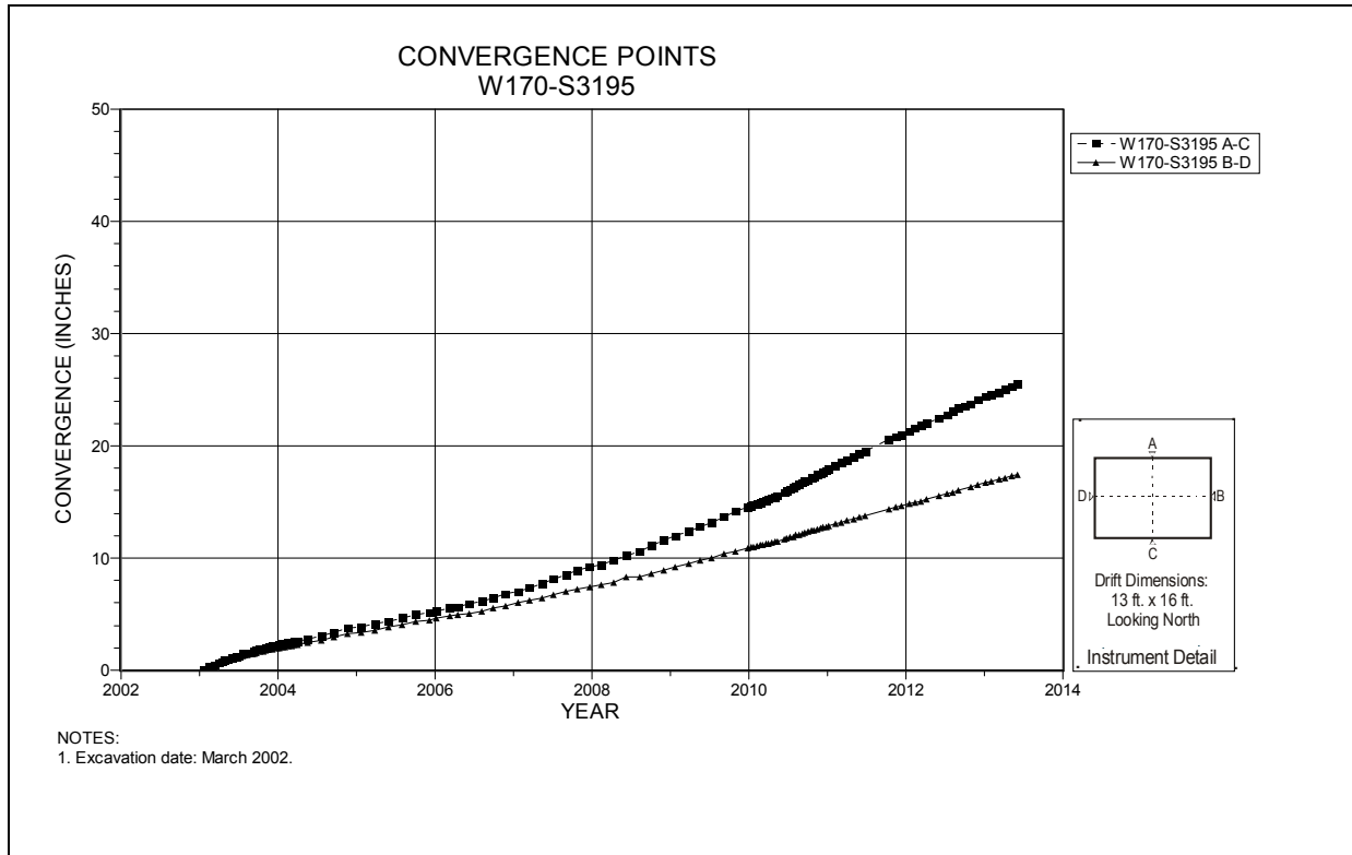
Figure 4-259 Convergence Point Array W170 S3195 – All Chords
