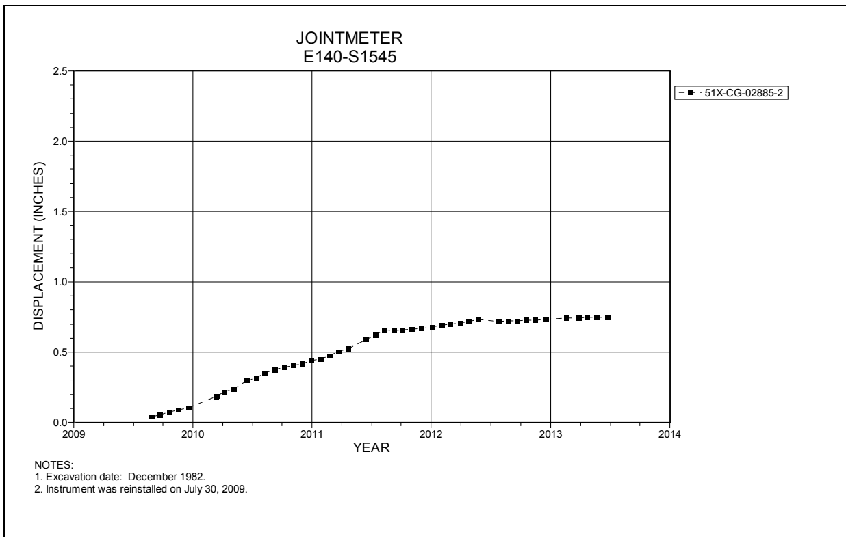
Figure 4-268 Joint Meter E140 S1545
