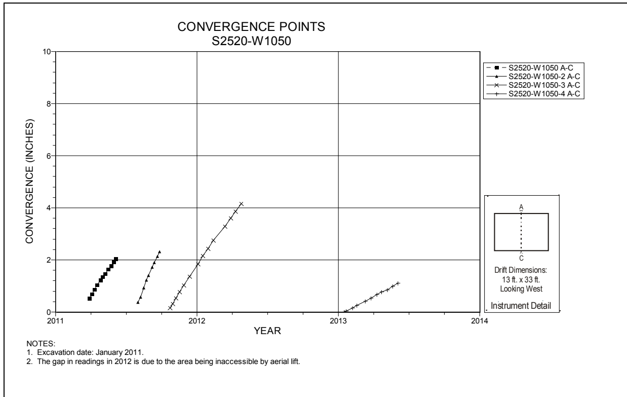
Figure 5-120 Convergence Point Array S2520 W1050 Intersection (Room 6, Panel 7) – Roof to Floor
