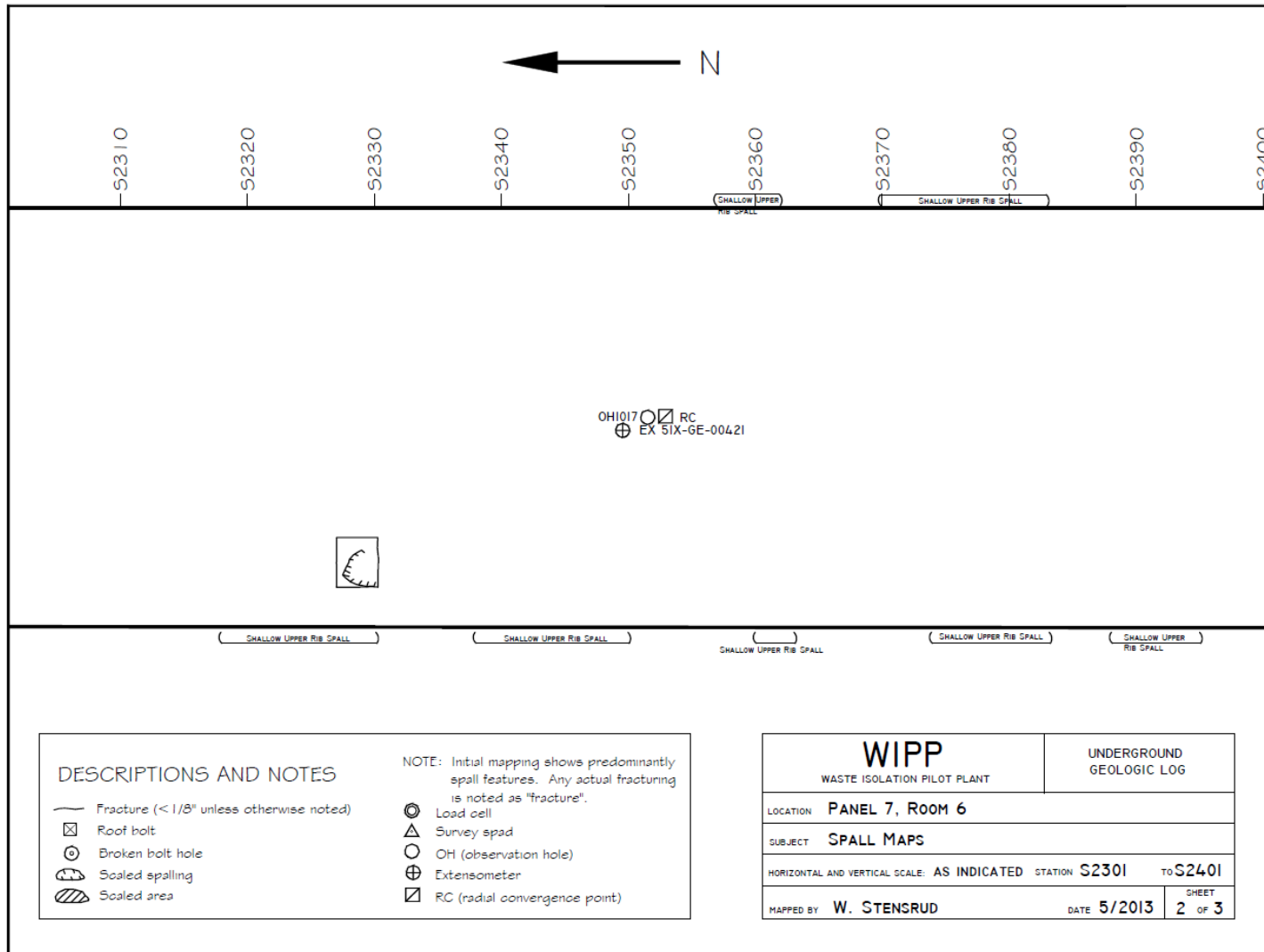
Figure 7-24 Panel 7 Room 6, S2301-S2401 Roof Fractures
