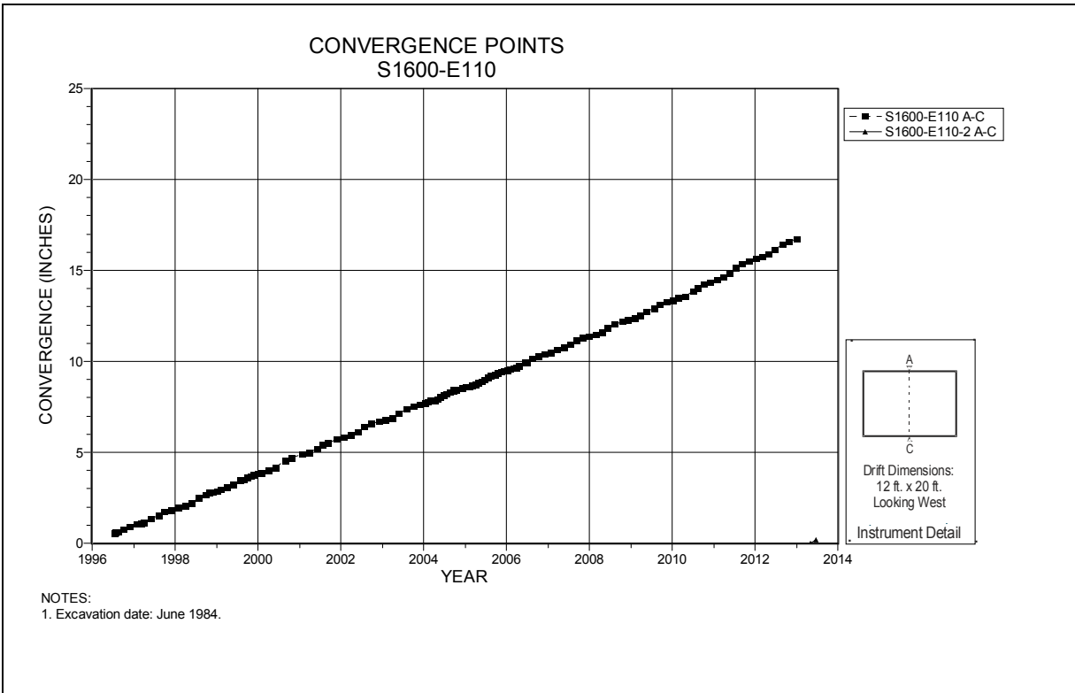
Figure 4-177 Convergence Point Array S1600 E110 – Roof to Floor
