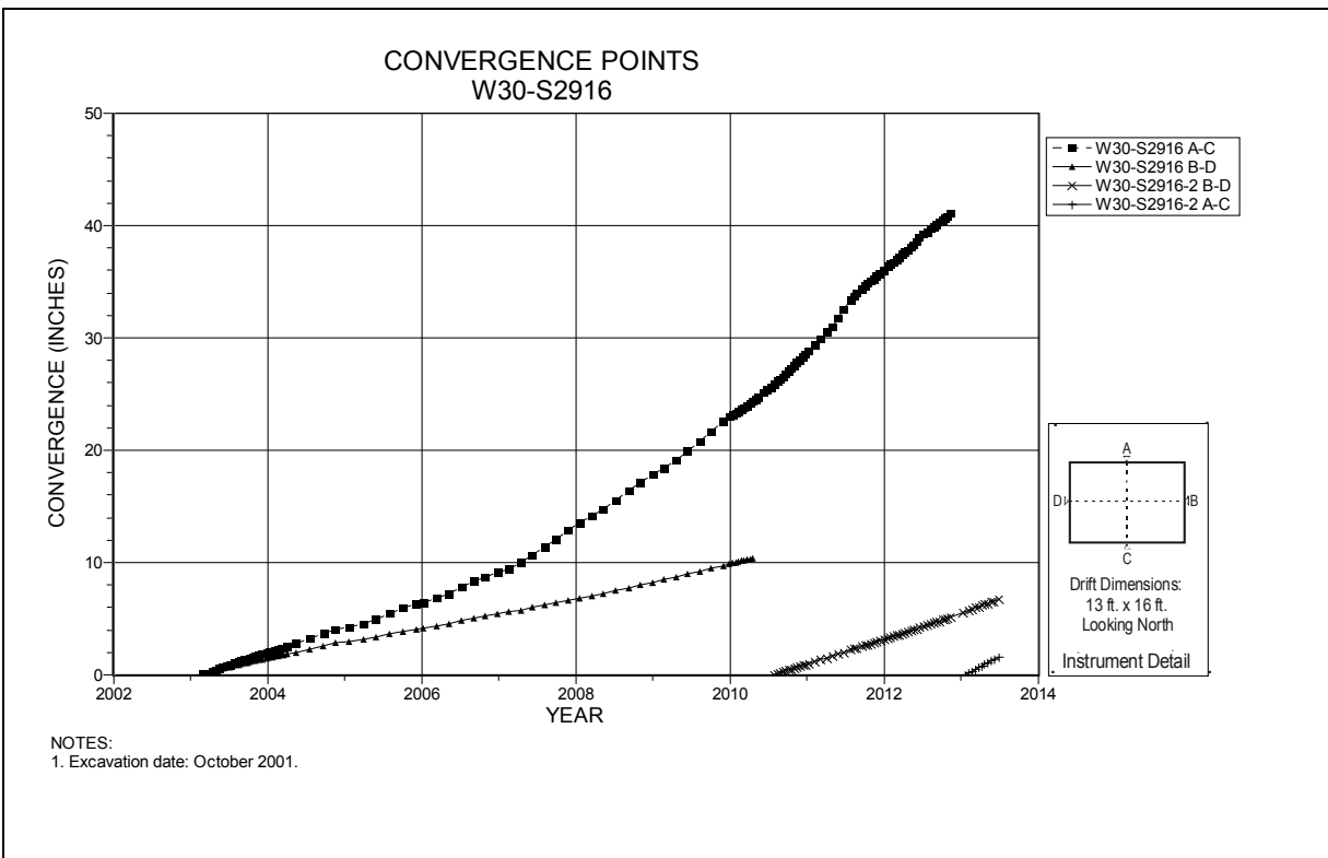
Figure 4-222 Convergence Point Array W30 S2916 – All Chords
