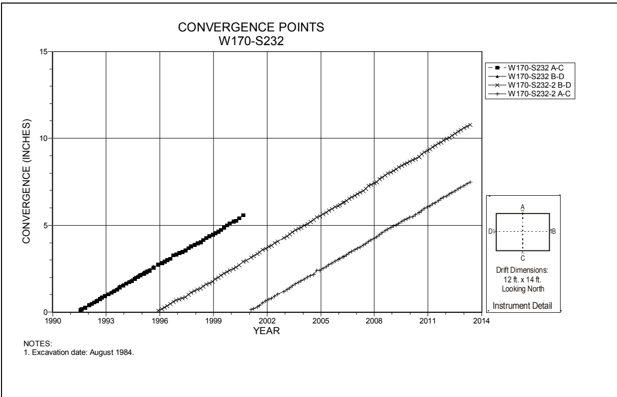
Figure 4-232 Convergence Point Array W170 S232 – All Chords
