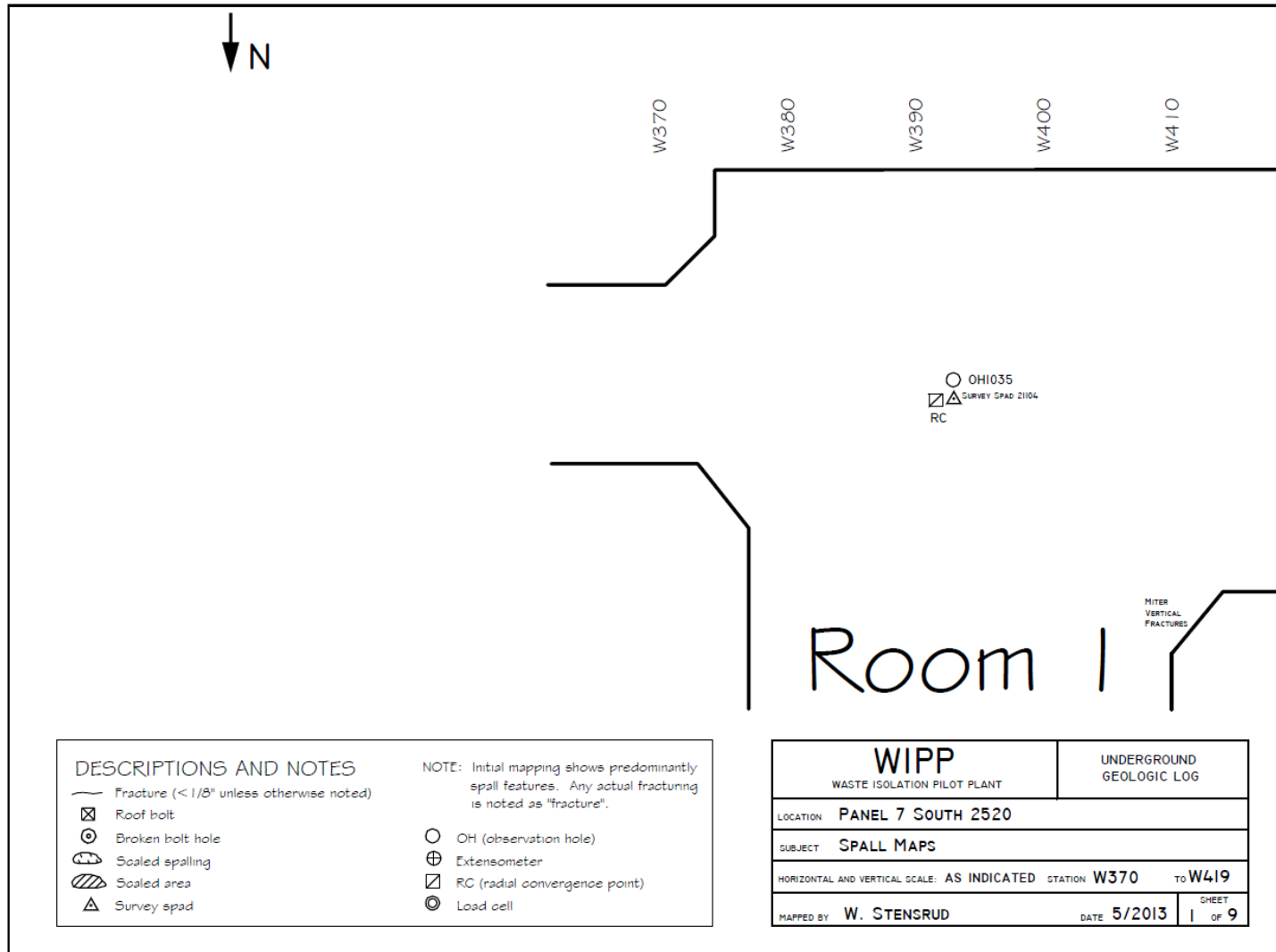
Figure 7-38 Panel 7 South 2520, W370-S419 Roof Fractures
