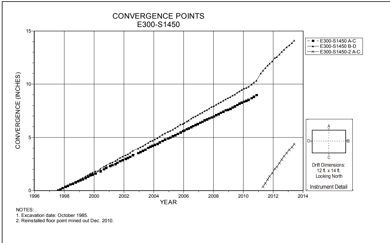
Figure 4-137 Convergence Point Array E300 S1450 – All Chords
