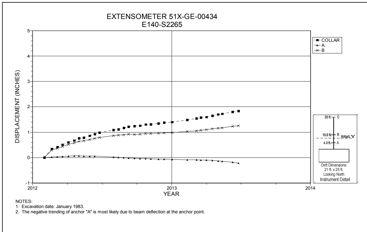
Figure 4-18 Extensometer 51X-GE-00434 E140 S2265 – Roof
