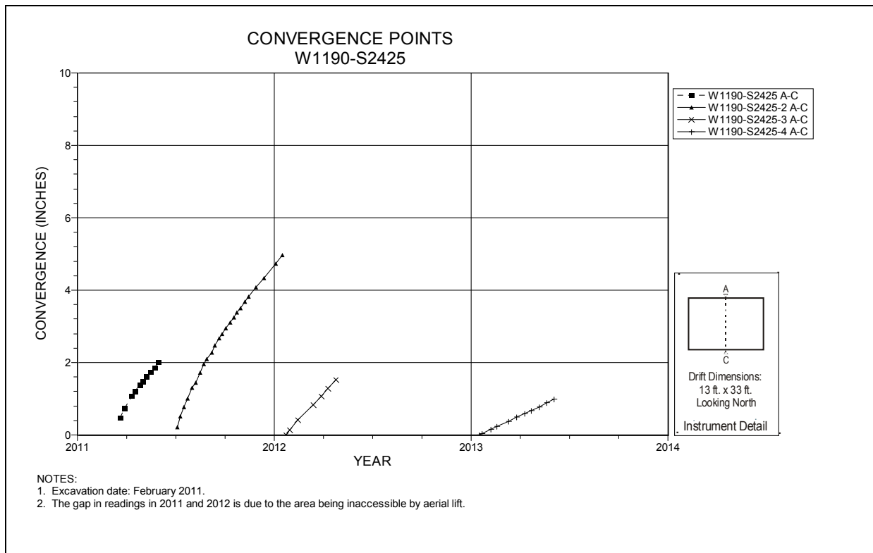
Figure 5-108 Convergence Point Array Room 7, Panel 7 at W1190 S2425 – Roof to Floor
