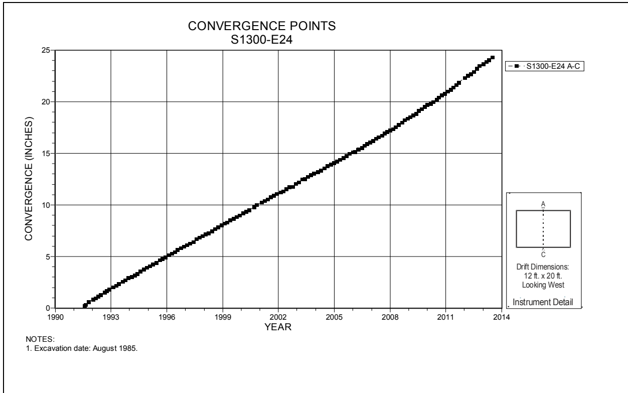
Figure 4-173 Convergence Point Array S1300 E24 – Roof to Floor
