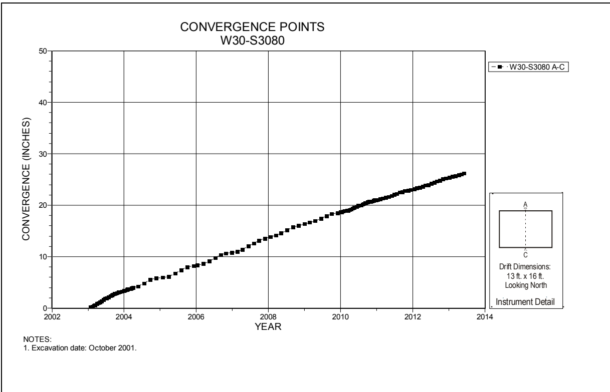
Figure 4-224 Convergence Point Array W30 S3080 – Roof to Floor
