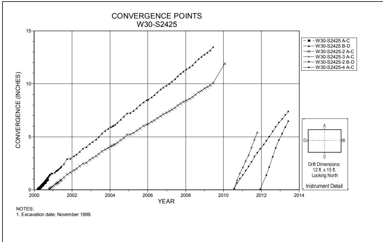
Figure 4-217 Convergence Point Array W30 S2425 – All Chords
