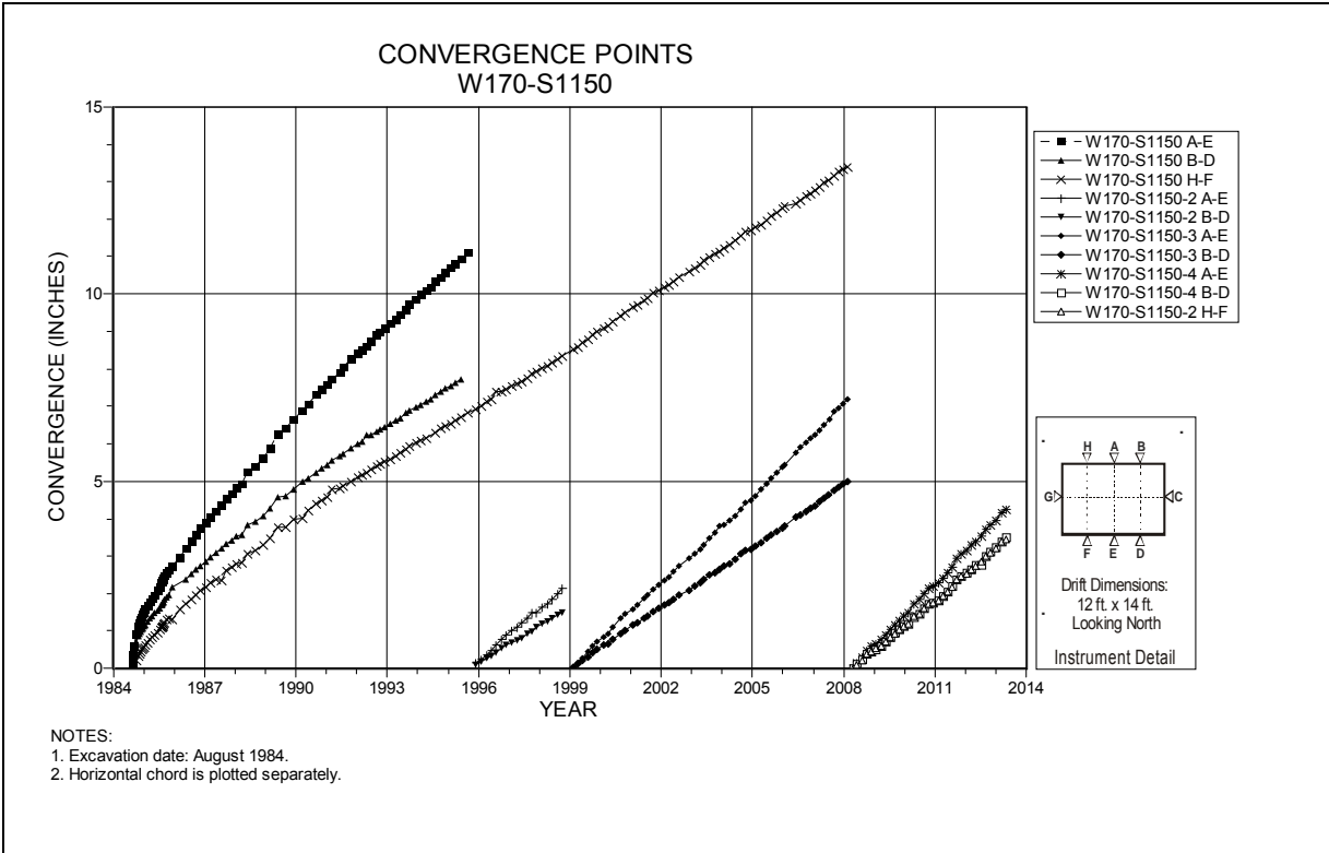
Figure 4-241 Convergence Point Array W170 S1150 – Roof to Floor
