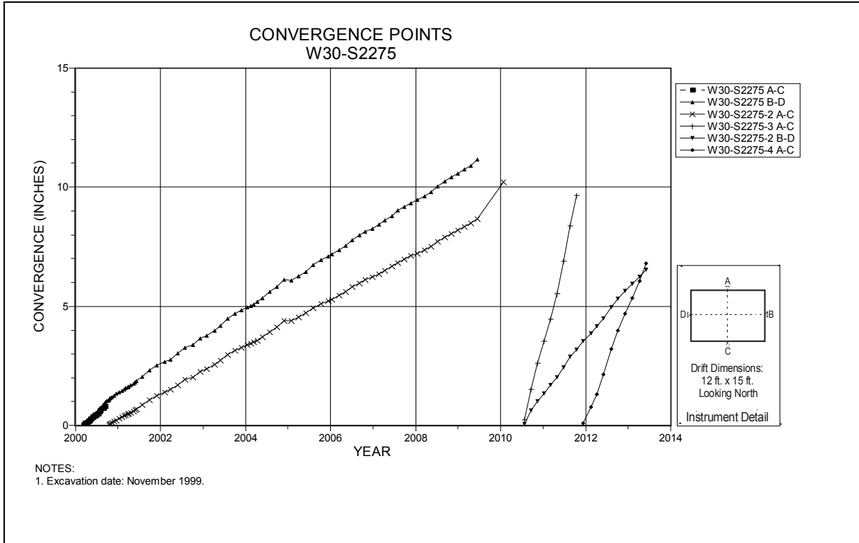
Figure 4-215 Convergence Point Array W30 S2275 – All Chords
