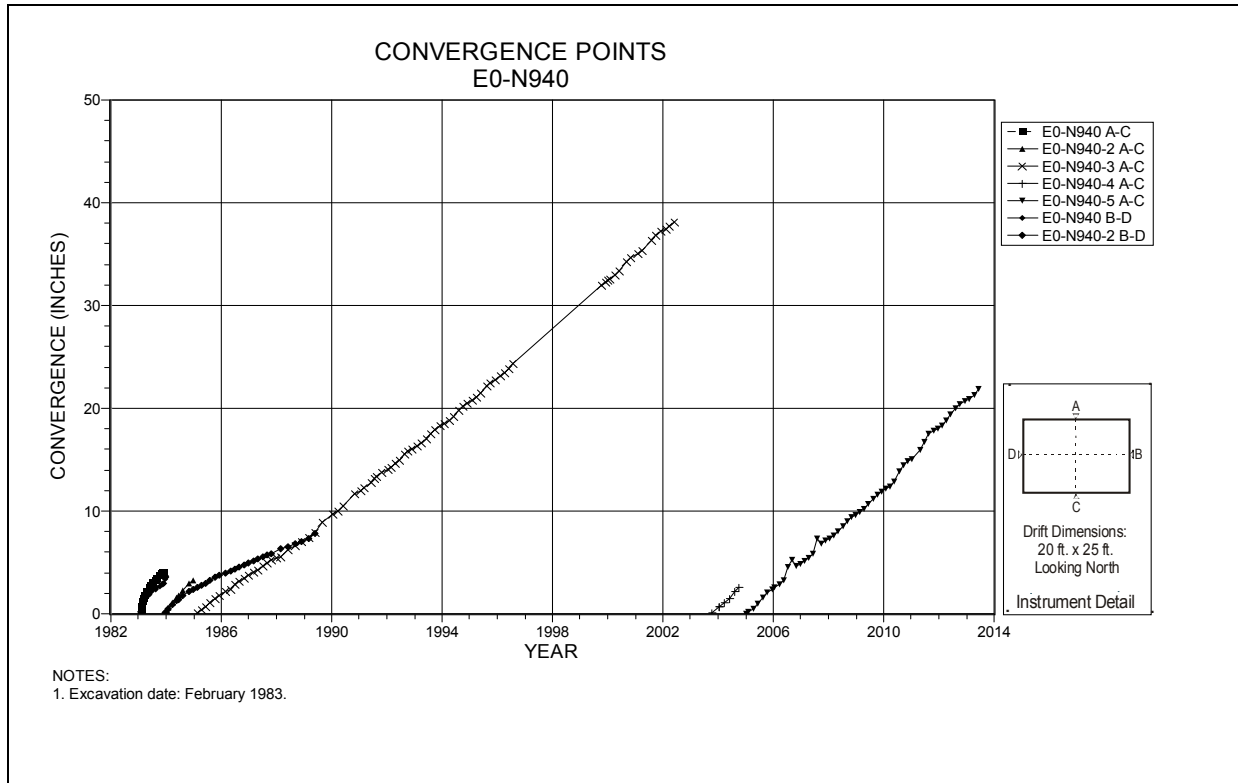
Figure 4-45 Convergence Point Array E0 N940 – All Chords
