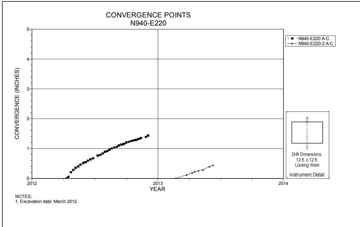
Figure 6-40 Convergence Point Array N940 E220 – Roof to Floor
