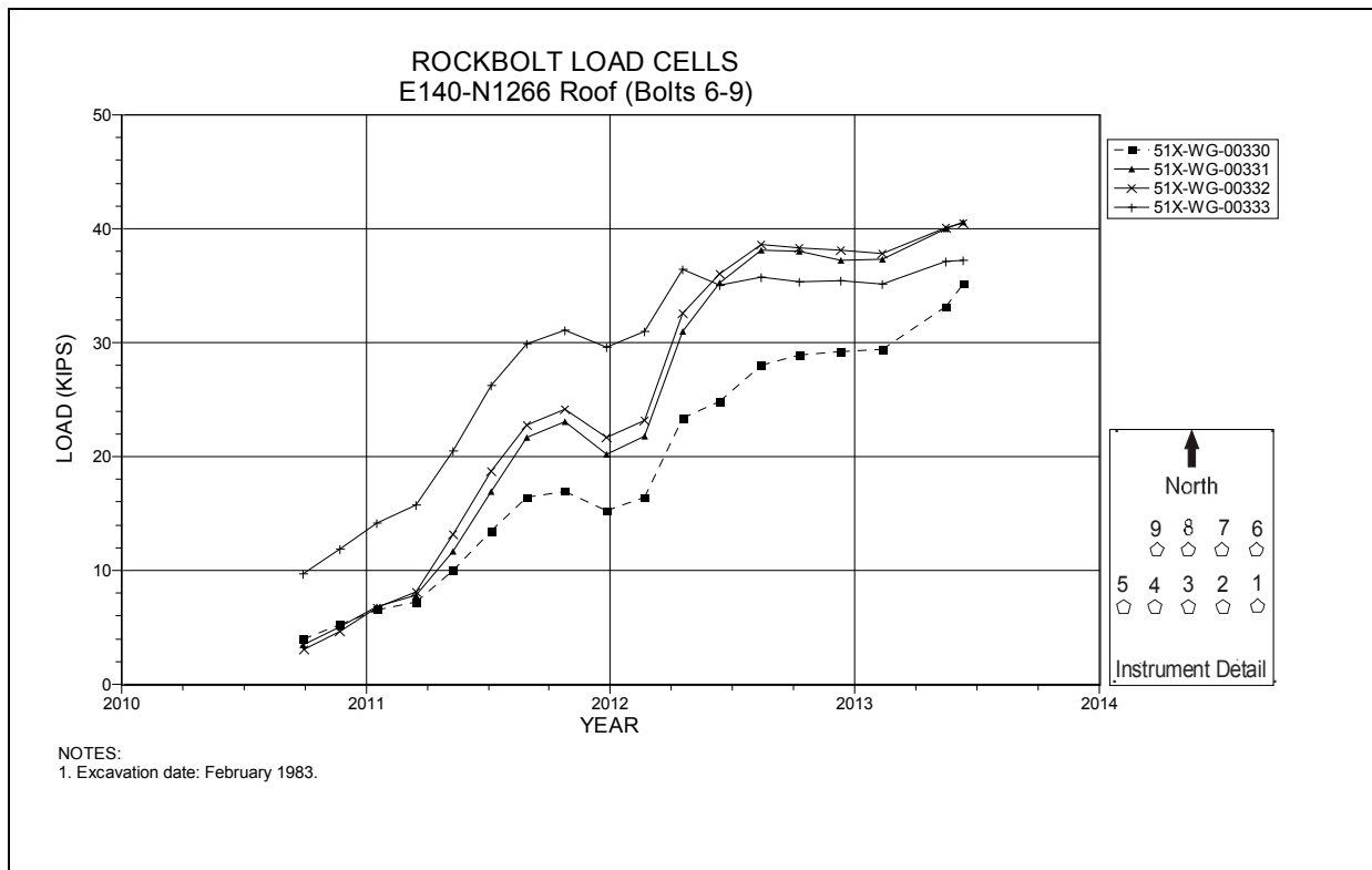
Figure 4-272 Rock Bolt Load Cells, Bolts 6-9 E140 N1266
