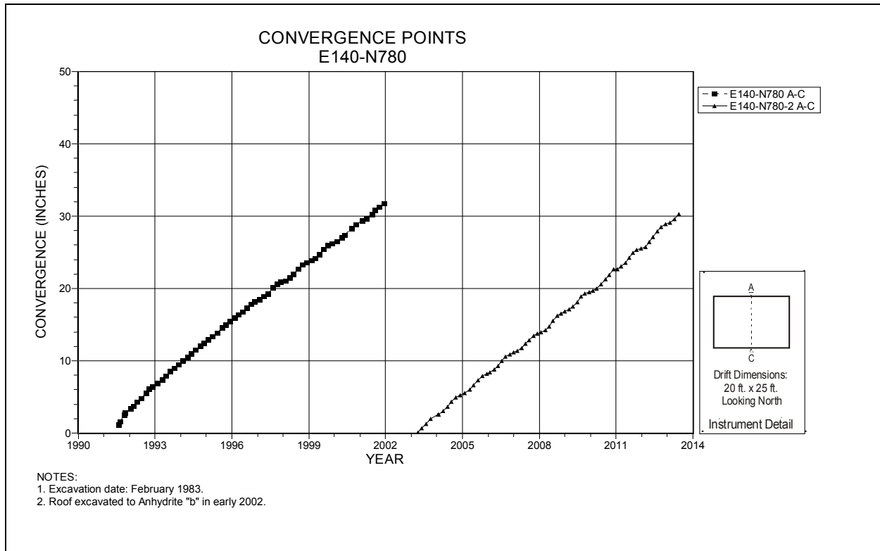
Figure 4-56 Convergence Point Array E140 N780 – Roof to Floor
