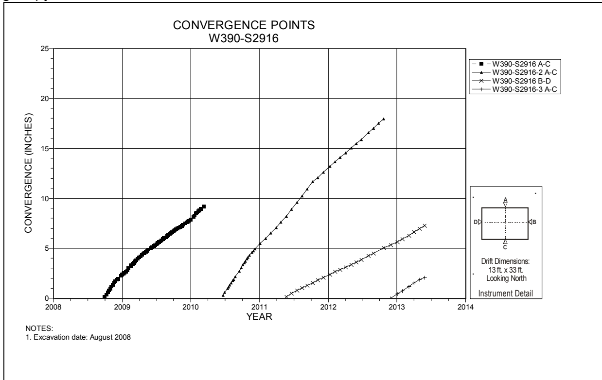
Figure 5-44 Convergence Point Array Room 1, Panel 6 at W390 S2916 – Room Center – All Chords
