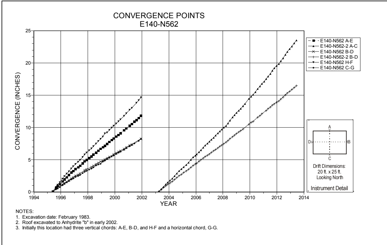
Figure 4-53 Convergence Point Array E140 N562 – All Chords
