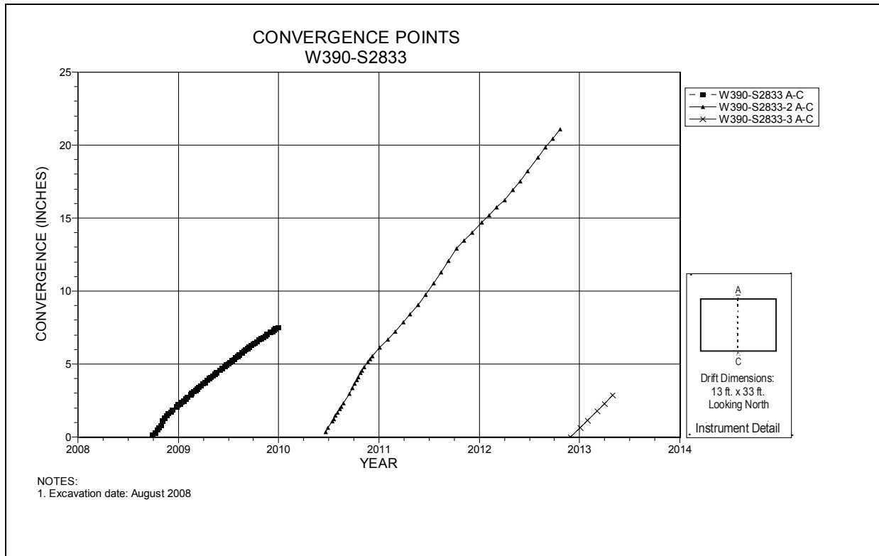
Figure 5-43 Convergence Point Array Room 1, Panel 6 at W390 S2833 – Roof to Floor
