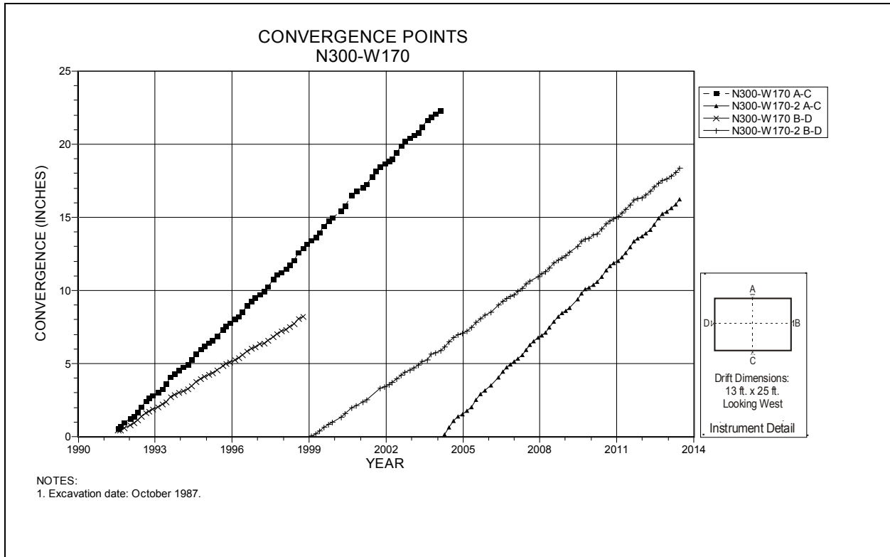
Figure 4-155 Convergence Point Array N300 W170 – All Chords
