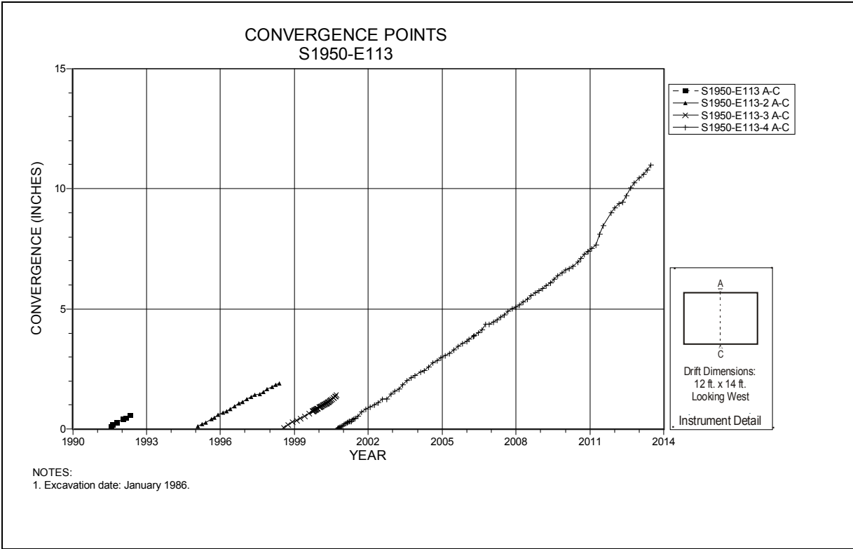
Figure 4-179 Convergence Point Array S1950 E113 – Roof to Floor
