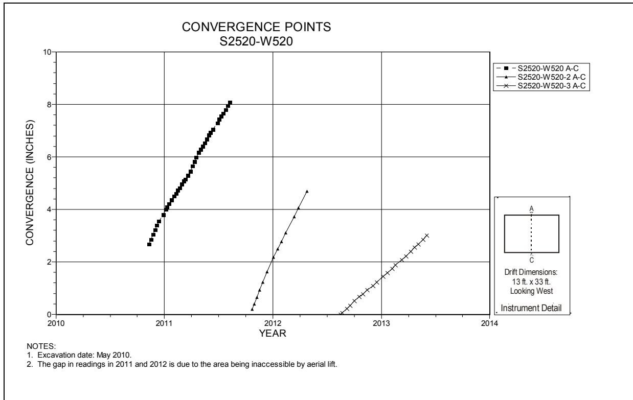
Figure 5-112 Convergence Point Array S2520 W520 Intersection (Room 2, Panel 7) – Roof to Floor
