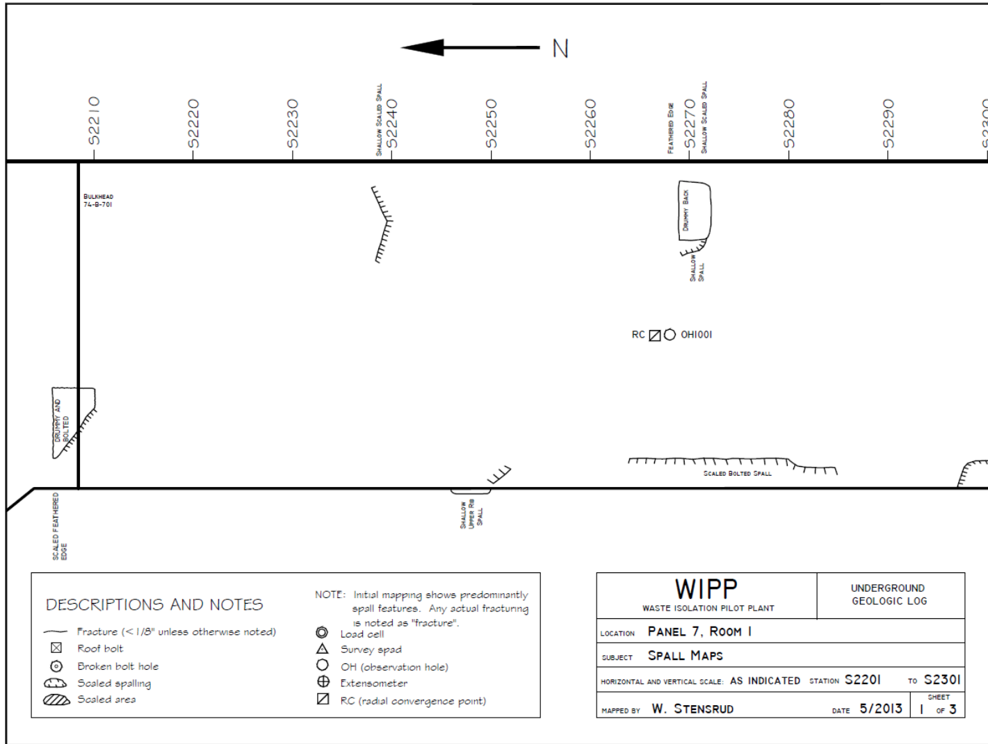
Figure 7-8 Panel 7 Room 1, S2201-S2301 Roof Fractures
