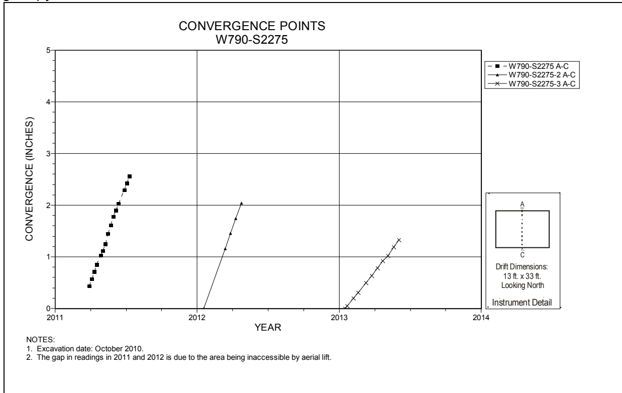
Figure 5-97 Convergence Point Array Room 4, Panel 7 at W790 S2275 – Roof to Floor
