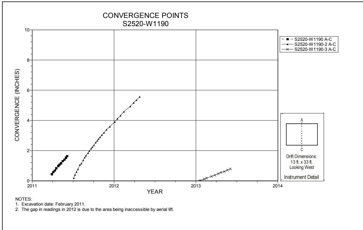
Figure 5-122 Convergence Point Array S2520 W1190 Intersection (Room 7, Panel 7) – Roof to Floor
