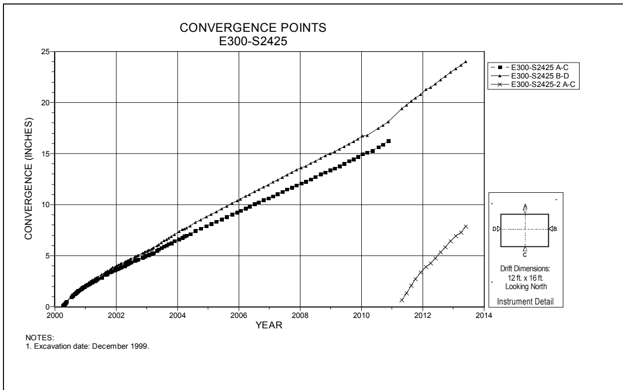
Figure 4-144 Convergence Point Array E300 S2425 – All Chords
