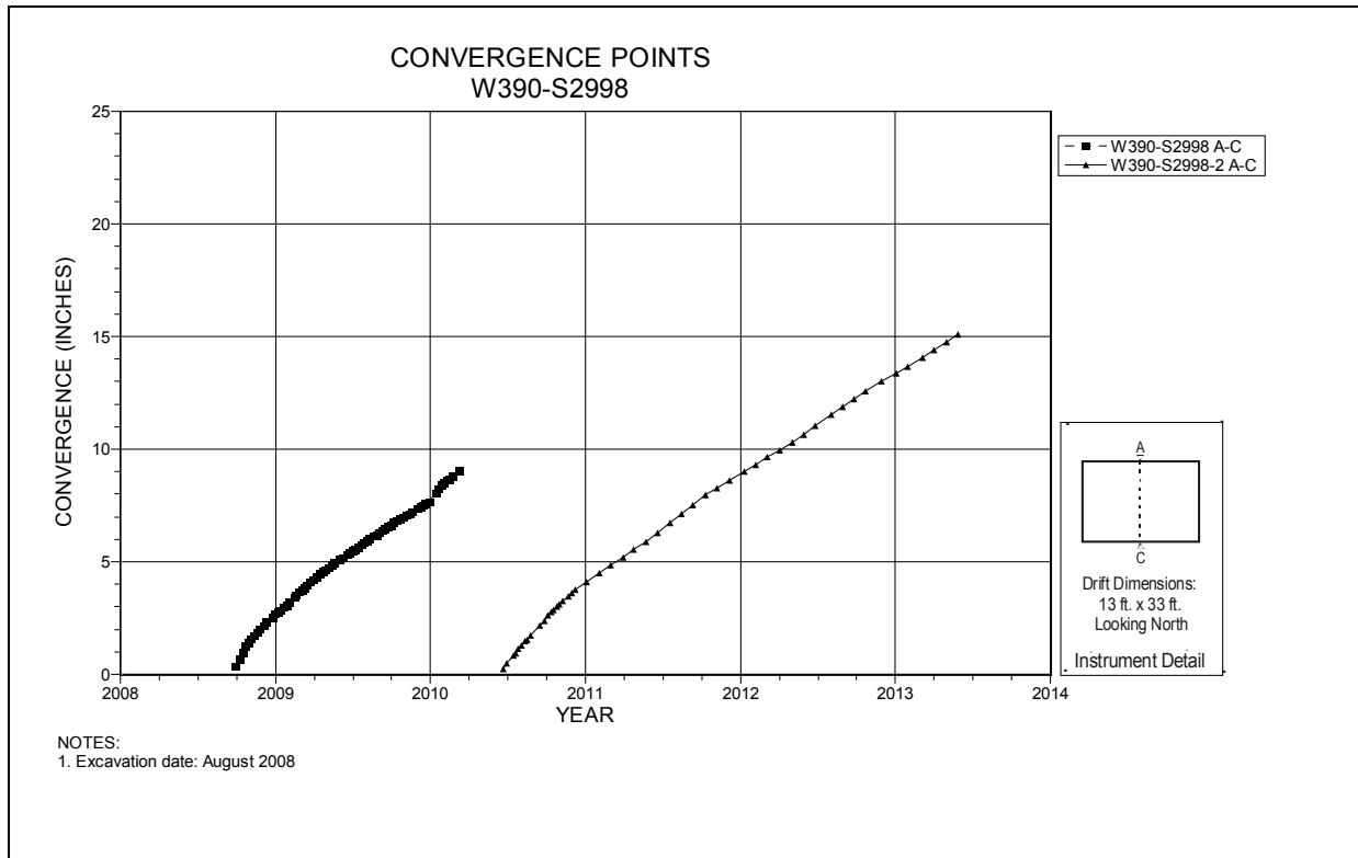
Figure 5-45 Convergence Point Array Room 1, Panel 6 at W390 S2998 – Roof to Floor
