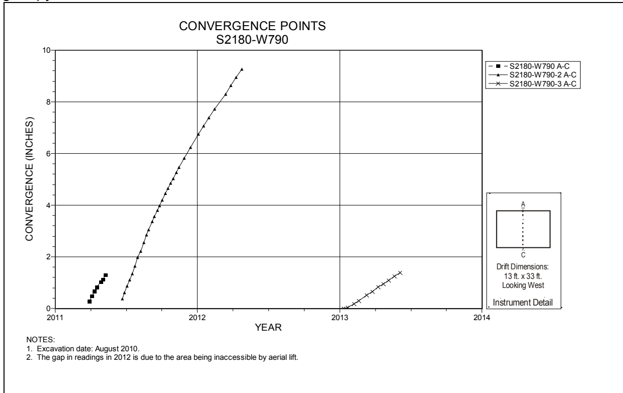
Figure 5-81 Convergence Point Array S2180 W790 Intersection (Room 4, Panel 7) – Roof to Floor
