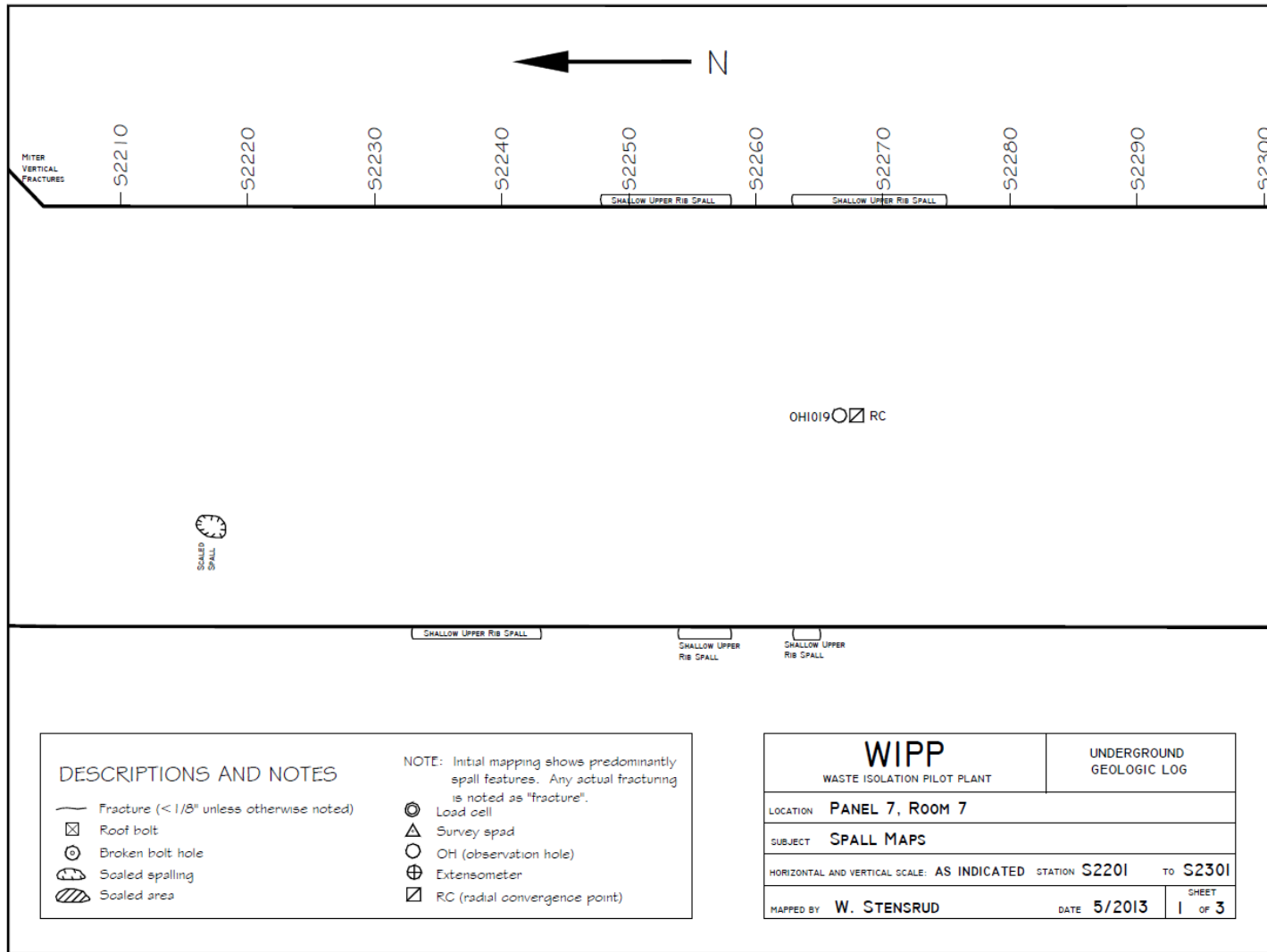
Figure 7-26 Panel 7 Room 7, S2201-S2301 Roof Fractures
