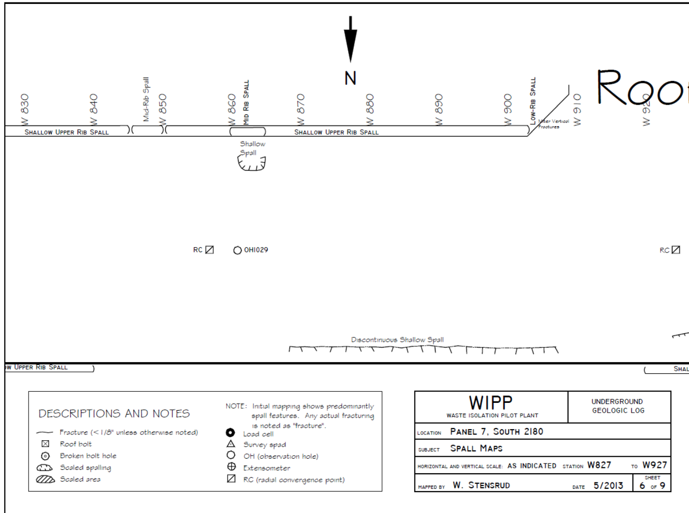
Figure 7-34 Panel 7 South 2180, W827-W927 Roof Fractures
