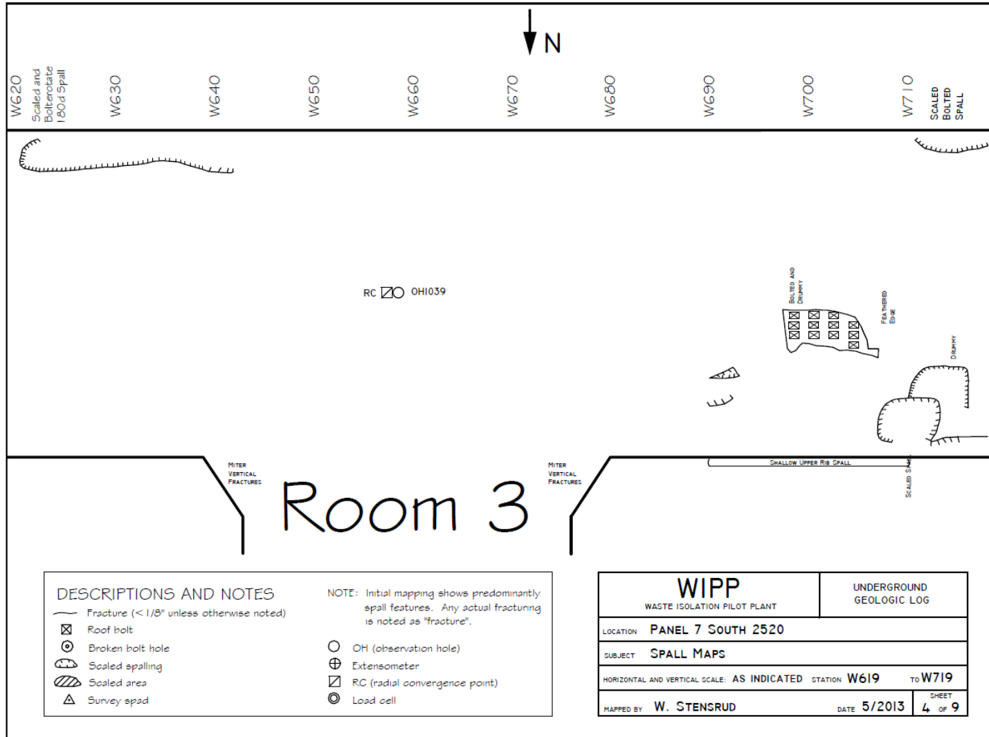
Figure 7-41 Panel 7 South 2520, W619-W719 Roof Fractures
