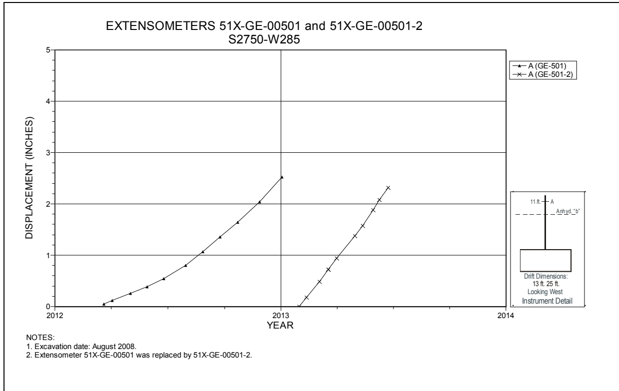
Figure 4-33 Extensometers 51X-GE-00501 and 51X-GE-00501-2 S2750 W285 – Roof
