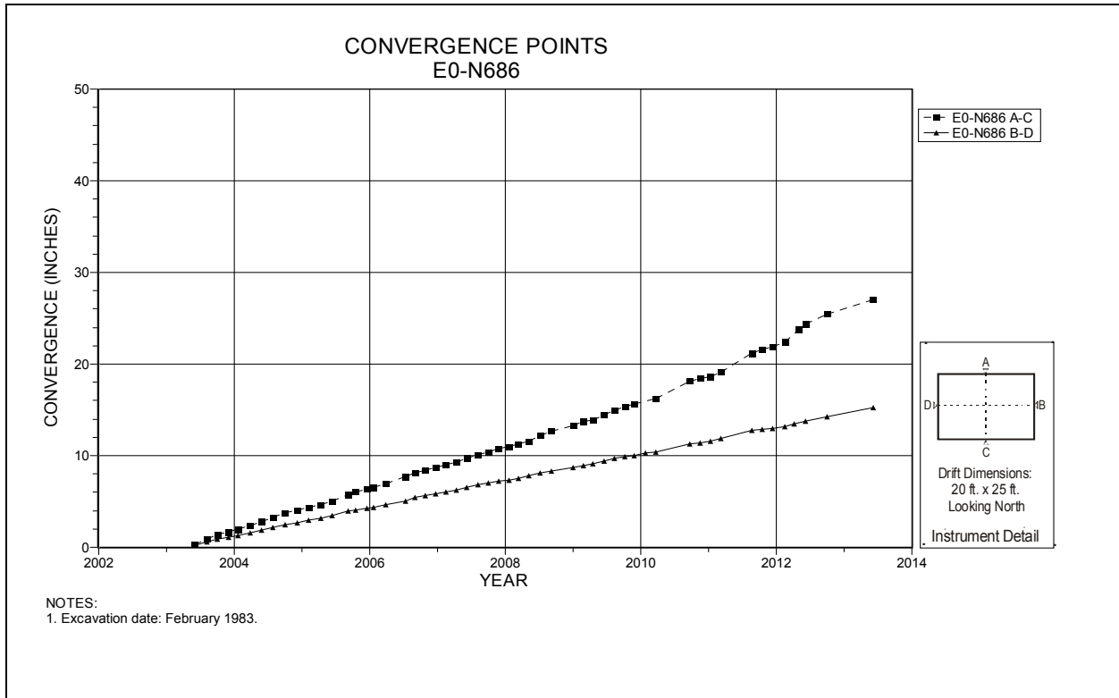
Figure 4-43 Convergence Point Array E0 N686 – All Chords
