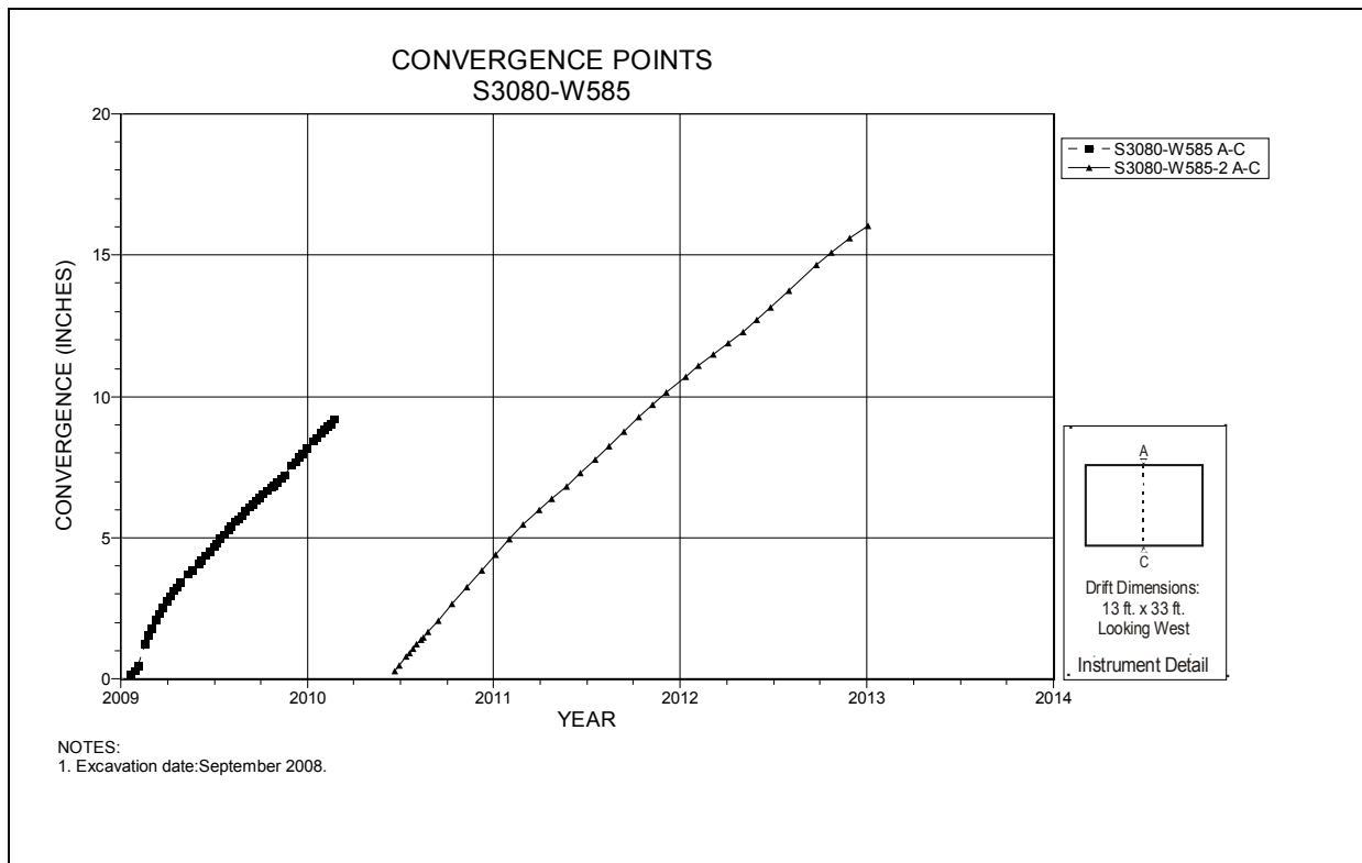
Figure 5-59 Convergence Point Array S3080 W585 – Roof to Floor
