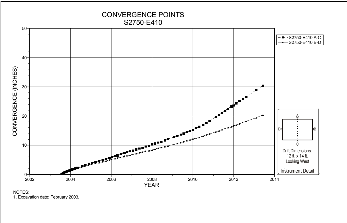
Figure 4-189 Convergence Point Array S2750 E410 – All Chords
