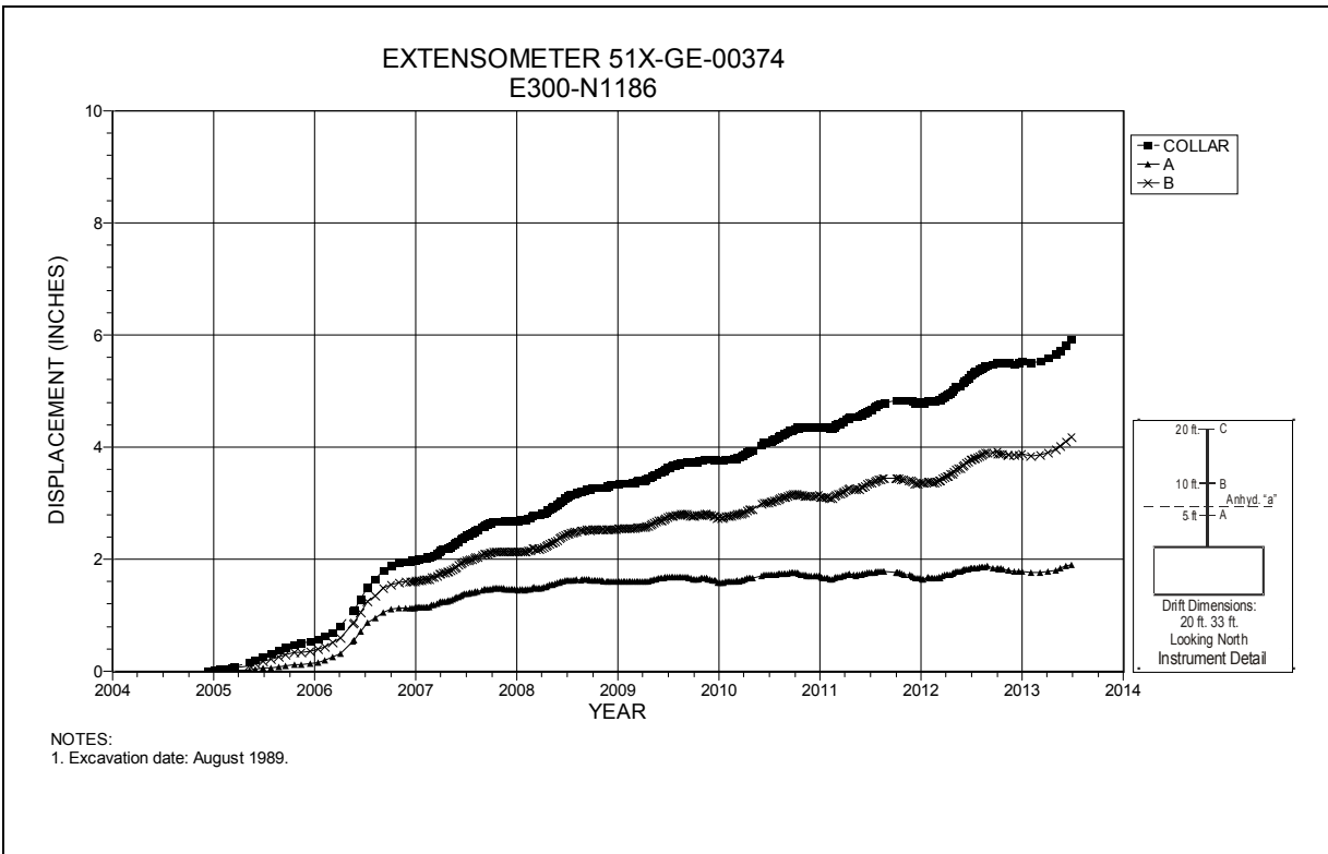
Figure 4-26 Extensometer 51X-GE-00374 E300 N1186 – Roof
