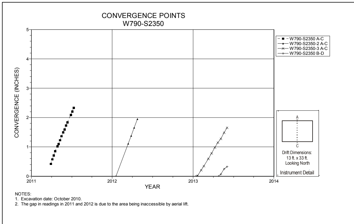
Figure 5-98 Convergence Point Array Room 4, Panel 7 at W790 S2350 – Room Center – All Chords
