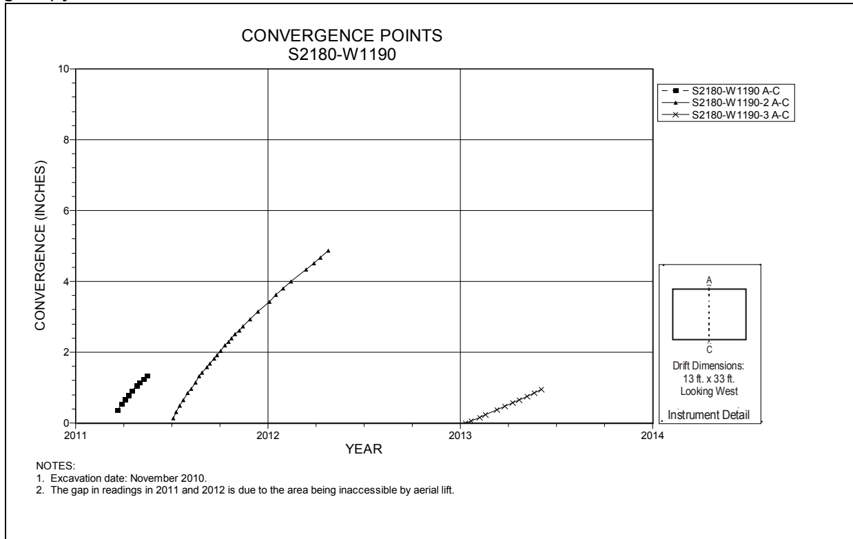
Figure 5-87 Convergence Point Array S2180 W1190 Intersection (Room 7, Panel 7) – Roof to Floor
