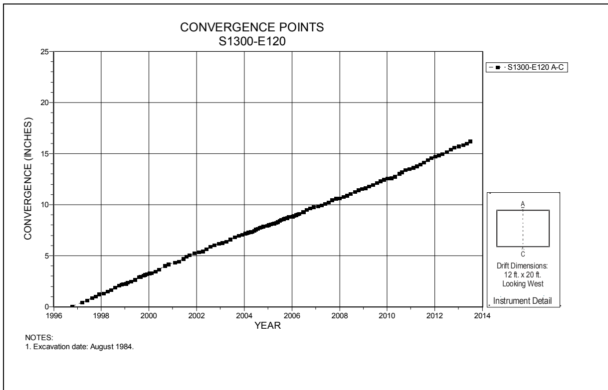
Figure 4-174 Convergence Point Array S1300 E120 – Roof to Floor
