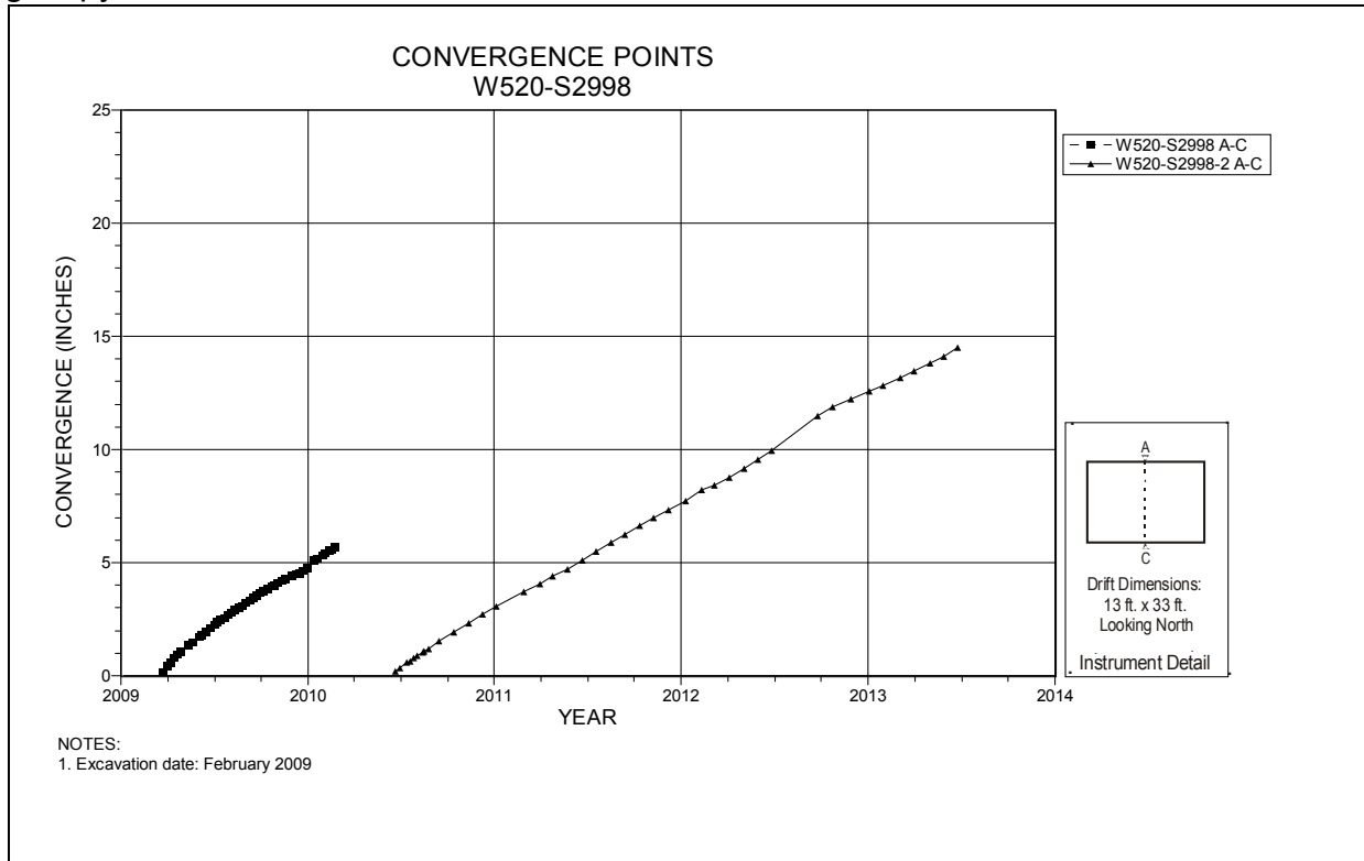
Figure 5-48 Convergence Point Array Room 2, Panel 6 at W520 S2998 – Roof to Floor
