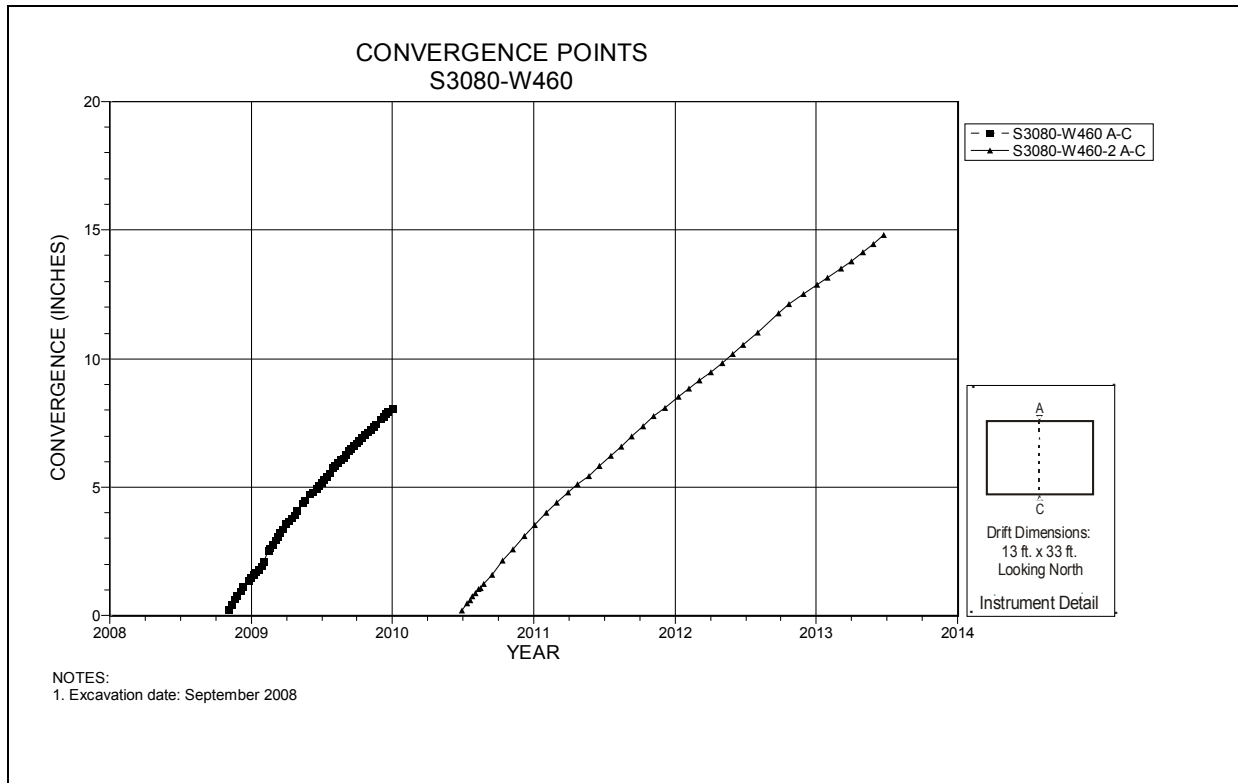
Figure 5-57 Convergence Point Array S3080 W460 – Roof to Floor
