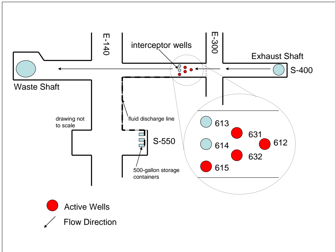
Figure 3 - 1 Location of Interception Wells and Storage Containers
