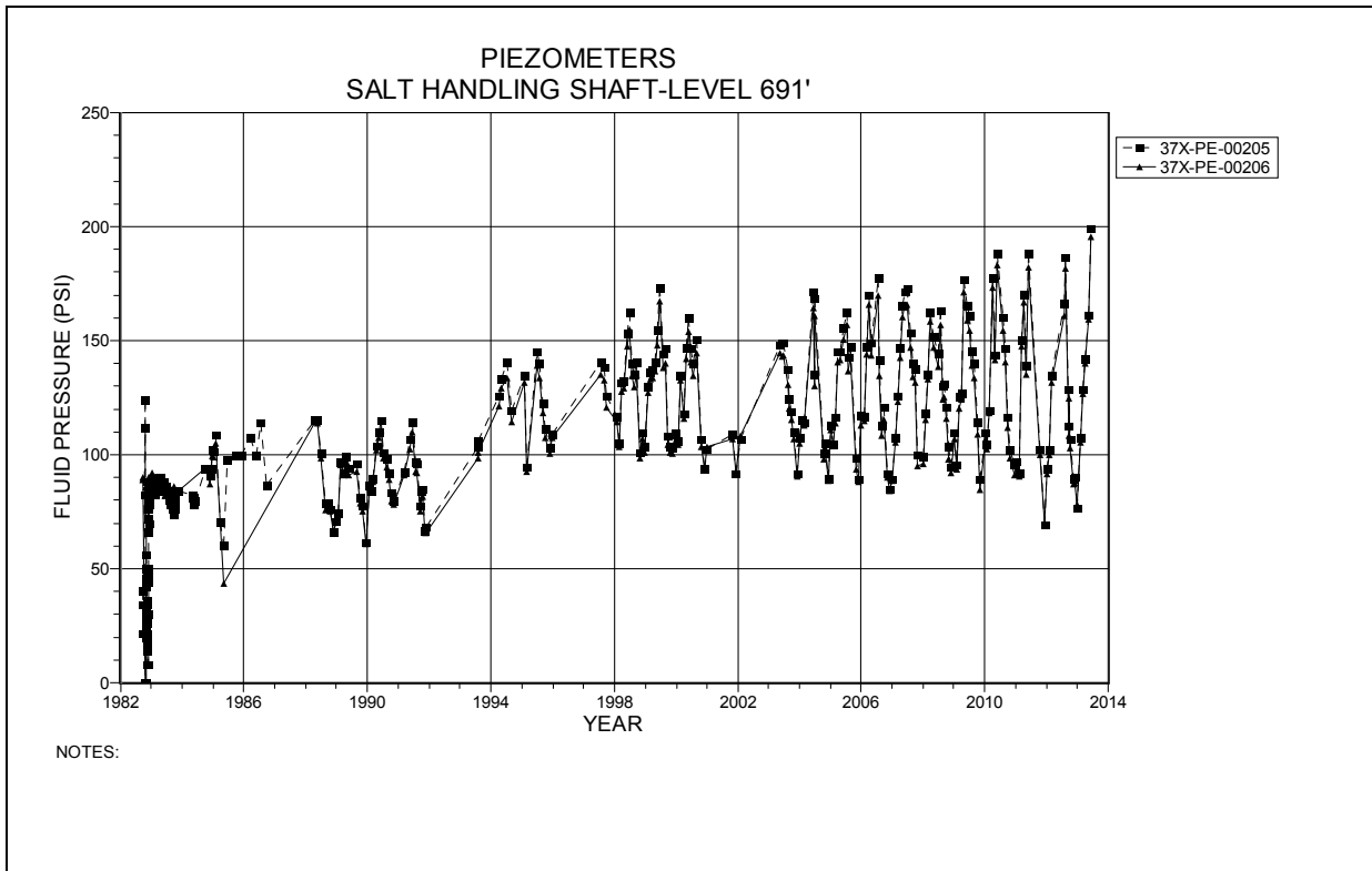
Figure 2-3 Piezometers Salt Handling Shaft – Level 691 at the Tamarisk Member
