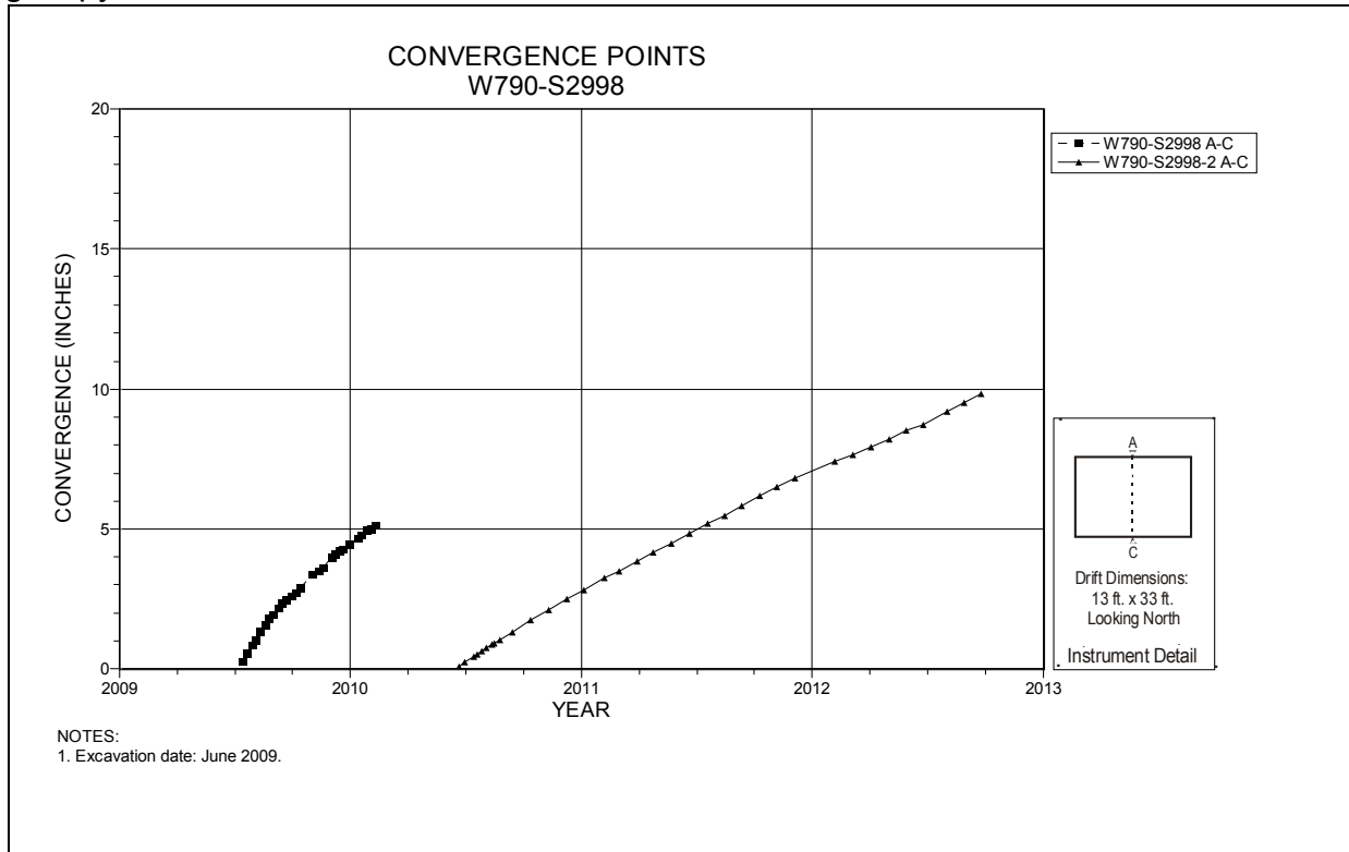
Figure 5-54 Convergence Point Array Room 4, Panel 6 at W790 S2998 – Roof to Floor
