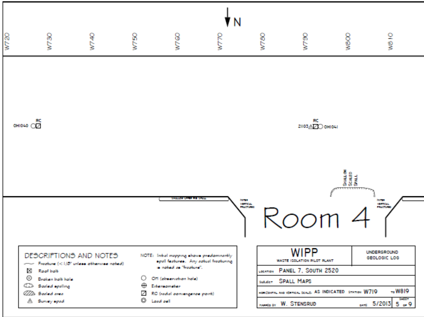
Figure 7-42 Panel 7 South 2520, W719-W819 Roof Fractures
