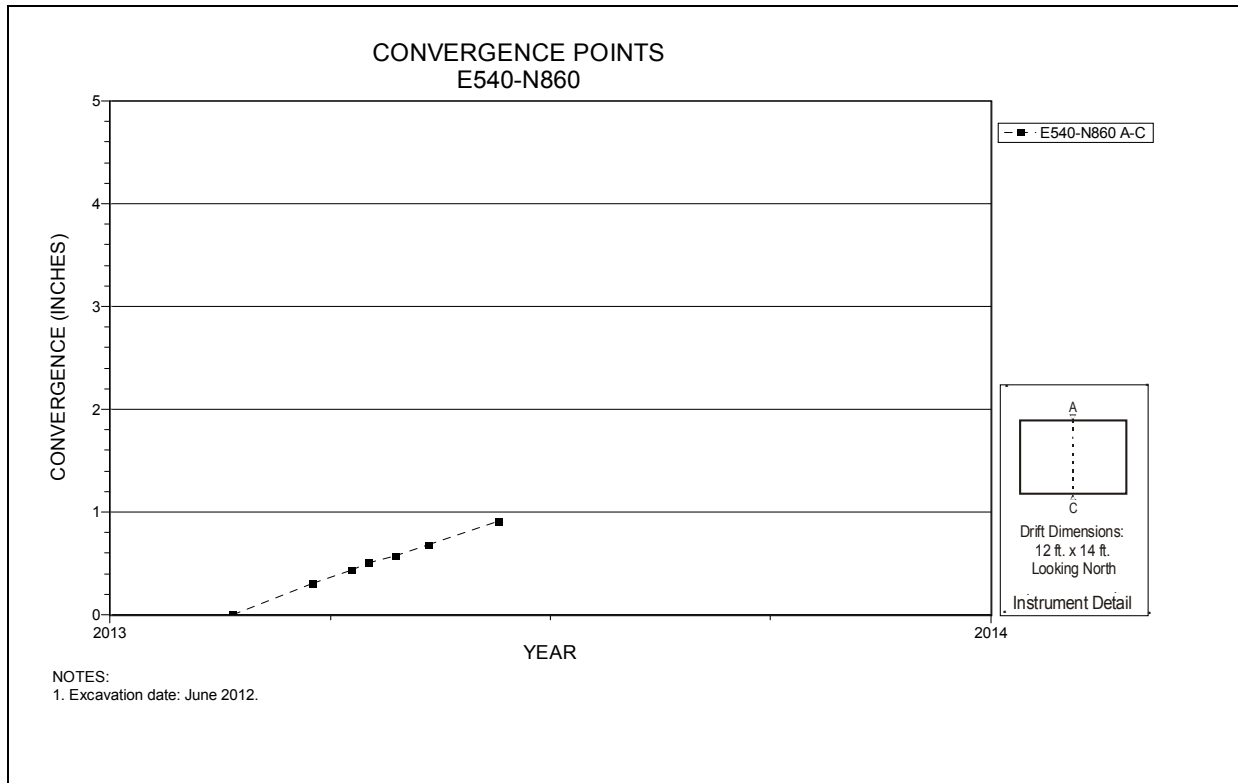
Figure 6-13 Convergence Point Array E540 N860 – Roof to Floor
