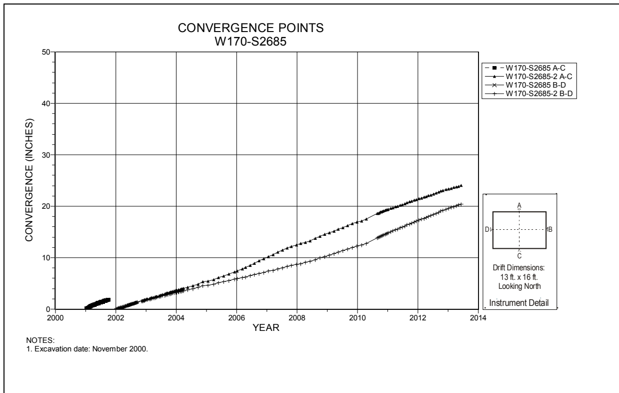
Figure 4-254 Convergence Point Array W170 S2685 – All Chords
