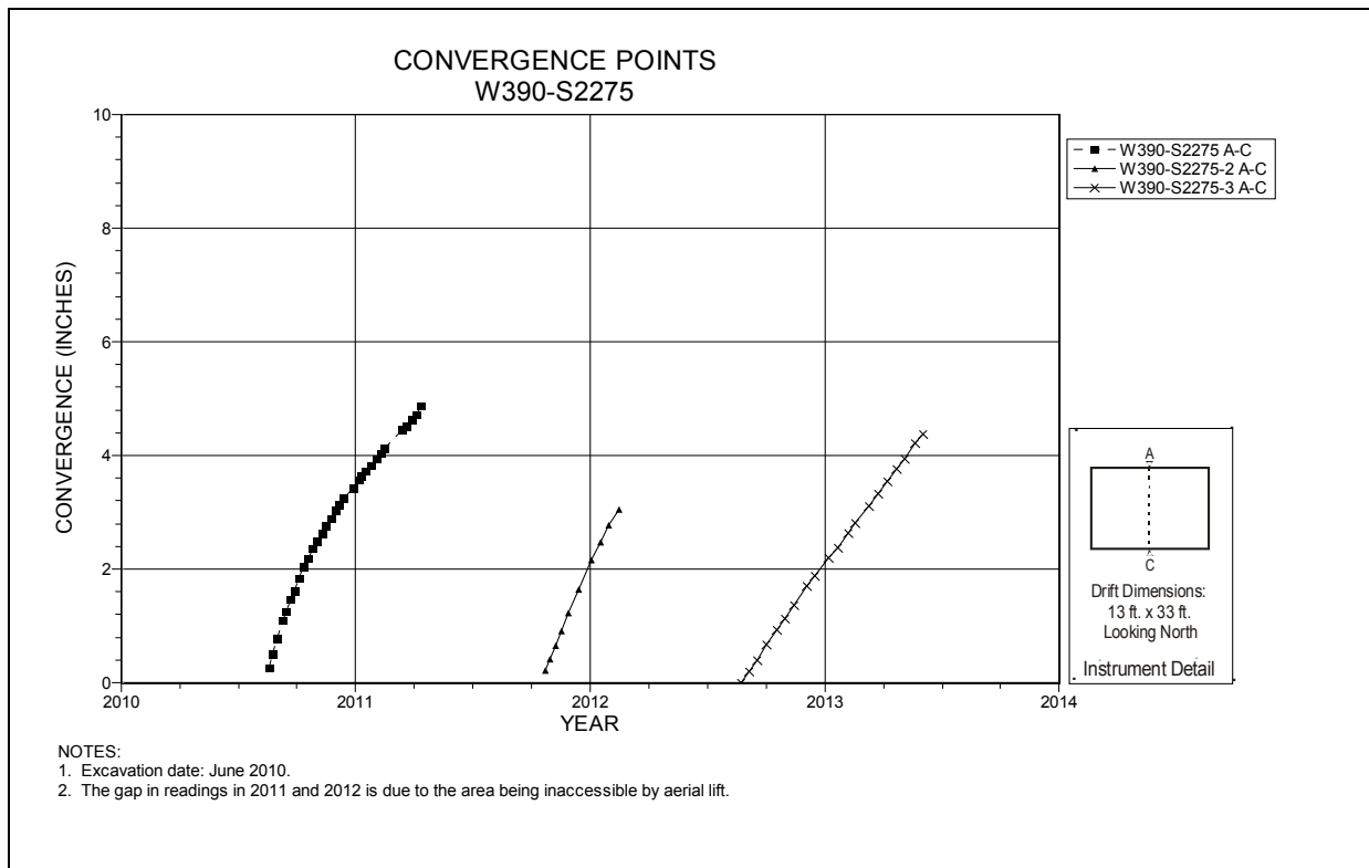
Figure 5-88 Convergence Point Array Room 1, Panel 7 at W390 S2275 – Roof to Floor
