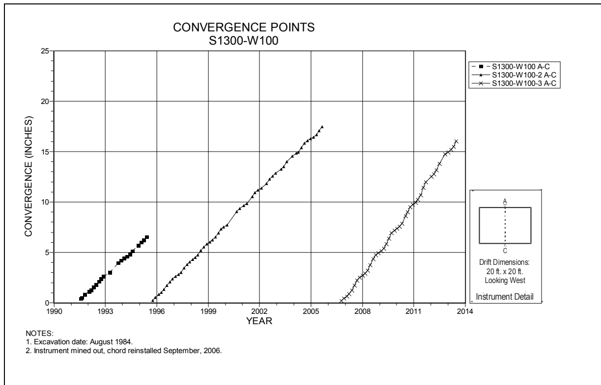
Figure 4-176 Convergence Point Array S1300 W100 – Roof to Floor
