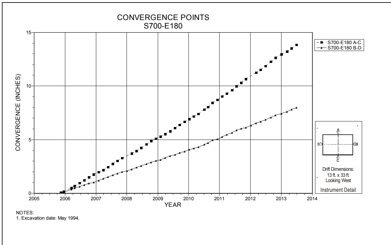
Figure 4-166 Convergence Point Array S700 E180 – All Chords
