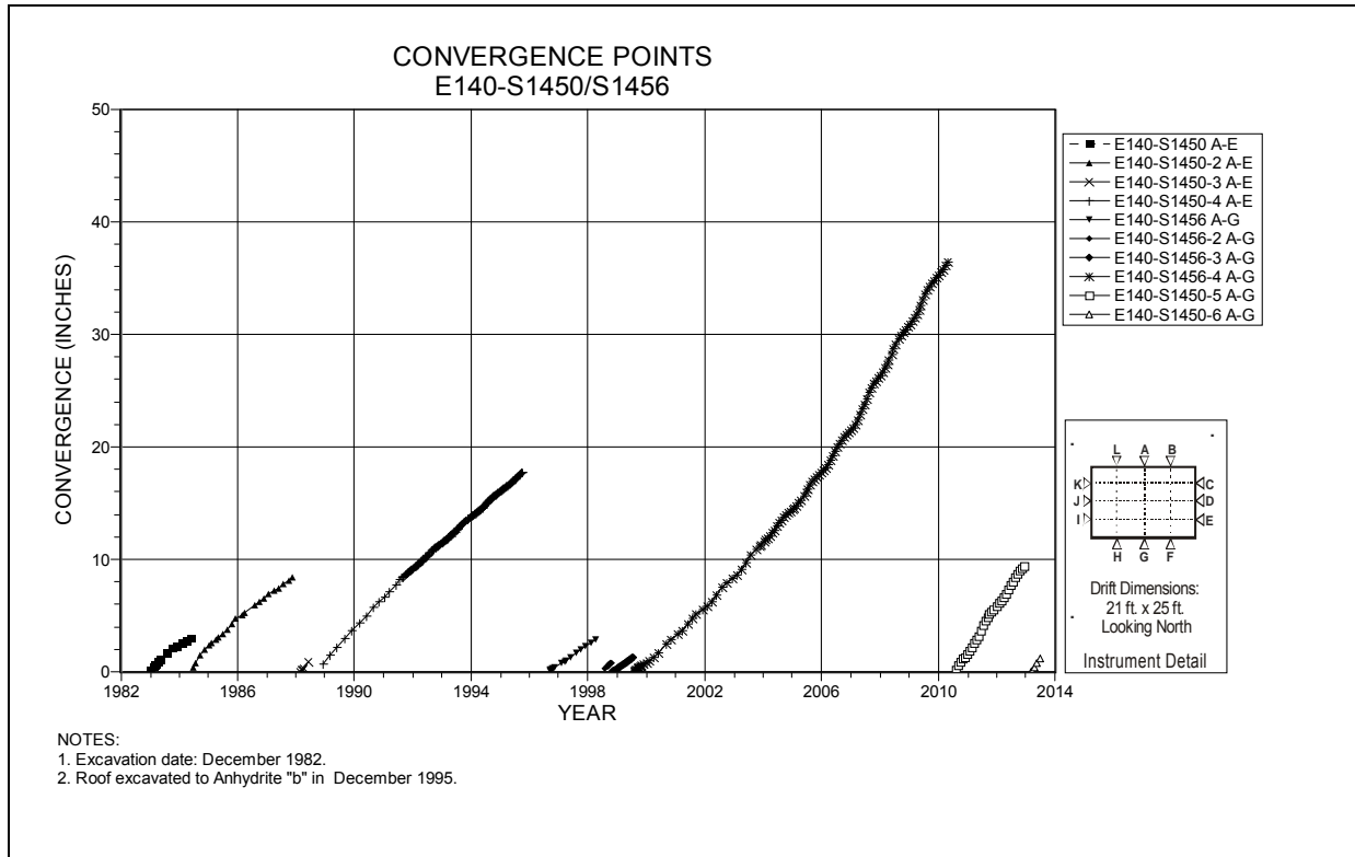
Figure 4-85 Convergence Point Array E140 S1450/S1456 – Roof to Floor – Centerline
