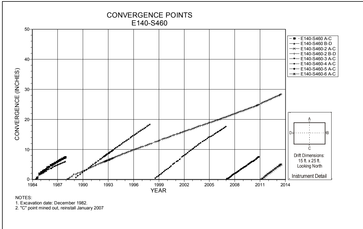
Figure 4-63 Convergence Point Array E140 S460 – All Chords
