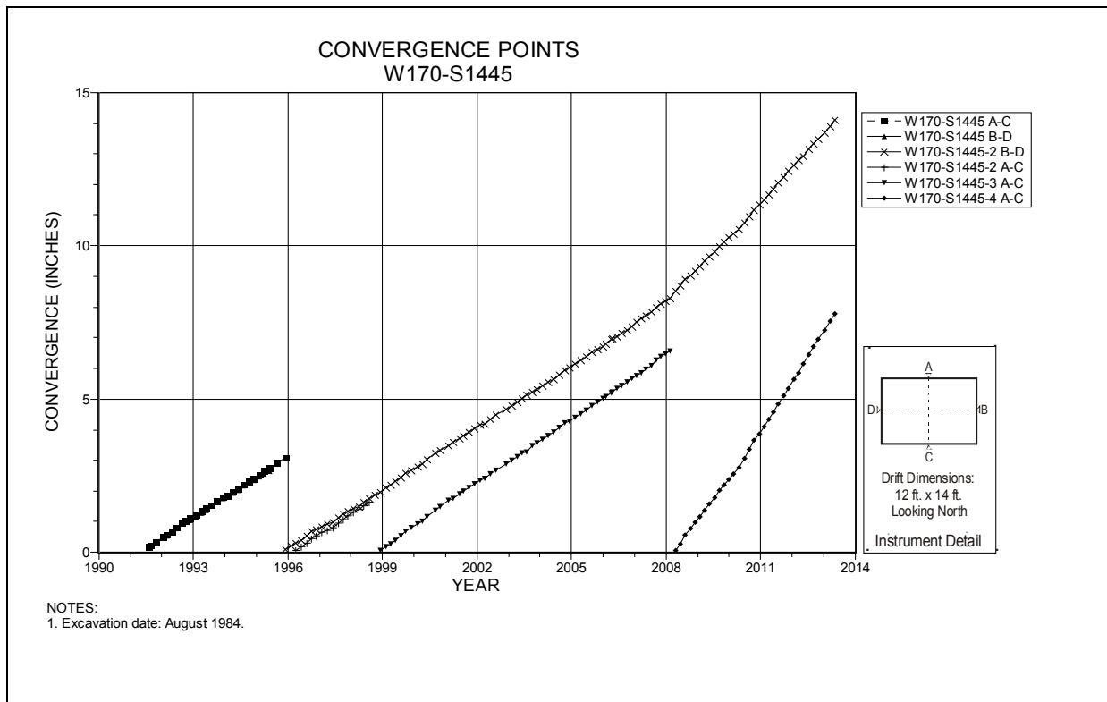
Figure 4-244 Convergence Point Array W170 S1445 – All Chords
