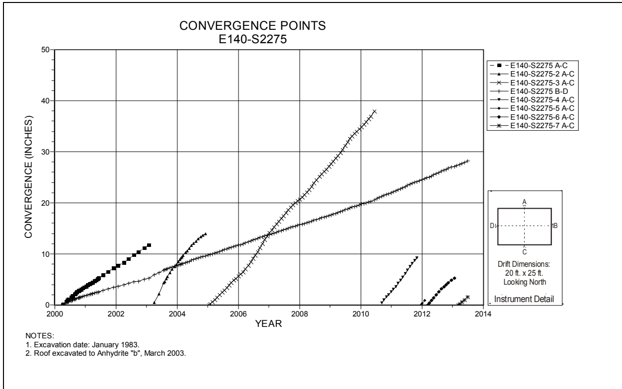
Figure 4-105 Convergence Point Array E140 S2275 – All Chords
