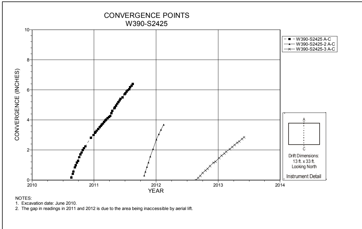
Figure 5-90 Convergence Point Array Room 1, Panel 7 at W390 S2425 – Roof to Floor
