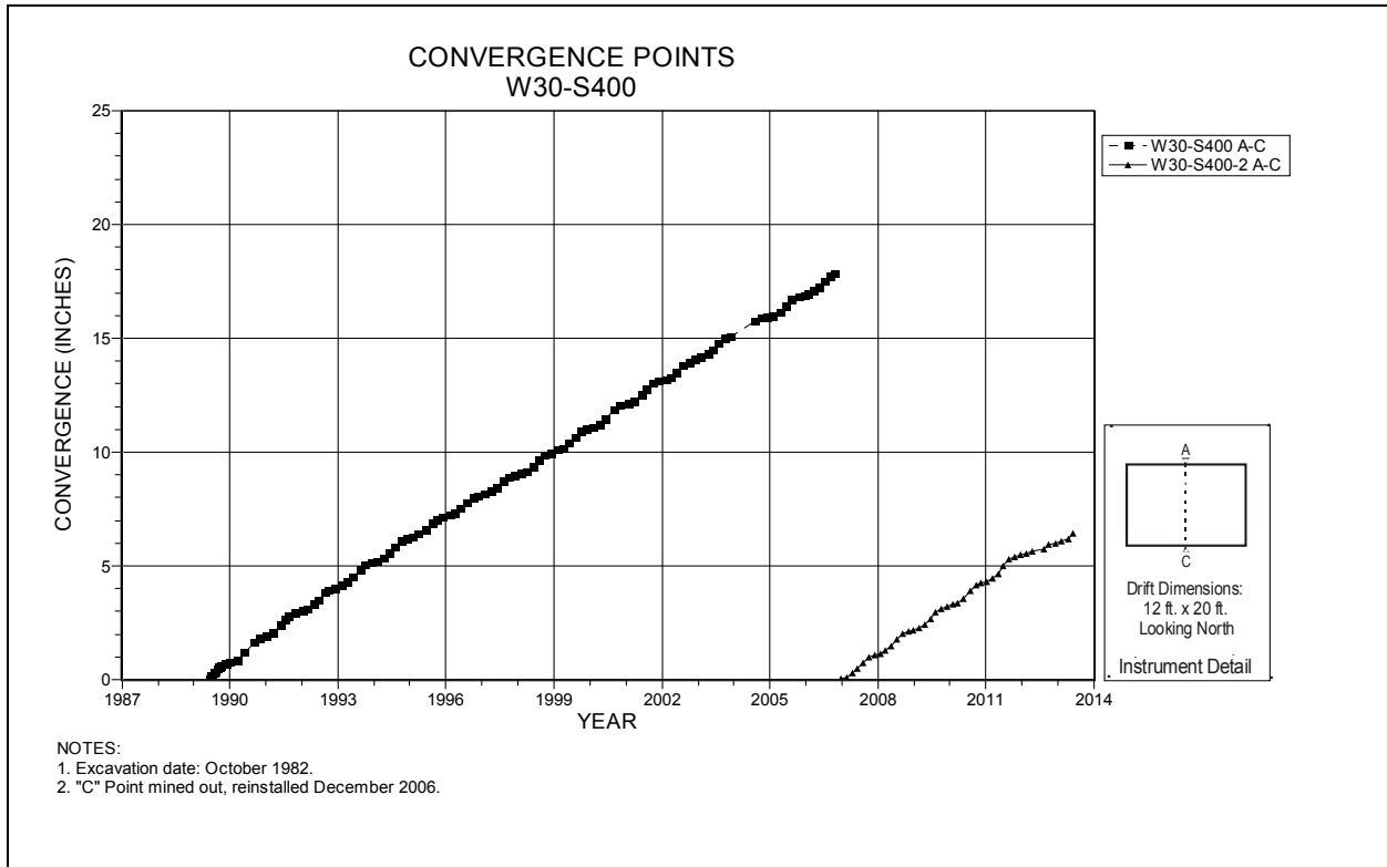
Figure 4-201 Convergence Point Array W30 S400 – Roof to Floor
