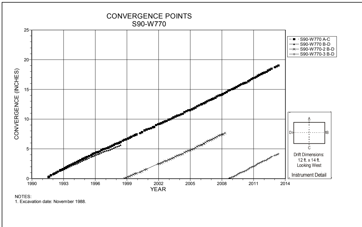
Figure 4-162 Convergence Point Array S90 W770 – All Chords
