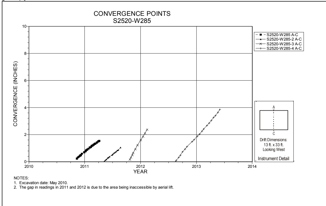
Figure 5-109 Convergence Point Array S2520 W285 – Roof to Floor
