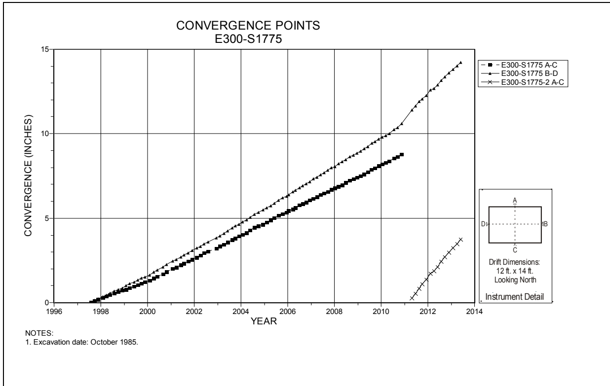
Figure 4-139 Convergence Point Array E300 S1775 – All Chords
