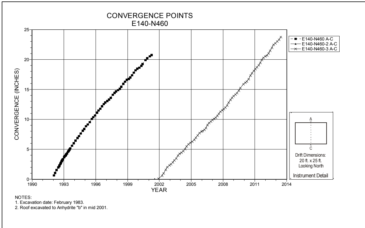
Figure 4-52 Convergence Point Array E140 N460 – Roof to Floor
