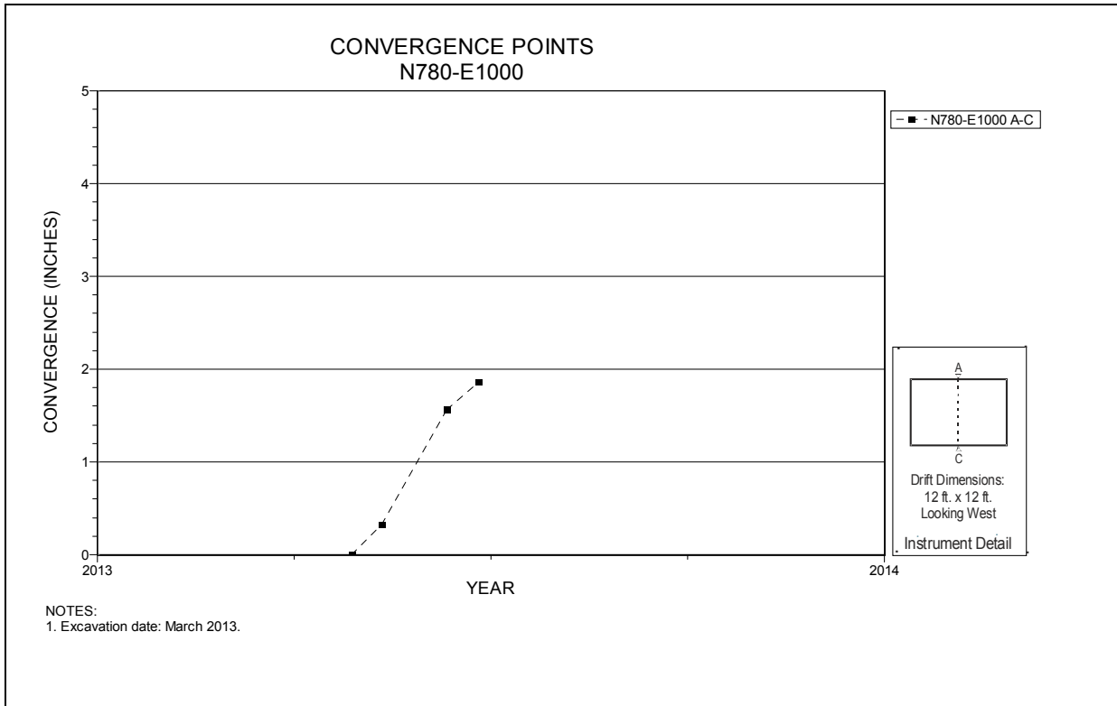
Figure 6-34 Convergence Point Array N780 E1000 – Roof to Floor
