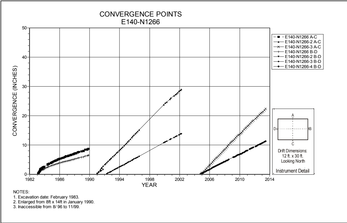
Figure 4-59 Convergence Point Array E140 N1266 – All Chords
