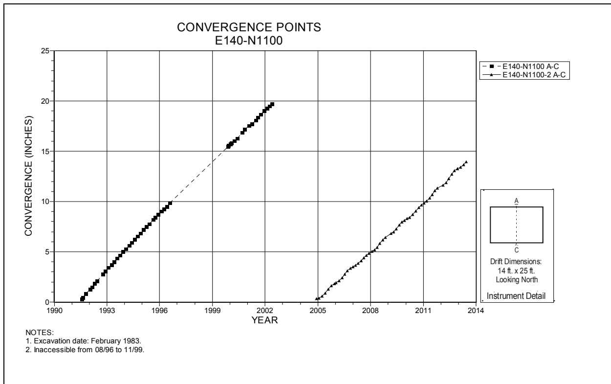
Figure 4-58 Convergence Point Array E140 N1100 – Roof to Floor
