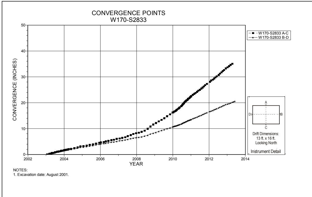
Figure 4-255 Convergence Point Array W170 S2833 – All Chords
