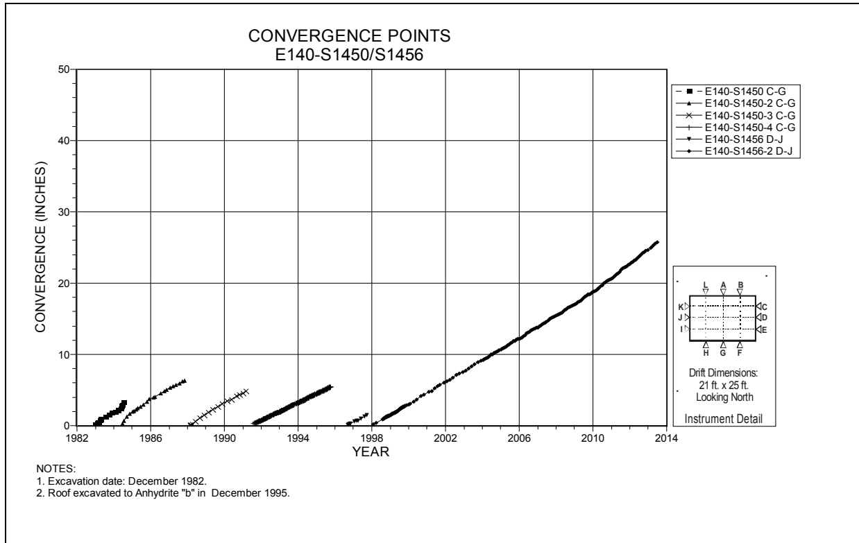
Figure 4-89 Convergence Point Array E140 S1450/S1456 – Rib to Rib – Mid-Height
