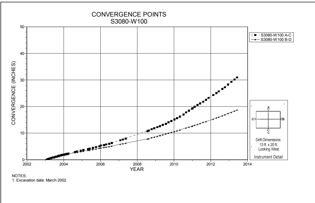
Figure 4-192 Convergence Point Array S3080 W100 – All Chords
