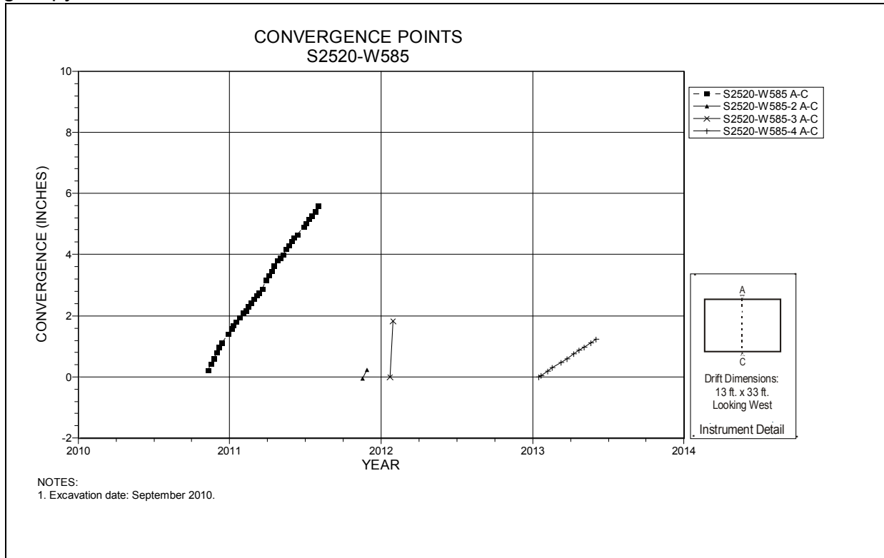
Figure 5-113 Convergence Point Array S2520 W585 – Roof to Floor
