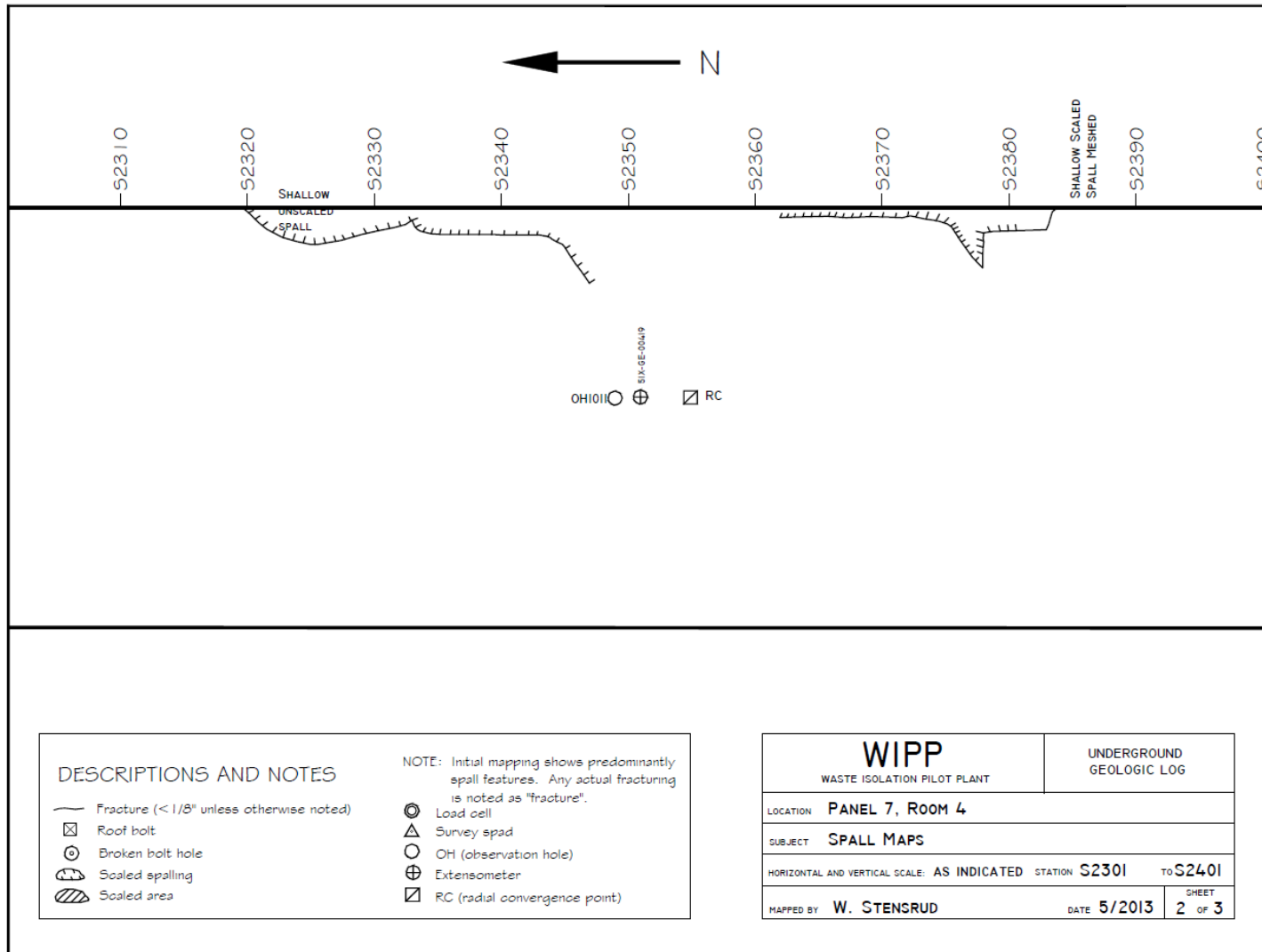
Figure 7-18 Panel 7 Room 4, S2301-S2401 Roof Fractures
