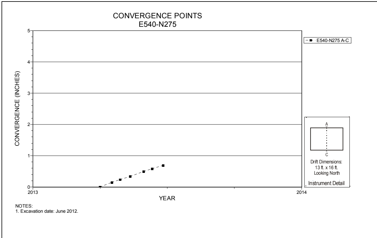
Figure 6-6 Convergence Point Array E540 N275 – Roof to Floor
