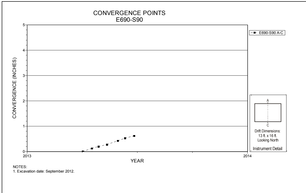
Figure 6-15 Convergence Point Array E690 S90 – Roof to Floor
