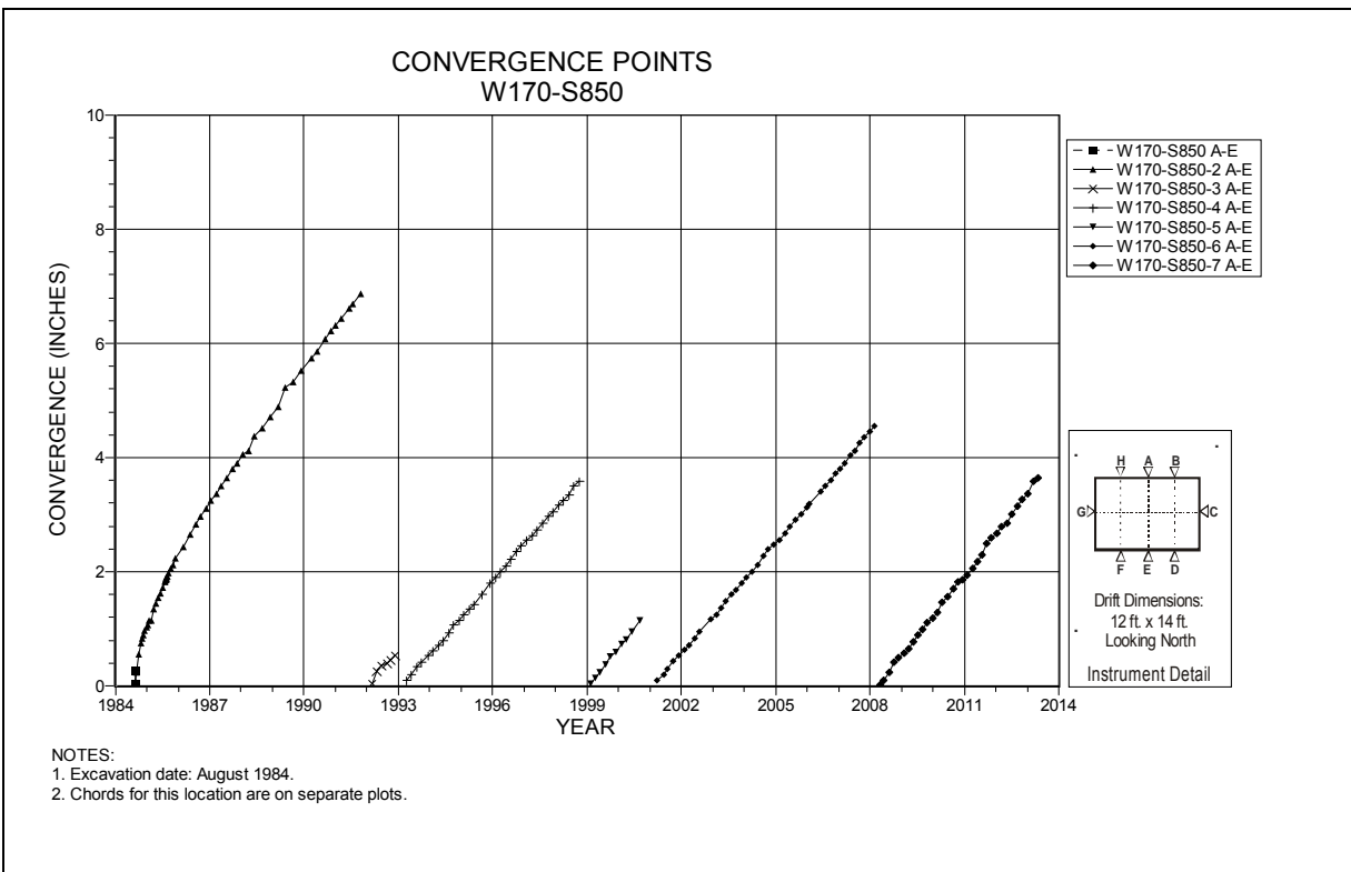
Figure 4-236 Convergence Point Array W170 S850 – Roof to Floor – Centerline
