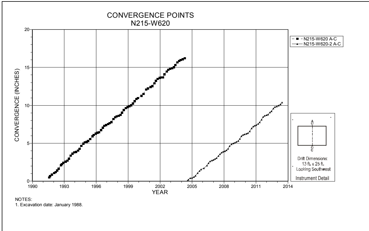
Figure 4-153 Convergence Point Array N215 W620 – Roof to Floor
