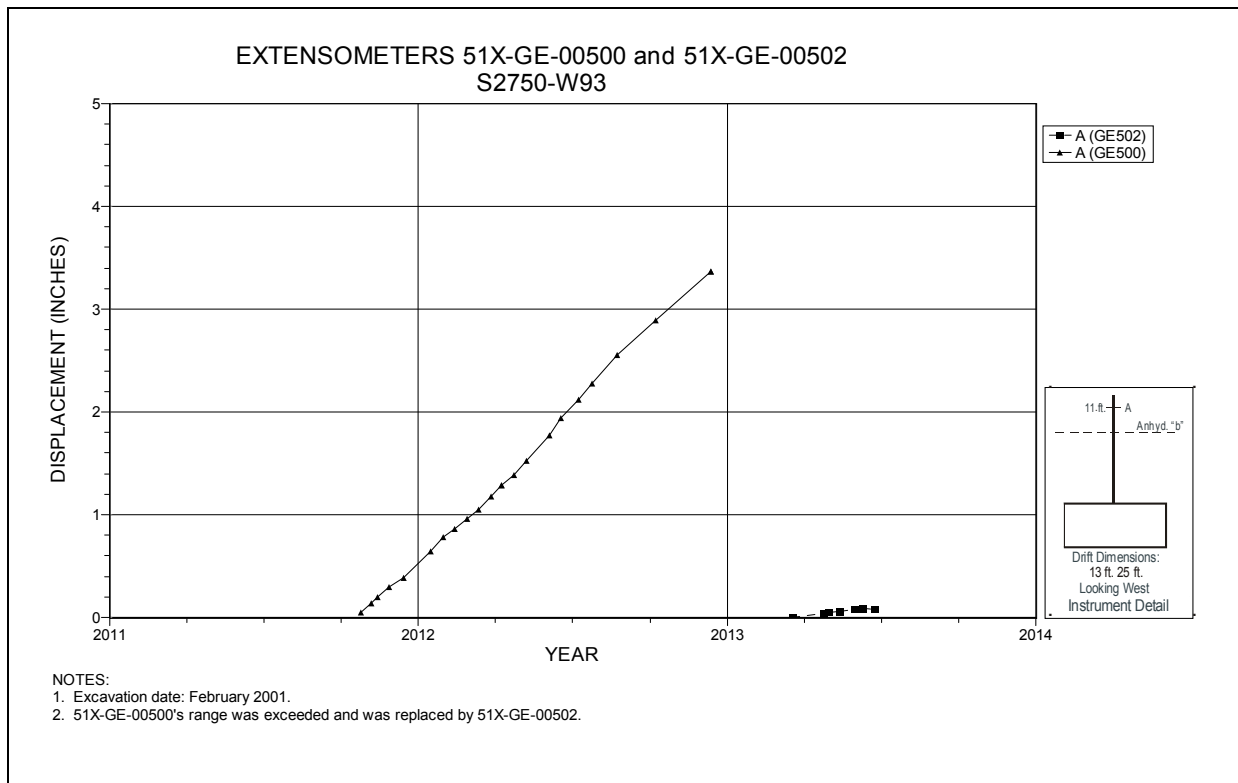
Figure 4-32 Extensometers 51X-GE-00500 and 51X-GE-00502 S2750 W93 – Roof
