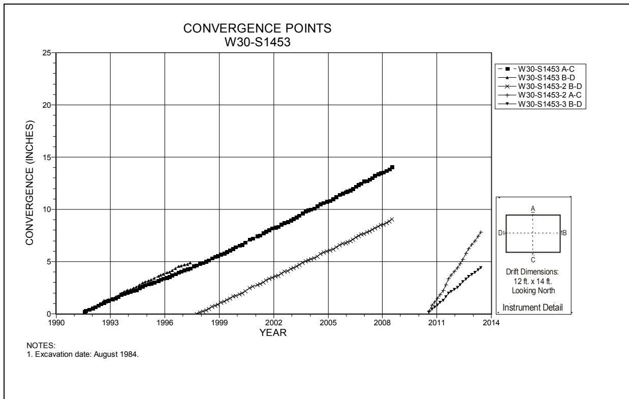
Figure 4-210 Convergence Point Array W30 S1453 – All Chords
