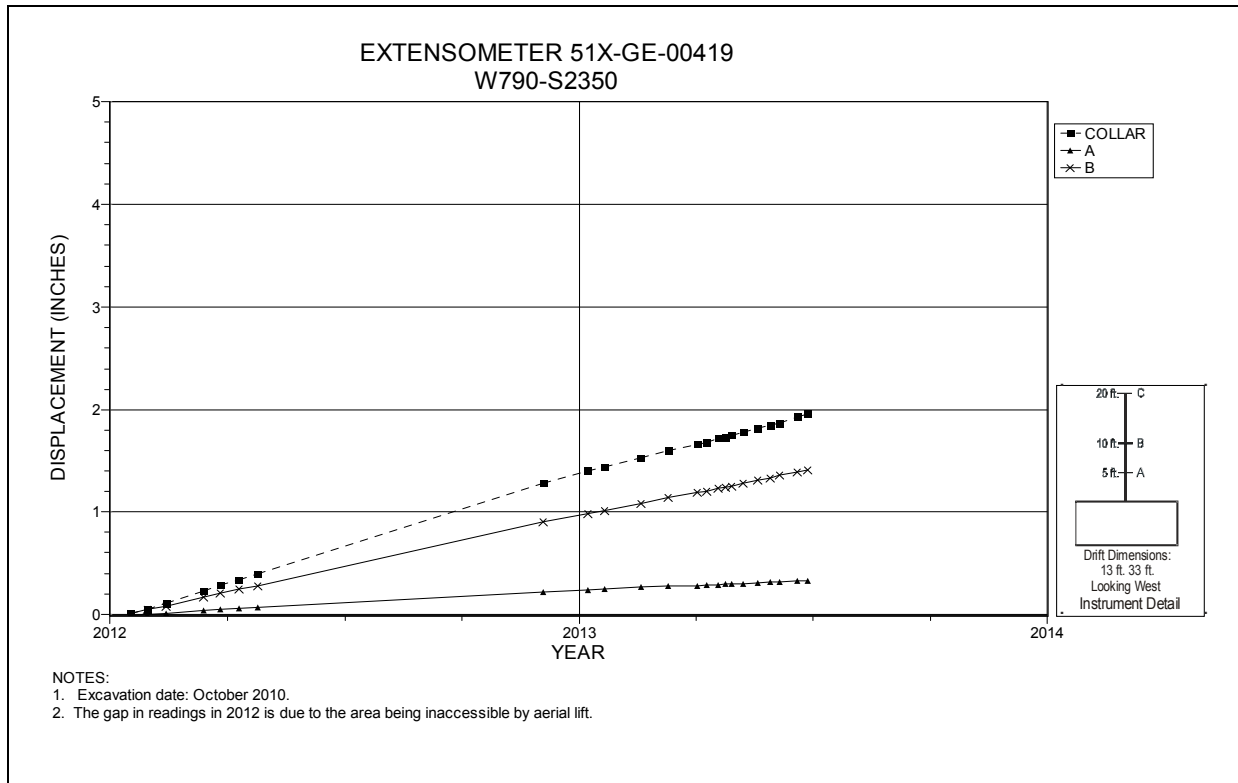
Figure 5-68 Extensometer 51X-GE-00419 Room 4, Panel 7 at W790 S2350 – Room Center – Roof
