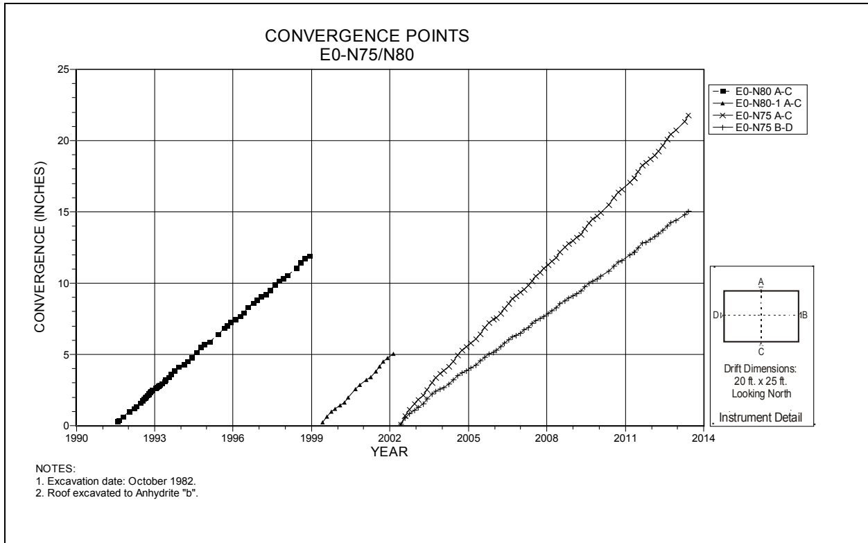
Figure 4-37 Convergence Point Array E0 N75/N80 – All Chords
