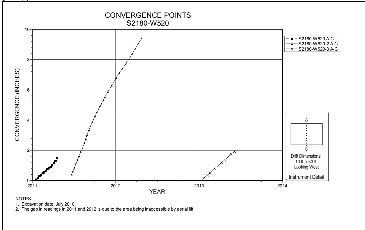
Figure 5-77 Convergence Point Array S2180 W520 Intersection (Room 2, Panel 7) – Roof to Floor
