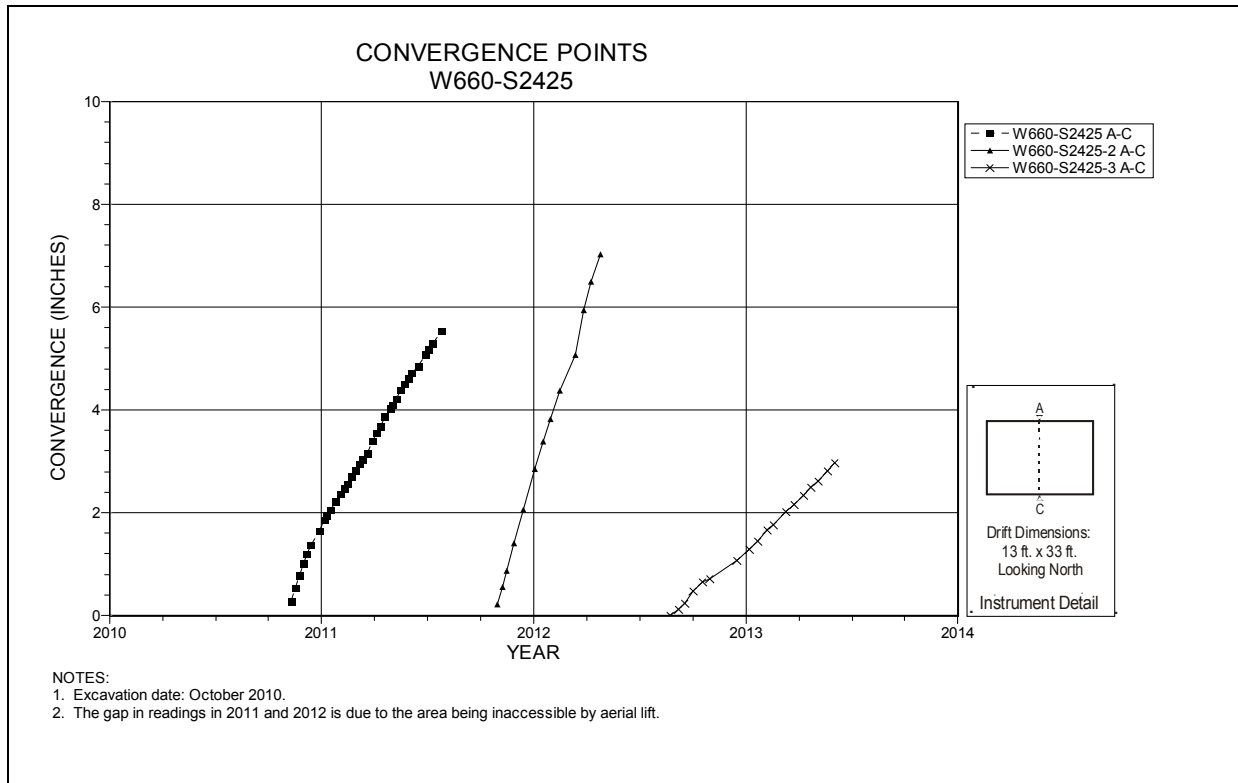
Figure 5-96 Convergence Point Array Room 3, Panel 7 at W660 S2425 – Roof to Floor
