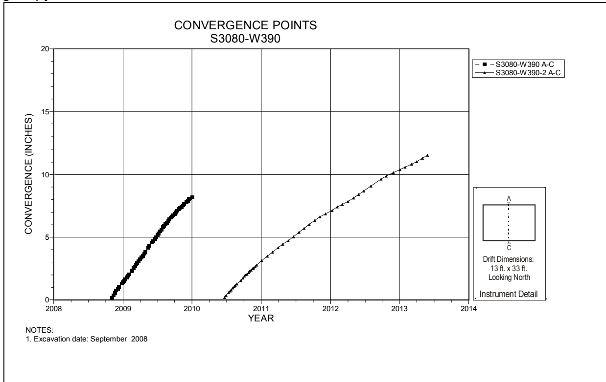
Figure 5-56 Convergence Point Array S3080 W390 Intersection (Room 1, Panel 6) – Roof to Floor
