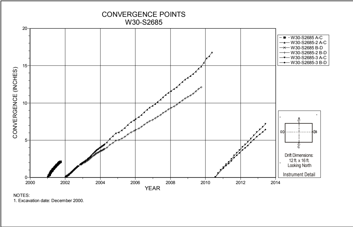
Figure 4-219 Convergence Point Array W30 S2685 – All Chords
