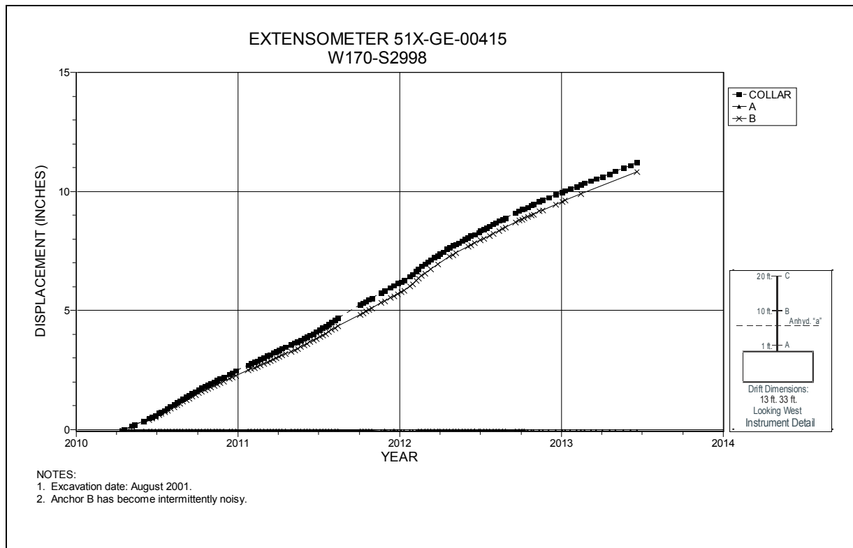
Figure 4-34 Extensometer 51X-GE-00415 W170 S2998 – Roof
