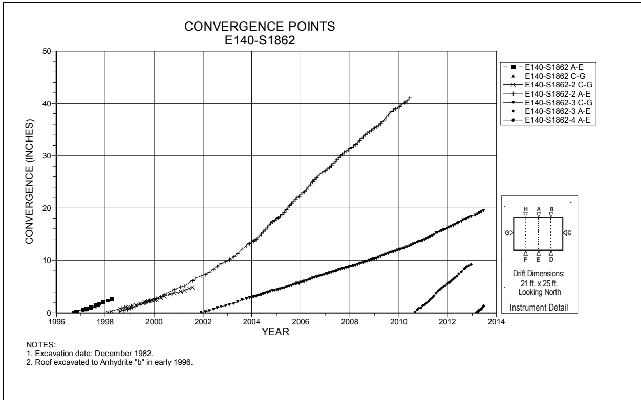
Figure 4-99 Convergence Point Array E140 S1862 – Roof to Floor – Centerline and Rib to Rib
