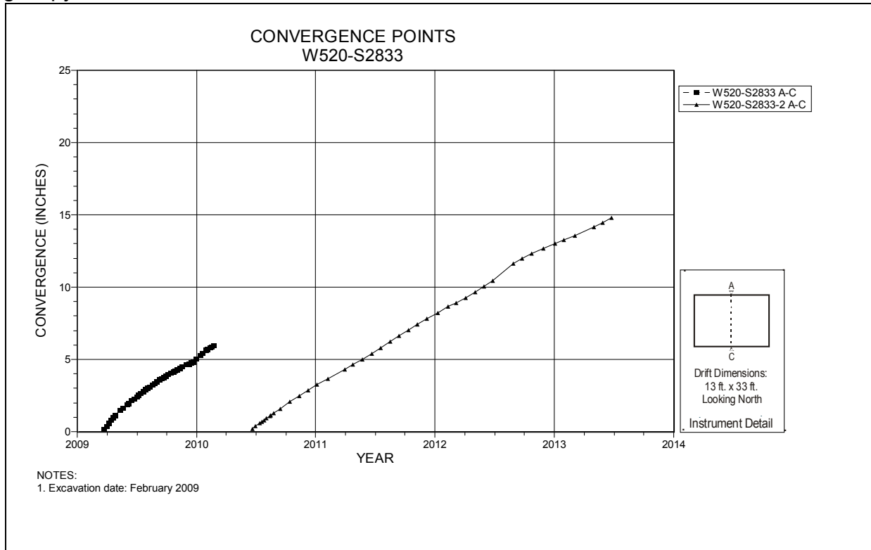
Figure 5-46 Convergence Point Array Room 2, Panel 6 at W520 S2833 – Roof to Floor
