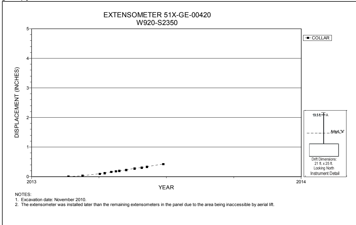
Figure 5-69 Extensometer 51X-GE-00420 Room 5, Panel 7 at W920 S2350 – Room Center – Roof
