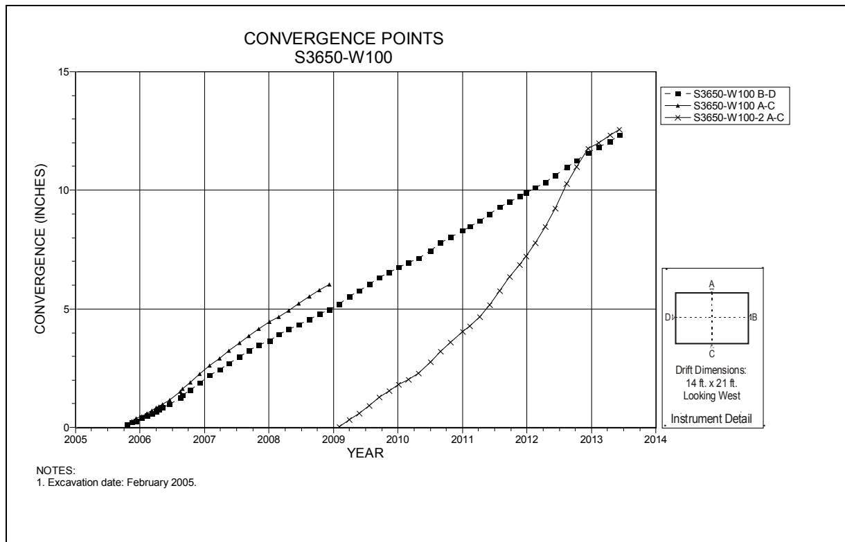
Figure 4-198 Convergence Point Array S3650 W100 – All Chords
