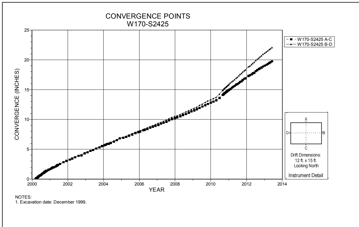
Figure 4-252 Convergence Point Array W170 S2425 – All Chords
