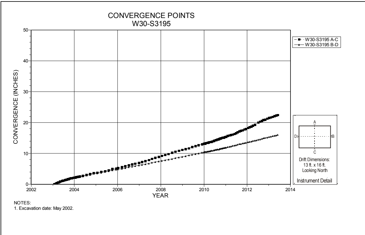
Figure 4-225 Convergence Point Array W30 S3195 – All Chords
