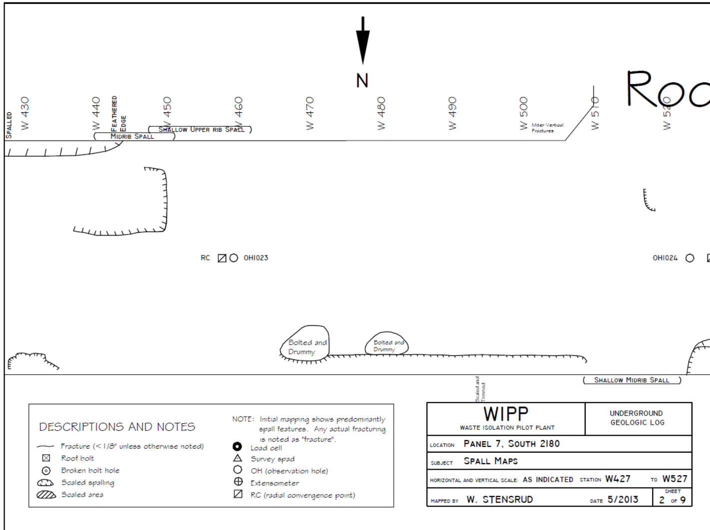
Figure 7-30 Panel 7 South 2180, W427-W527 Roof Fractures
