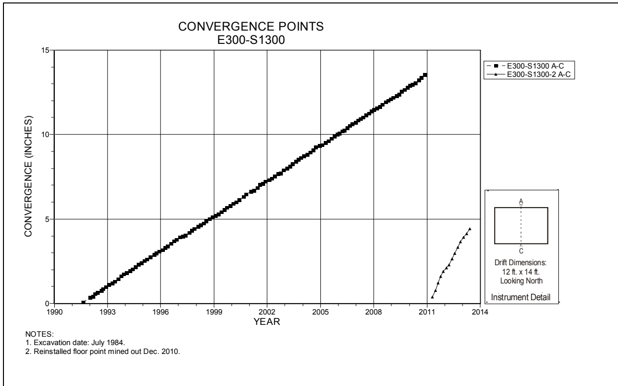
Figure 4-136 Convergence Point Array E300 S1300 – Roof to Floor
