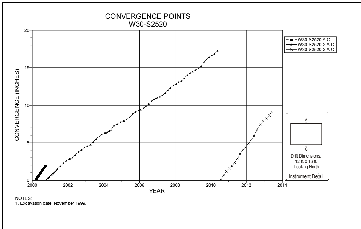
Figure 4-218 Convergence Point Array W30 S2520 – Roof to Floor
