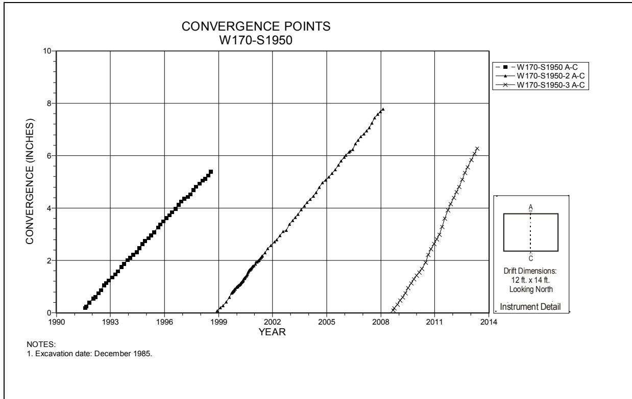
Figure 4-247 Convergence Point Array W170 S1950 – Roof to Floor
