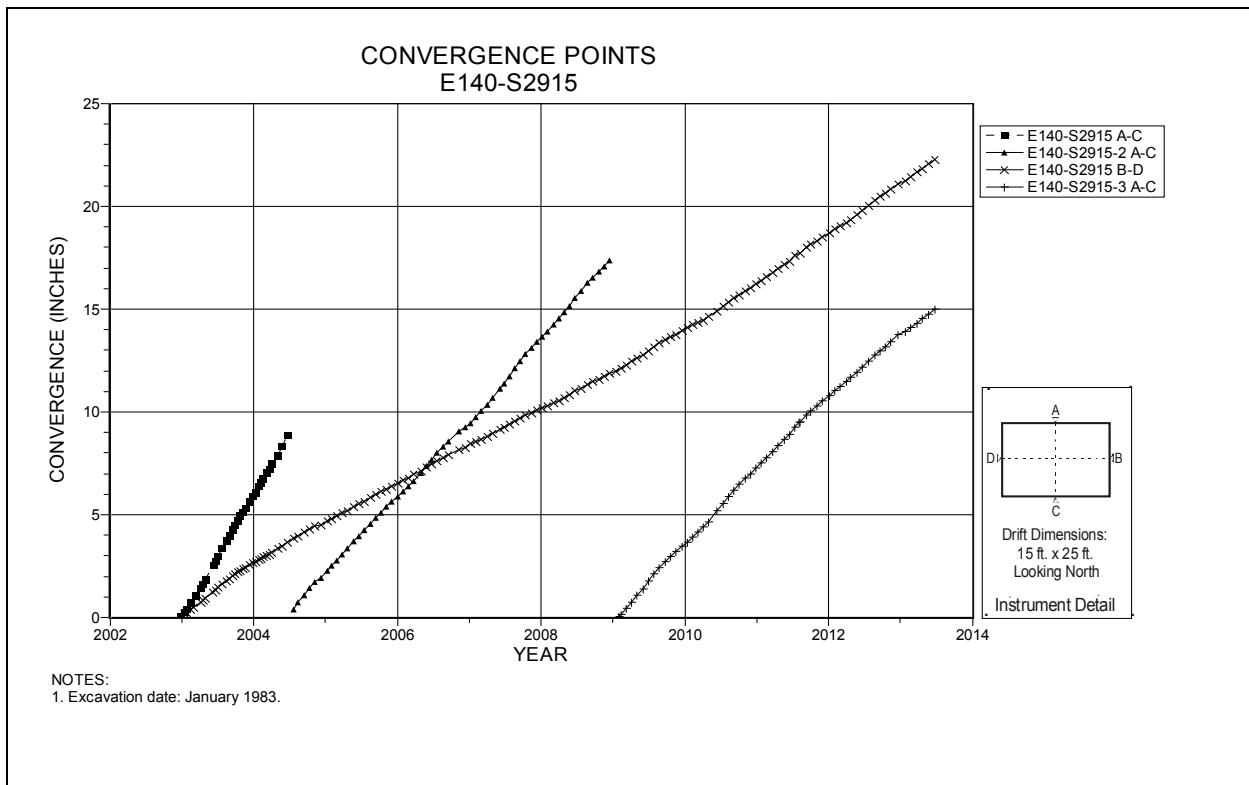
Figure 4-112 Convergence Point Array E140 S2915 – All Chords
