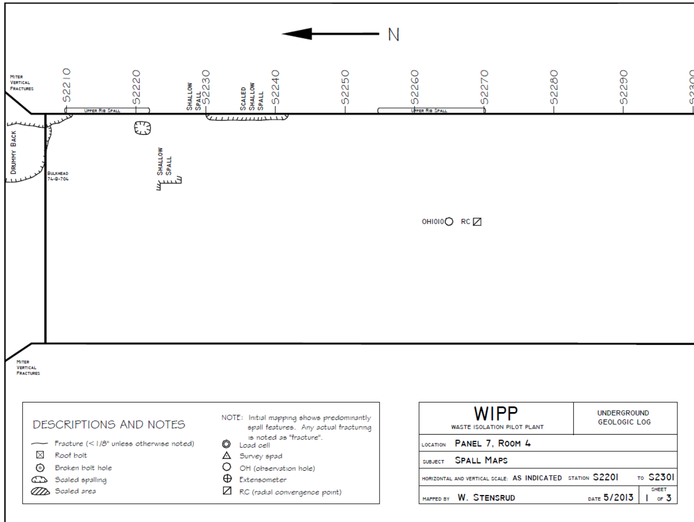
Figure 7-17 Panel 7 Room 4, S2201-S2301 Roof Fractures
