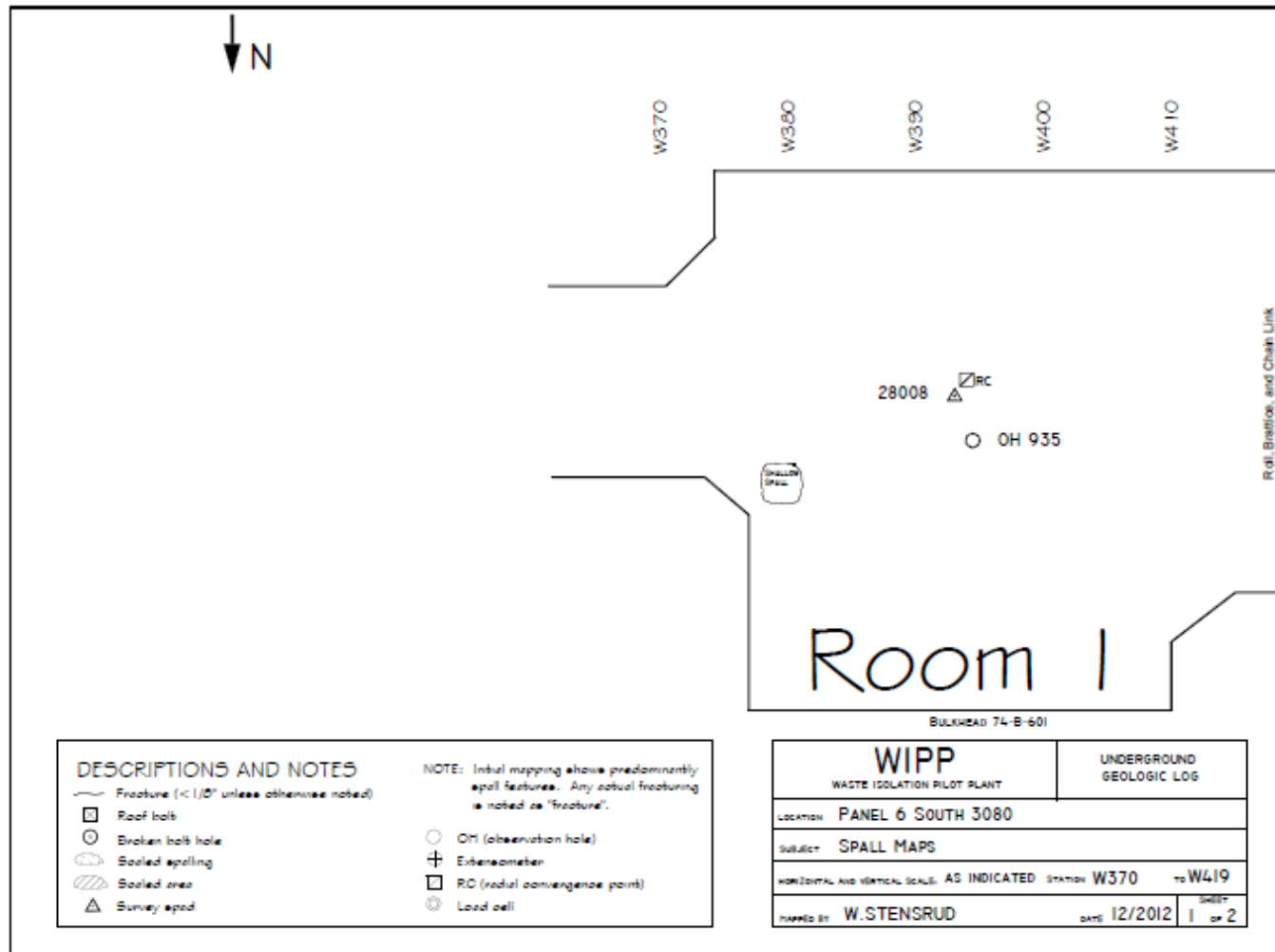
Figure 7-6 Panel 6 South 3080, W370-W419 Roof Fractures
