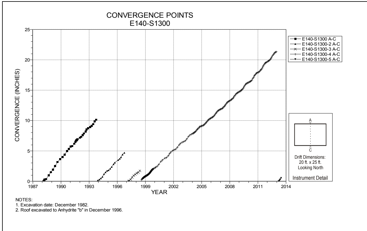
Figure 4-81 Convergence Point Array E140 S1300 – Roof to Floor
