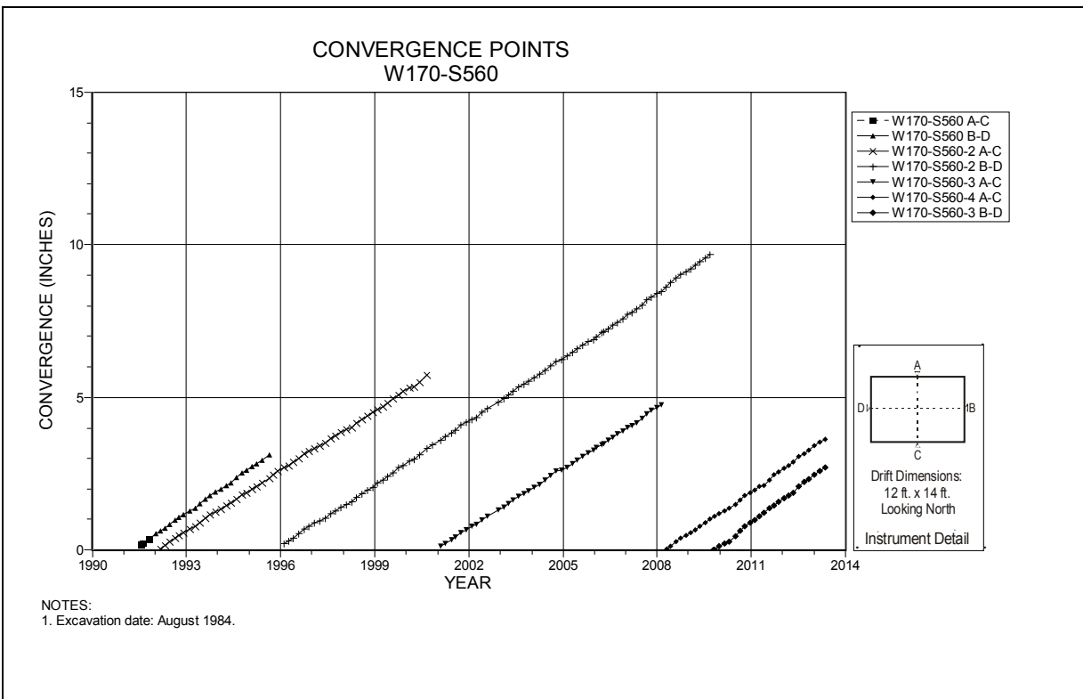
Figure 4-234 Convergence Point Array W170 S560 – All Chords
