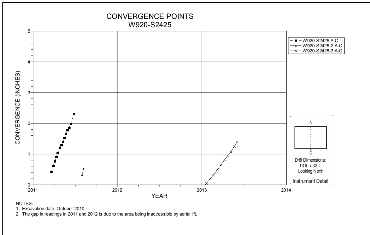
Figure 5-102 Convergence Point Array Room 5, Panel 7 at W920 S2425 – Roof to Floor
