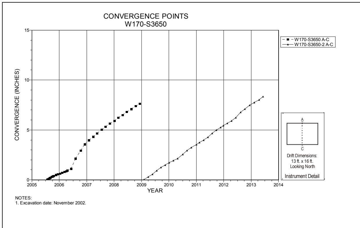
Figure 4-264 Convergence Point Array W170 S3650 – Roof to Floor
