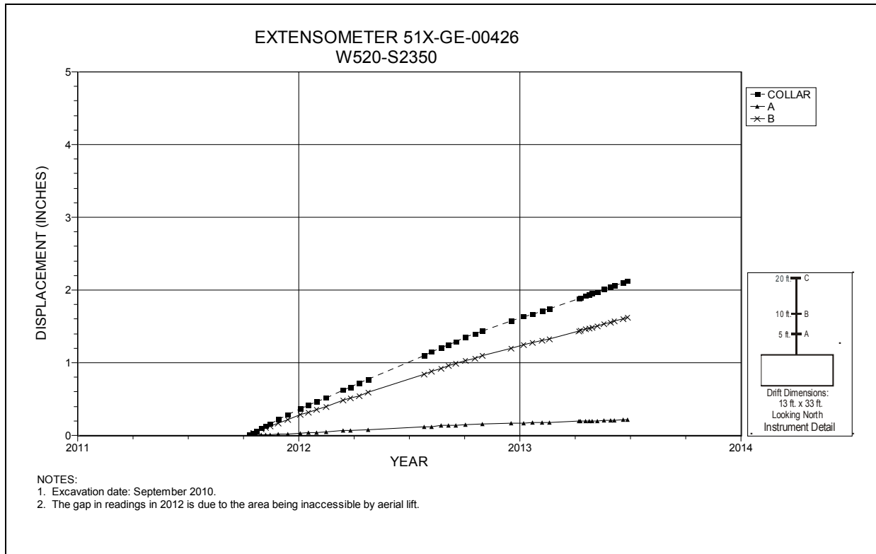
Figure 5-66 Extensometer 51X-GE-00426 Room 2, Panel 7 at W520 S2350 – Room Center – Roof
